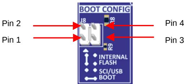
Figure 28. Boot Configuration Jumper J8
