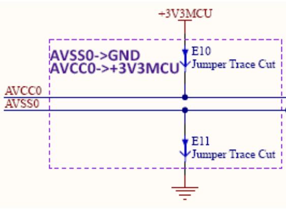
Figure 29. Analog and Reference Voltages
