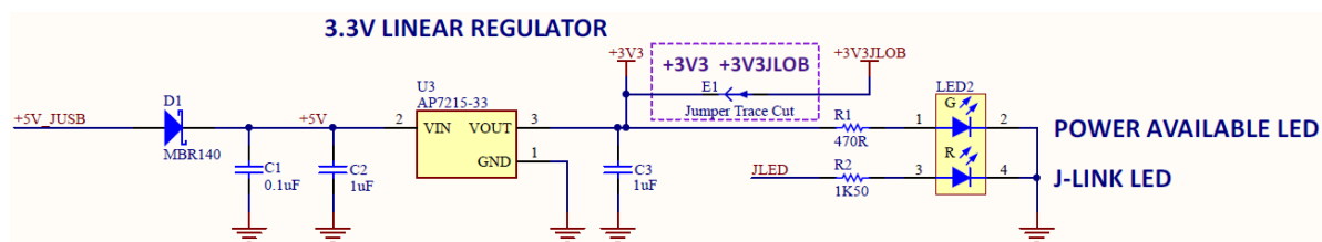
Figure 10. 3.3 V Power Regulator Circuit
