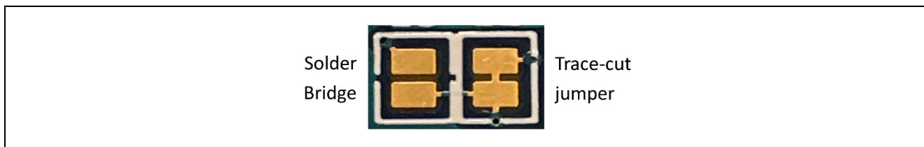
Figure 4. Copper Jumpers
