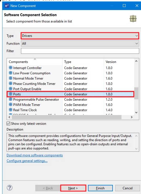
Figure 4-18 Select Ports
