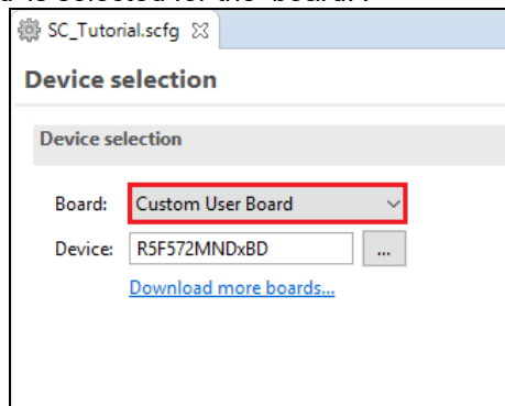
Figure 4-3 Select board
