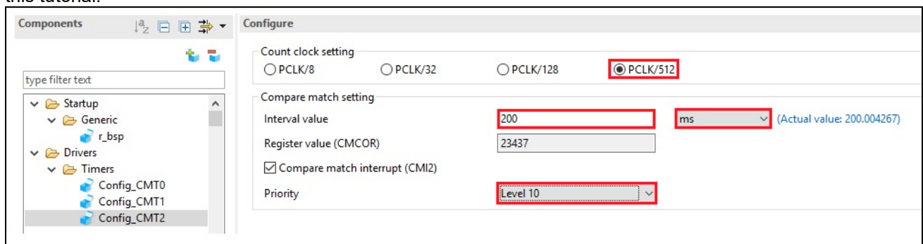
Figure 4-14 Config_CMT2 setting
