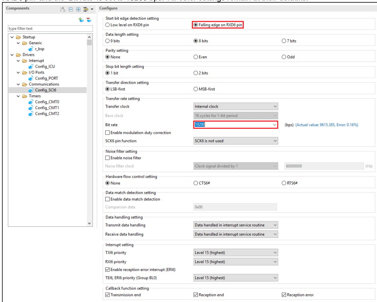
Figure 4-33 Config_SCI6 setting
