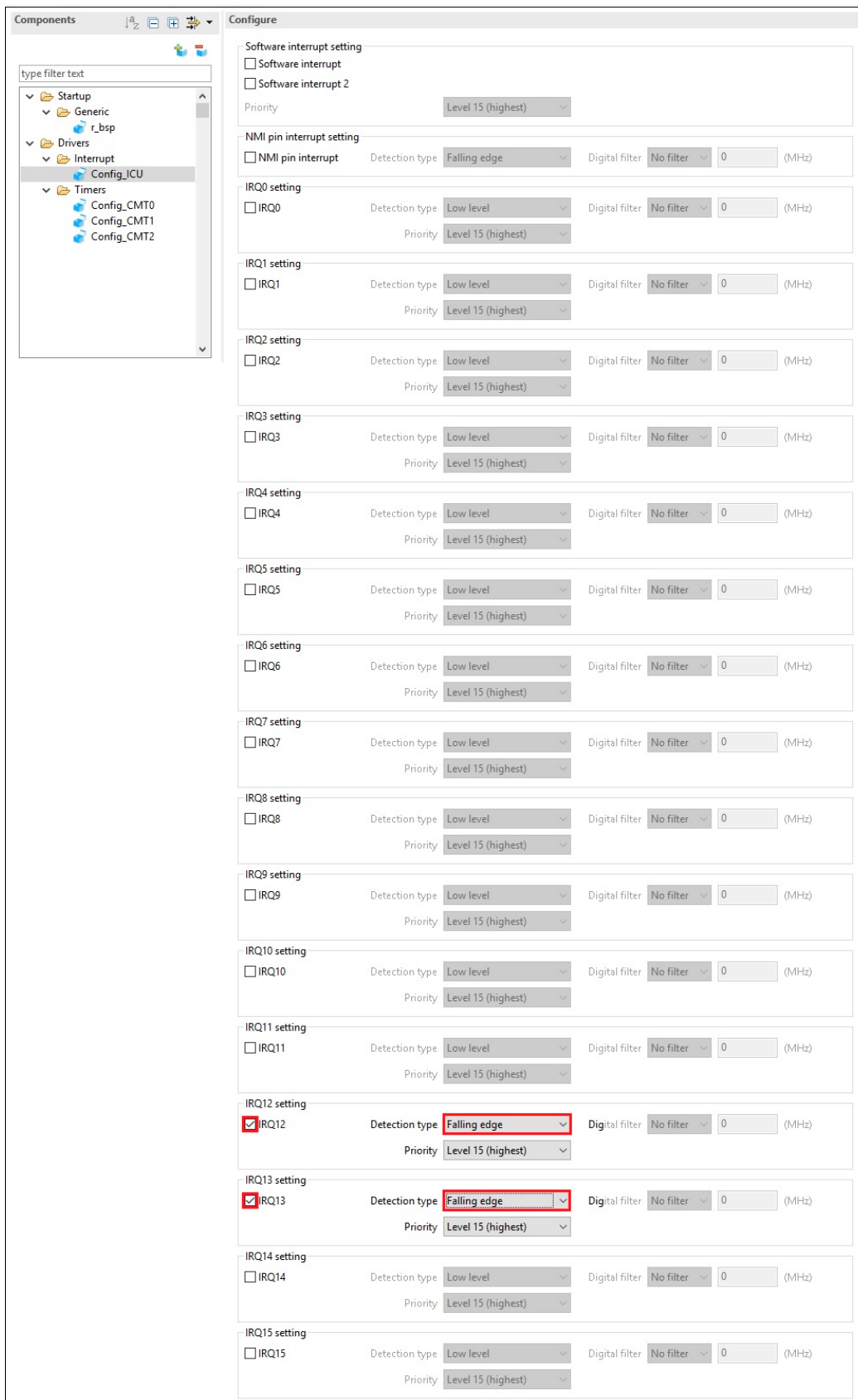
Figure 4-17 Config_ICU setting
