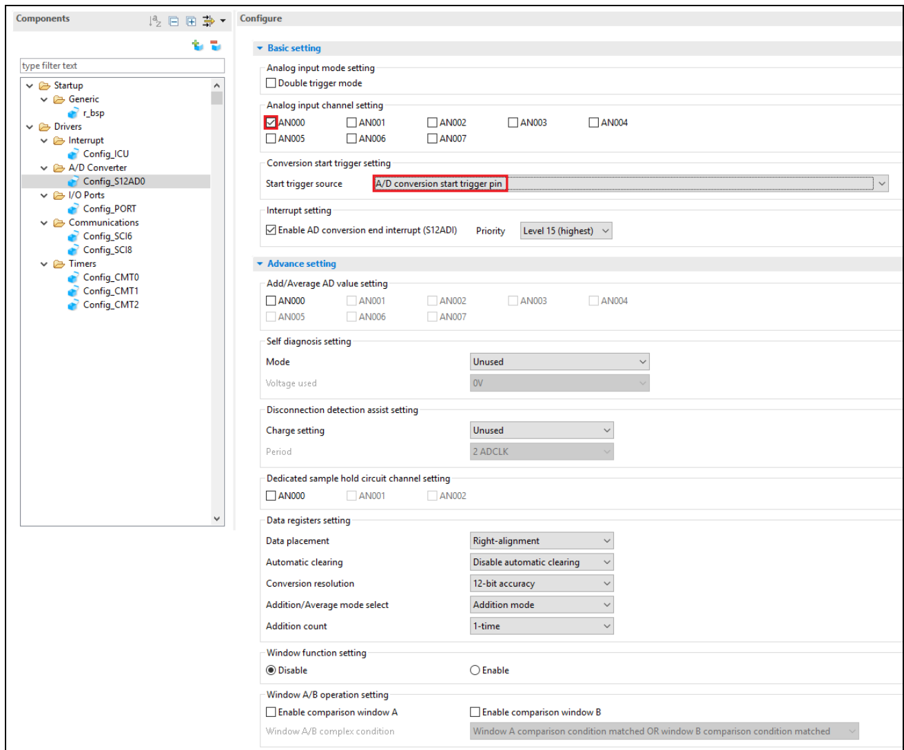
Figure 4-41 Config_S12AD0 setting (1)
