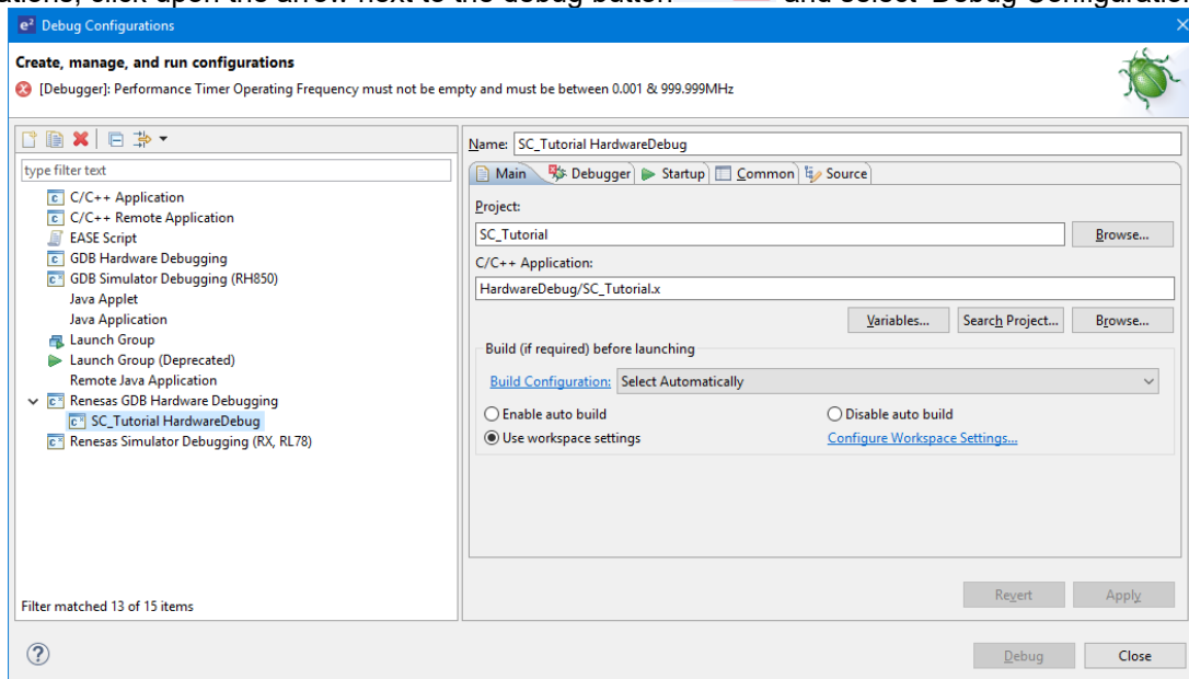
Figure 6-1 Debug Configurations
