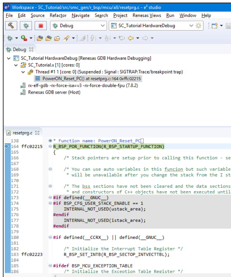
Figure 6-5 Debugger start up screen
