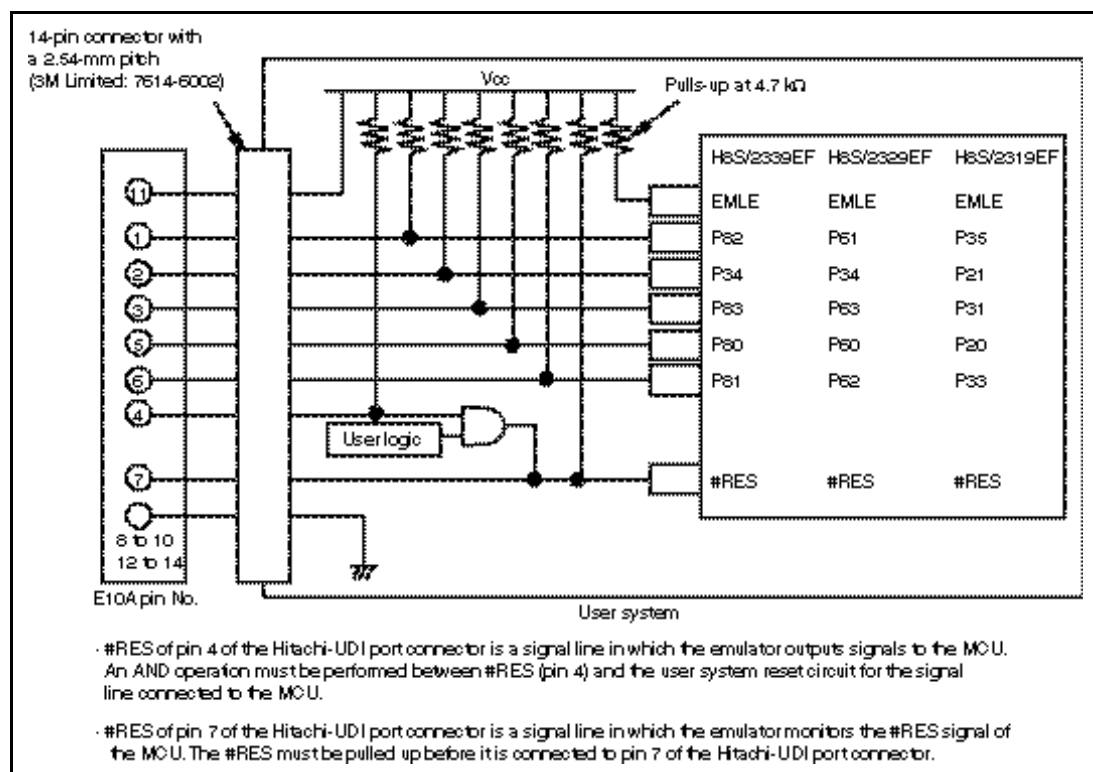
Figure 4.1 Example of Emulator Connection
