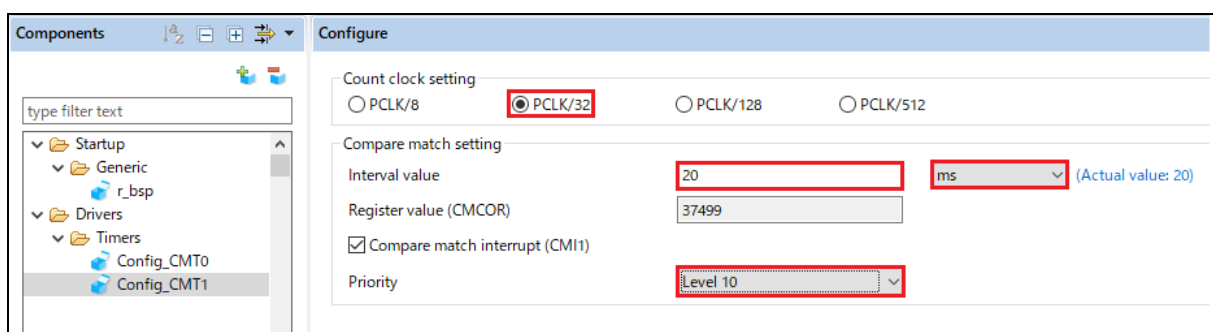
Figure 4-16 Config_CMT1 setting
