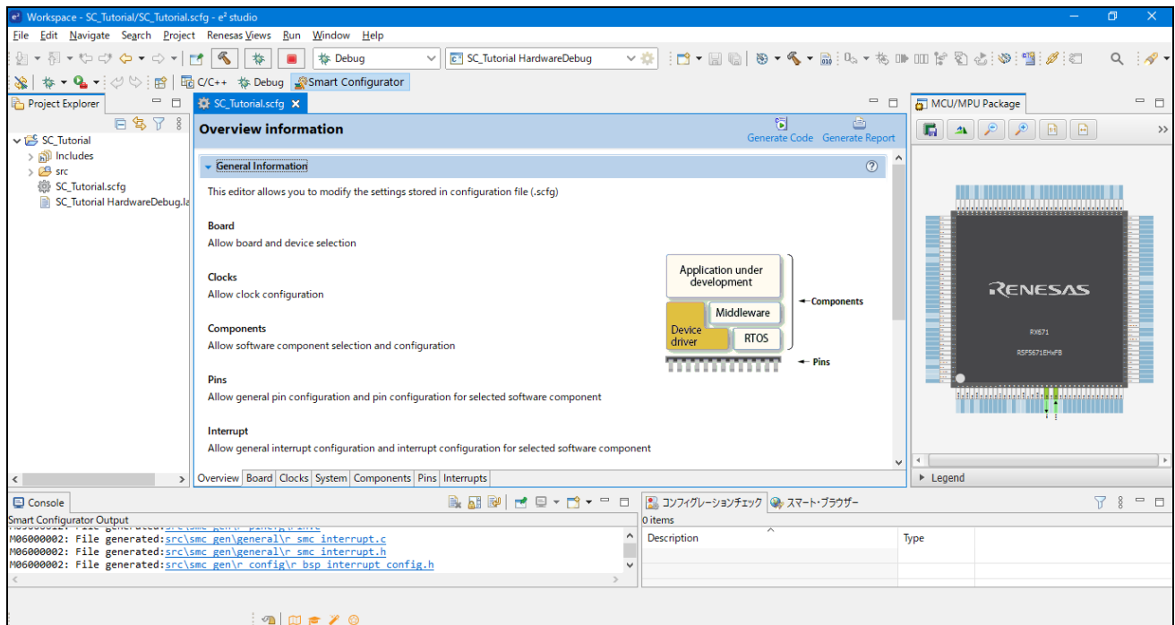
Figure 4-1 Overview page
