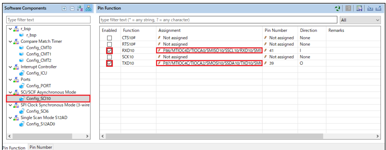
Figure 4-48 Configure pin assignment - Config_SCI10
