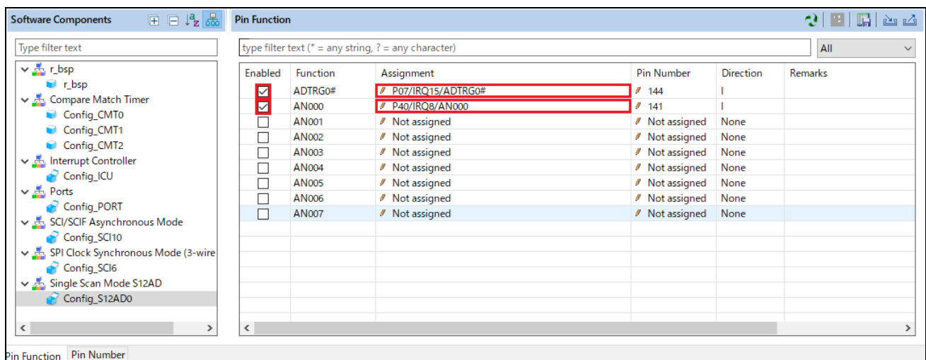
Figure 4-50 Configure pin assignment - Config_S12AD0
