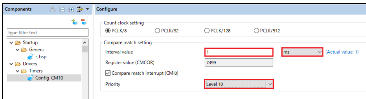
Figure 4-13 Config_CMT0 setting
