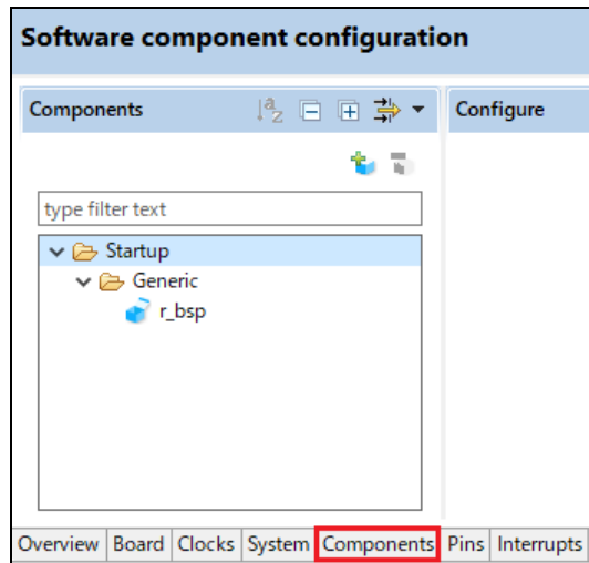
Figure 4-7 Components page
