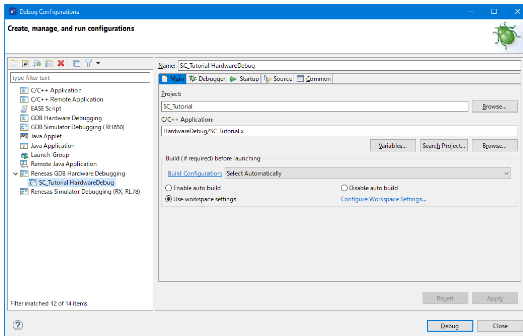
Figure 6-1 Debug Configurations
