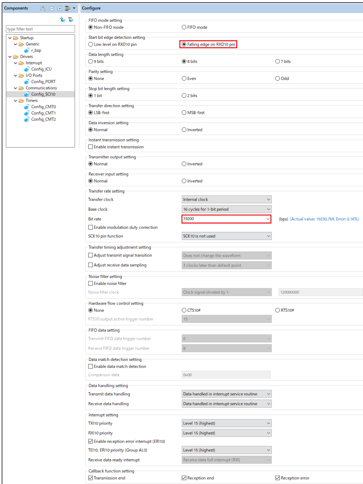
Figure 4-35 Config_SCI10 setting
