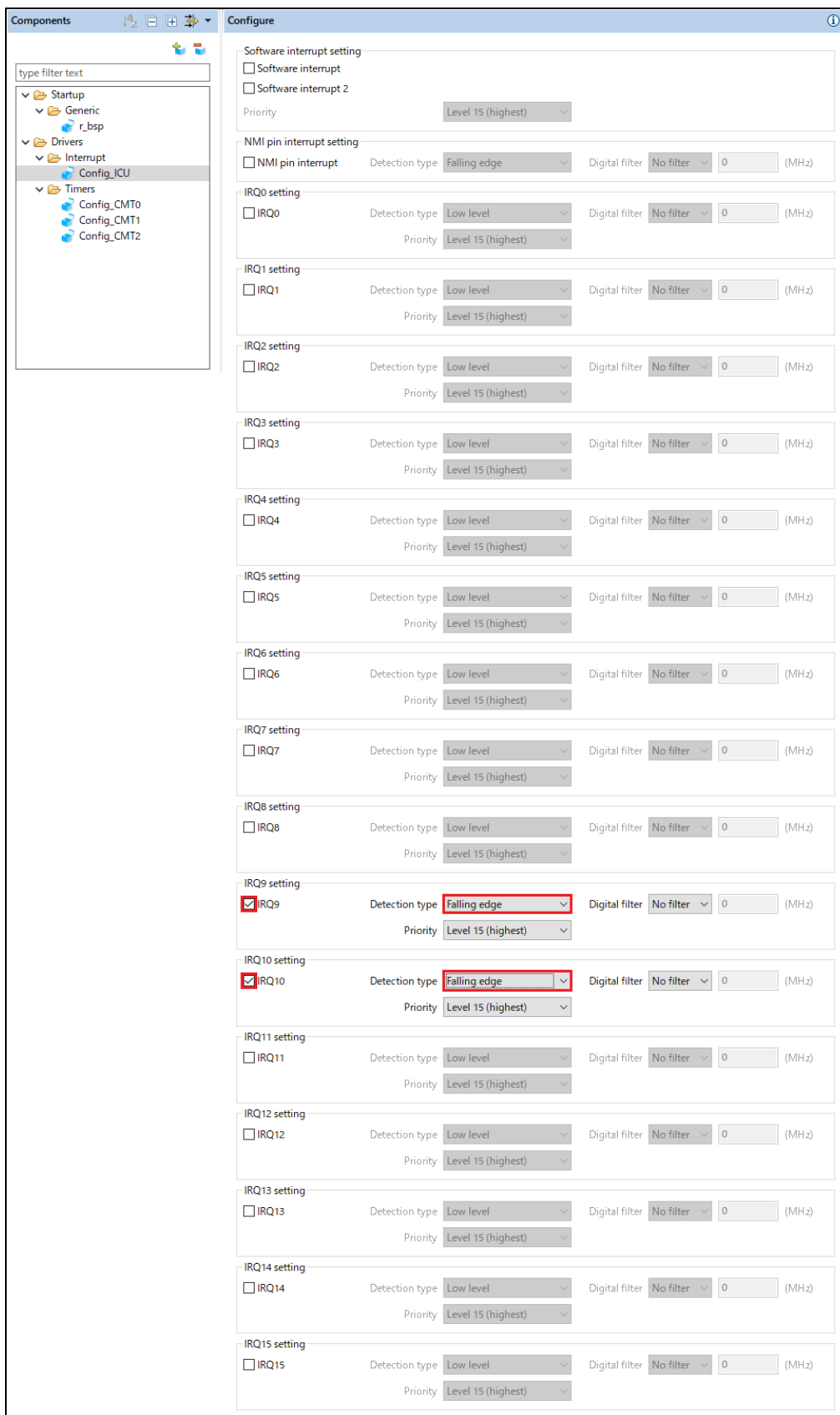
Figure 4-22 Config_ICU setting
