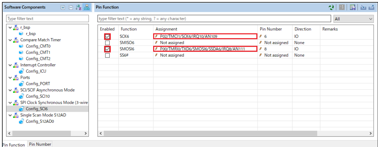
Figure 4-49 Configure pin assignment - Config_SCI6
