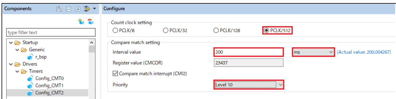
Figure 4-19 Config_CMT2 setting
