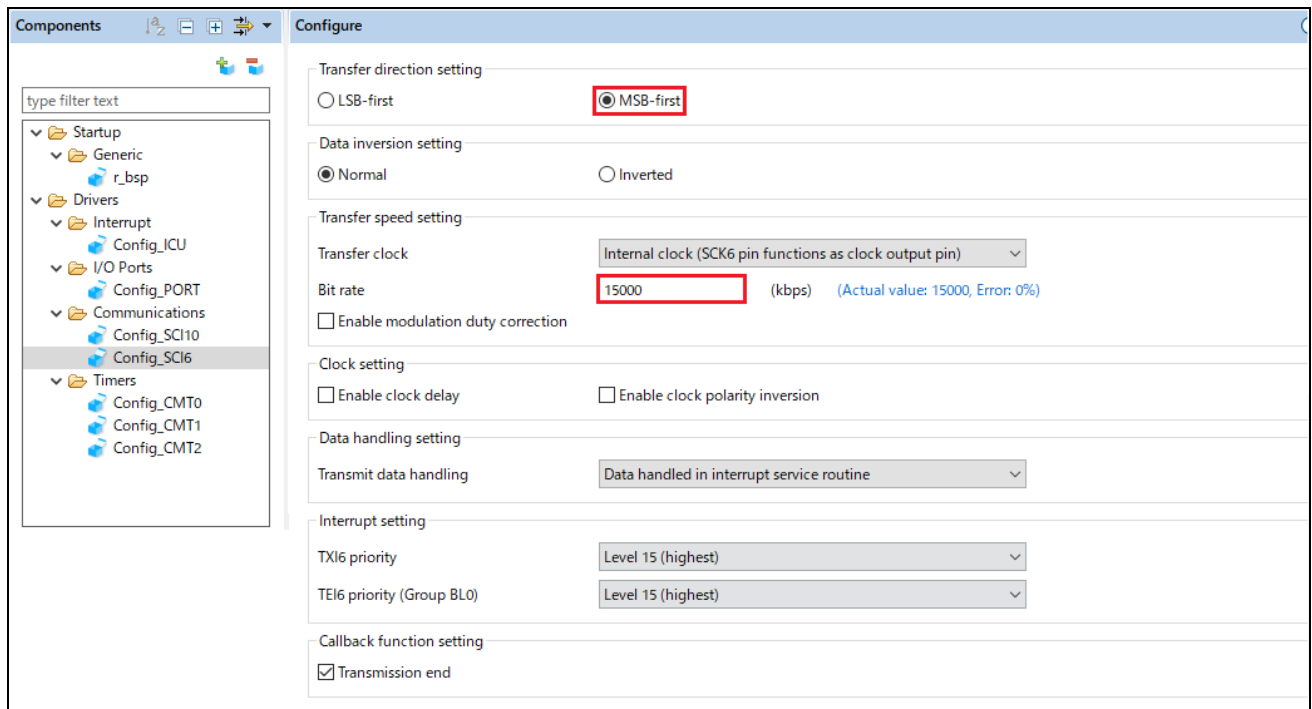
Figure 4-40 Config_SCI6 setting
