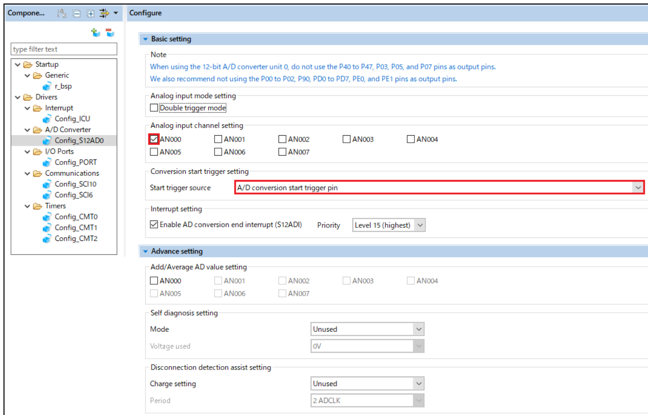
Figure 4-43 Config_S12AD0 setting (1)
