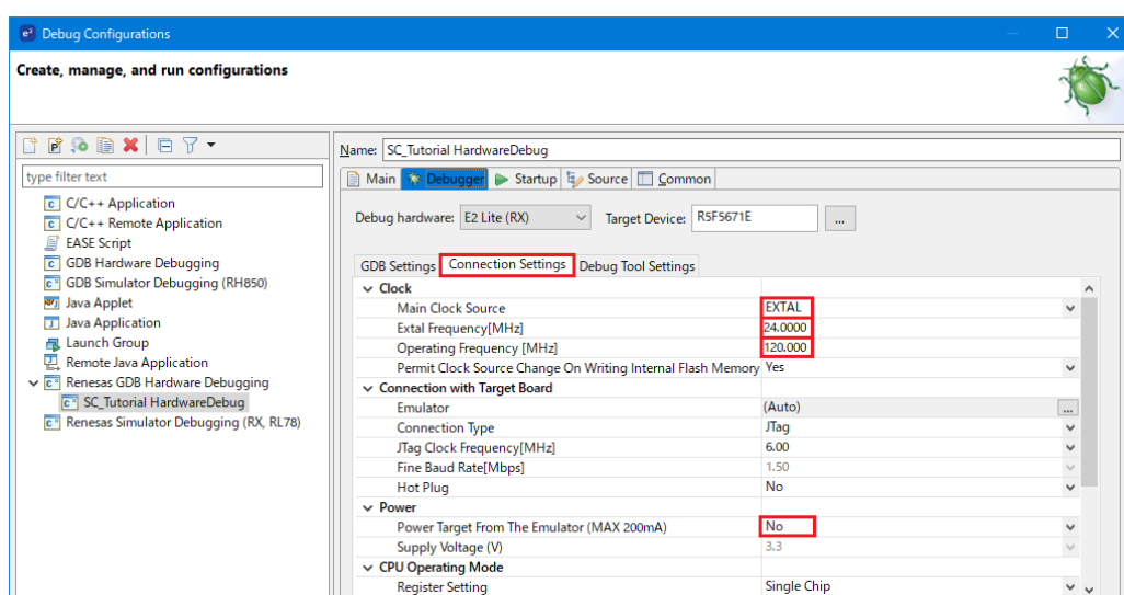
Figure 6-2 Connection Settings
