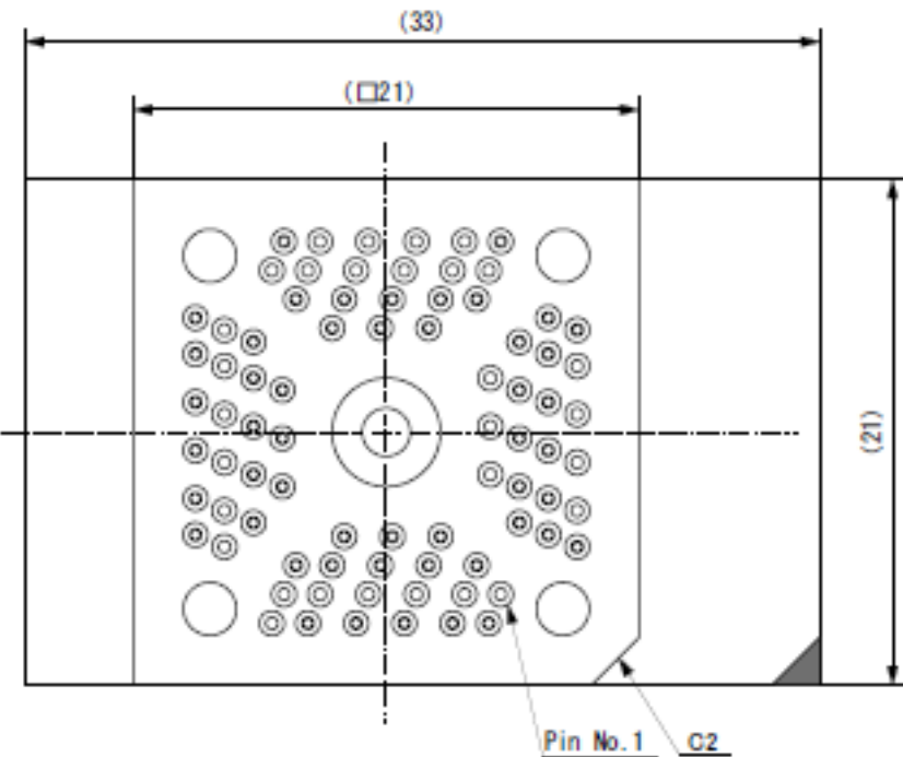
< Bottom view >
