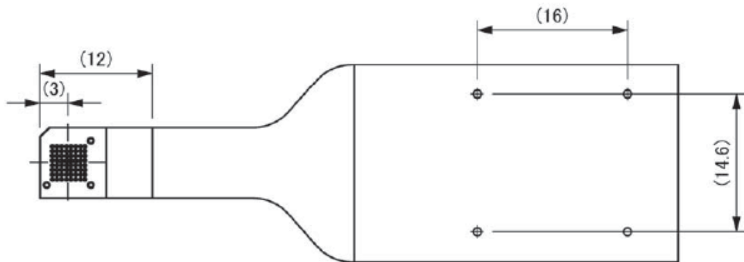
< Bottom view >
