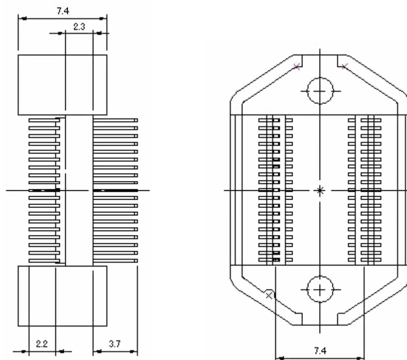
< Bottom view >
