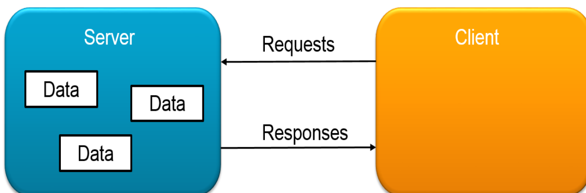
Figure 1: Client-Server Architecture
