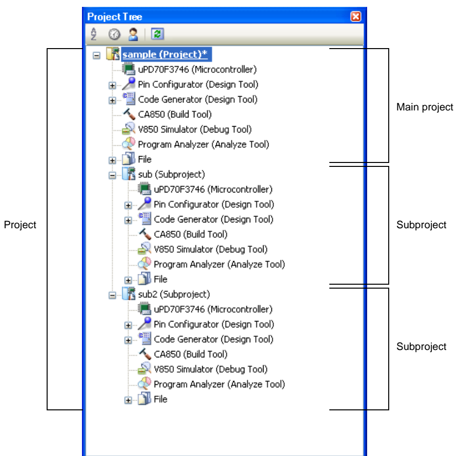
Figure 2-43. Project Tree Panel (When Subprojects Added)
