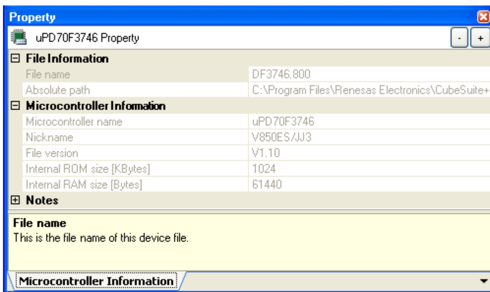
Figure A-23. Property Panel : [Microcontroller Information] Tab
