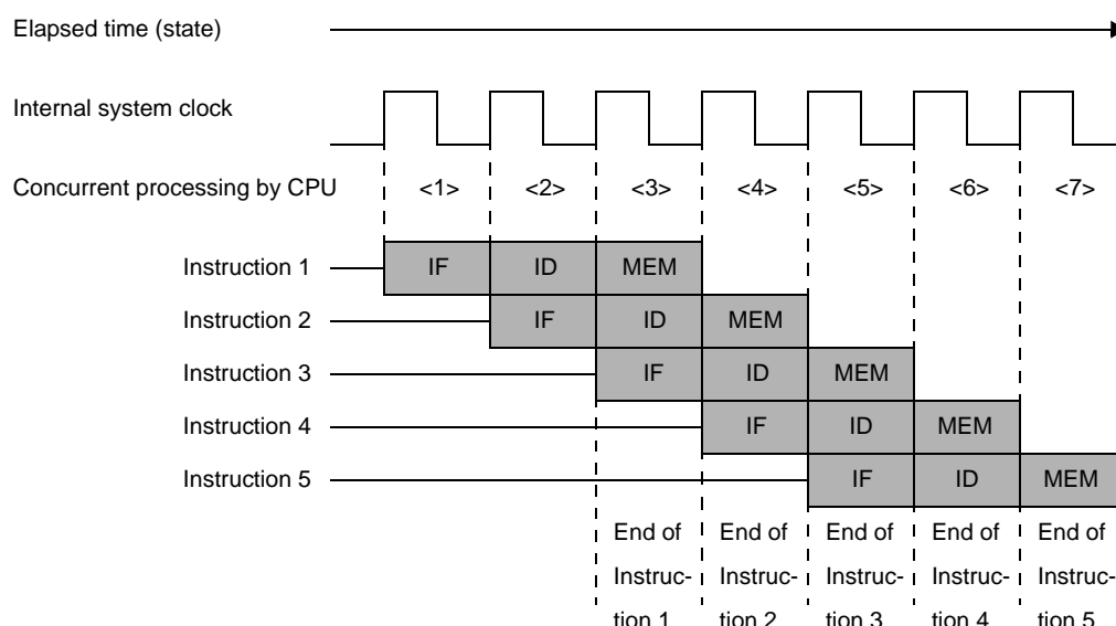
Figure 4-38. Pipeline Execution of Five Typical Instructions (Example)
