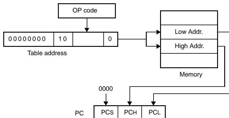
Figure 4-19. How Table Indirect Addressing Works
