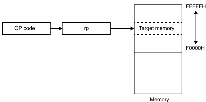
Figure 4-28. Example of ES:[DE] and ES:[HL] Addressing
