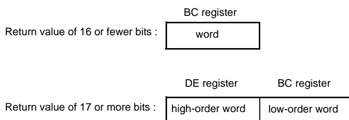
Figure 9-6. Argument Passing
