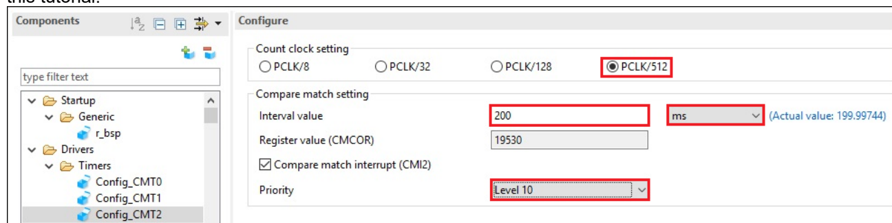
Figure 4-15 Config_CMT2 setting
