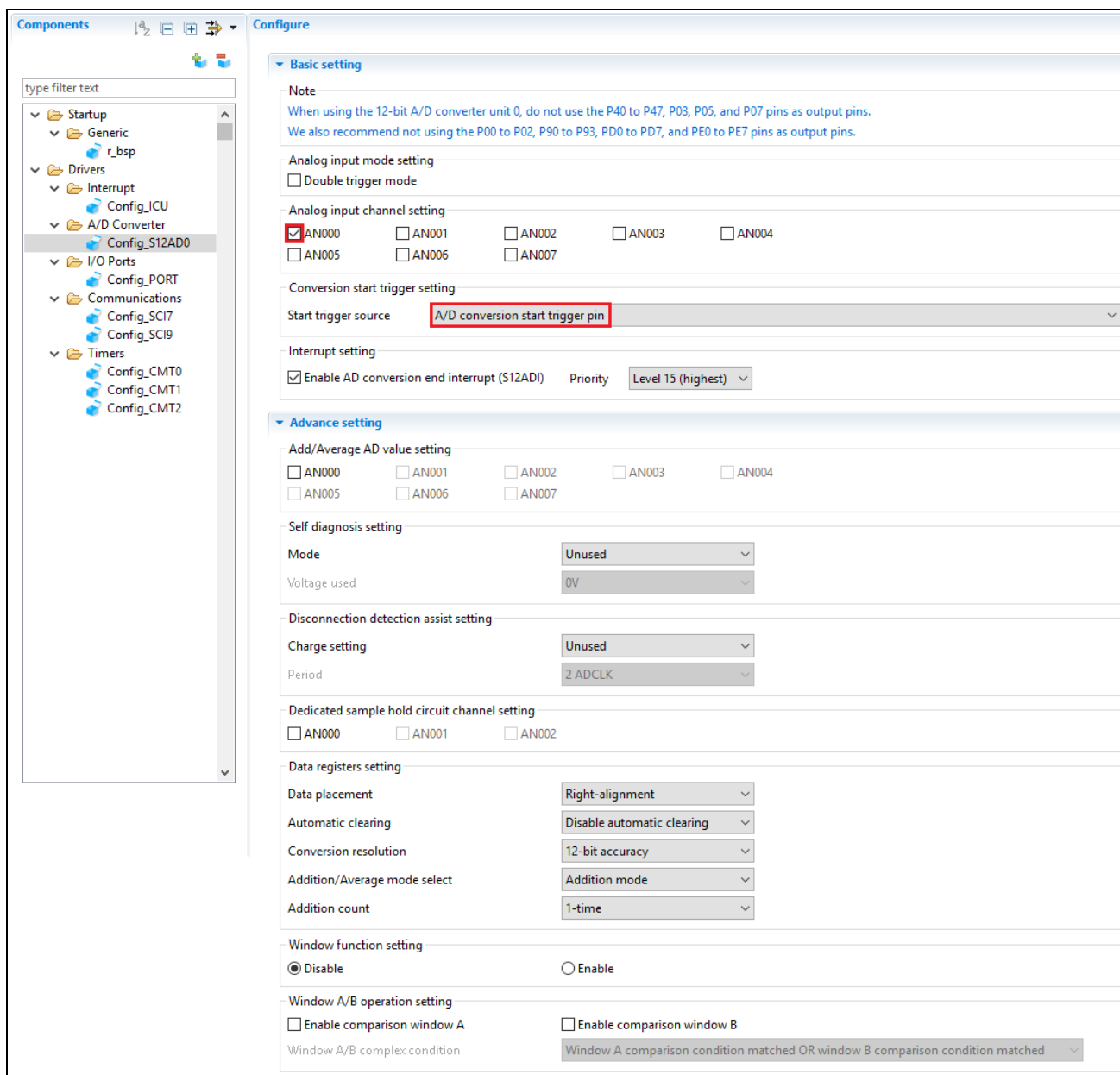
Figure 4-41 Config_S12AD0 setting (1)
