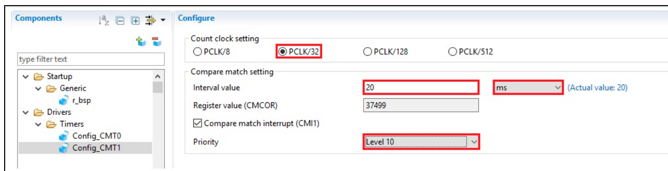
Figure 4-14 Config_CMT1 setting
