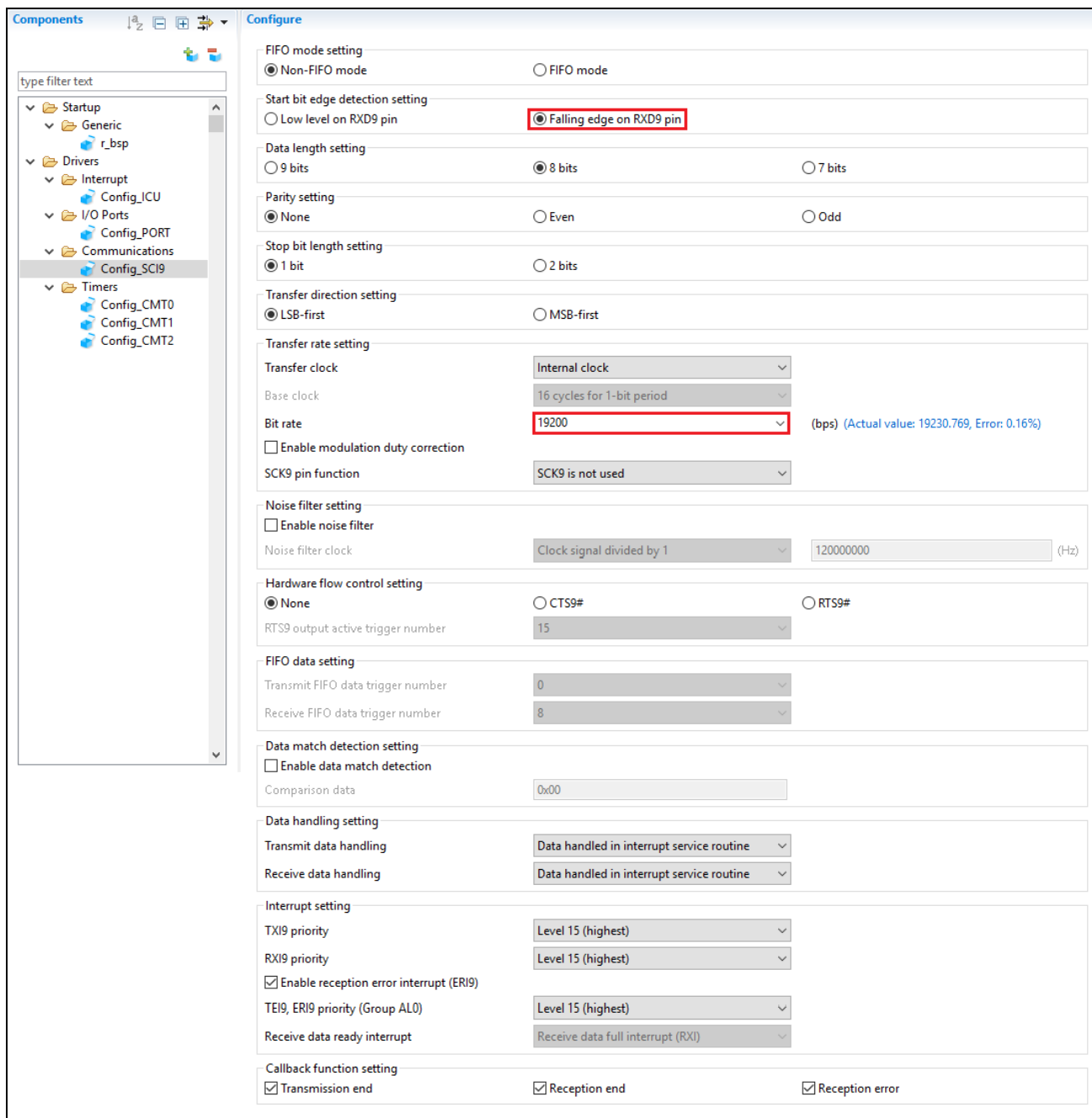
Figure 4-33 Config_SCI9 setting
