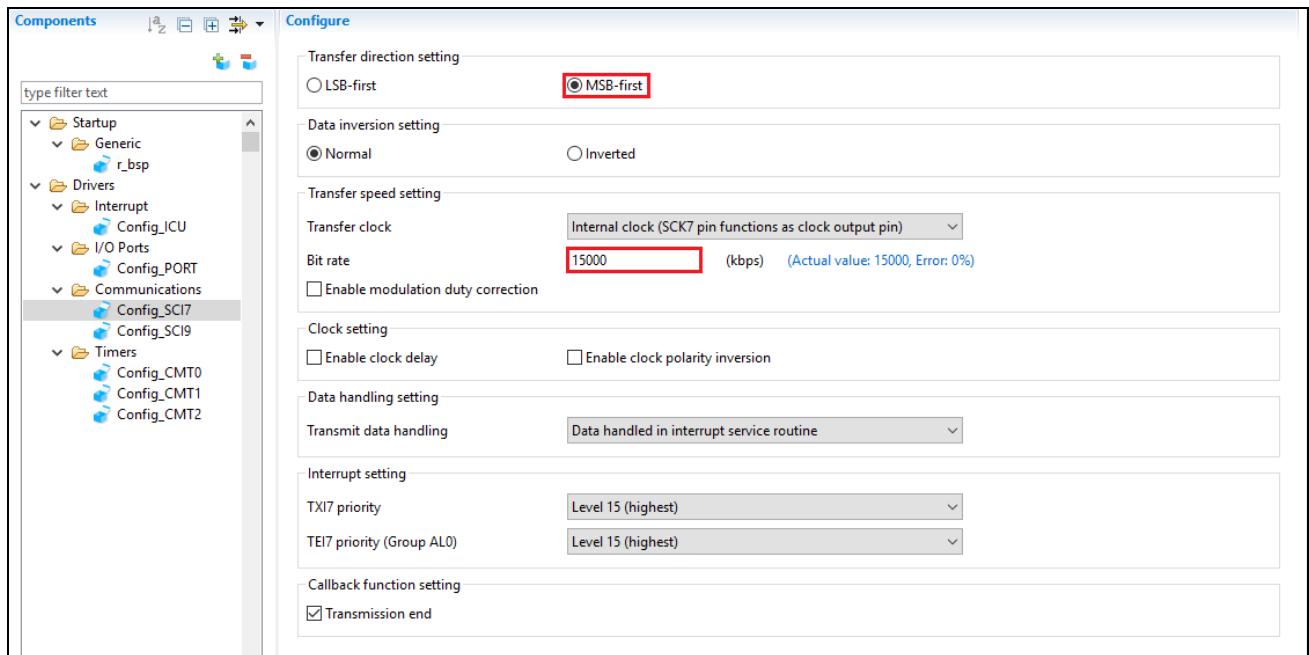
Figure 4-38 Config_SCI7 setting
