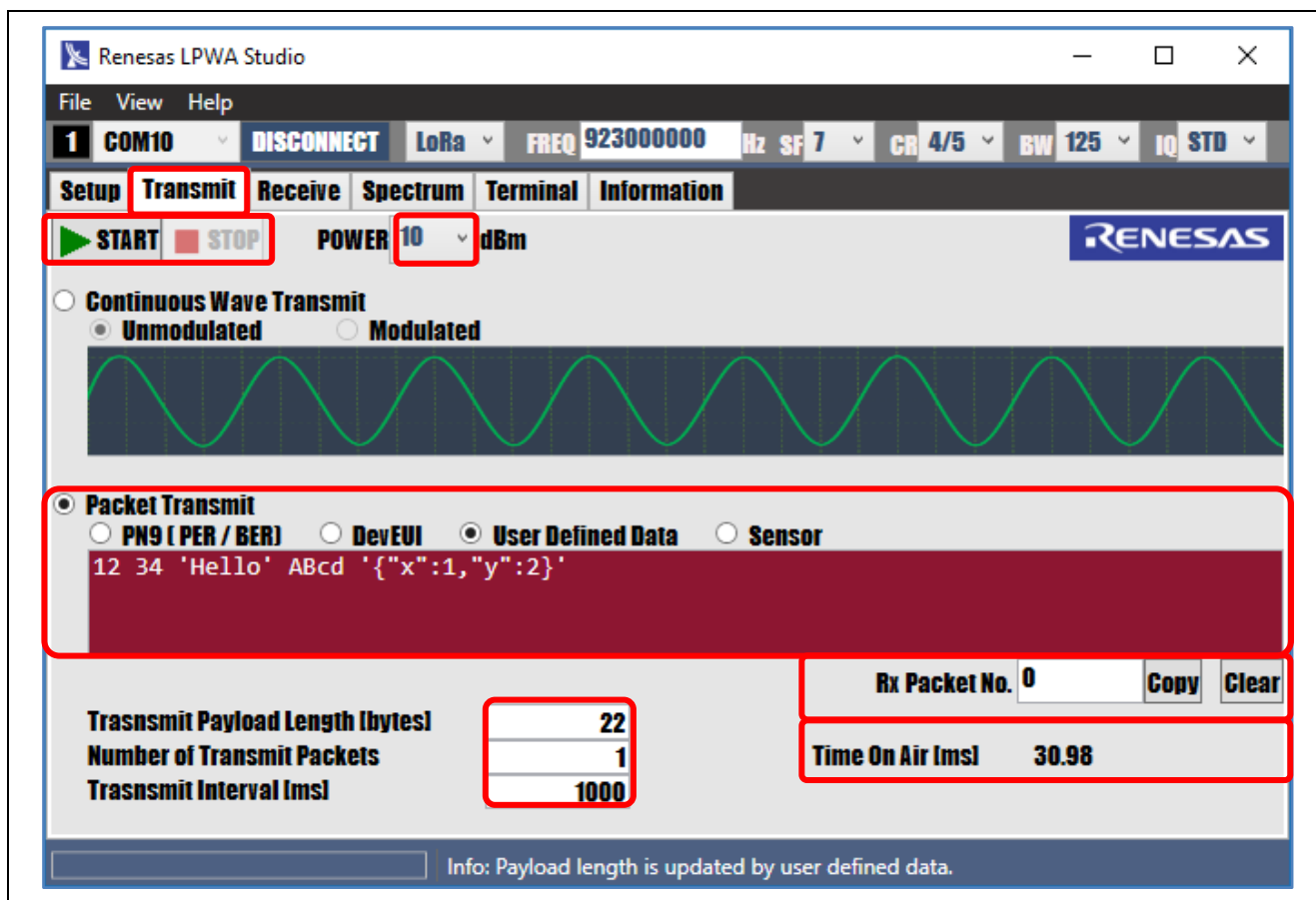
Figure 12. Packet Transmission Parameters
