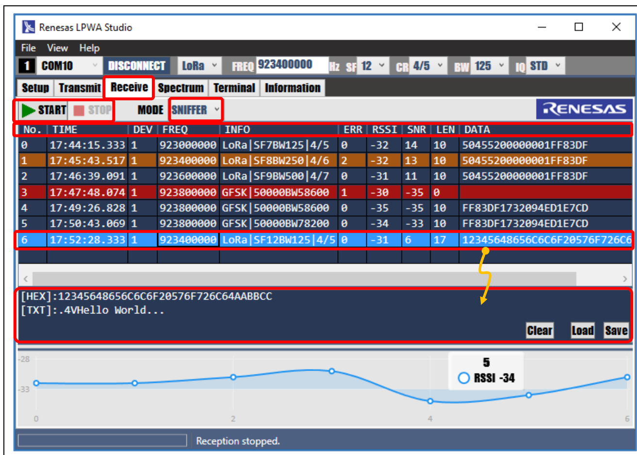
Figure 13. SNIFFER Mode
