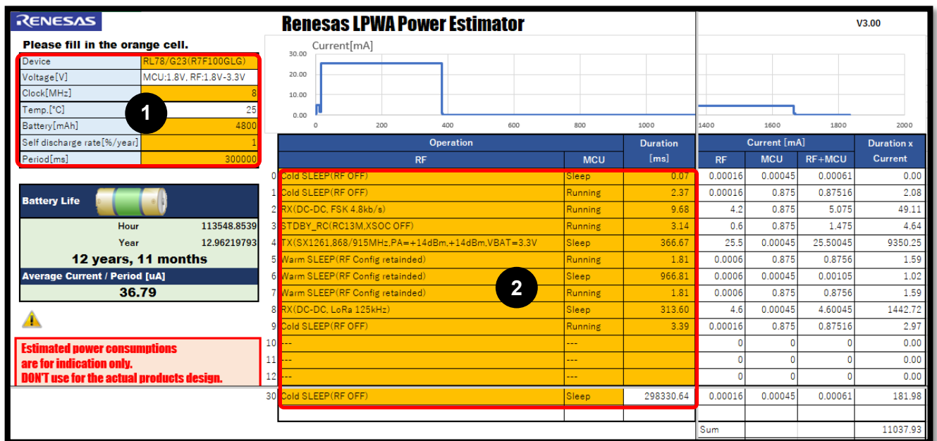
Figure 1 Renesas LPWA Power Estimator GUI
