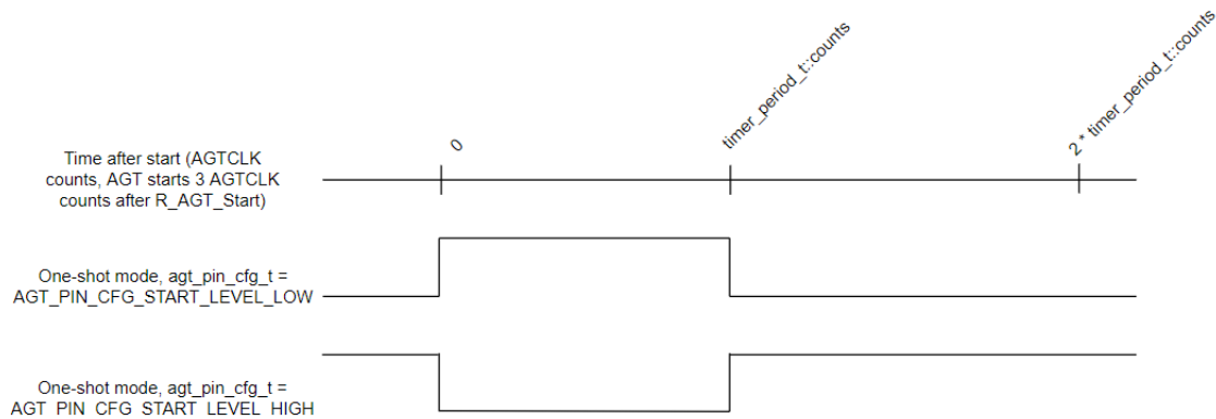
Figure 291: AGT One-Shot Output
