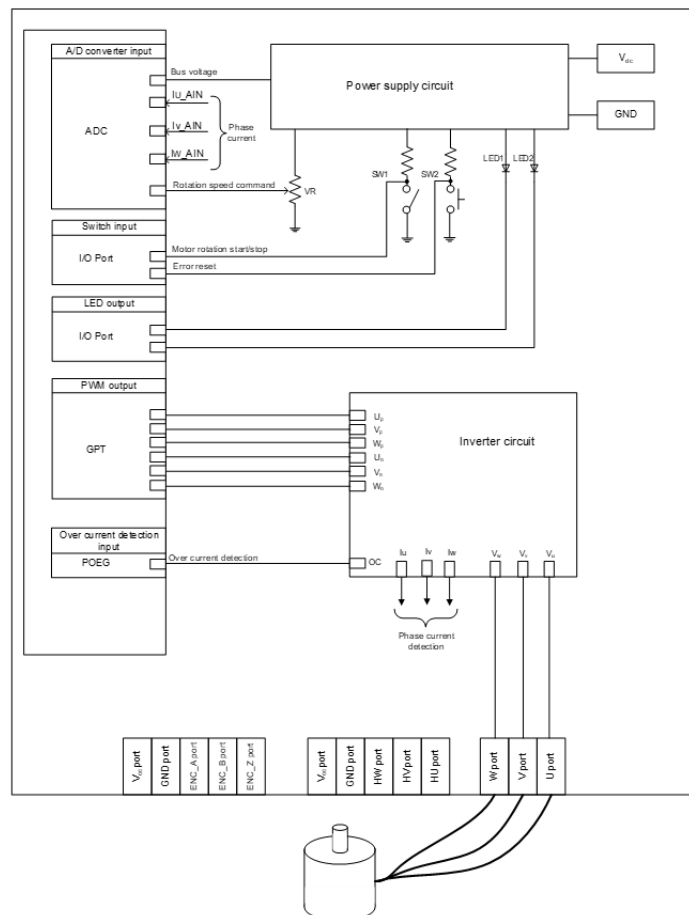
Figure 240: Example of target hardware of motor sensorless module
