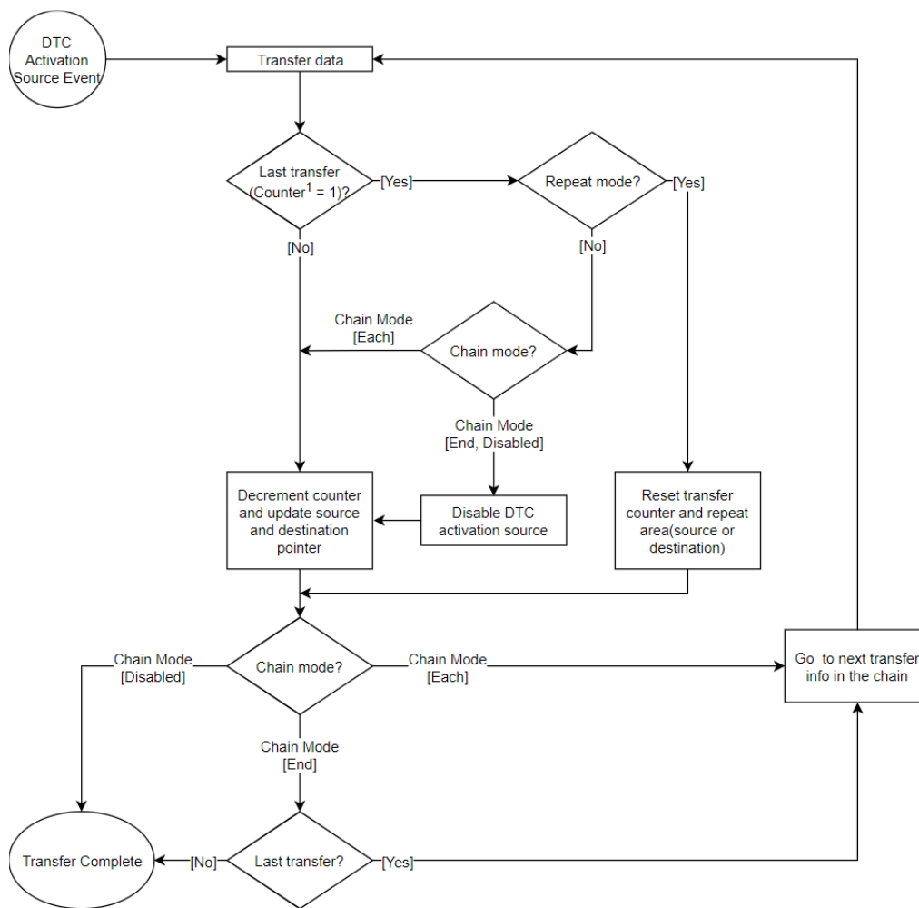
Figure 296: DTC Transfer Flowchart
