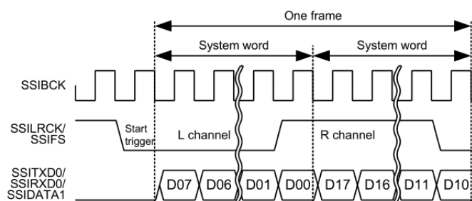
Figure 184: SSI Frame Diagram (8-bit word, 8-bit samples)
