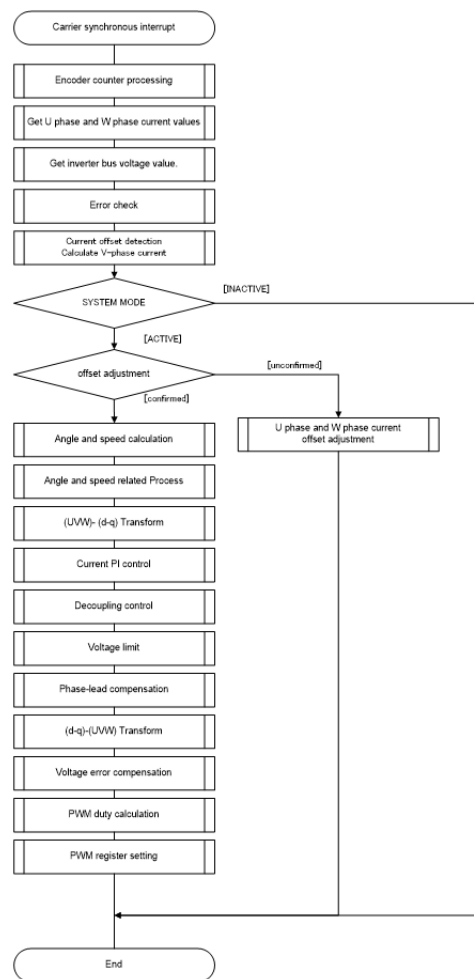
Figure 265: Current control process
