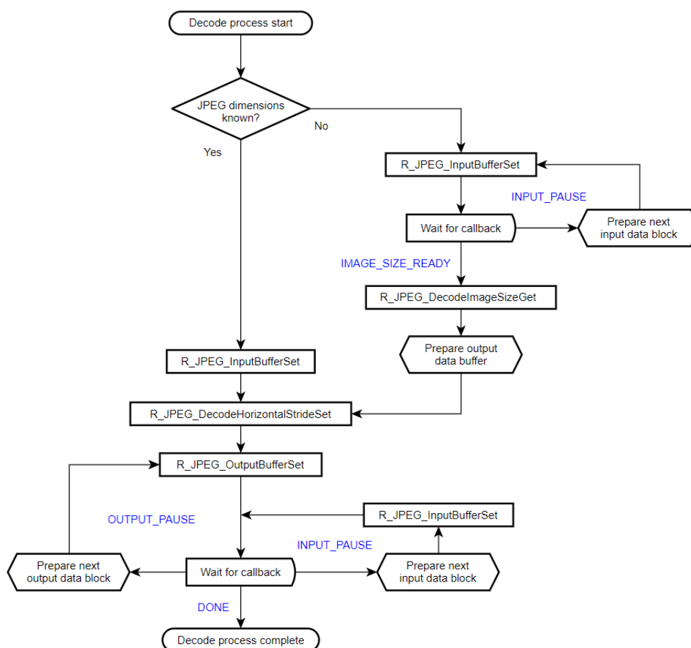
Figure 215: JPEG Decode Operational Flow
