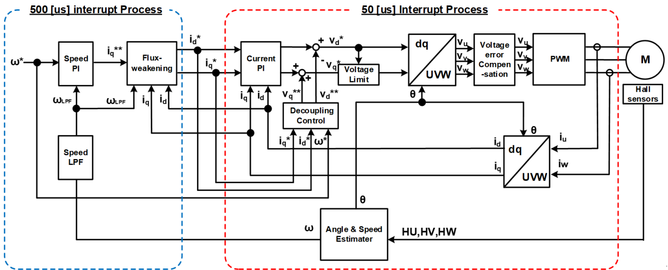
Figure 251: Block diagram of vector control with hall sensors
