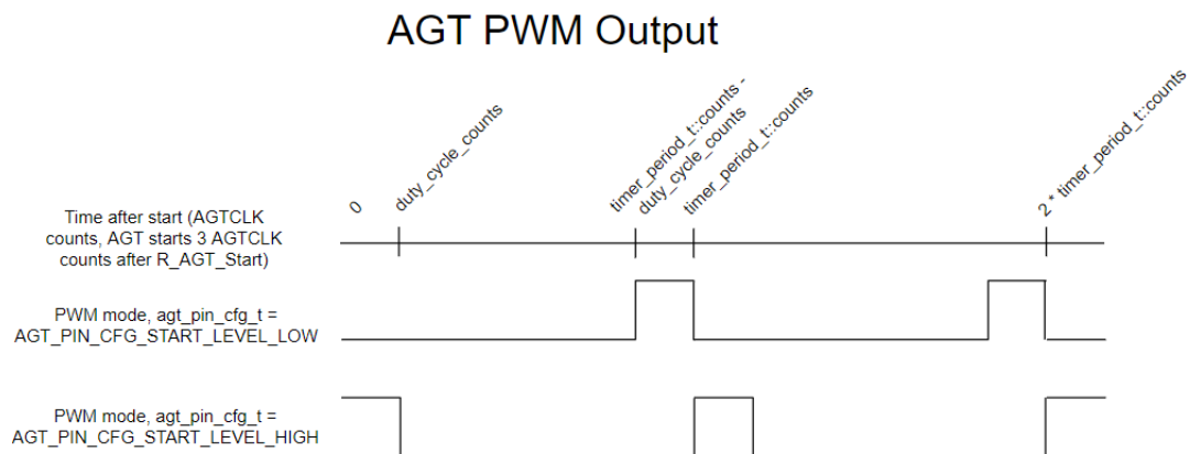
Figure 293: AGT PWM Output
