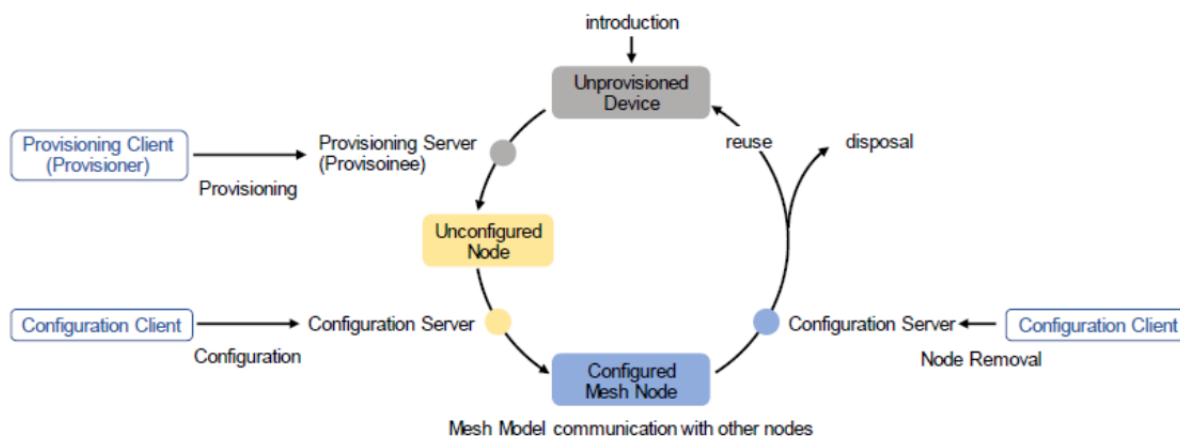
Figure 272: Device Life Cycle Image
