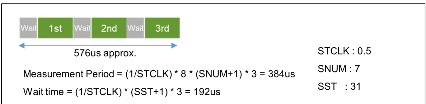
Figure 159: Self-capacitance Measurement Period (CTSU2)
