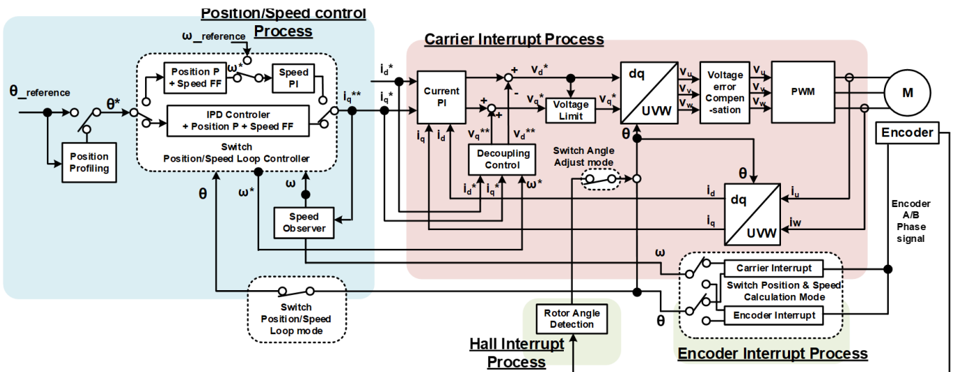
Figure 231: Block diagram of encoder vector control (PI feedback loop)
