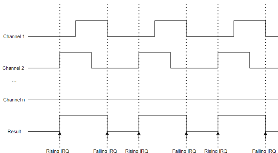
Figure 276: IPLS IRQ Generation
