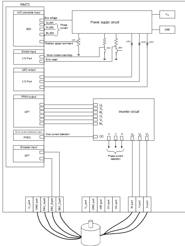
Figure 230: Example of target hardware of motor encoder module
