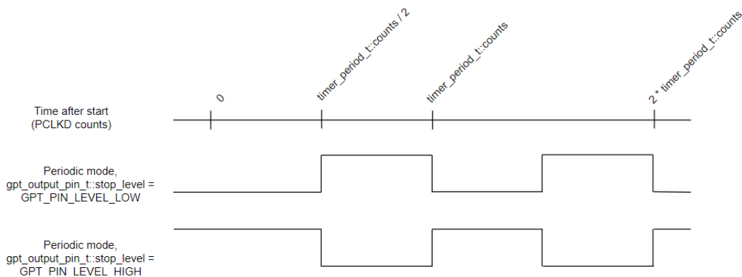
Figure 287: GPT Periodic Output
