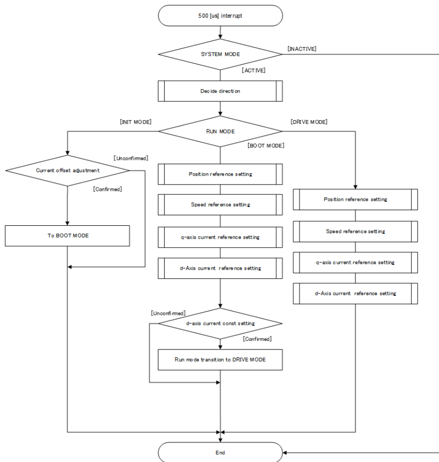
Figure 266: Speed control process
