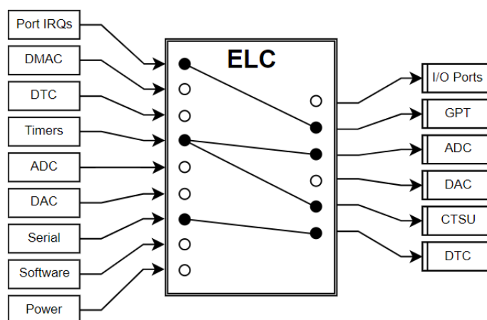
Figure 282: Event Link Controller Conceptual Diagram
