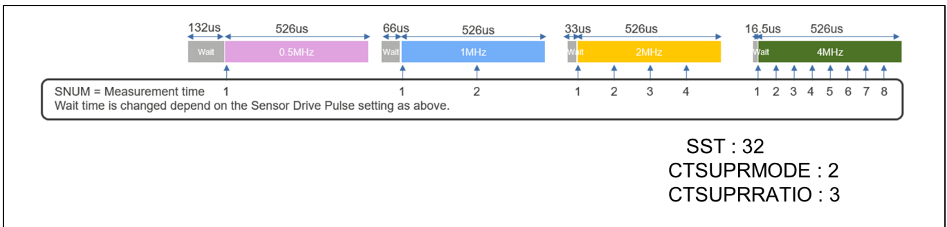
Figure 158: Self-capacitance Measurement Period (CTSU1)
