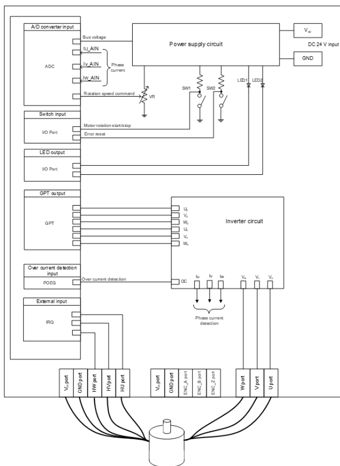
Figure 221: Example of target hardware of motor 120-degree with hall sensor
