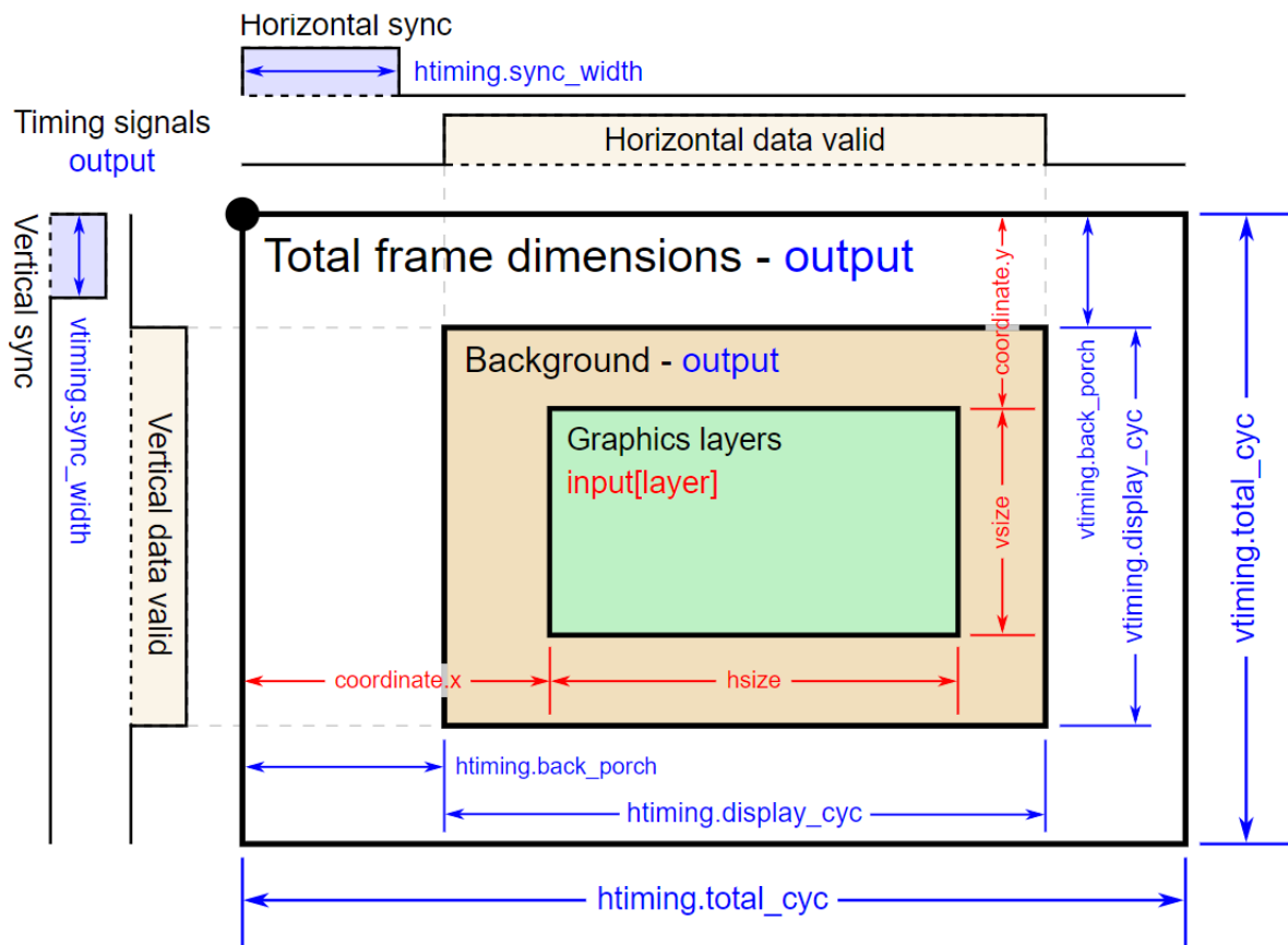
Figure 214: GLCDC layers and timing
