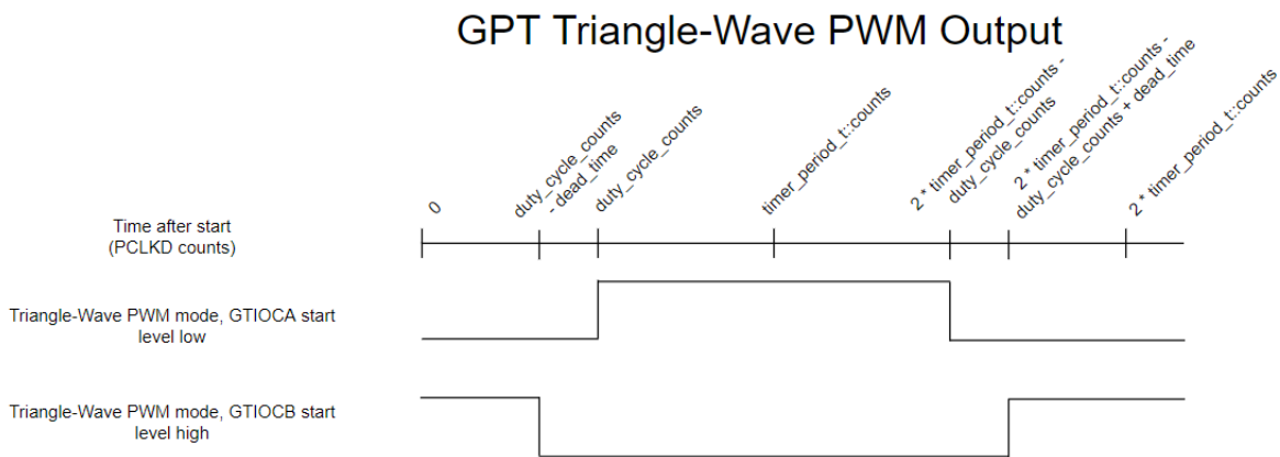
Figure 289: GPT Triangle-Wave PWM Output
