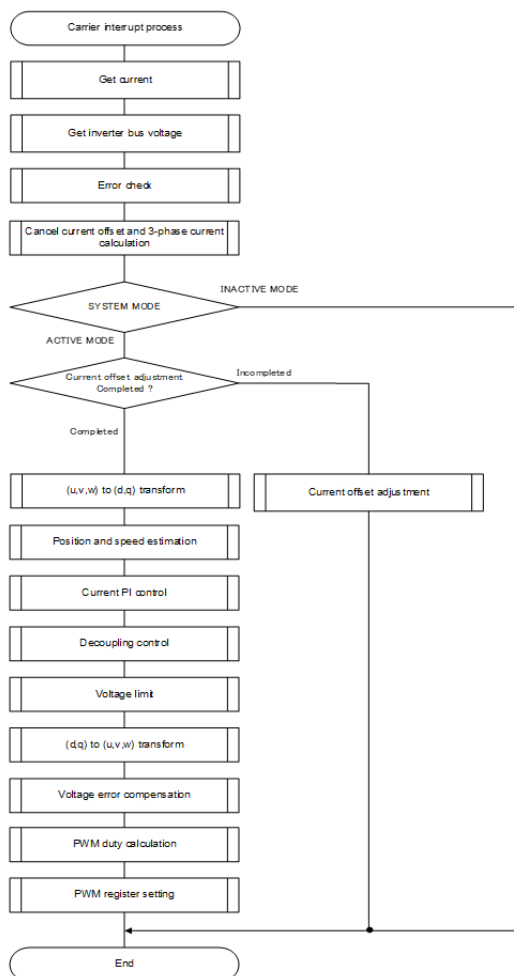
Figure 256: Current control process
