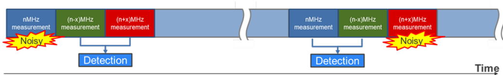
Figure 155: Multi-frequency Measurements
