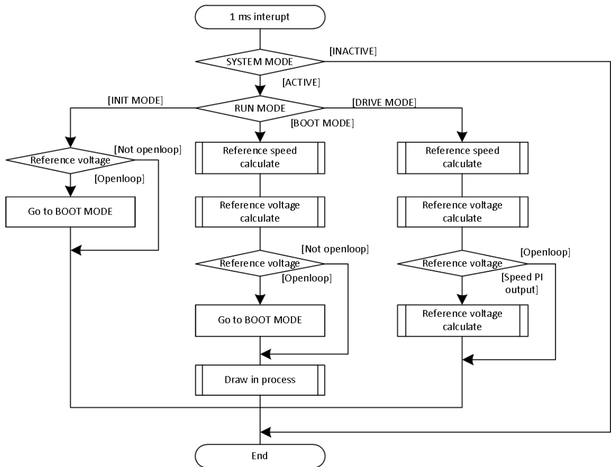
Figure 226: Speed control process of 120-degree sensorless
