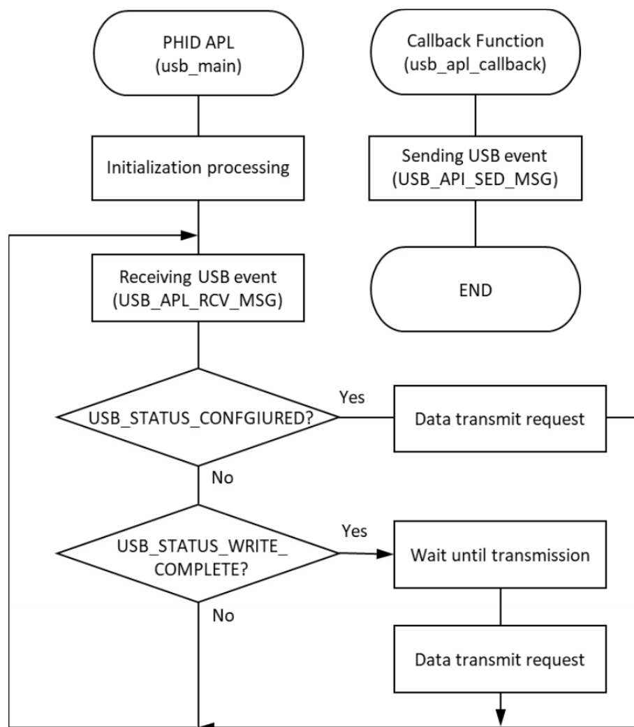
Figure 208: Main Loop processing for RTOS example
