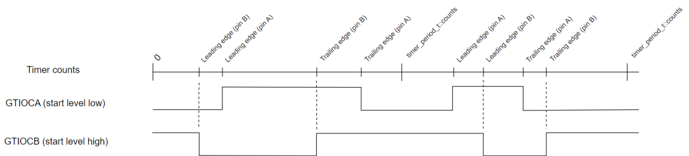
Figure 285: GPT One-Shot Pulse Output (without dead time)
