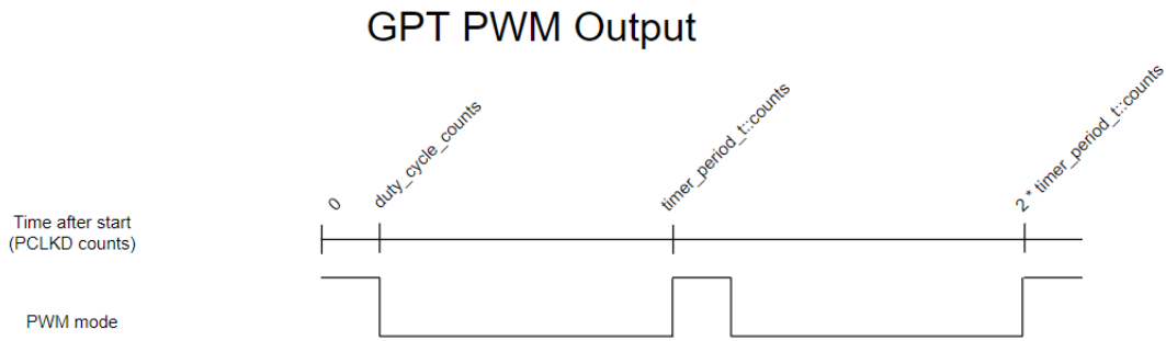
Figure 288: GPT PWM Output
