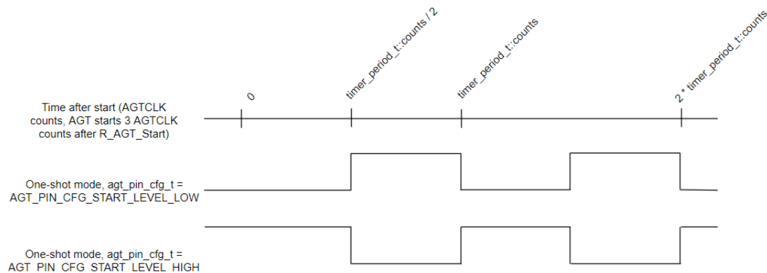
Figure 292: AGT Periodic Output
