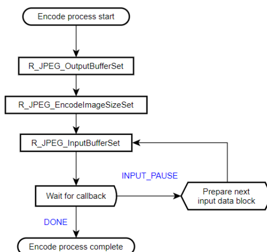
Figure 211: JPEG Encode Operational Flow
