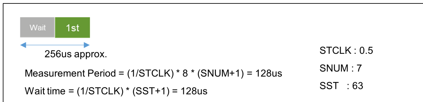
Figure 158: Current Measurement Period
