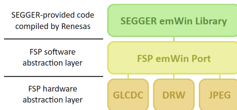
Figure 212: SEGGER emWin FSP Port Block Diagram
