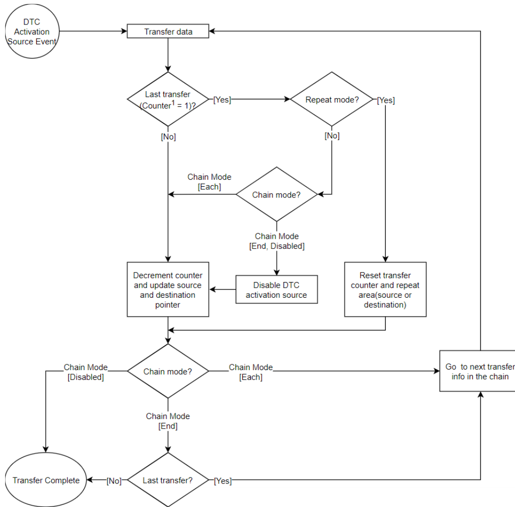
Figure 241: DTC Transfer Flowchart
