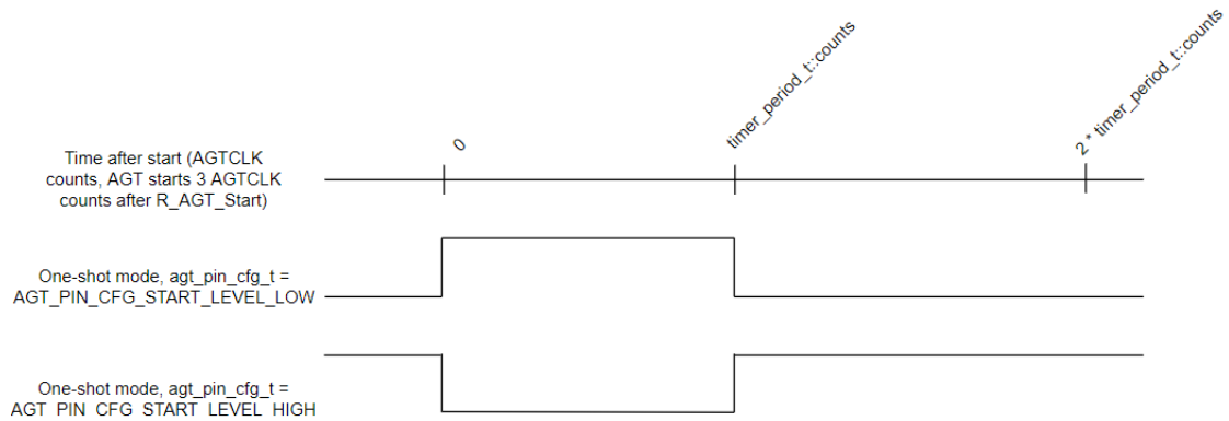
Figure 238: AGT One-Shot Output
