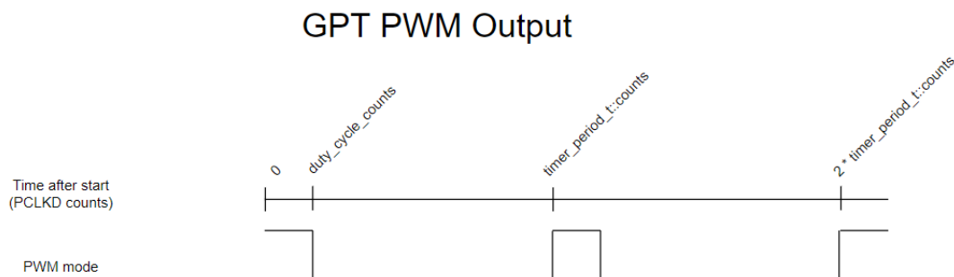
Figure 235: GPT PWM Output
