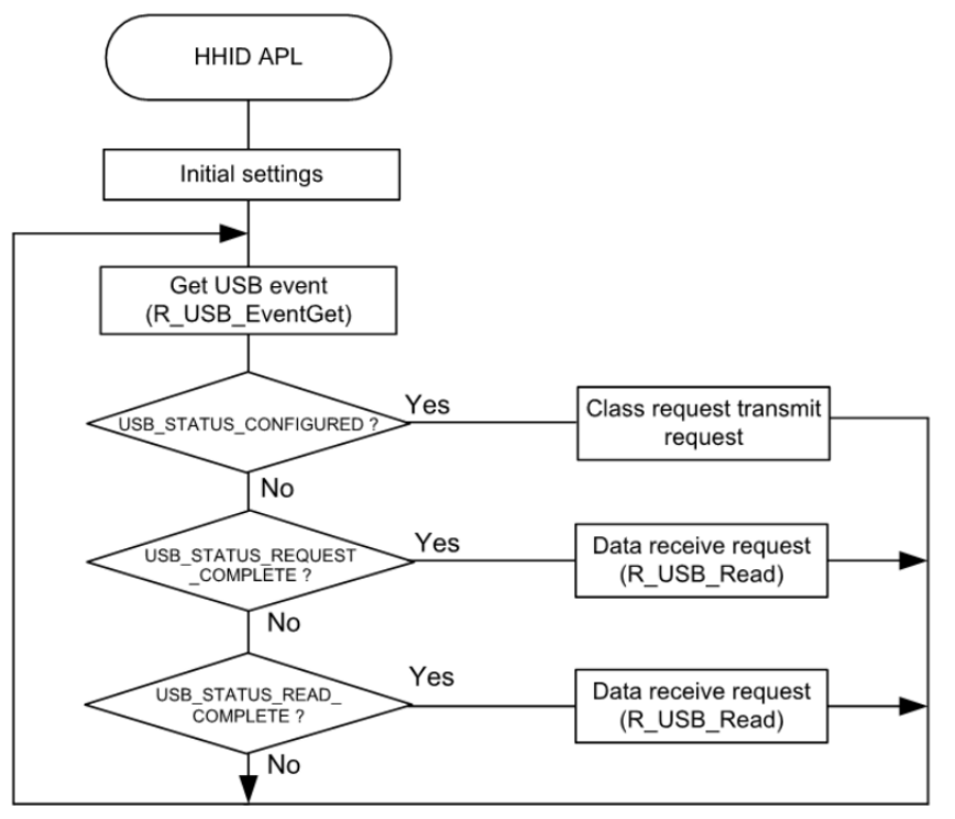
Figure 191: Main Loop (Normal mode)
