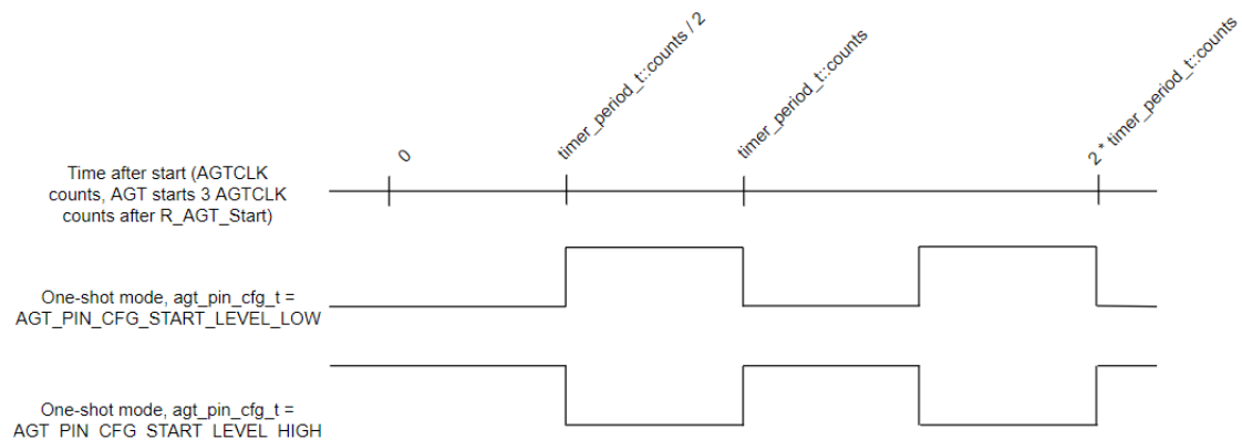
Figure 239: AGT Periodic Output
