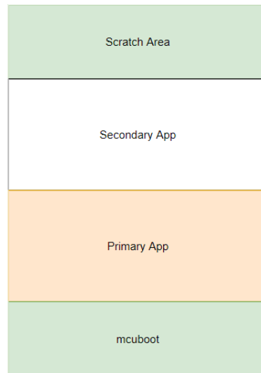
Figure 148: MCUboot Memory Map
