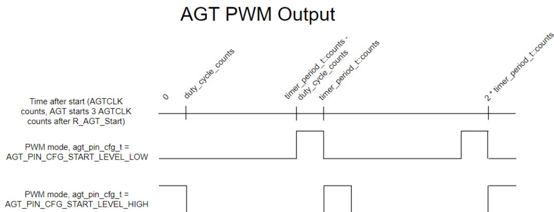
Figure 240: AGT PWM Output
