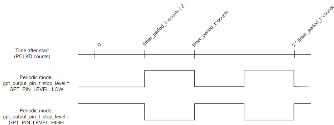
Figure 234: GPT Periodic Output
