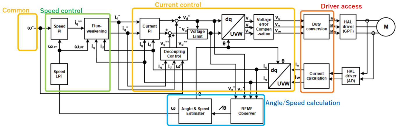
Figure 214: Image of Current Control Module(yellow block)
