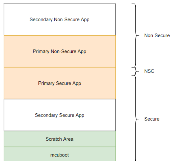
Figure 149: MCUboot Memory Map (TrustZone)
