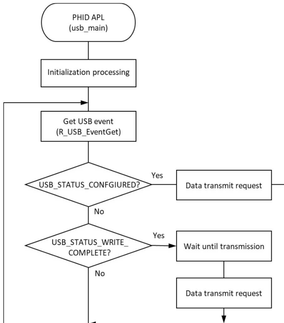
Figure 202: Main Loop processing for non-RTOS example
