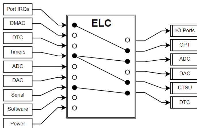
Figure 229: Event Link Controller Conceptual Diagram
