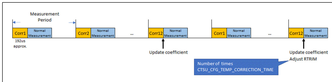
Figure 159: Temperature Correction Measurement Timing Chart
