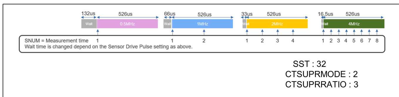
Figure 155: Self-capacitance Measurement Period (CTSU1)
