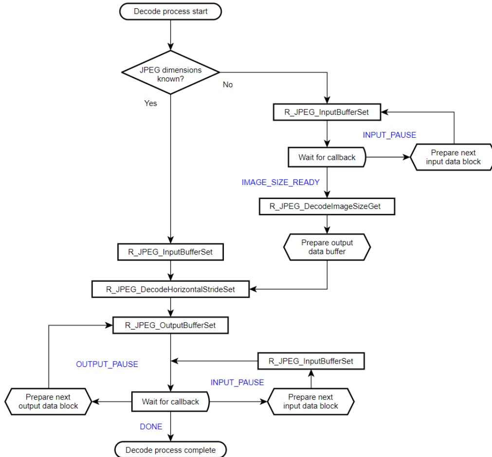
Figure 210: JPEG Decode Operational Flow
