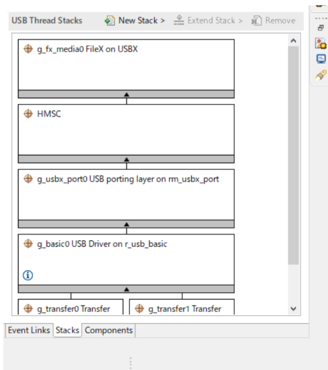
Figure 201: FileX on USBX Stack
