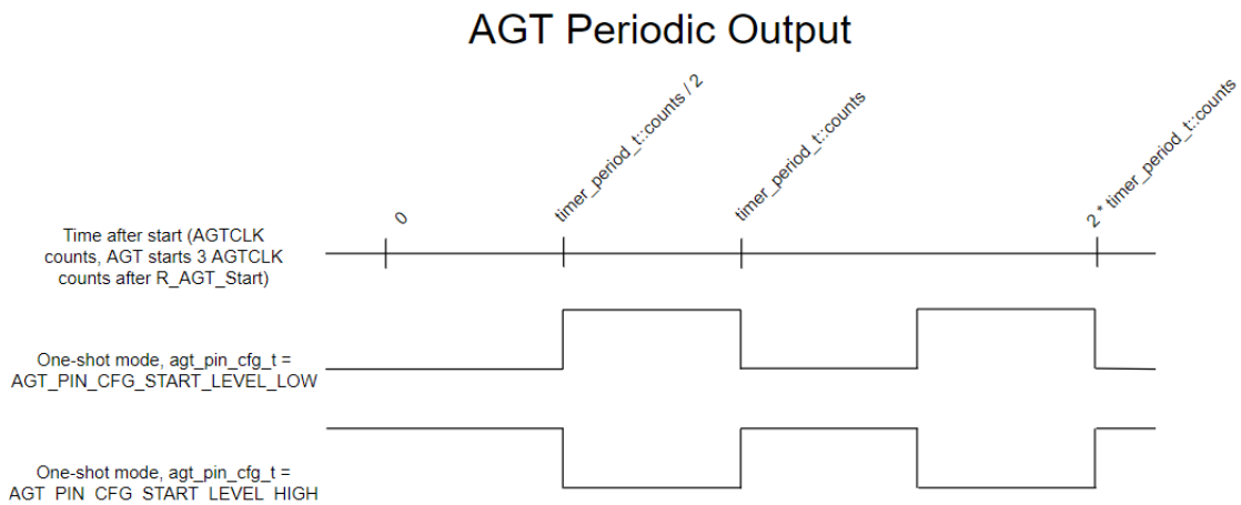
Figure 143: AGT Periodic Output
