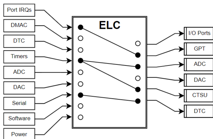
Figure 153: Event Link Controller Conceptual Diagram
