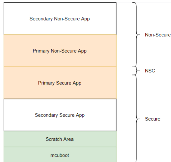
Figure 194: MCUboot Memory Map (TrustZone)
