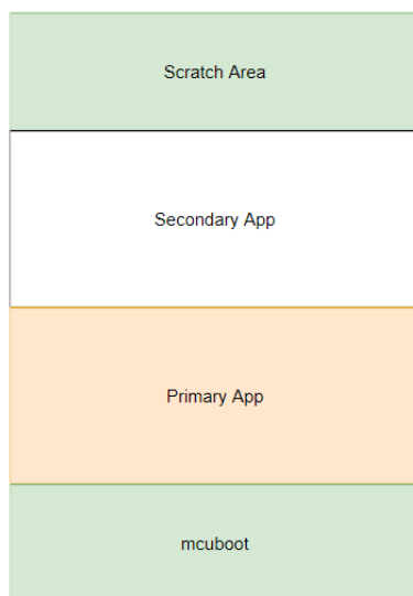
Figure 193: MCUboot Memory Map
