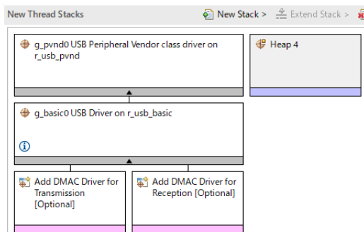
Figure 189: USB Peripheral Vendor Class Stack
