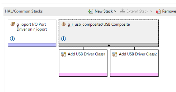
Figure 169: USB Composite Stack
