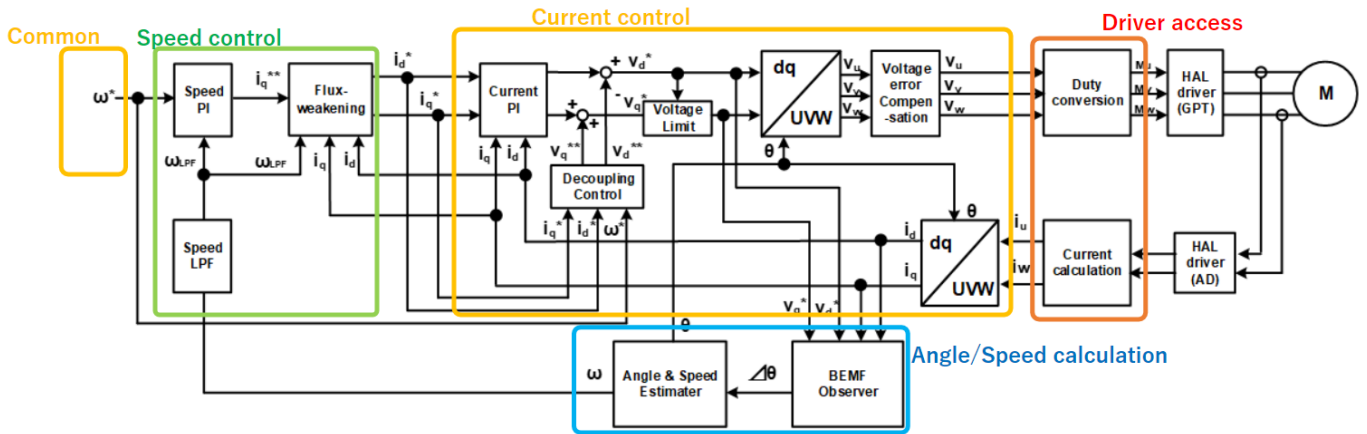
Figure 198: Image of Sensorless Vector Control Structure
