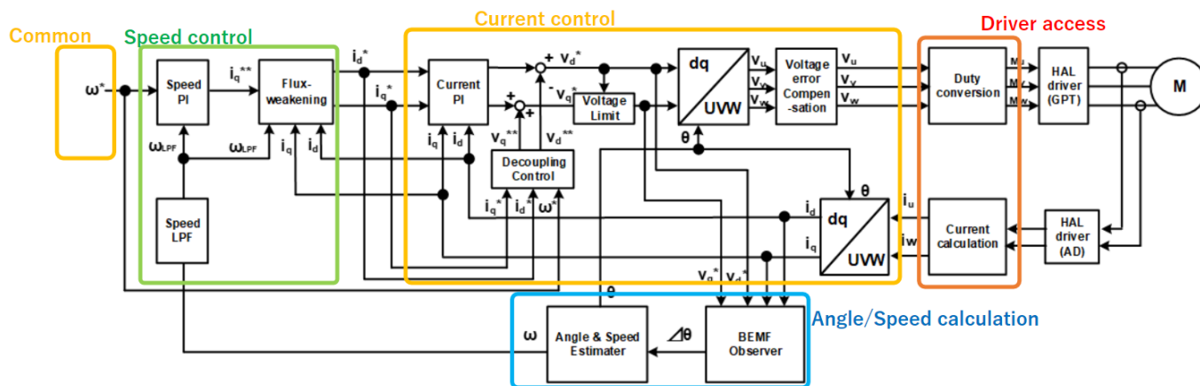
Figure 195: Image of Current Control Module(yellow block)
