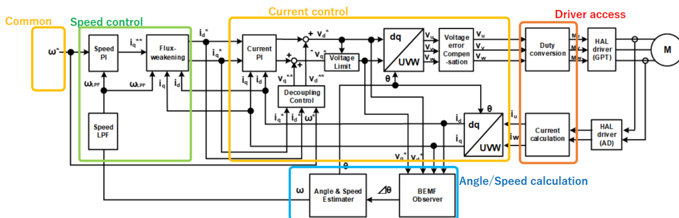
Figure 196: Image of Driver Module (red block)
