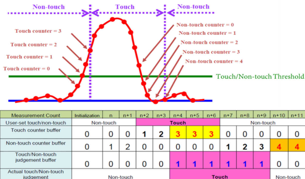
Figure 201: Touch/Non-touch judgement Image
