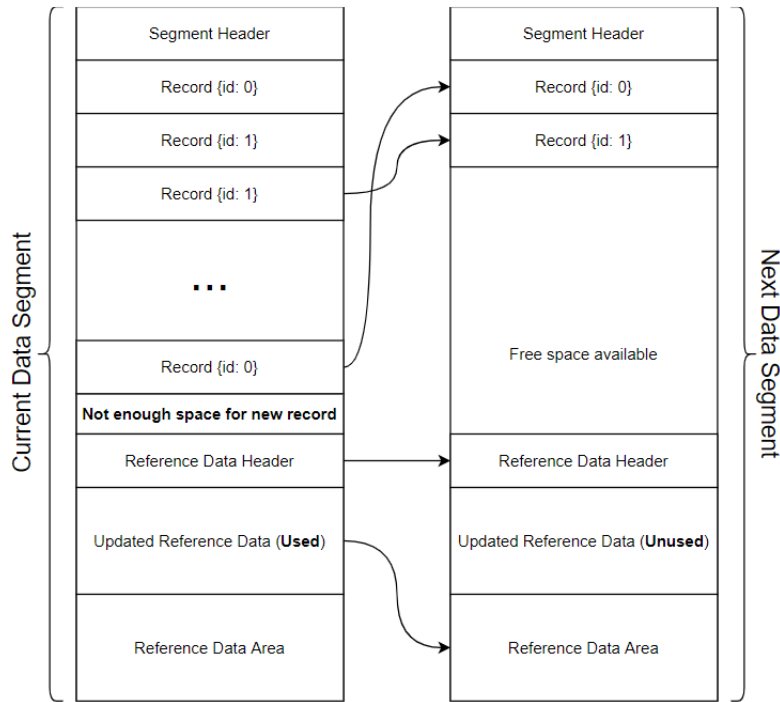
Figure 208: Refresh Operation
