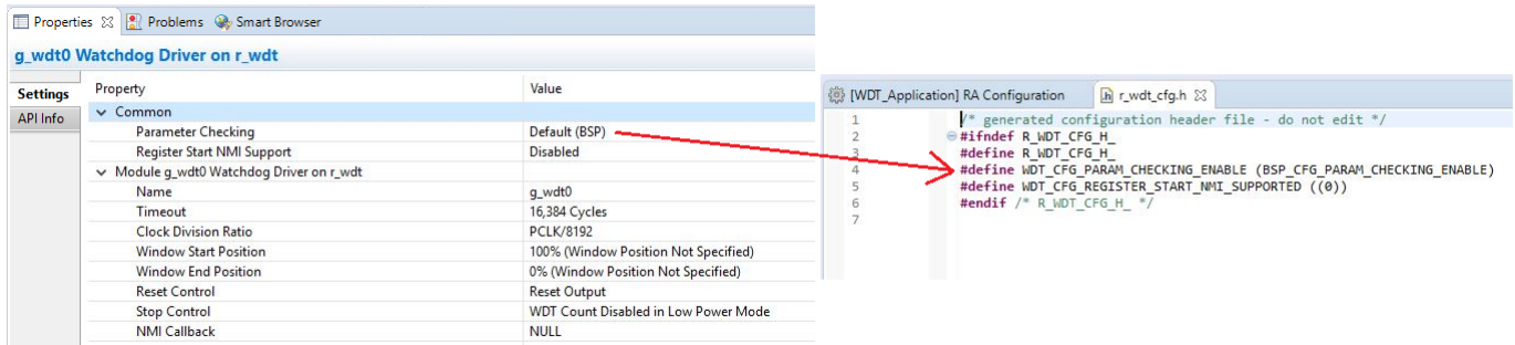
Figure 94: r_wdt_cfg.h contents
