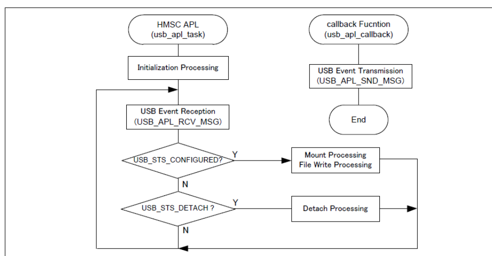
Figure 146: usb_apl_task
