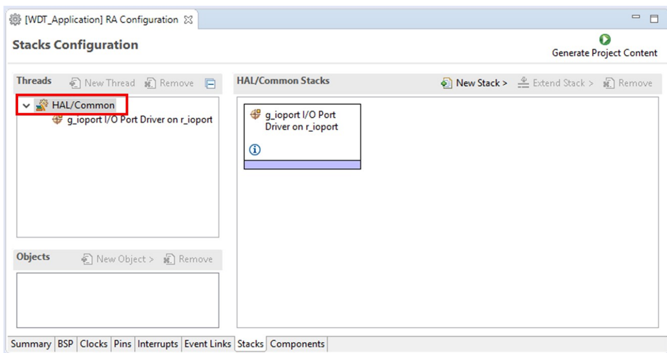
Figure 88: Stacks tab
