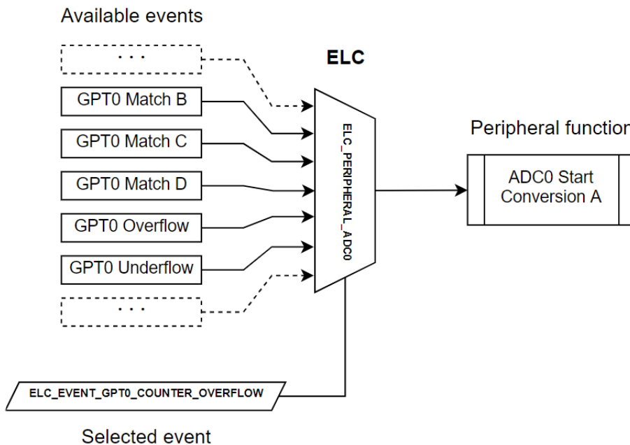
Figure 128: ELC Example
