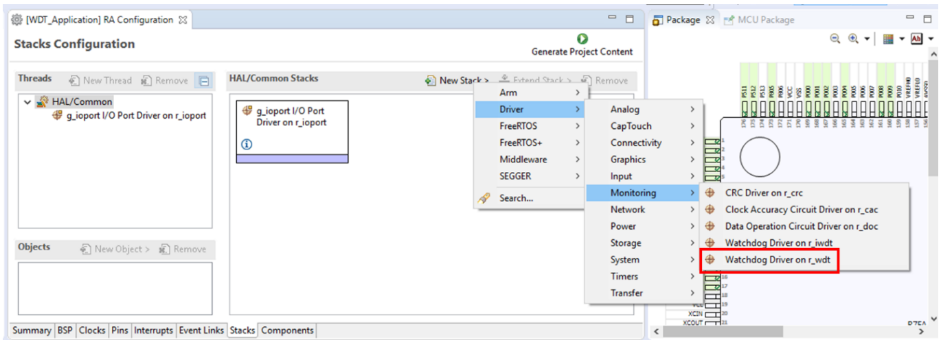
Figure 89: Module Selection
