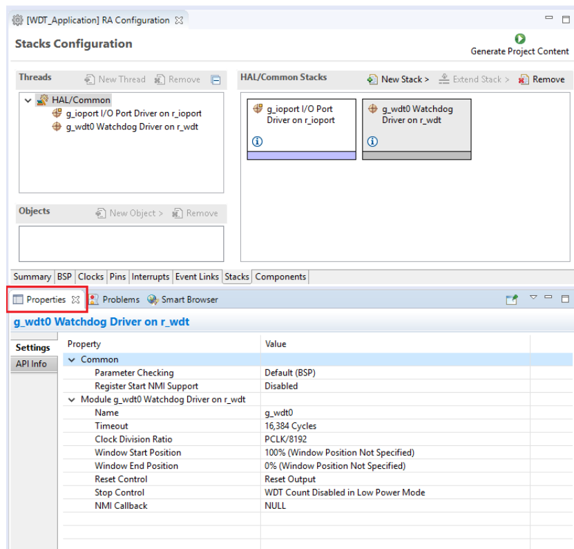
Figure 90: Module Properties
