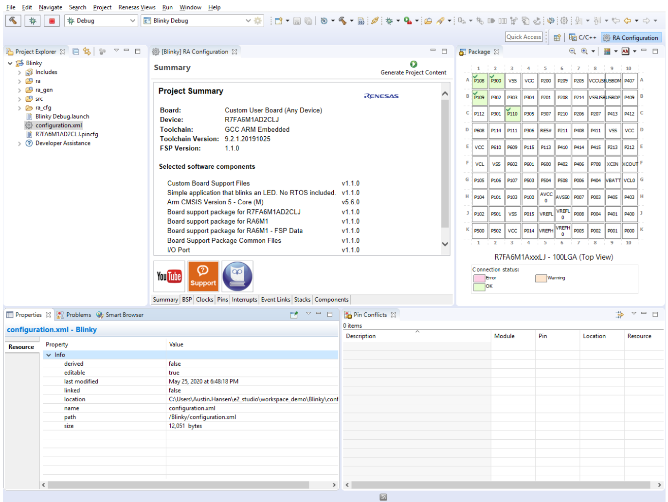
Figure 2: Default Perspective
