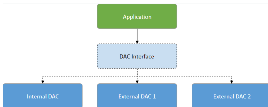
Figure 113: DAC Interface
