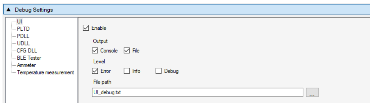
Figure 71: Debug Settings
