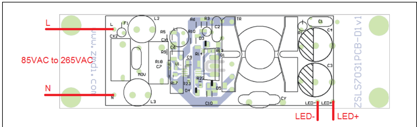
Figure 4.1 ZSLS7031PCB-D1 Connection Diagram
