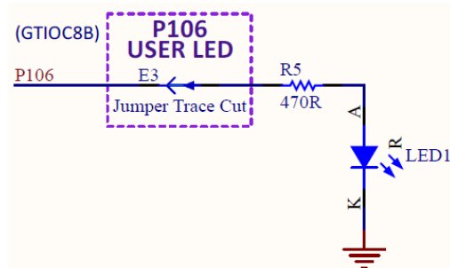
Figure 14. LED1 Control Circuit
