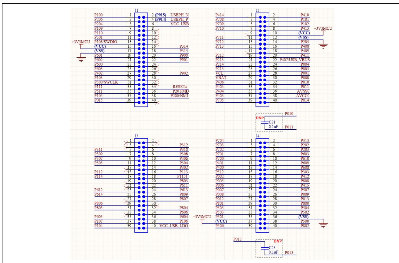
Figure 23. TB-S3A1 Pin Headers Circuit
