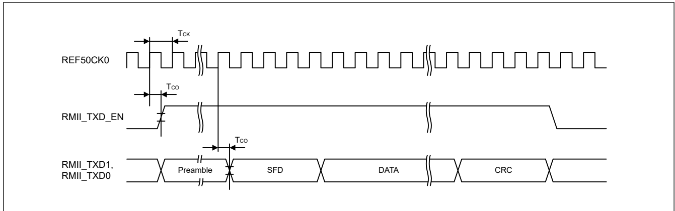
Figure 53.65 RMIITransmission timing
