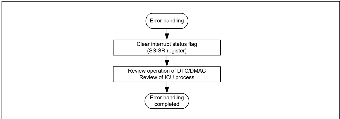
Figure 38.57 Error-handling procedure
