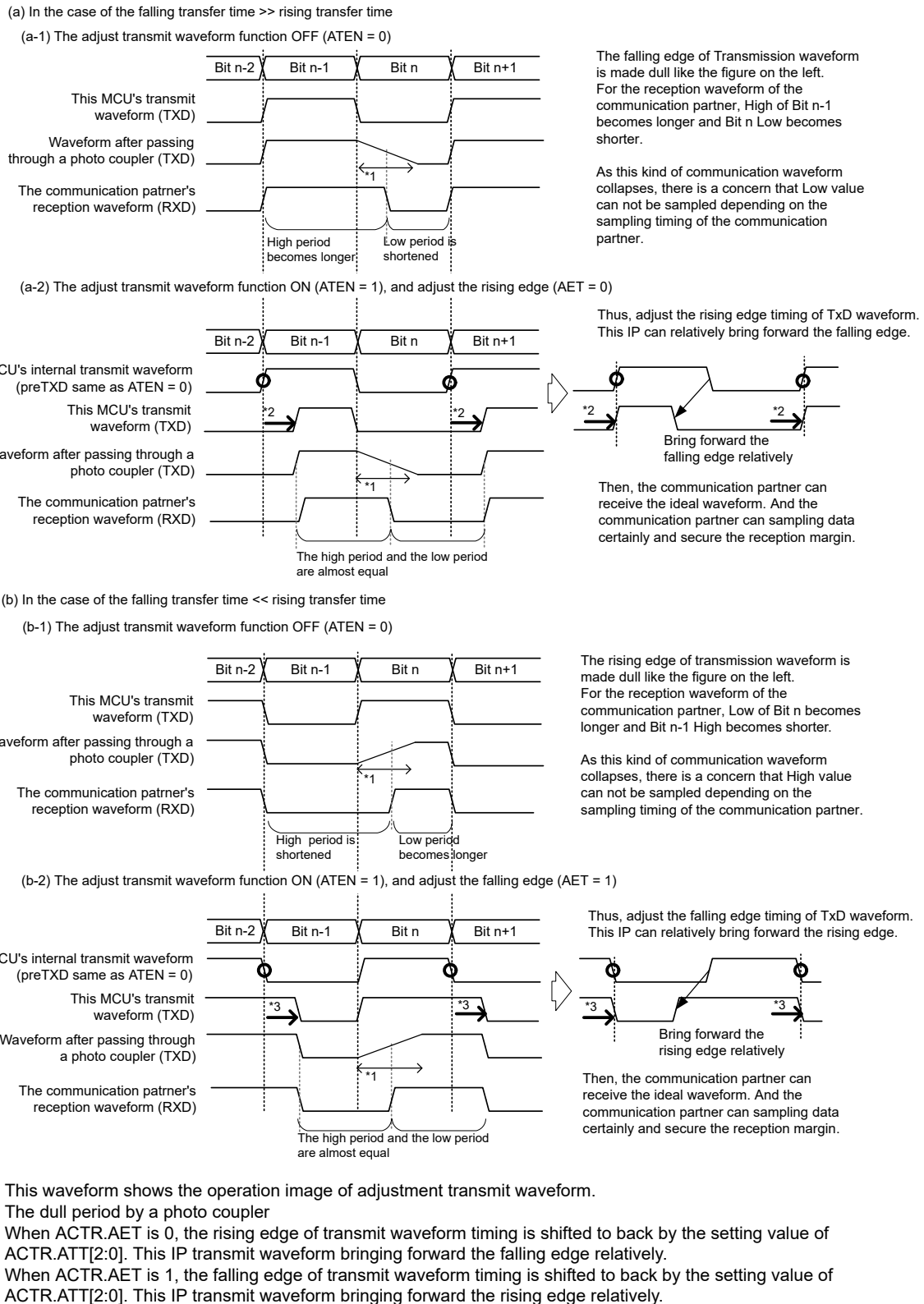
Figure 30.36 The overview of transmission operation in the communication through a photo coupler
