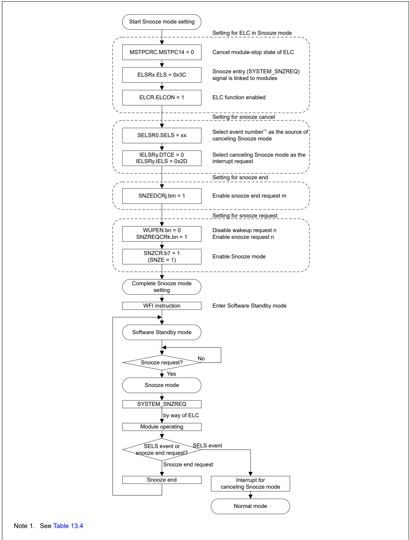
Figure 10.8 Setting example of using ELC in Snooze mode
