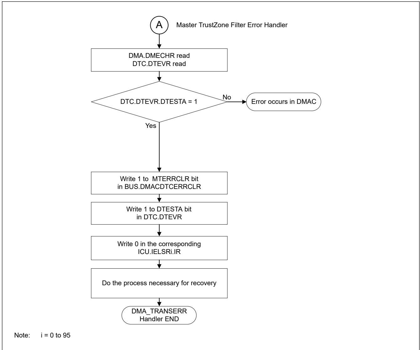
Figure 17.18 Processing in DMA_TRANSERR handler by Master TrustZone Filter Error
