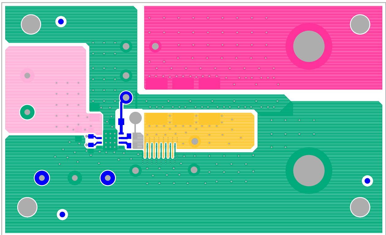
Figure 7. Top Layer
