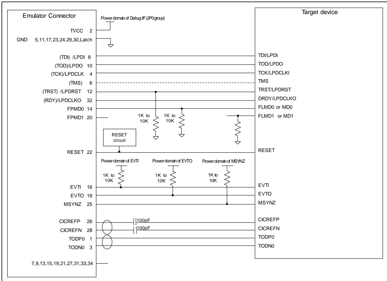
Figure 4-3 Example of Recommended Connections for Debugging (4-Pin LPD) and Tracing (One Lane)
