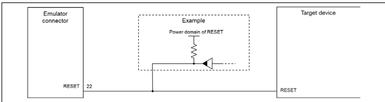
Figure 4-4 Example of Connecting a Reset Circuit
