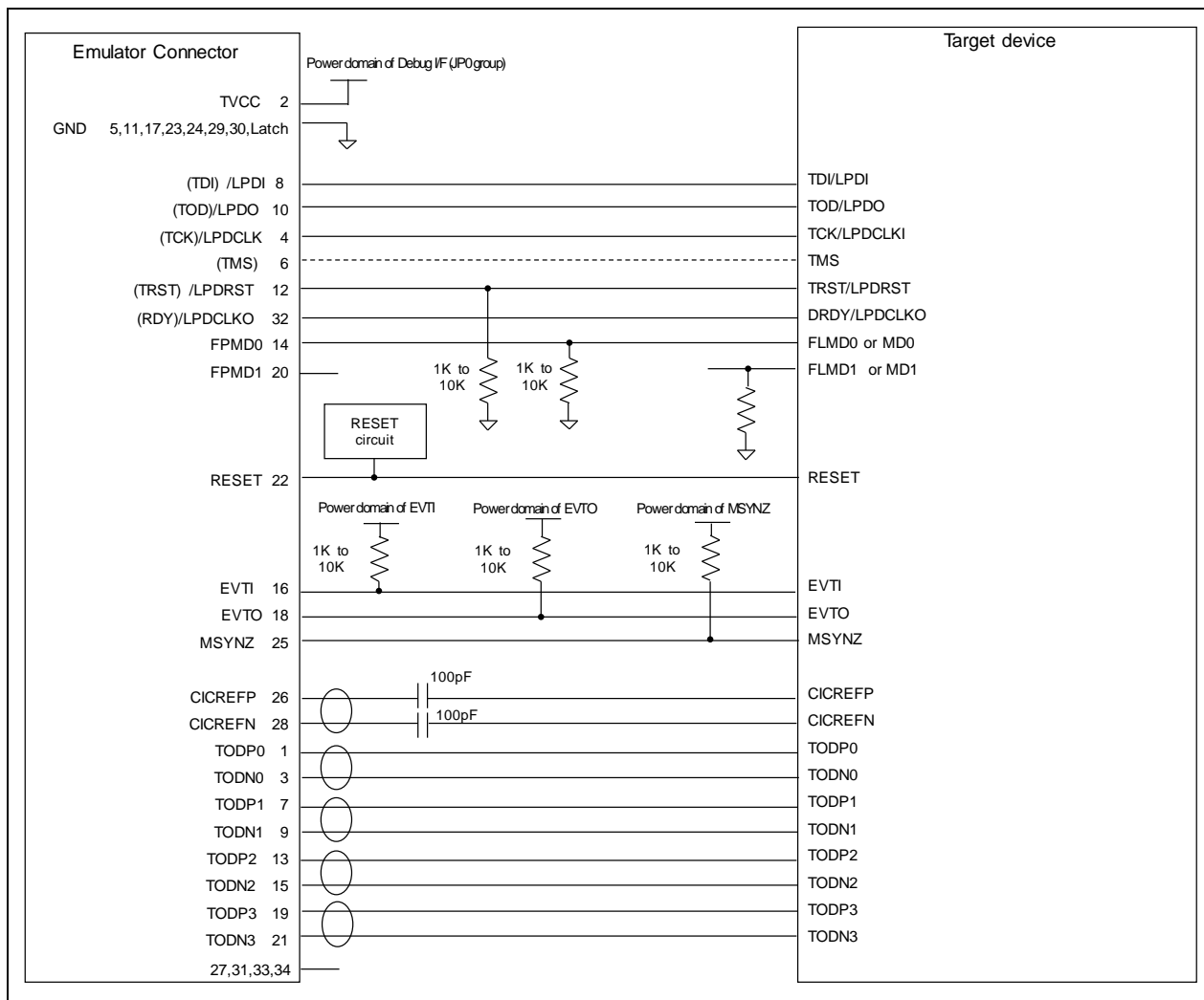
Figure 4-2 Example of Recommended Connections for Debugging (4-Pin LPD) and Tracing (Four Lanes)
