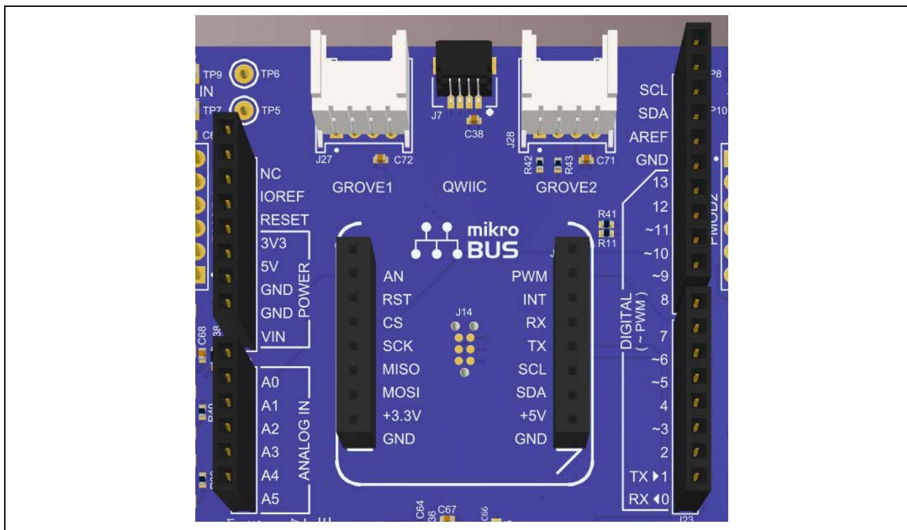
Figure 14. Arduino Uno Connectors
