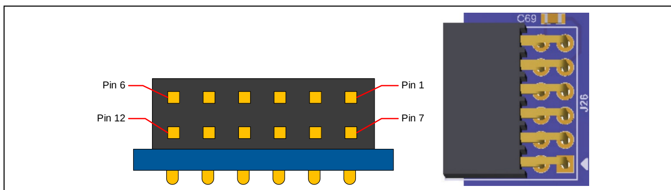
Figure 11. Pmod 1 Connector
