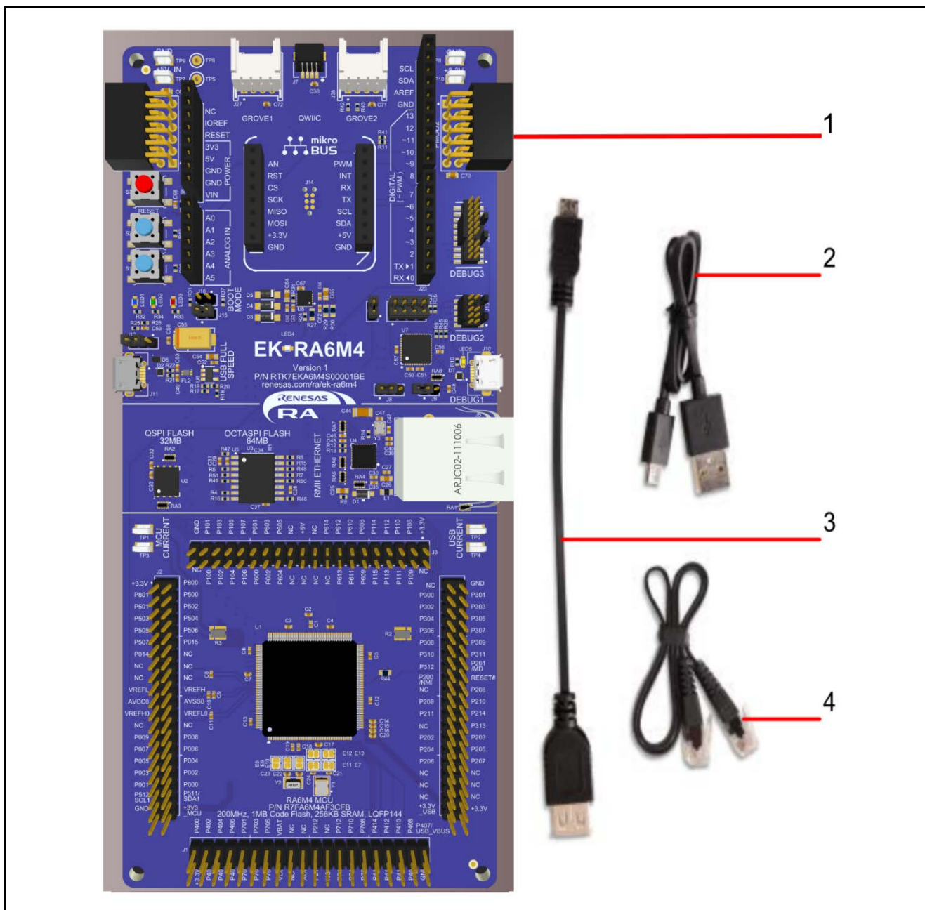
Figure 3. EK-RA6M4 Kit Contents
