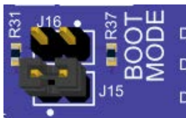
Figure 20. Boot Mode
