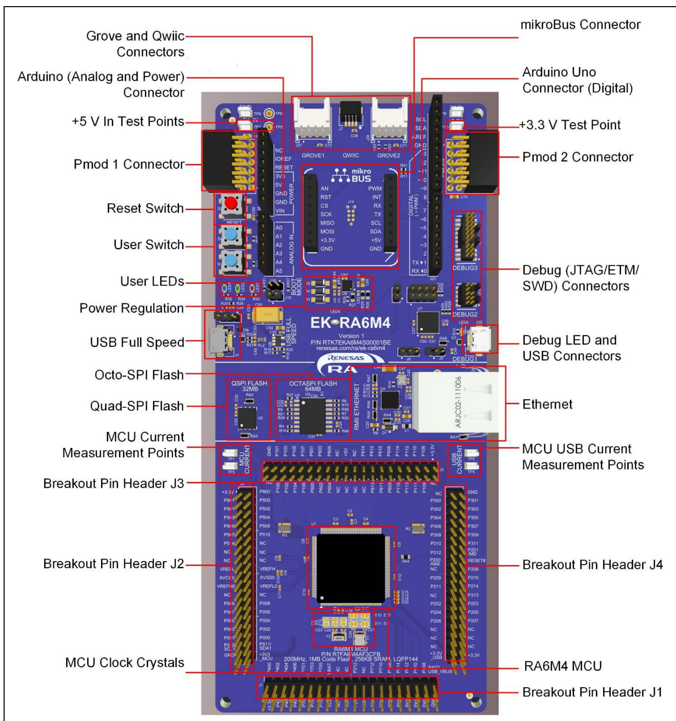
Figure 1. EK-RA6M4 Board Top Side
