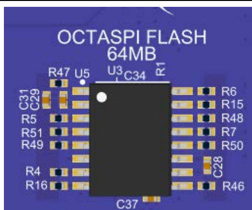
Figure 24. Octo-SPI Flash
