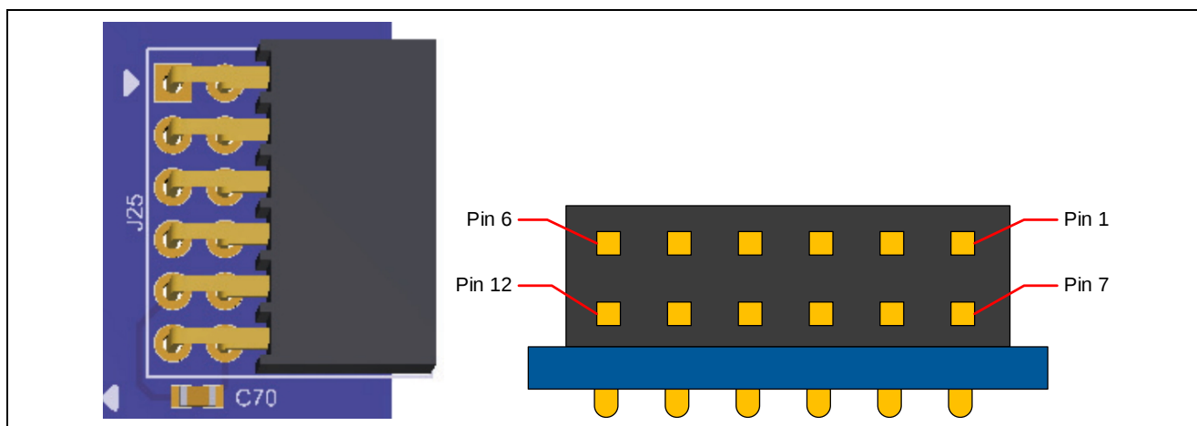
Figure 13. Pmod 2 Connector
