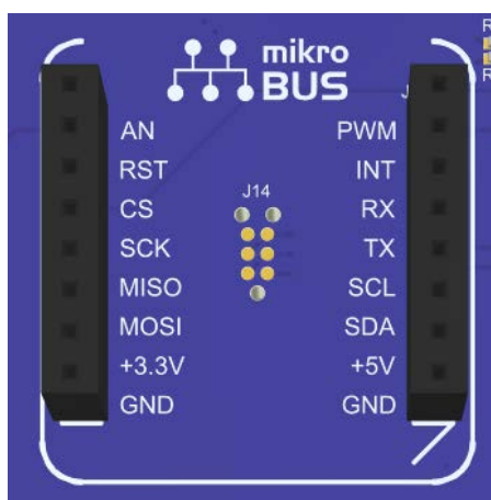
Figure 15. mikroBUS Connection
