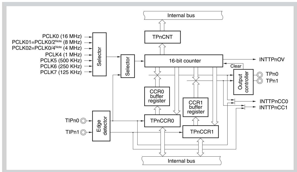
Figure 11-1 Block diagram of TMPn
