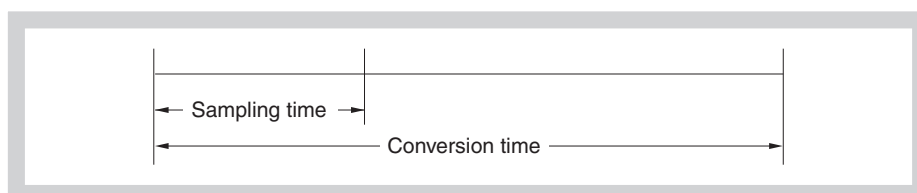
Figure 21-16 Sampling time
