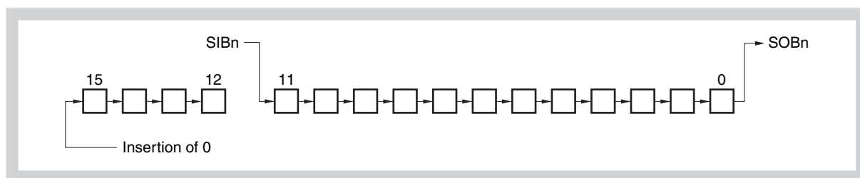
Figure 18-3 (ii) Transfer bit length = 12 bits, LSB first
