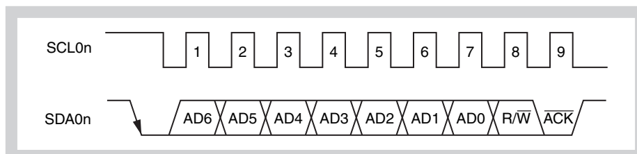
Figure 19-10 \overline{\text{ACK}} signal
