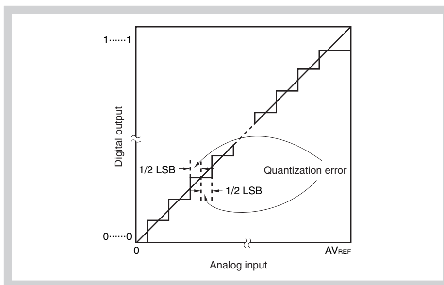
Figure 21-11 Quantization error
