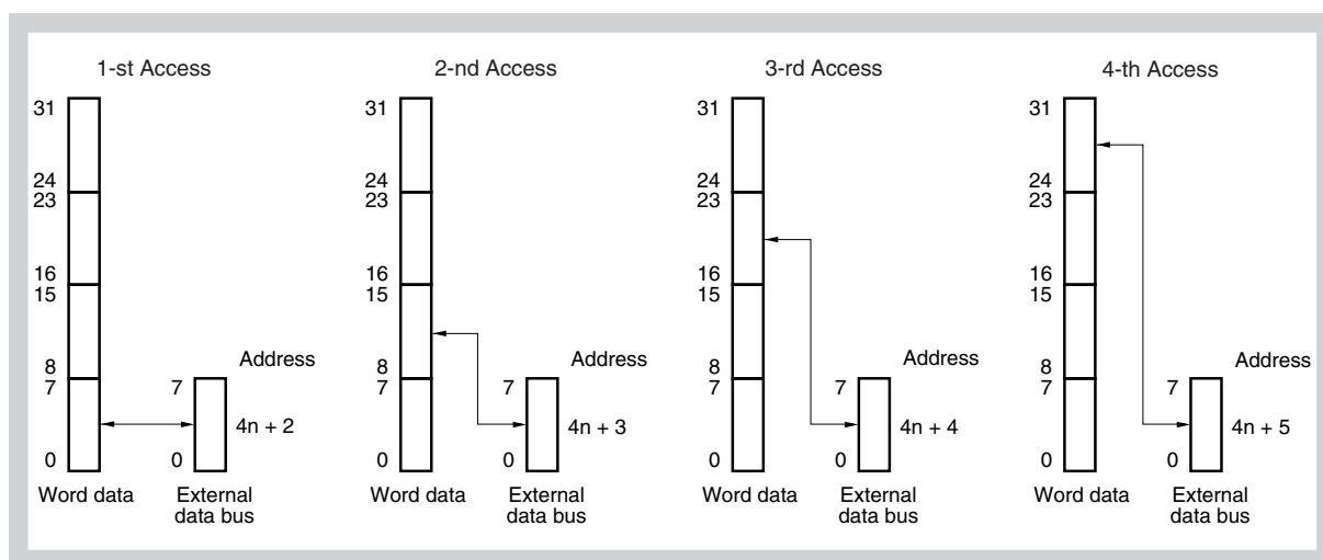
Figure 7-27 Access to address 4n + 2
