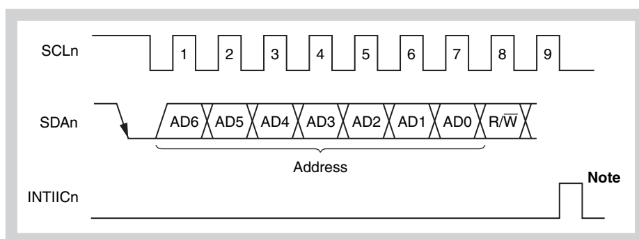
Figure 19-8 Address
