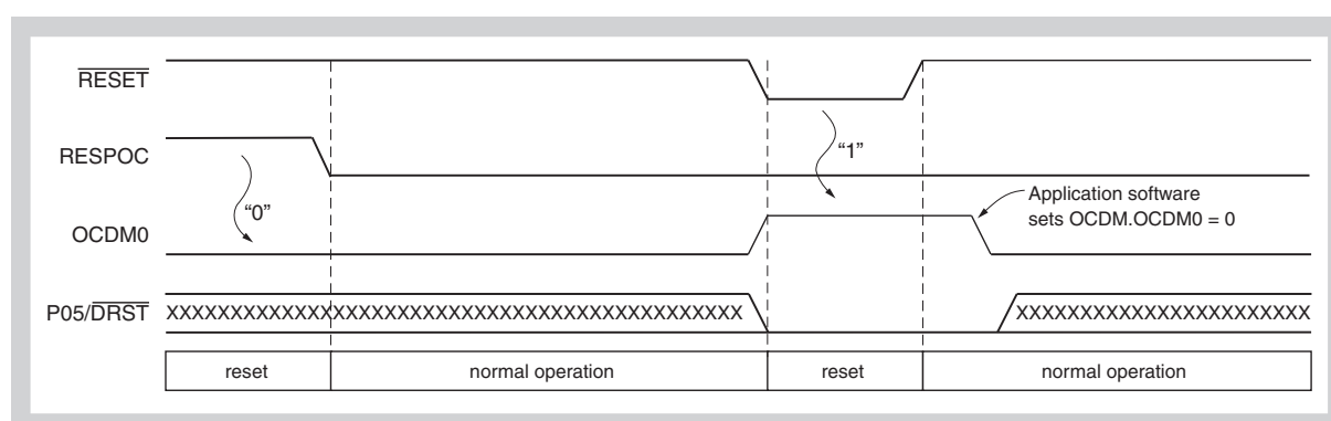
Figure 29-1 Start without N-Wire activation
