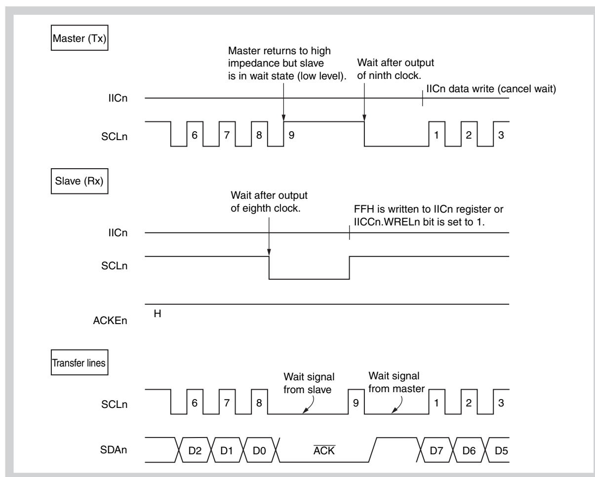
Figure 19-12 Wait signal (1/2)
