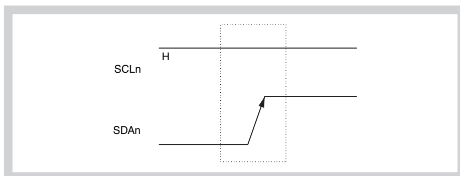
Figure 19-11 Stop condition
