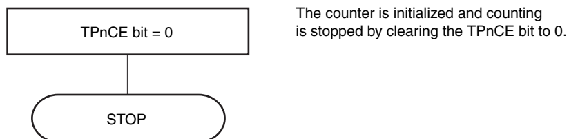
Figure 11-39 Software processing flow in pulse width measurement mode
