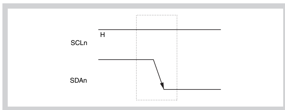
Figure 19-7 Start condition
