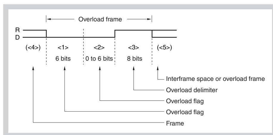
Figure 20-16 Overload frame
