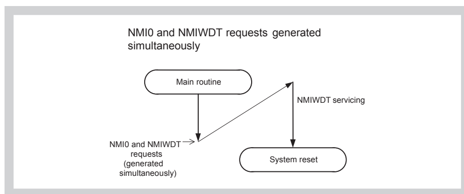
Figure 5-1 Example of non-maskable interrupt request acknowledgement operation: multiple NMI requests generated at the same time
