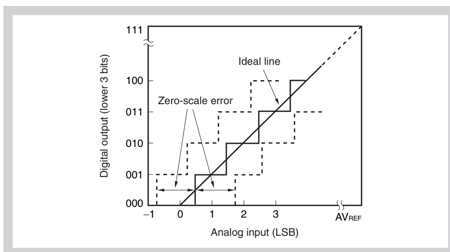
Figure 21-12 Zero-scale error
