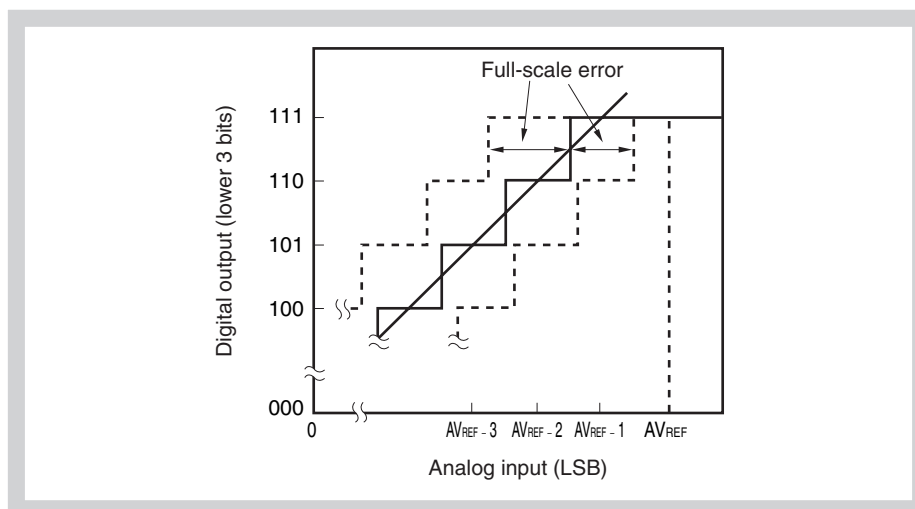
Figure 21-13 Full-scale error
