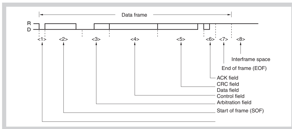
Figure 20-3 Data frame
