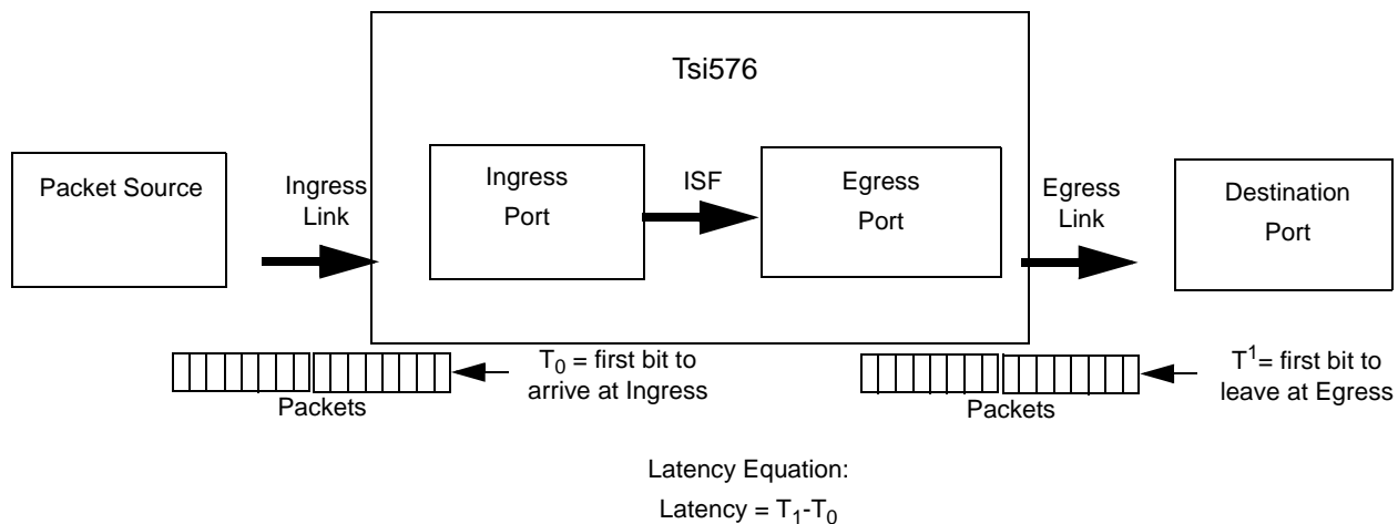
Figure 43: Latency Illustration
