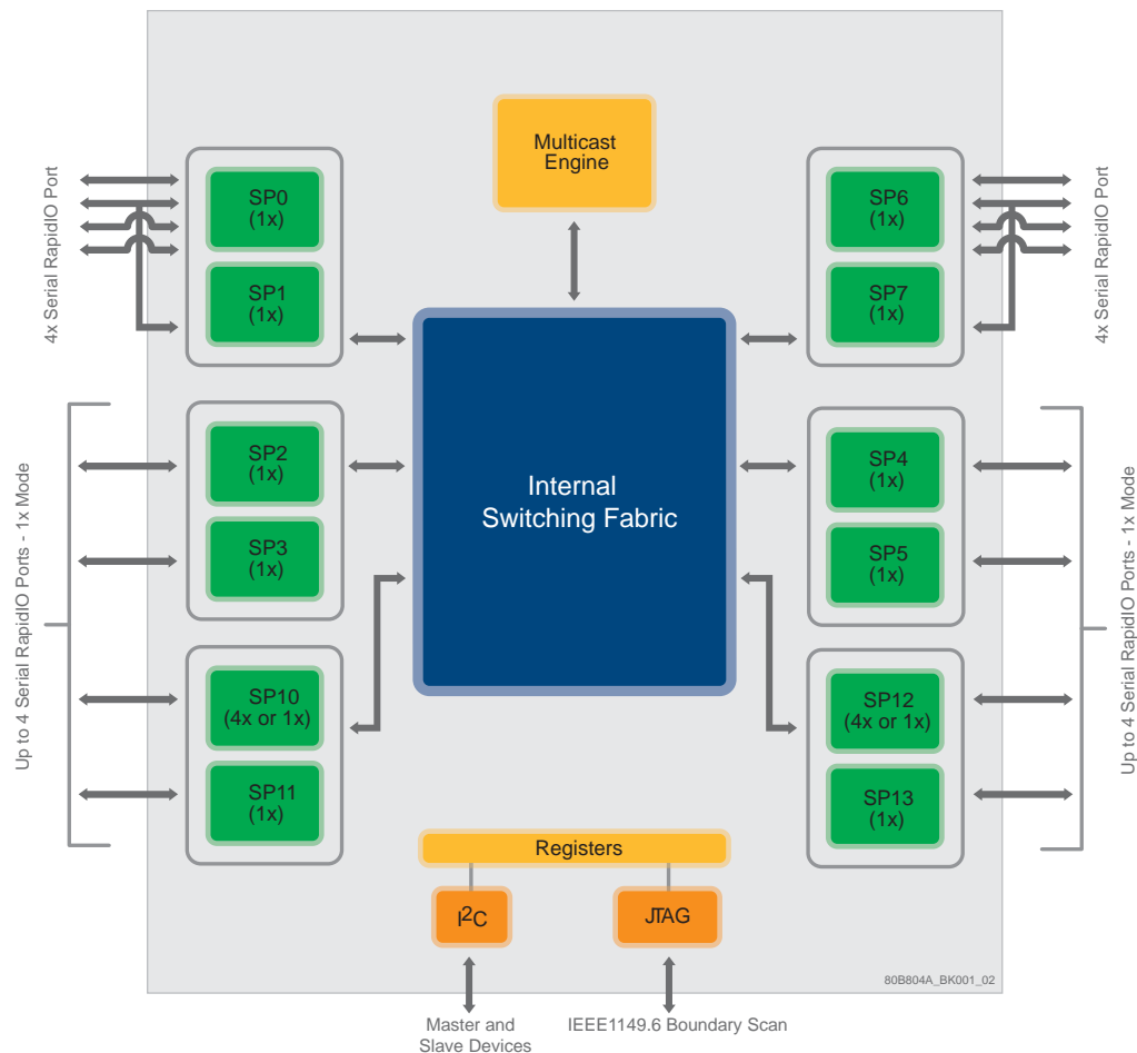
Figure 1: Block Diagram
