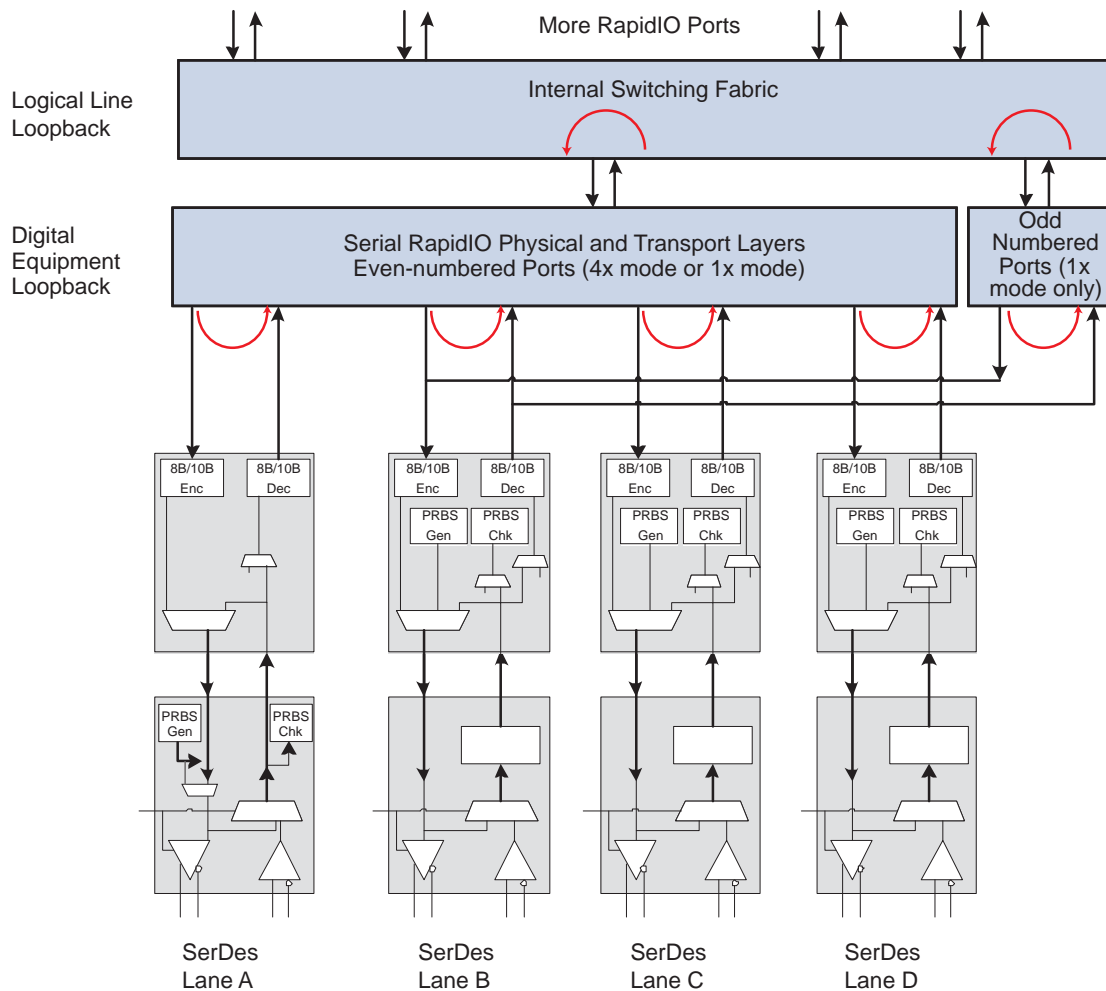
Figure 15: Tsi576 Loopbacks
