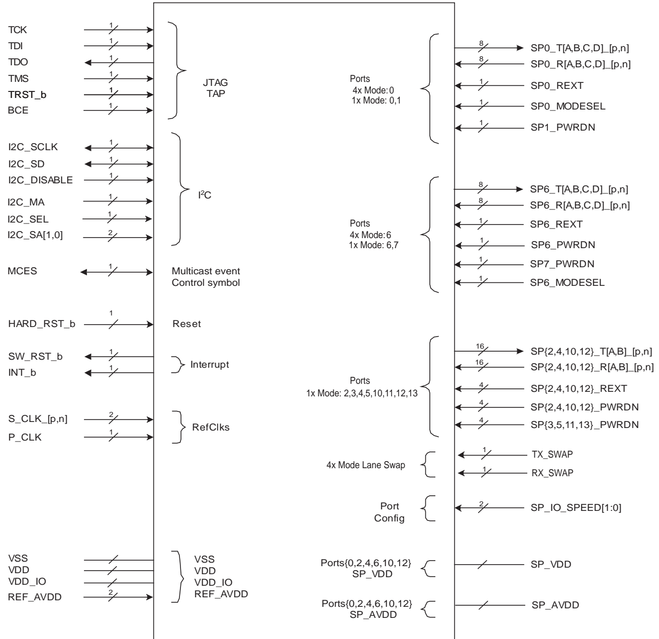
Figure 49: Signal Groupings
