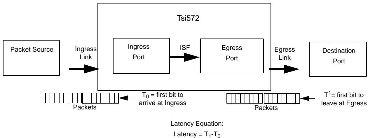
Figure 39: Latency Illustration
