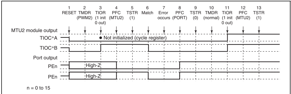
Figure 12.129 Error Occurrence in PWM Mode 2, Recovery in Normal Mode
