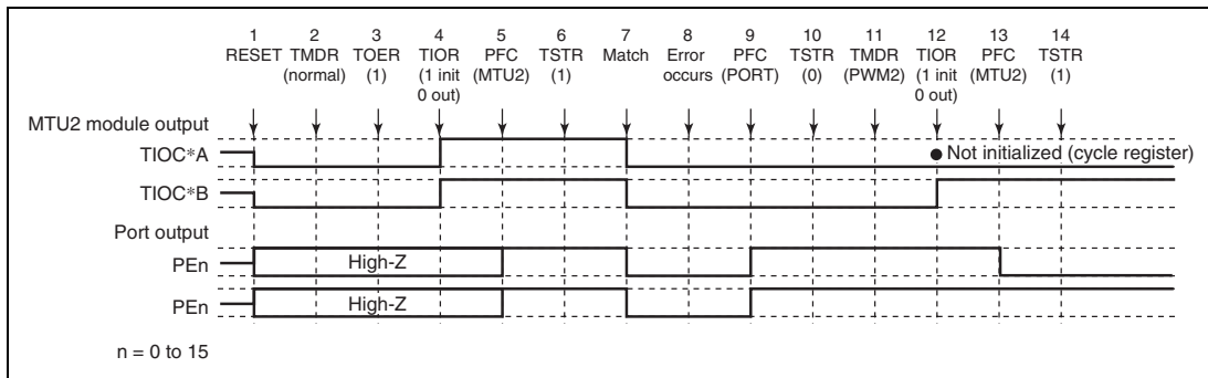
Figure 12.119 Error Occurrence in Normal Mode, Recovery in PWM Mode 2
