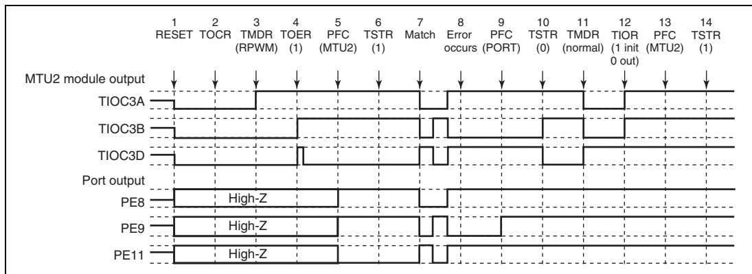
Figure 12.142 Error Occurrence in Reset-Synchronized PWM Mode, Recovery in Normal Mode
