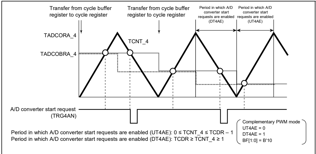
Figure 12.74 Basic Example of A/D Converter Start Request Signal (TRG4AN) Operation
