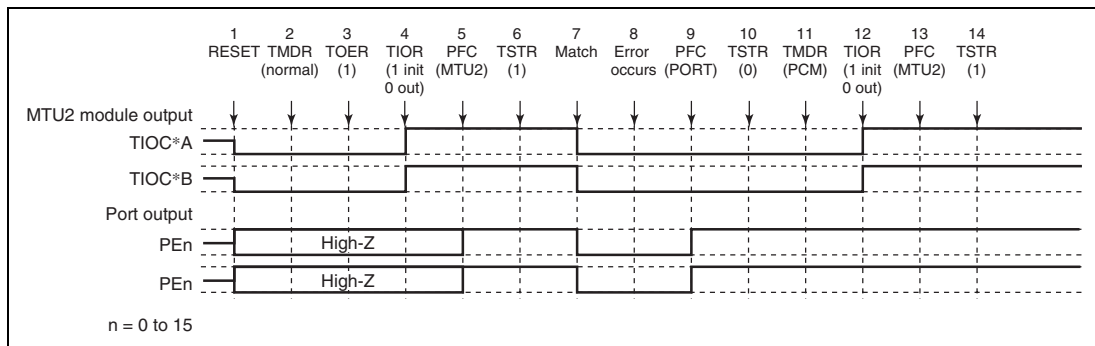
Figure 12.120 Error Occurrence in Normal Mode, Recovery in Phase Counting Mode
