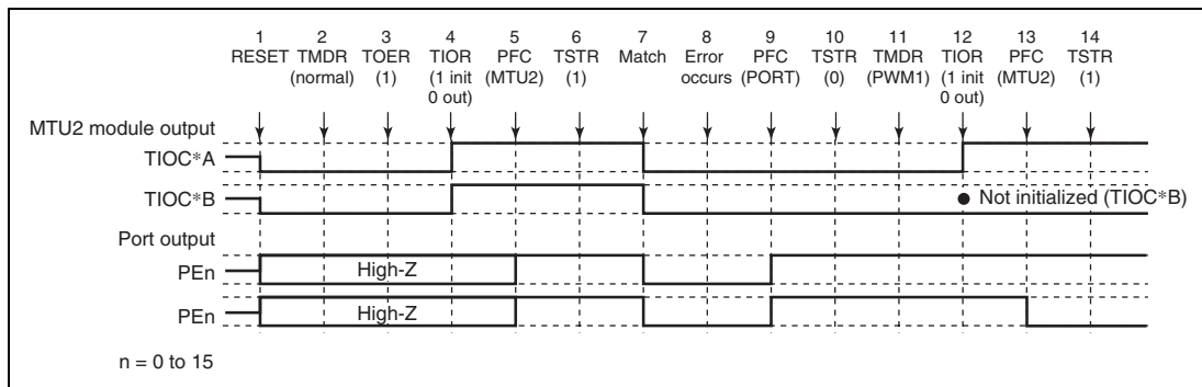
Figure 12.118 Error Occurrence in Normal Mode, Recovery in PWM Mode 1
