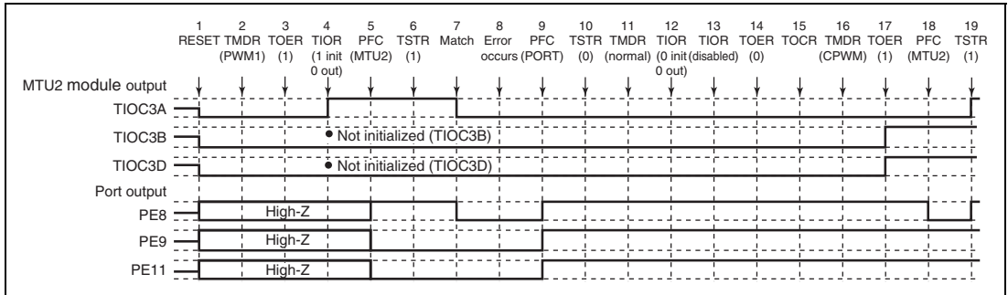
Figure 12.127 Error Occurrence in PWM Mode 1, Recovery in Complementary PWM Mode
