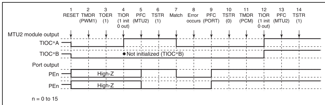
Figure 12.126 Error Occurrence in PWM Mode 1, Recovery in Phase Counting Mode
