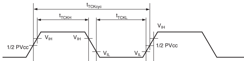
Figure 35.60 TCK Input Timing
