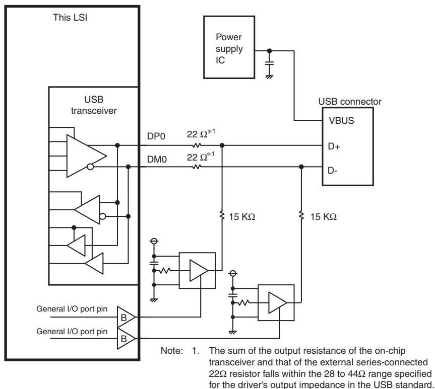
Figure 27.1 (2) Example of Connection to a USB Connector (when Host Controller Operation is Selected)
