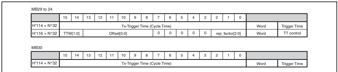
Figure 22.6 Tx-Trigger control field
