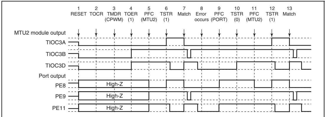
Figure 12.139 Error Occurrence in Complementary PWM Mode, Recovery in Complementary PWM Mode
