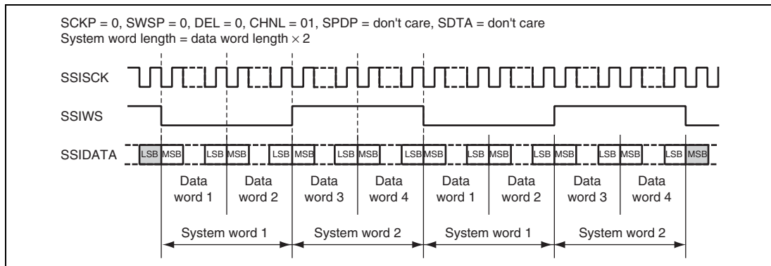
Figure 20.6 Multi-Channel Format (4 Channels Without Padding)
