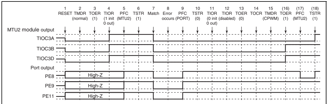
Figure 12.121 Error Occurrence in Normal Mode, Recovery in Complementary PWM Mode
