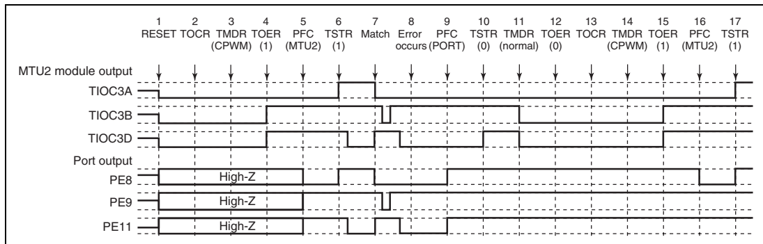
Figure 12.140 Error Occurrence in Complementary PWM Mode, Recovery in Complementary PWM Mode
