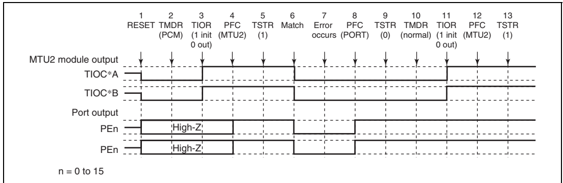
Figure 12.133 Error Occurrence in Phase Counting Mode, Recovery in Normal Mode
