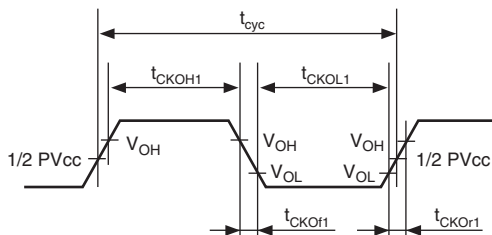
Figure 35.2 (1) CKIO Clock Output Timing 1
