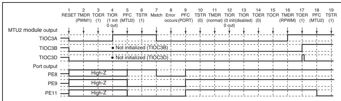
Figure 12.128 Error Occurrence in PWM Mode 1, Recovery in Reset-Synchronized PWM Mode
