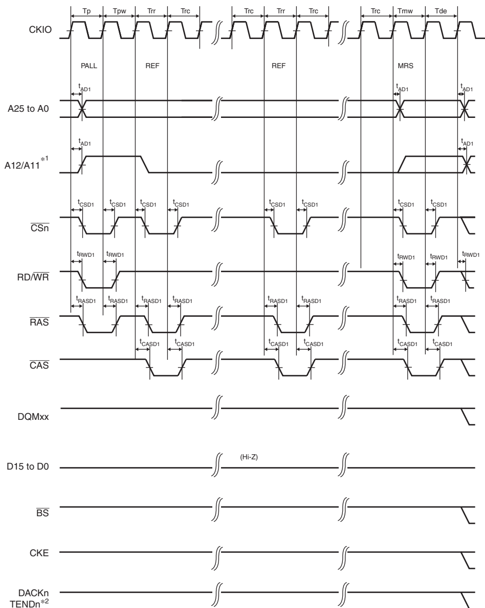
Figure 35.31 Synchronous DRAM Mode Register Write Timing (WTRP = 1 Cycle)
