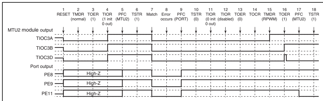
Figure 12.122 Error Occurrence in Normal Mode, Recovery in Reset-Synchronized PWM Mode
