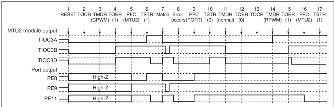
Figure 12.141 Error Occurrence in Complementary PWM Mode, Recovery in Reset-Synchronized PWM Mode
