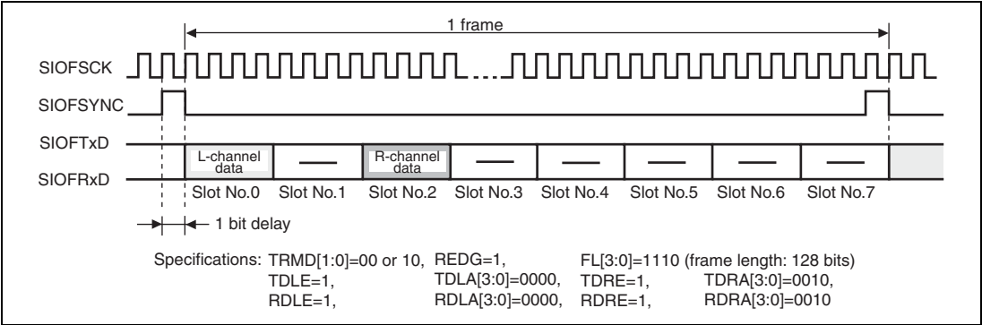
Figure 21.14 Transmit and Receive Timing (16-Bit Stereo Data (2))
