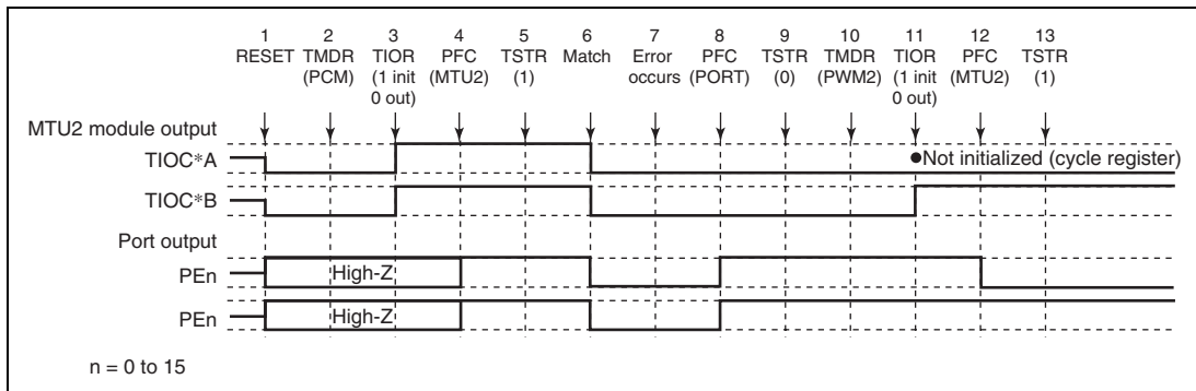
Figure 12.135 Error Occurrence in Phase Counting Mode, Recovery in PWM Mode 2
