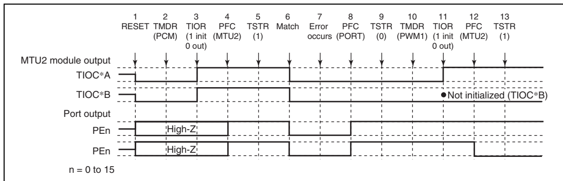
Figure 12.134 Error Occurrence in Phase Counting Mode, Recovery in PWM Mode 1
