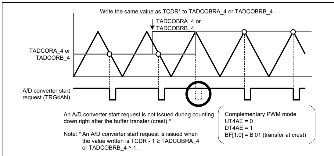
Figure 12.116 A/D Converter Start Request When the Same Value as TCDR is Written to TADCOBRA_4 or TADCOBRB_4
