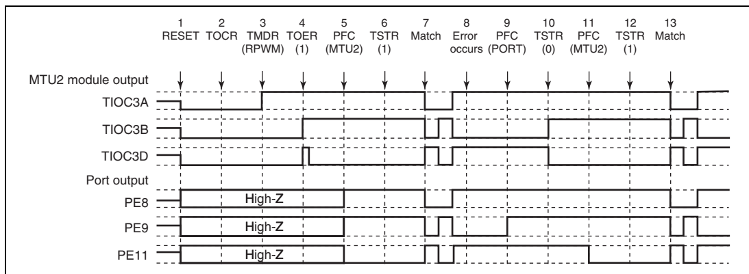
Figure 12.145 Error Occurrence in Reset-Synchronized PWM Mode, Recovery in Reset-Synchronized PWM Mode
