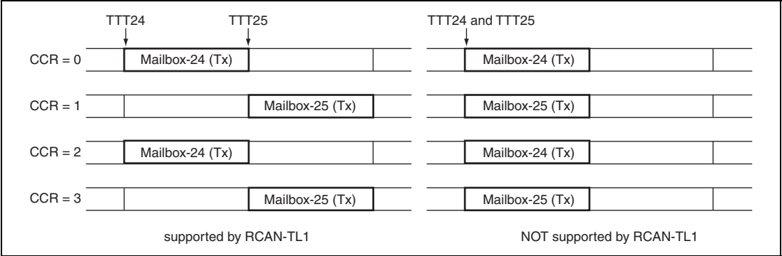
Figure 22.18 Limitation on Tx-Trigger Time
