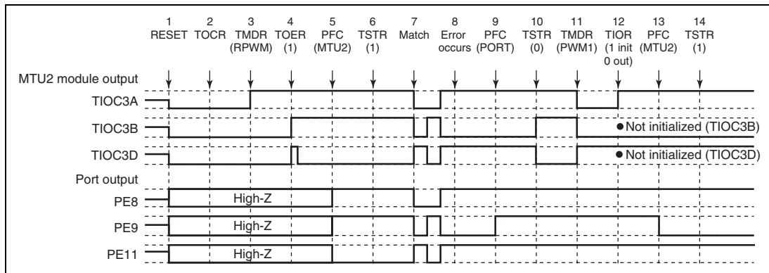
Figure 12.143 Error Occurrence in Reset-Synchronized PWM Mode, Recovery in PWM Mode 1
