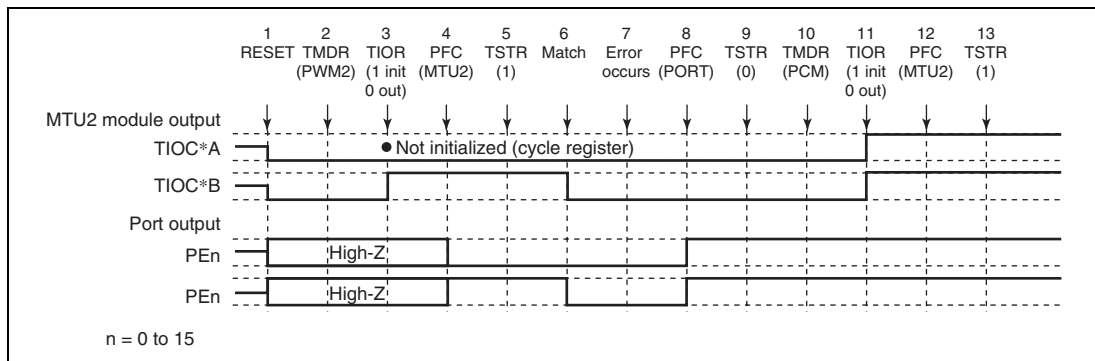
Figure 12.132 Error Occurrence in PWM Mode 2, Recovery in Phase Counting Mode
