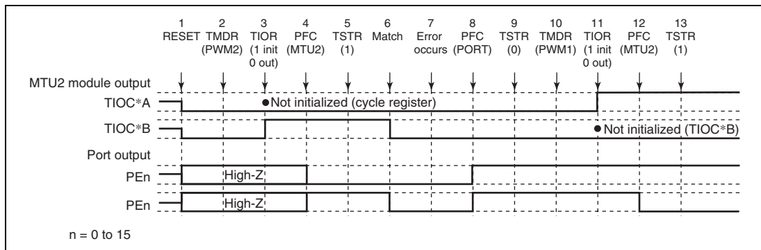
Figure 12.130 Error Occurrence in PWM Mode 2, Recovery in PWM Mode 1
