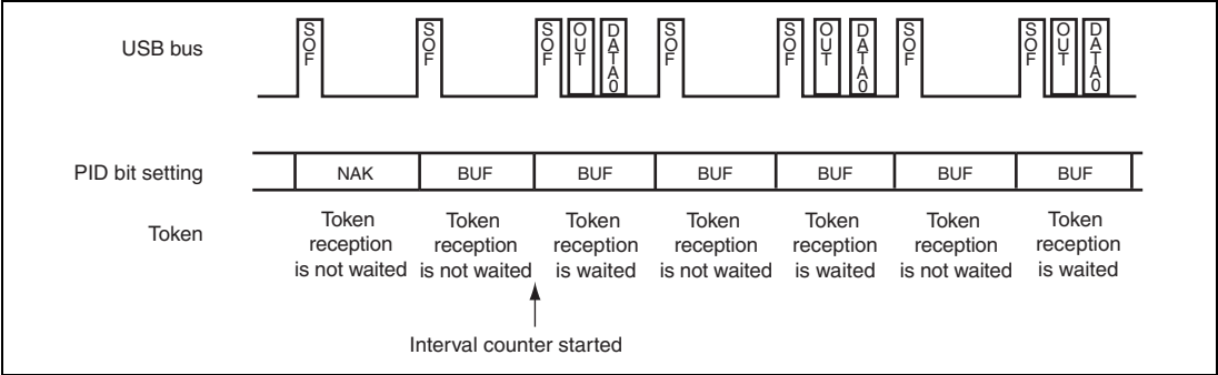
Figure 27.11 Relationship between Frames and Expected Token Reception when IITV = 1
