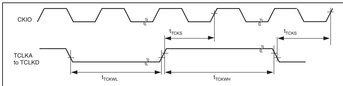
Figure 35.35 Clock Input Timing
