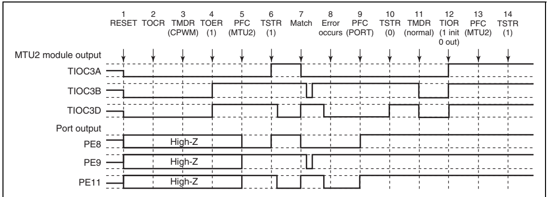
Figure 12.137 Error Occurrence in Complementary PWM Mode, Recovery in Normal Mode
