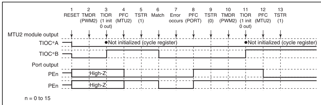
Figure 12.131 Error Occurrence in PWM Mode 2, Recovery in PWM Mode 2
