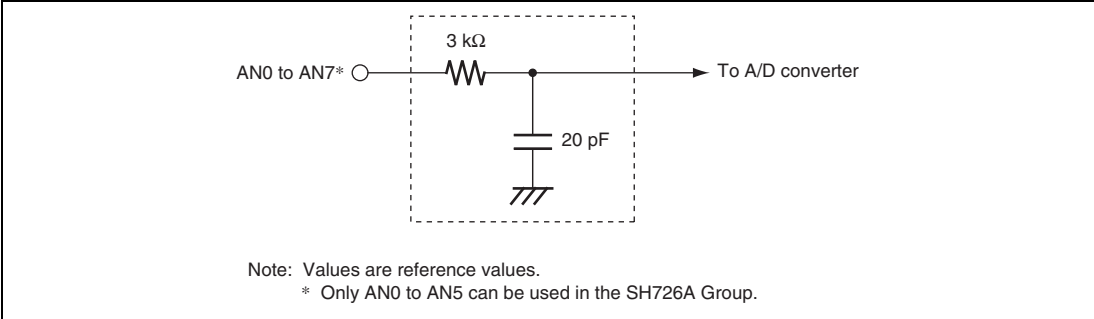
Figure 26.9 Analog Input Pin Equivalent Circuit
