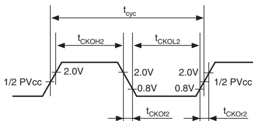
Figure 35.2 (2) CKIO Clock Output Timing 2
