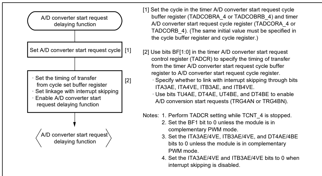
Figure 12.73 Example of Procedure for Specifying A/D Converter Start Request Delaying Function
