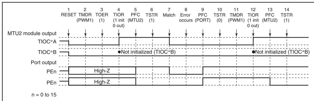
Figure 12.124 Error Occurrence in PWM Mode 1, Recovery in PWM Mode 1
