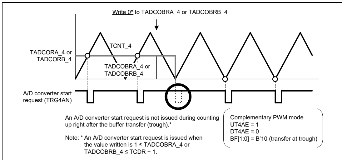
Figure 12.115 A/D Converter Start Request When 0 is Written to TADCOBRA_4 or TADCOBRB_4
