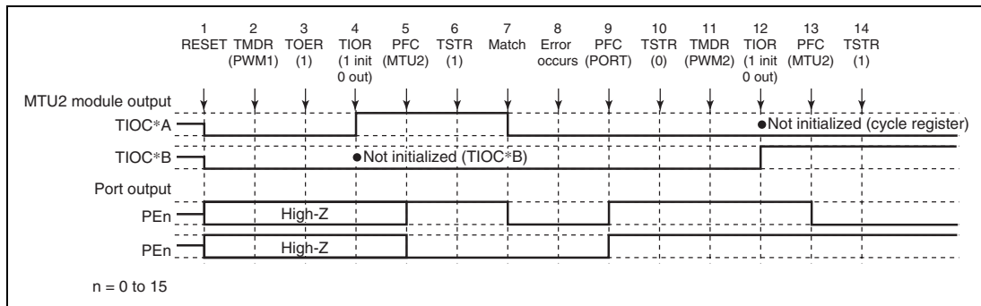
Figure 12.125 Error Occurrence in PWM Mode 1, Recovery in PWM Mode 2
