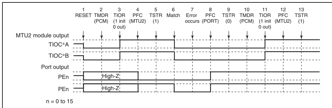
Figure 12.136 Error Occurrence in Phase Counting Mode, Recovery in Phase Counting Mode
