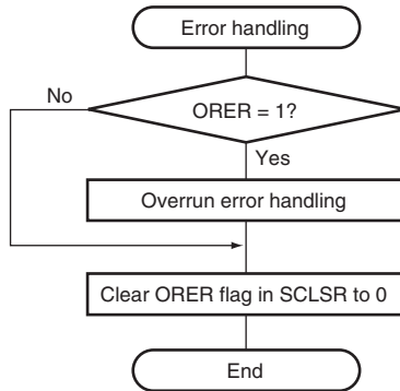
Figure 16.16 Sample Flowchart for Receiving Serial Data (2)
