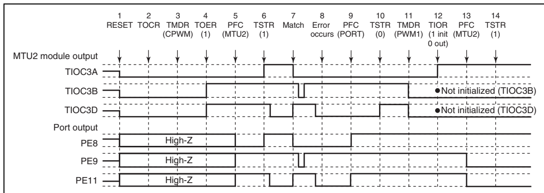
Figure 12.138 Error Occurrence in Complementary PWM Mode, Recovery in PWM Mode 1
