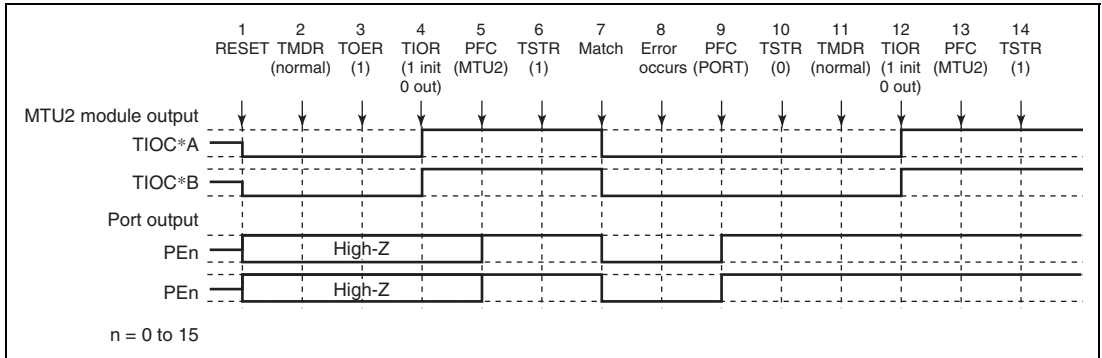
Figure 12.117 Error Occurrence in Normal Mode, Recovery in Normal Mode
