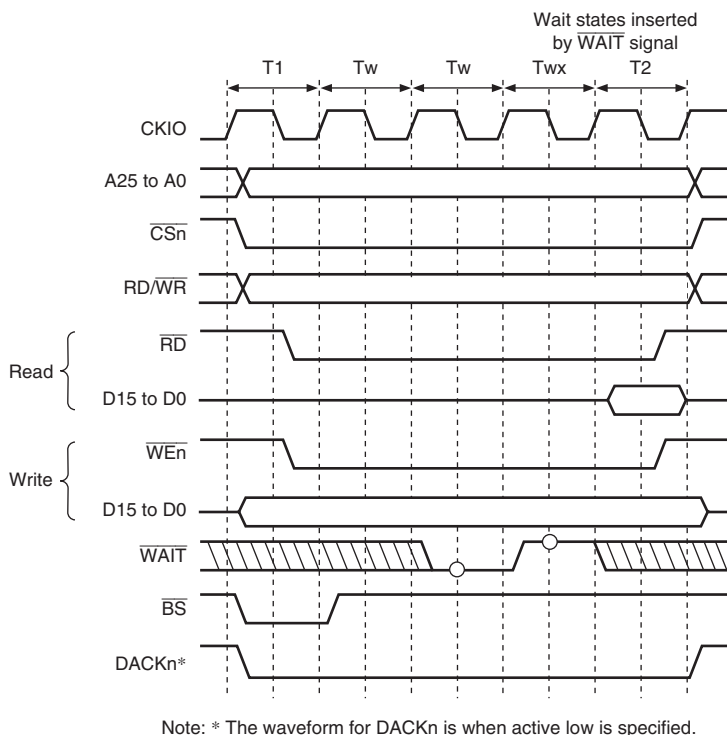
Figure 10.8 Wait Cycle Timing for Normal Space Access (Wait Cycle Insertion Using WAIT Signal)
