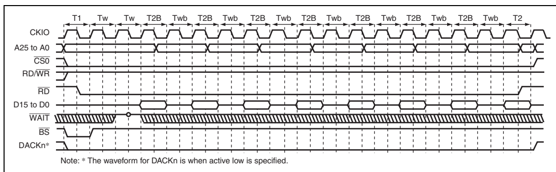
Figure 10.33 Burst ROM Access Timing (Clocked Synchronous) (Burst Length = 8, Wait Cycles Inserted in First Access = 2, Wait Cycles Inserted in Second and Subsequent Access Cycles = 1)
