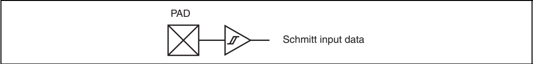
Figure 1.3 (1) Simplified Circuit Diagram (Schmitt Input Buffer)
