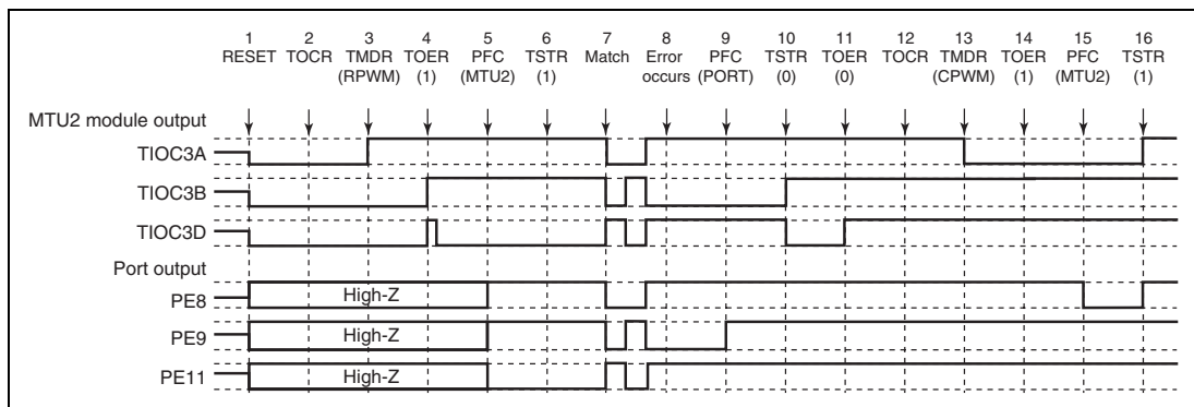
Figure 12.144 Error Occurrence in Reset-Synchronized PWM Mode, Recovery in Complementary PWM Mode
