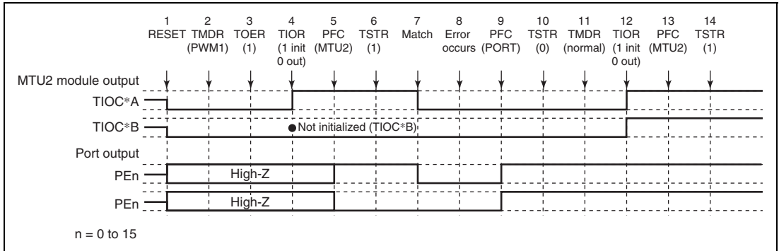
Figure 12.123 Error Occurrence in PWM Mode 1, Recovery in Normal Mode
