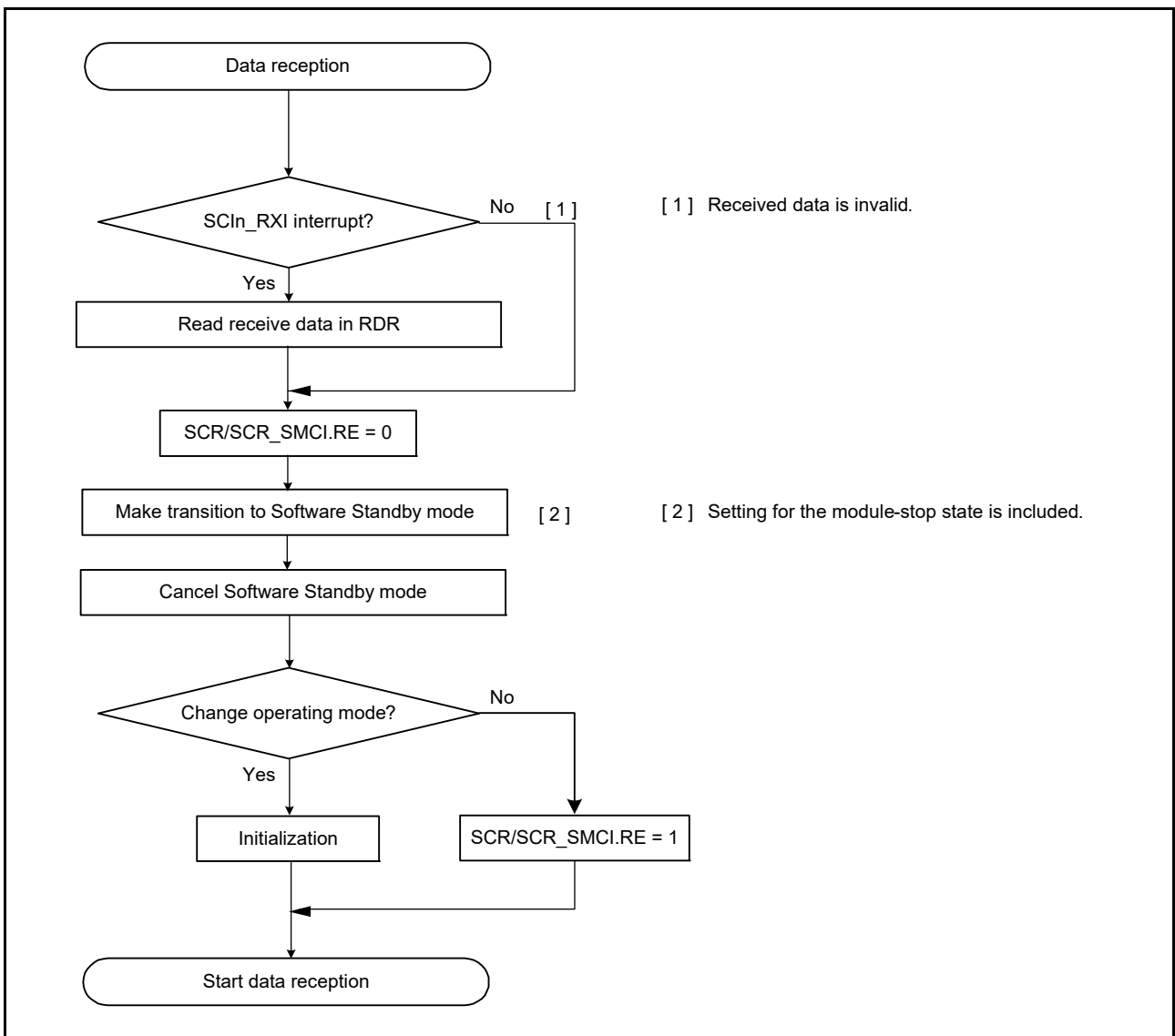
Figure 32.76 Example flow of transition to Software Standby mode during reception
