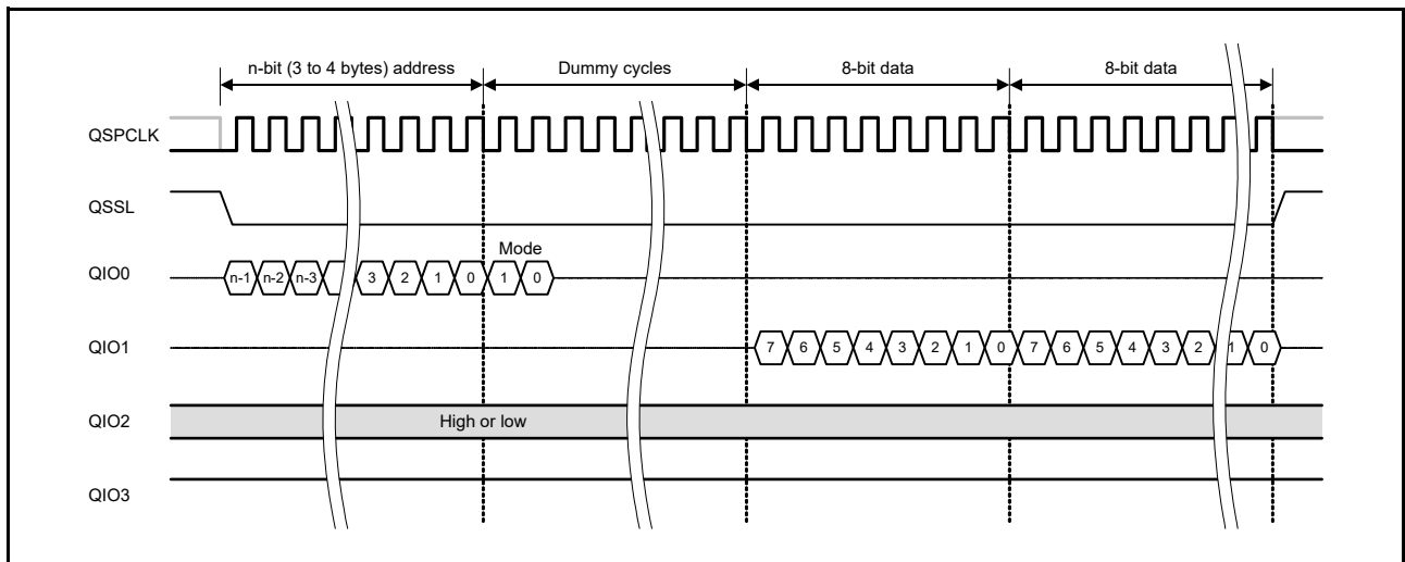
Figure 37.17 Fast Read bus cycle in XIP mode
