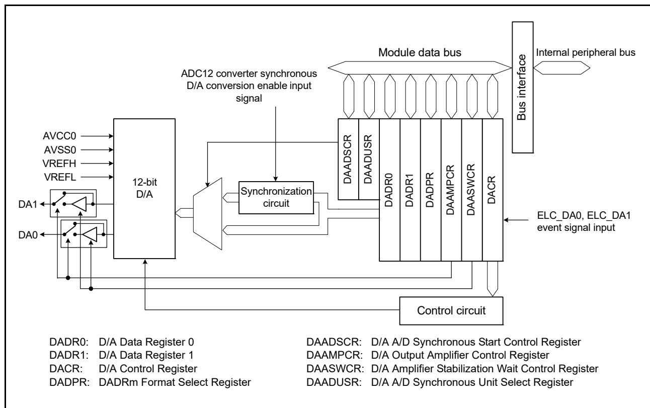
Figure 46.1 DAC12 block diagram
