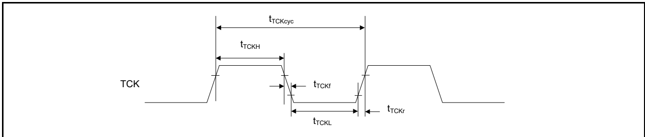
Figure 55.92 JTAG TCK timing
