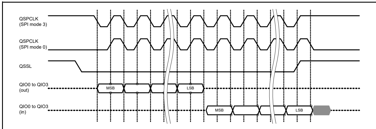
Figure 37.8 Basic serial interface timing
