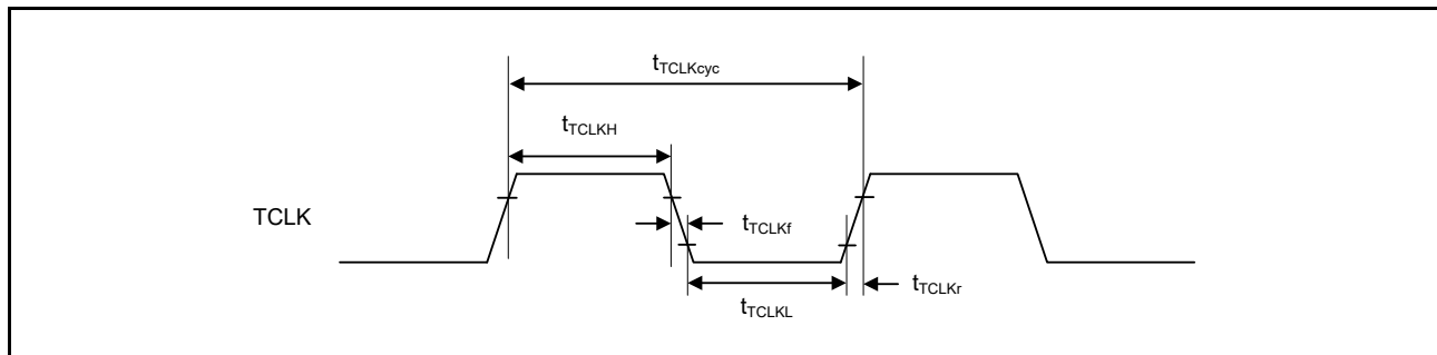
Figure 55.96 ETM TCLK timing
