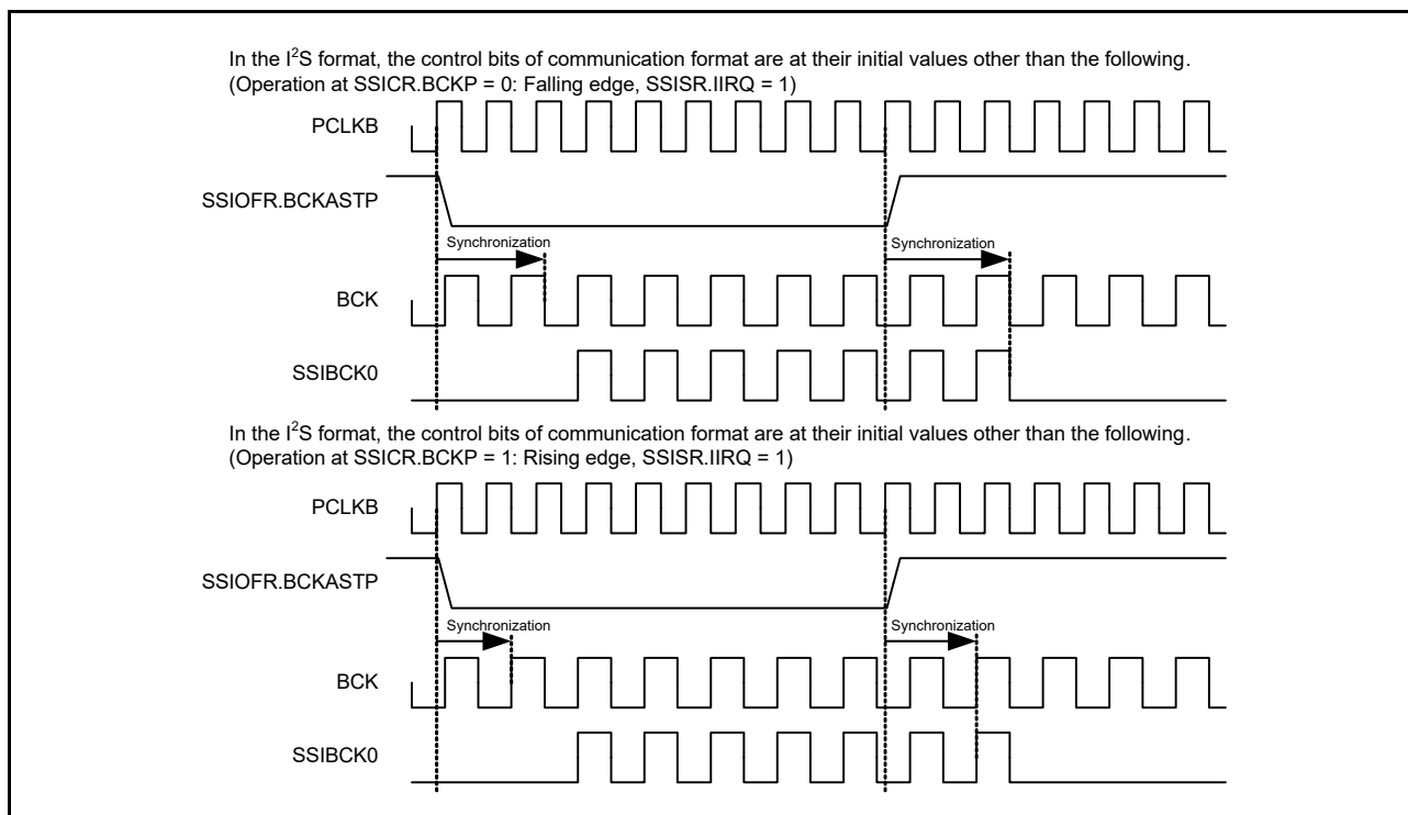
Figure 39.45 Example of stopping SSIBCK0 with SSIOFR.BCKASTP
