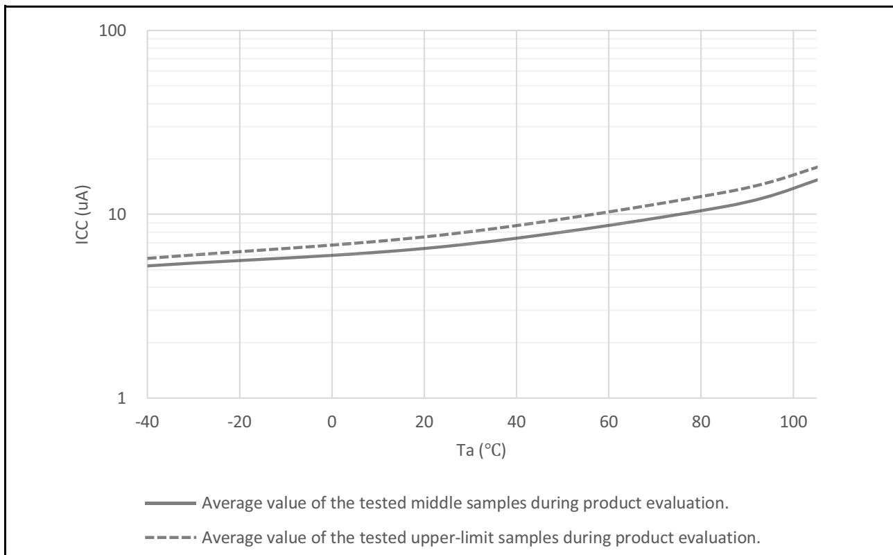
Figure 55.5 Temperature dependency in Deep Software Standby mode, power not supplied to SRAM or USB resume detecting unit, power-on reset circuit low power function enabled (reference data)
