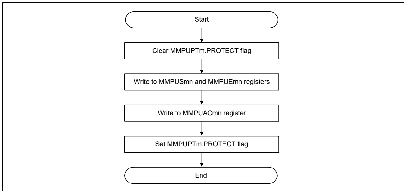
Figure 16.8 Register setting flow for region addition
