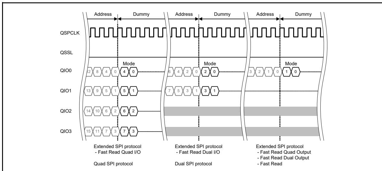
Figure 37.32 XIP mode control data
