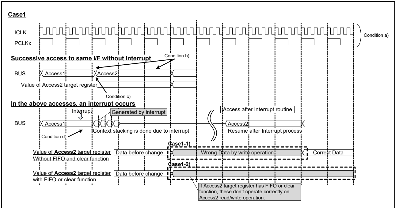
Figure 15.66 A wrong access to target register of Access2 (Case1)
