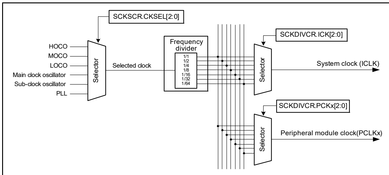
Figure 9.13 Clock source selector block diagram
