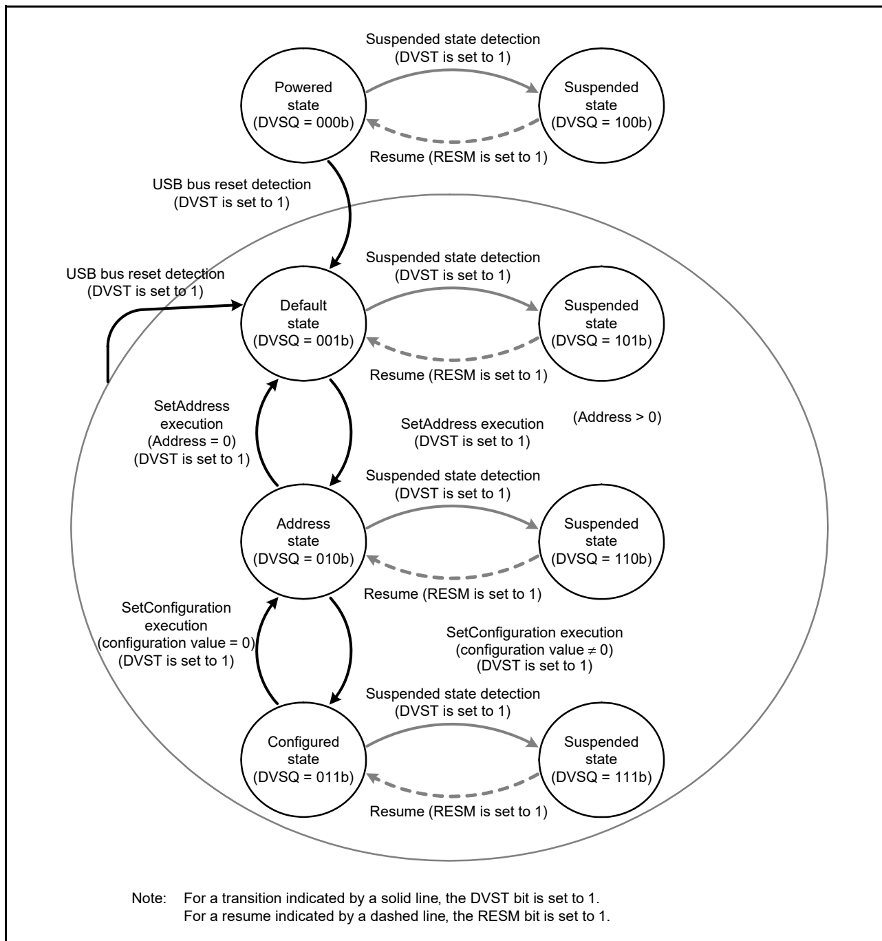
Figure 31.14 Device state transitions
