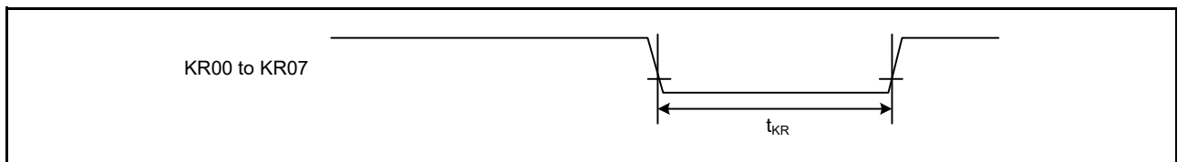
Figure 55.39 Key interrupt input timing
