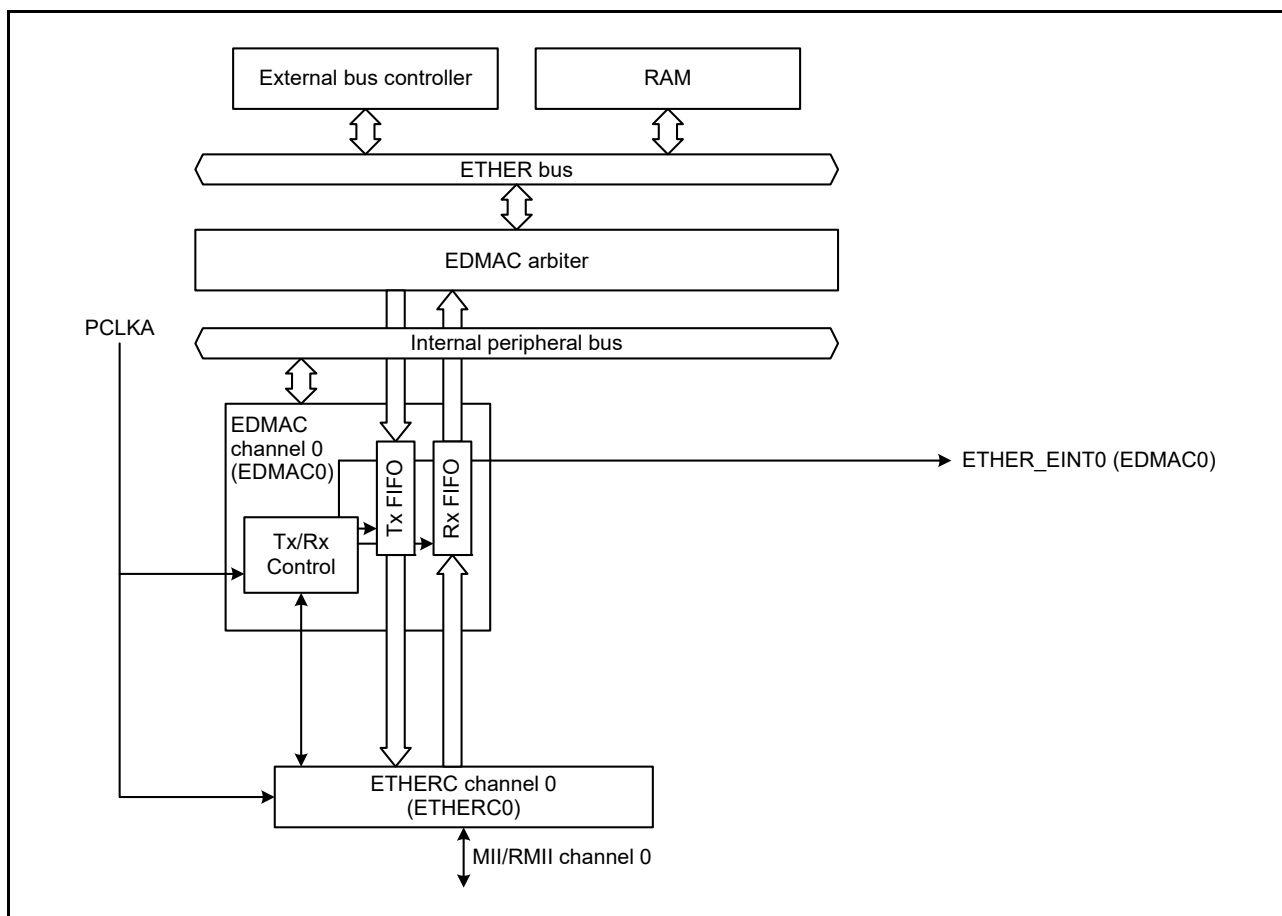
Figure 30.1 EDMAC configuration
