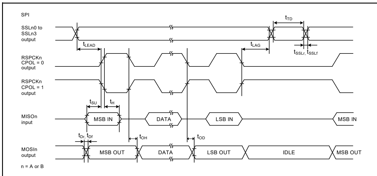
Figure 55.49 SPI timing for master when CPHA = 0
