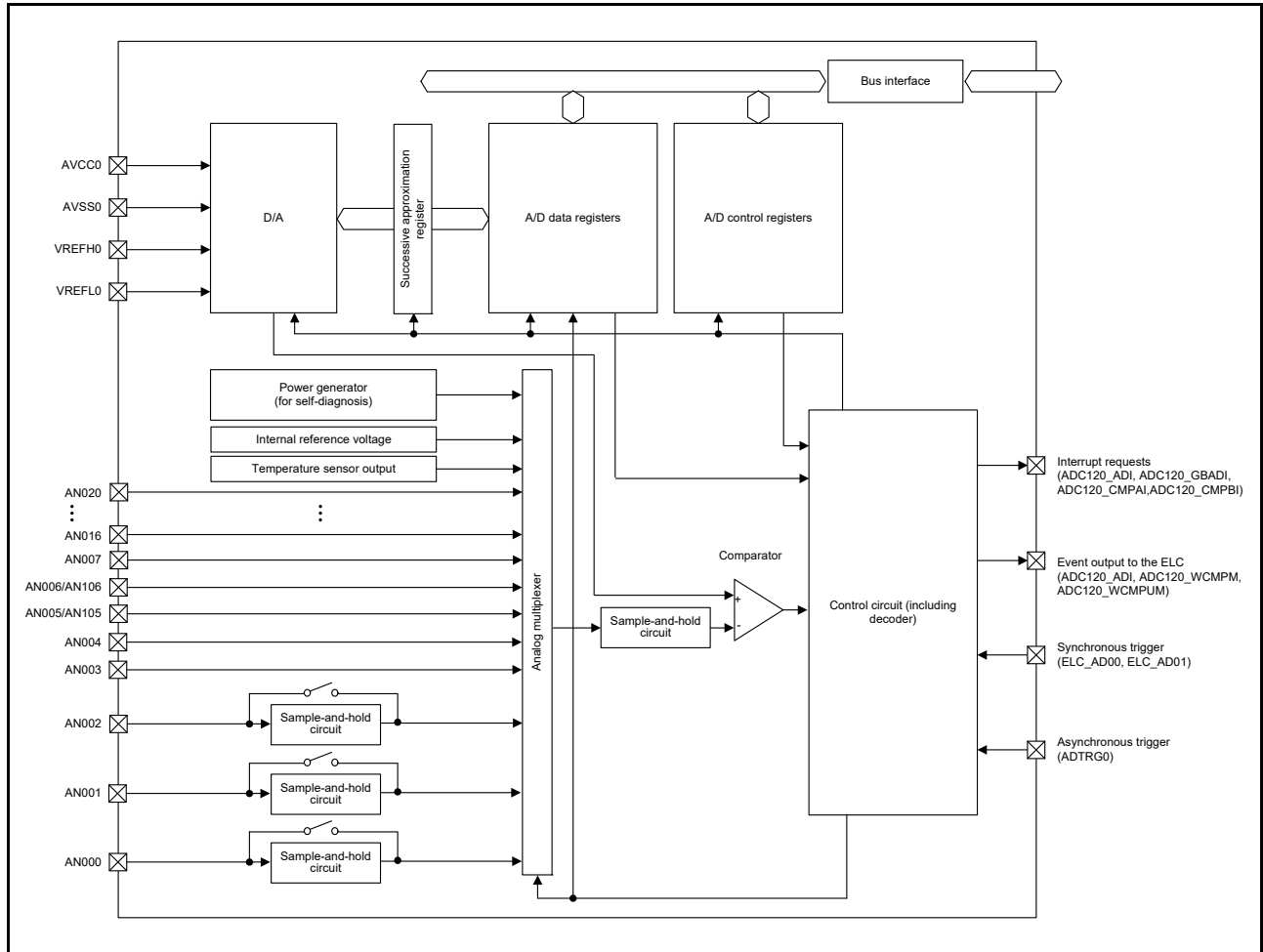
Figure 45.1 ADC12 unit 0 block diagram
