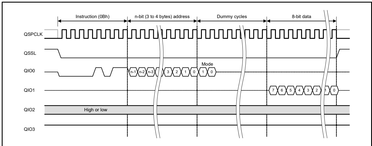
Figure 37.16 Fast Read bus cycle
