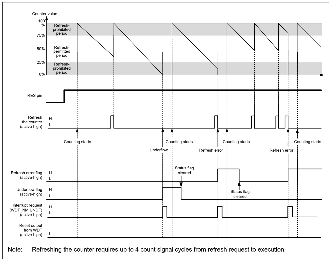
Figure 27.4 Operation example in auto start mode
