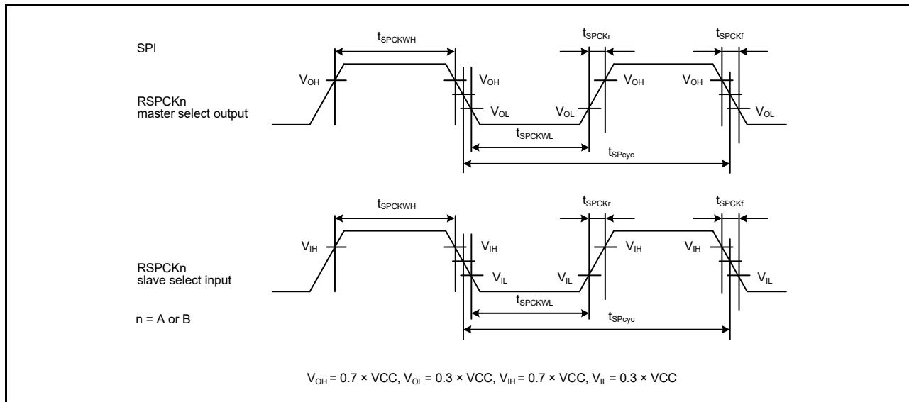
Figure 55.48 SPI clock timing
