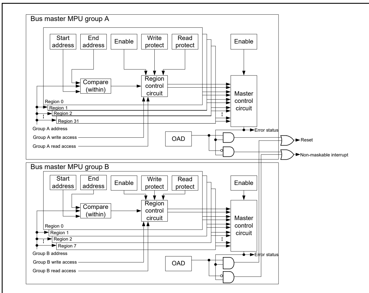
Figure 16.4 Bus master MPU groups A and B
