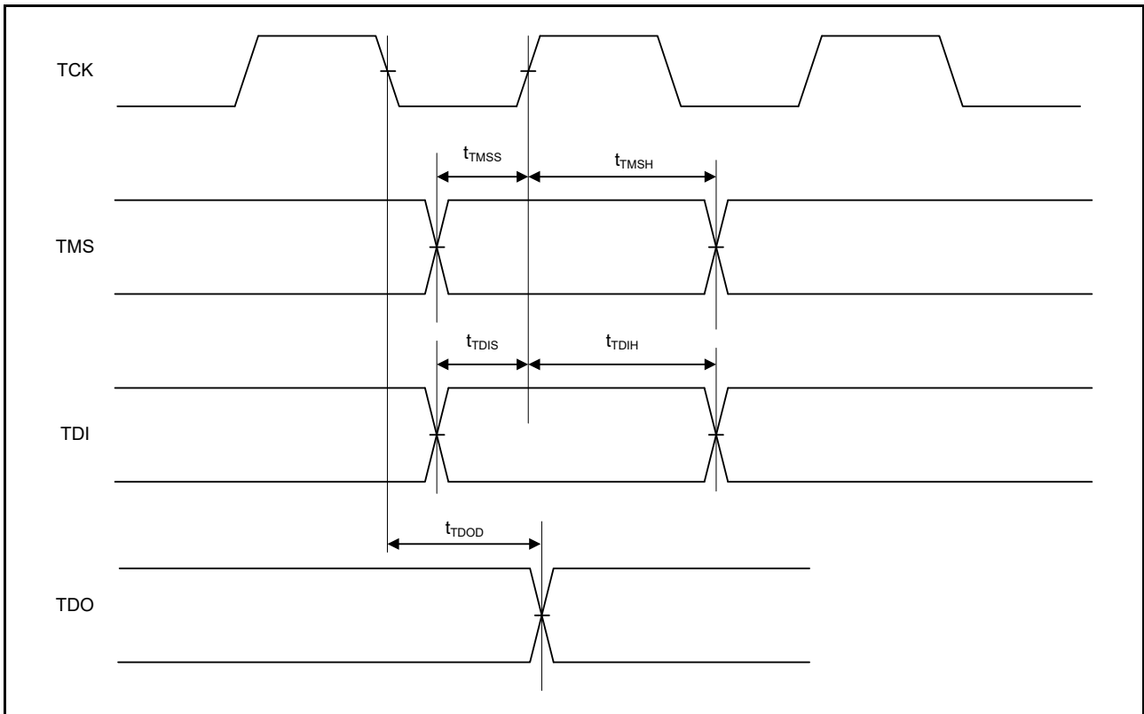
Figure 55.93 JTAG input/output timing
