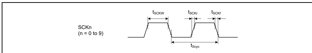
Figure 55.40 SCK clock input/output timing
