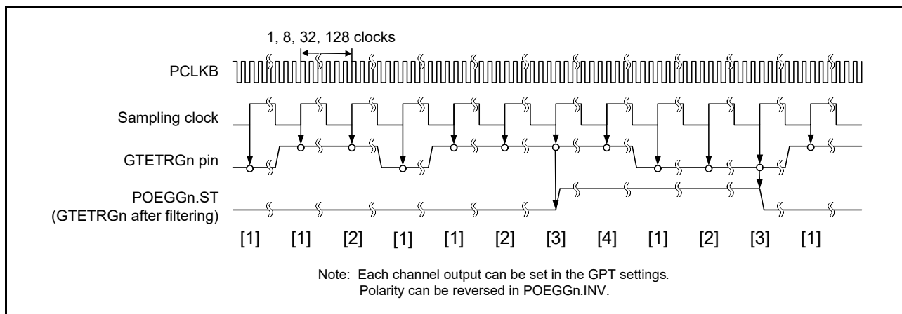
Figure 22.4 Output timing of external trigger to GPT
