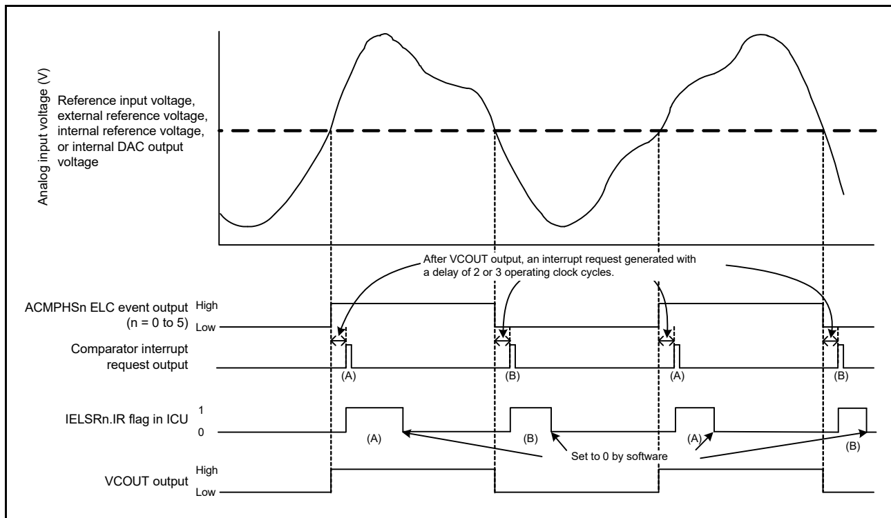
Figure 48.2 ACMPHS operation example
