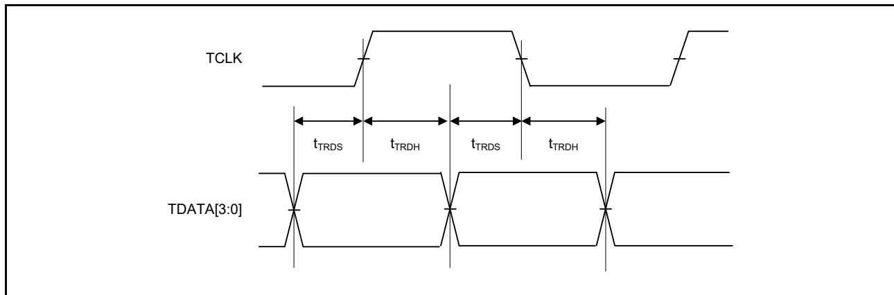
Figure 55.97 ETM output timing
