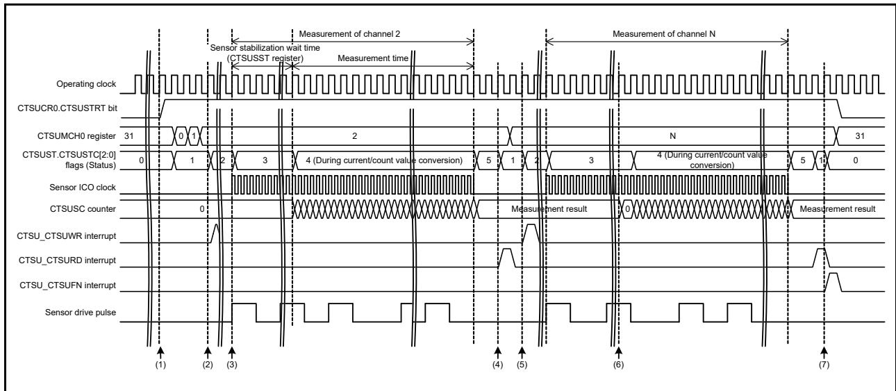
Figure 49.15 Timing of self-capacitance multi-scan mode when the measurement start condition is a software trigger
