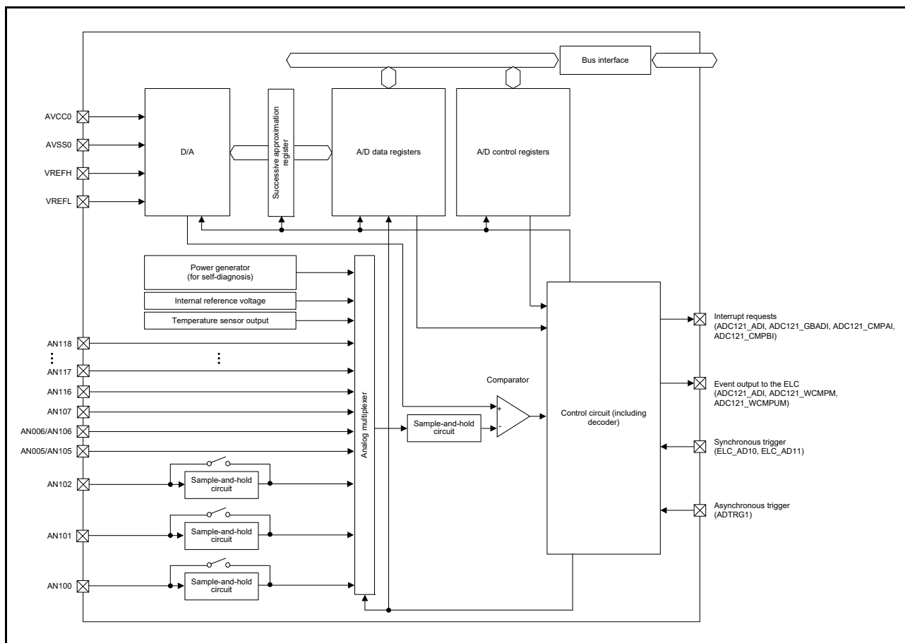
Figure 45.2 ADC12 unit 1 block diagram
