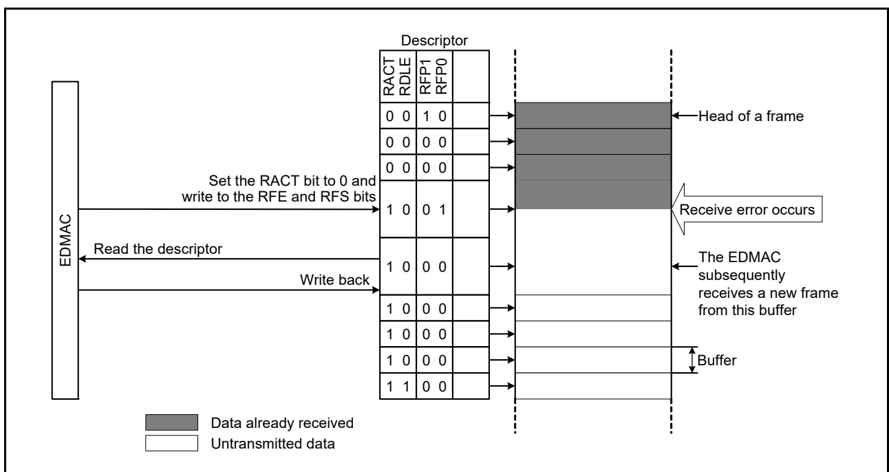
Figure 30.8 EDMAC operation after receive error occurs
