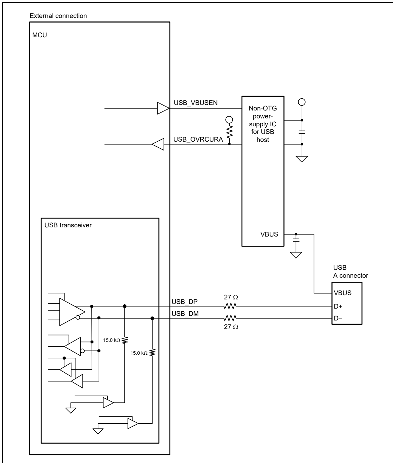
Figure 31.4 Example host connection
