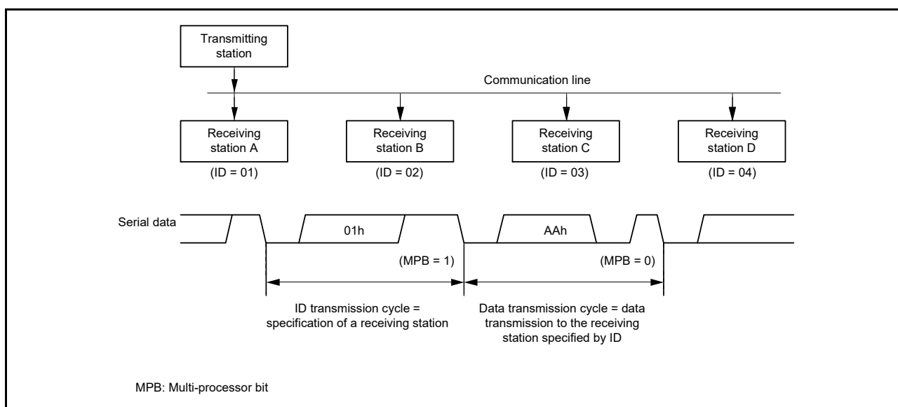
Figure 32.22 Example of communication using multi-processor format with transmission of data AAh to receiving station A
