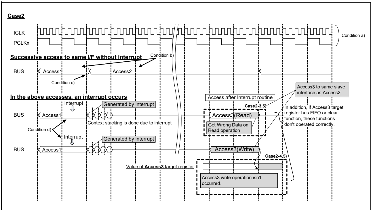
Figure 15.67 A wrong access in interrupt service routines (Case2)
