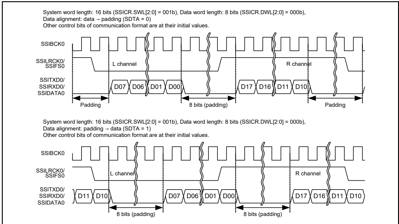
Figure 39.10 Alignment setting of serial data with padding bits
