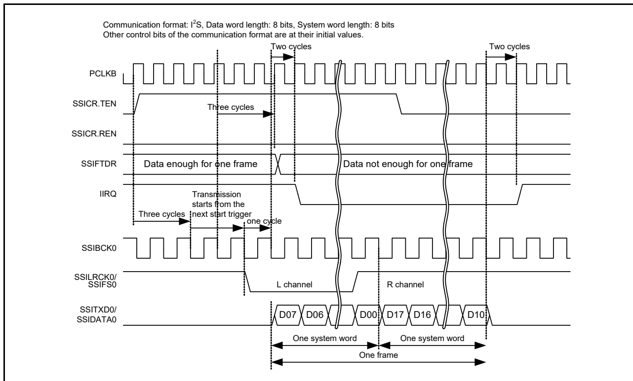
Figure 39.14 IIRQ setting timing (transmission)
