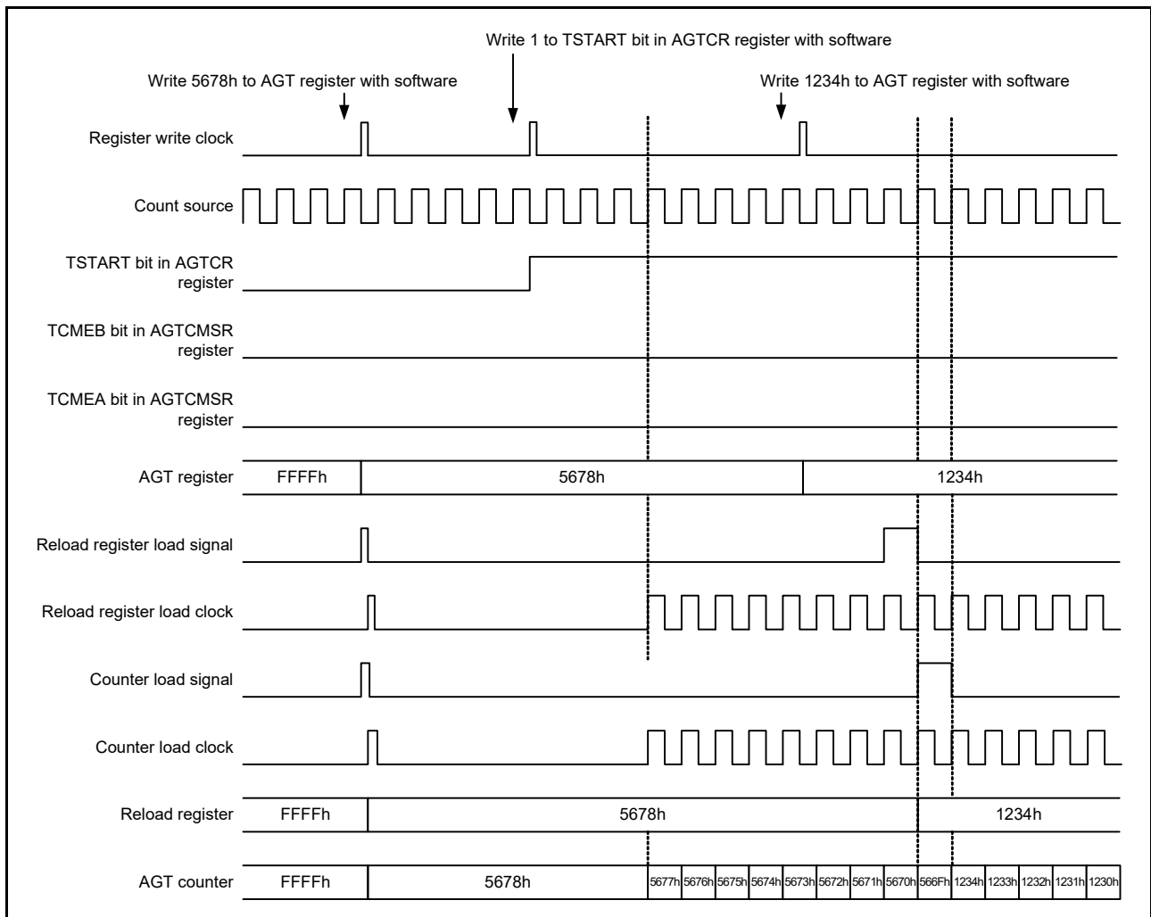
Figure 25.2 Timing of rewrite operation with TSTART, TCMEA and TCMEB bit values when compare match registers A and B are invalid
