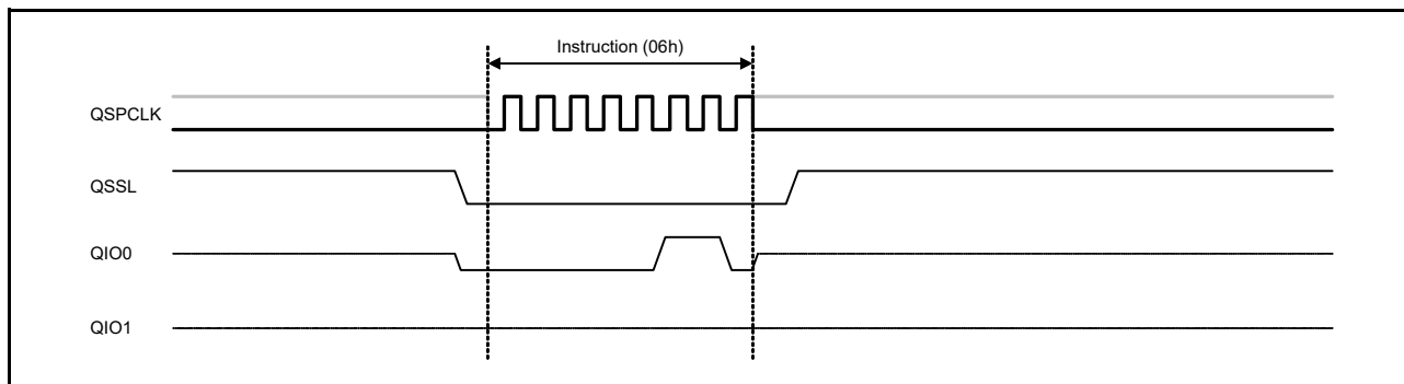
Figure 37.28 Write Enable bus cycle
