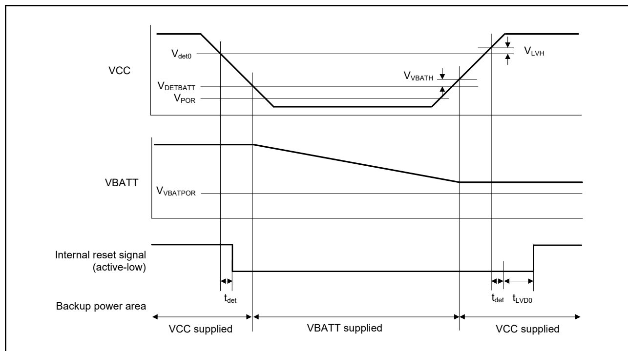
Figure 48.78 Power supply switching and LVD0 reset timing
