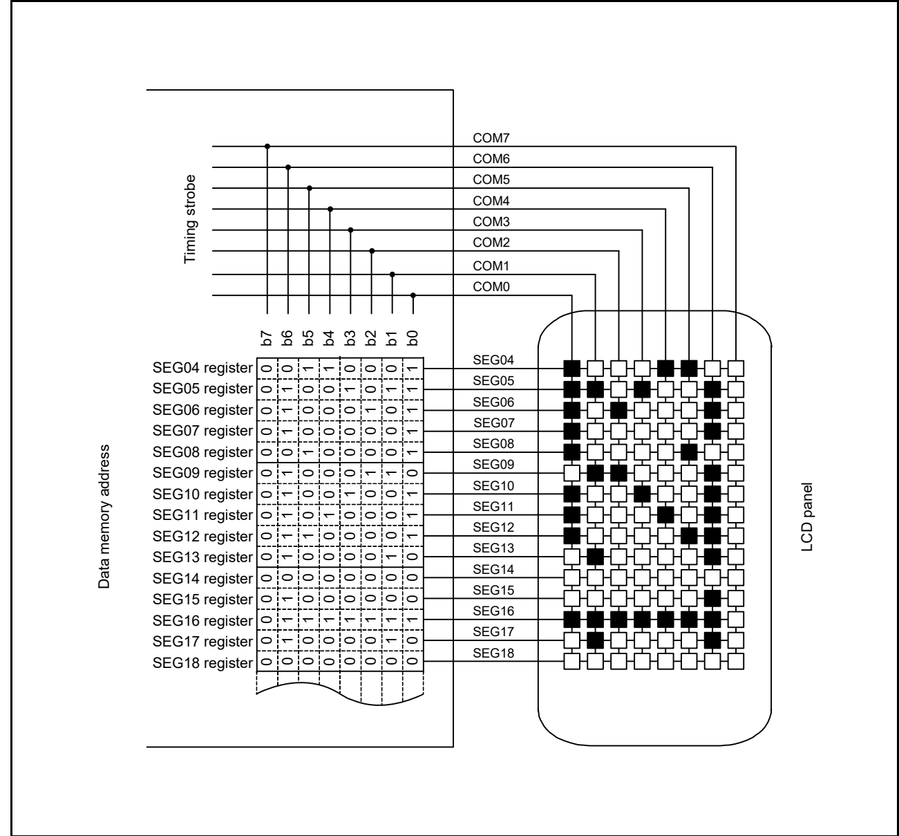
Figure 45.33 Example of connecting eight-time-slice LCD panel
