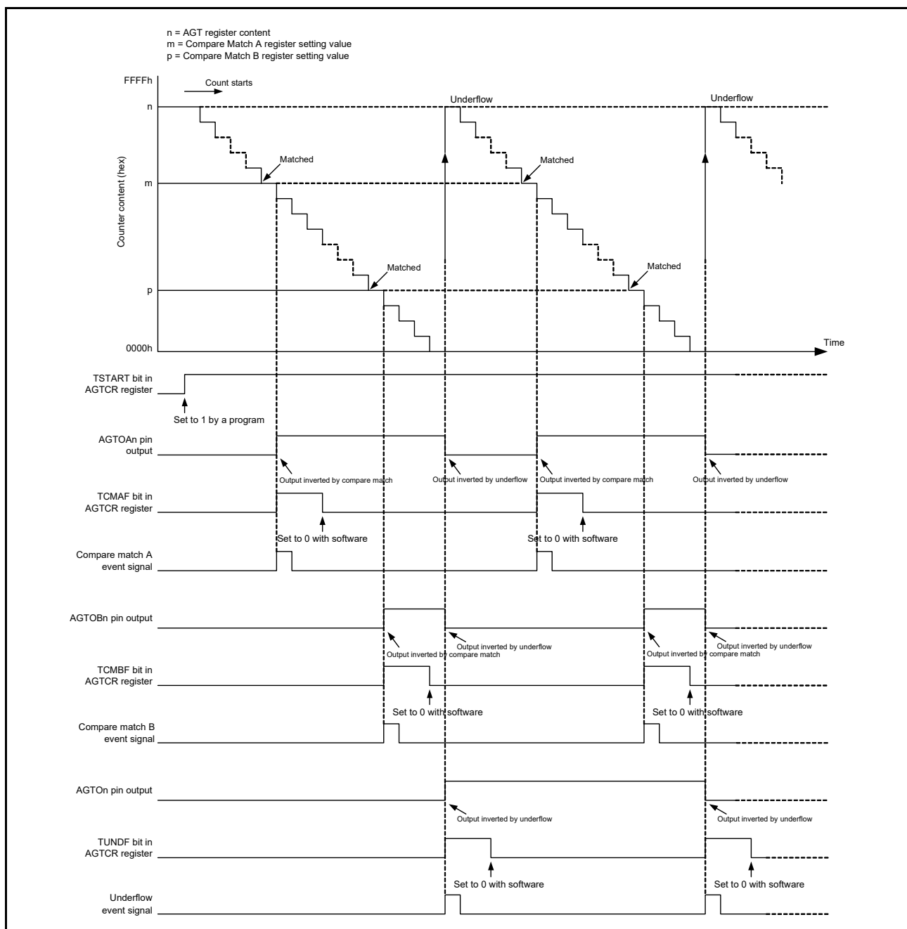
Figure 23.11 Operation example in compare match mode (TOPOLA = 0, TOPOLB = 0)
