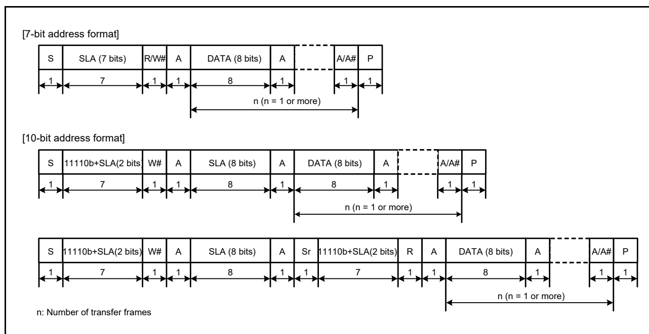
Figure 29.3 I 2 C bus format
