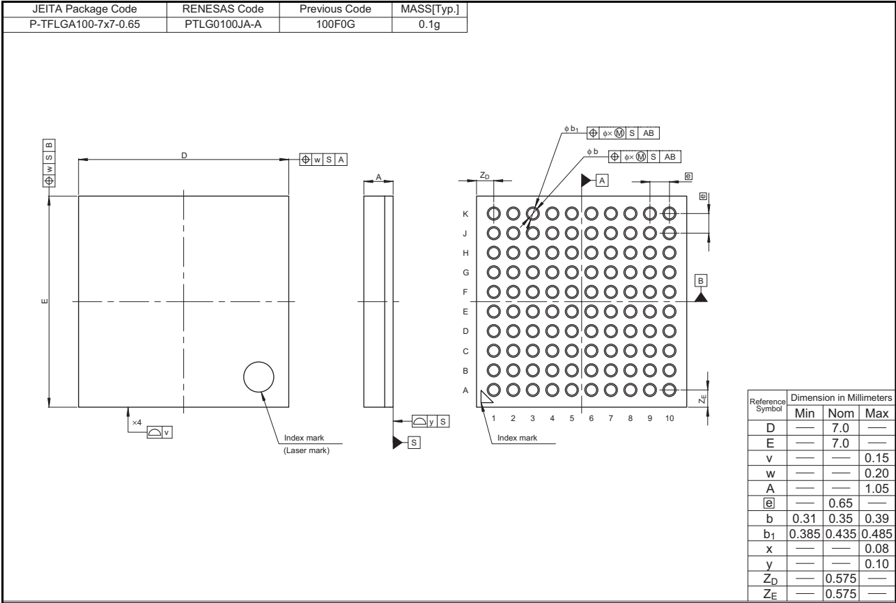
Figure 2.1 100-pin LGA
