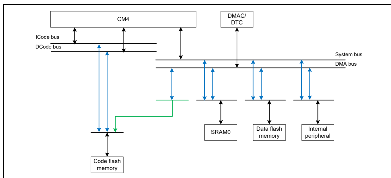
Figure 14.1 Bus configuration
