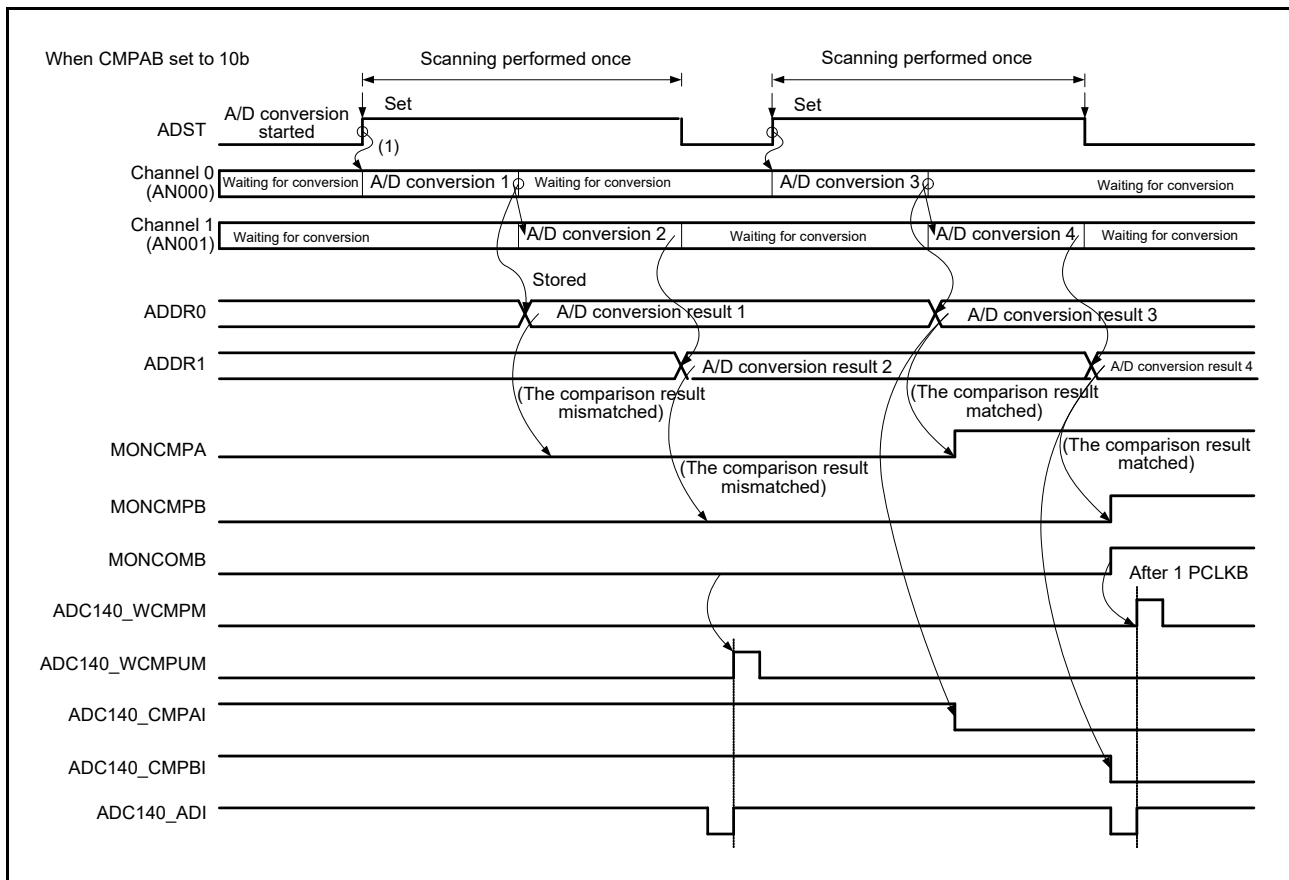
Figure 35.23 Event output operation example of compare function when AN000 to AN001 are compared
