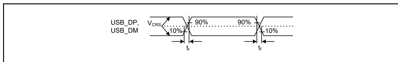
Figure 48.65 USB_DP and USB_DM output timing
