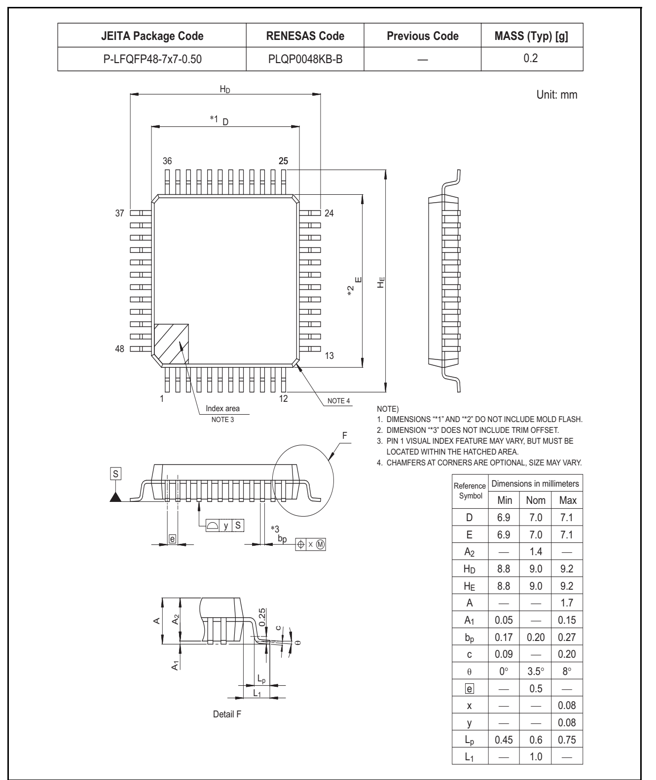
Figure 2.6 48-pin LQFP
