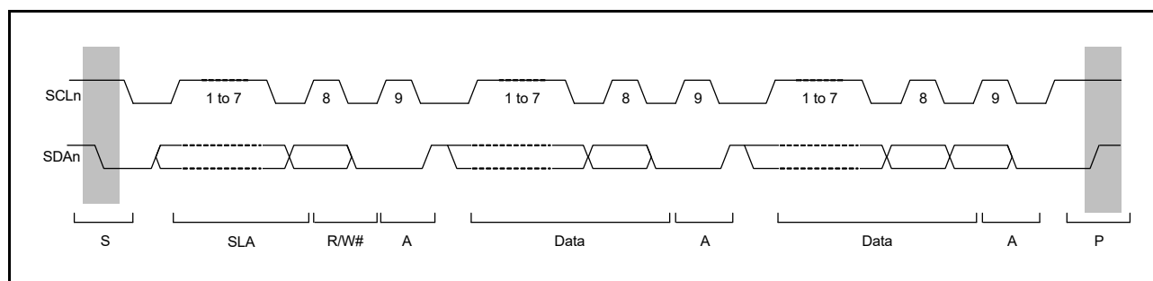
Figure 29.4 I 2 C bus timing (SLA = 7 bits)
