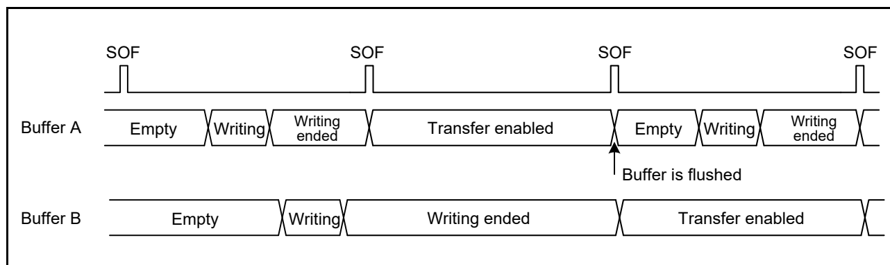
Figure 27.22 Example buffer flush operation
