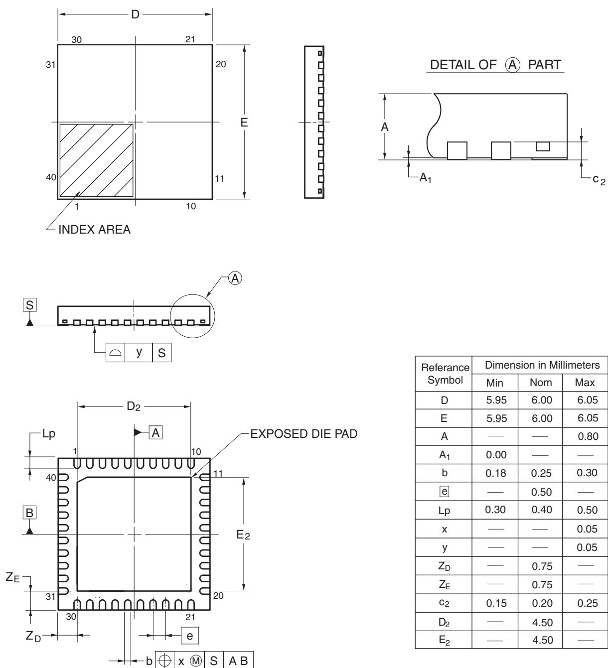
Figure 2.9 40-pin QFN (1)
