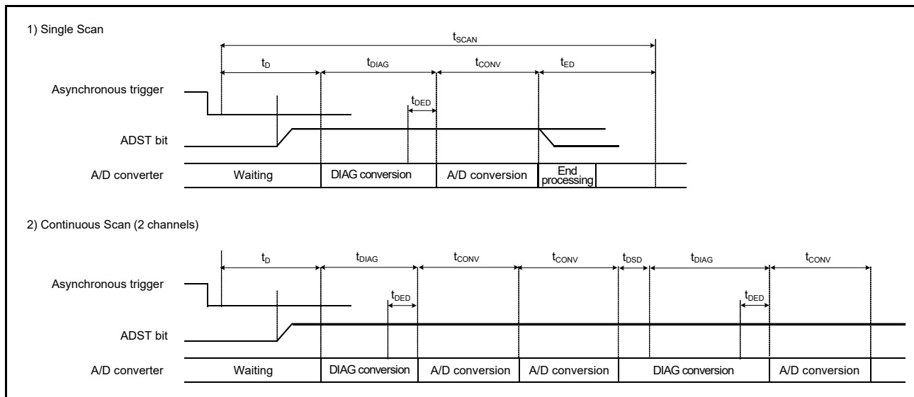
Figure 35.25 Scan conversion timing activated by asynchronous input (ADTRG0)
