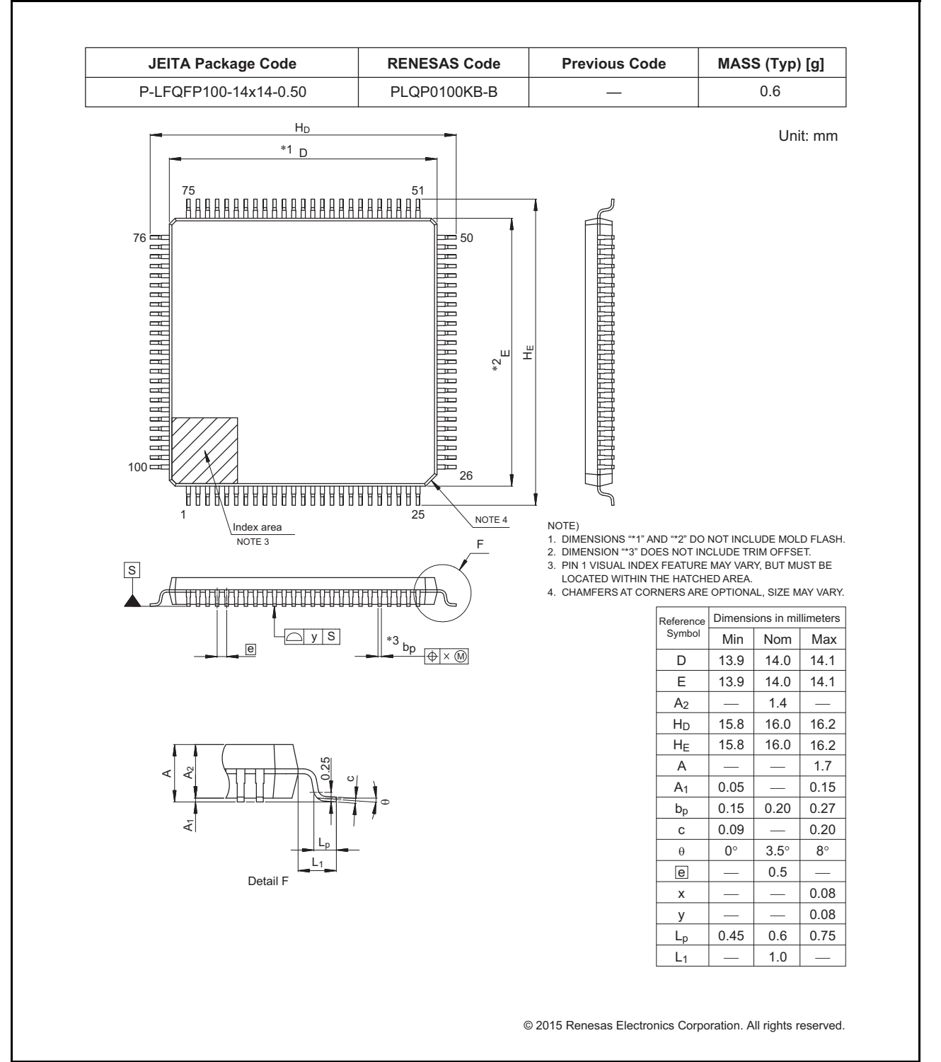
Figure 2.2 100-pin LQFP
