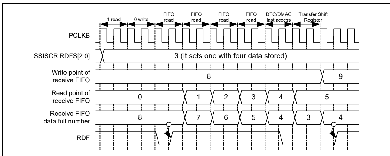
Figure 33.26 Timing diagram for setting and clearing RDF
