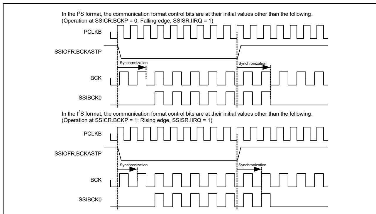
Figure 33.41 Example of stopping SSIBCK0 with SSIOFR.BCKASTP
