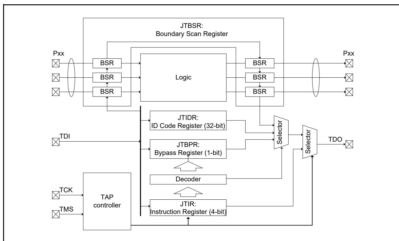
Figure 34.1 Boundary scan function block diagram
