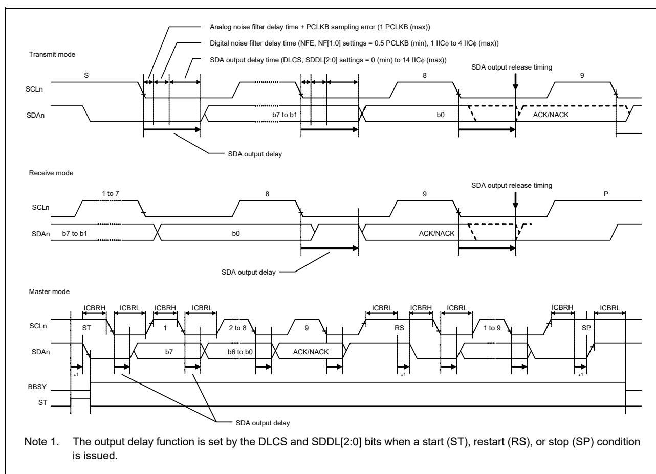
Figure 29.22 SDA output delay function
