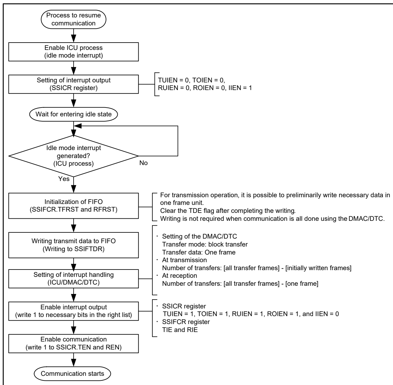
Figure 33.54 Procedure to resume communication (CPU operation)
