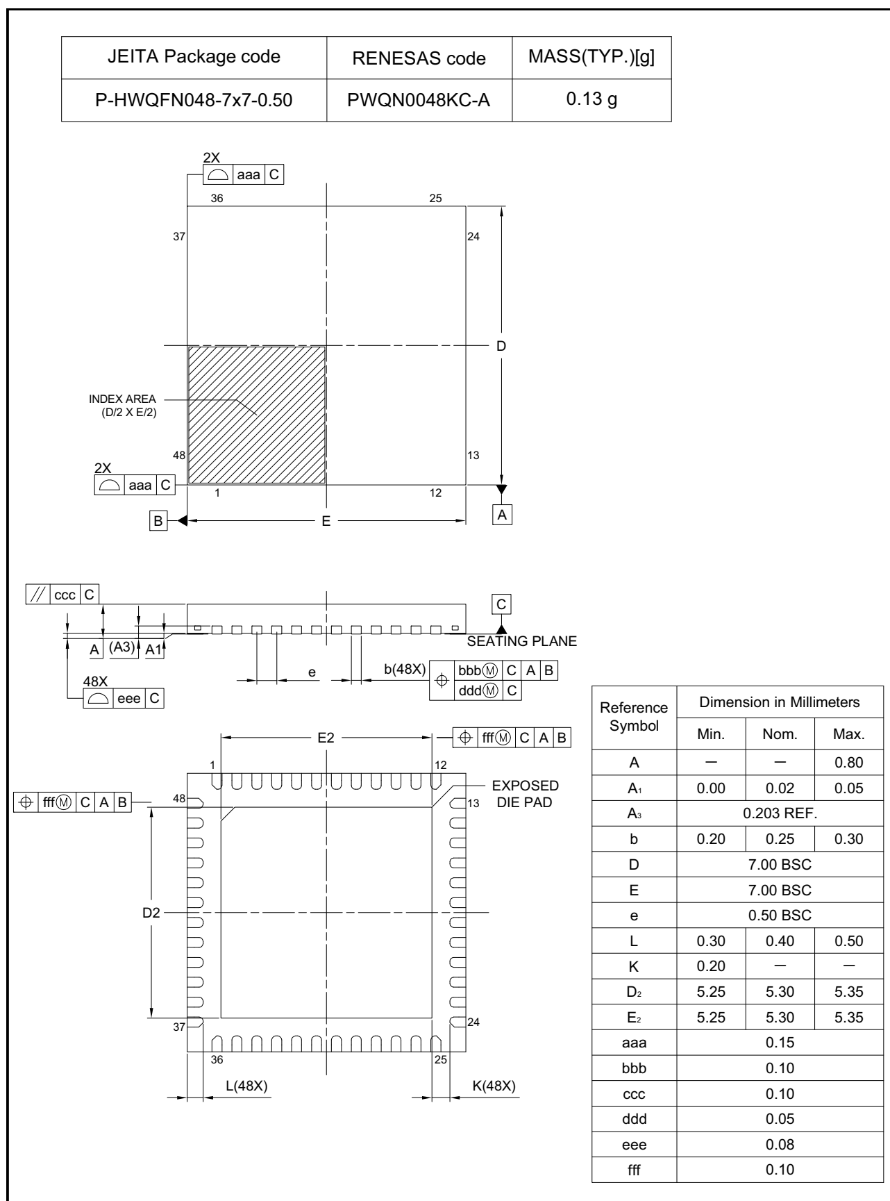
Figure 2.8 48-pin QFN (2)
