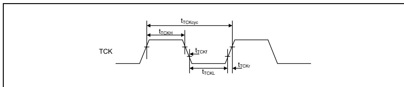
Figure 48.82 Boundary scan TCK timing
