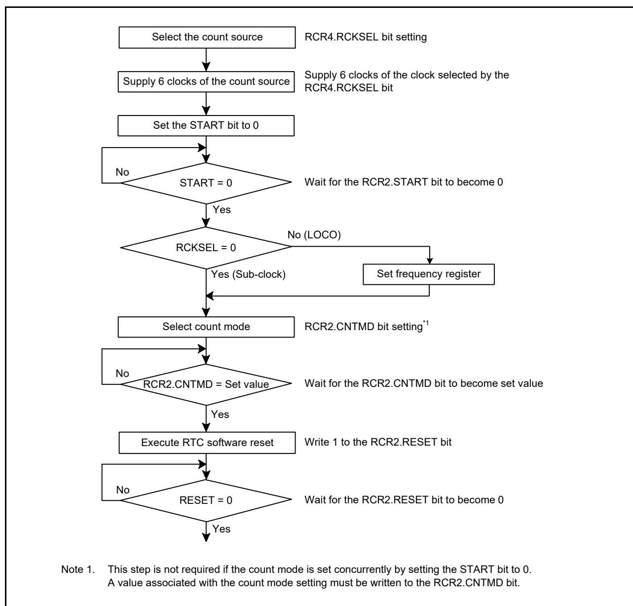
Figure 24.3 Clock and count mode setting procedure
