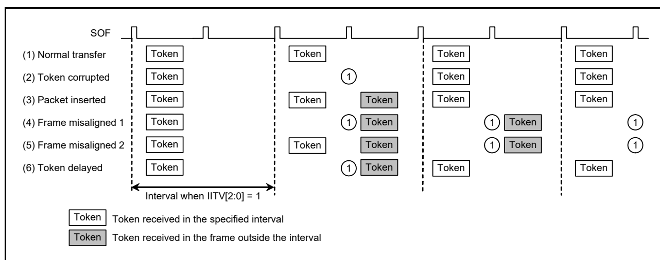
Figure 27.23 Example interval error occurrence when IITV[2:0] = 1
