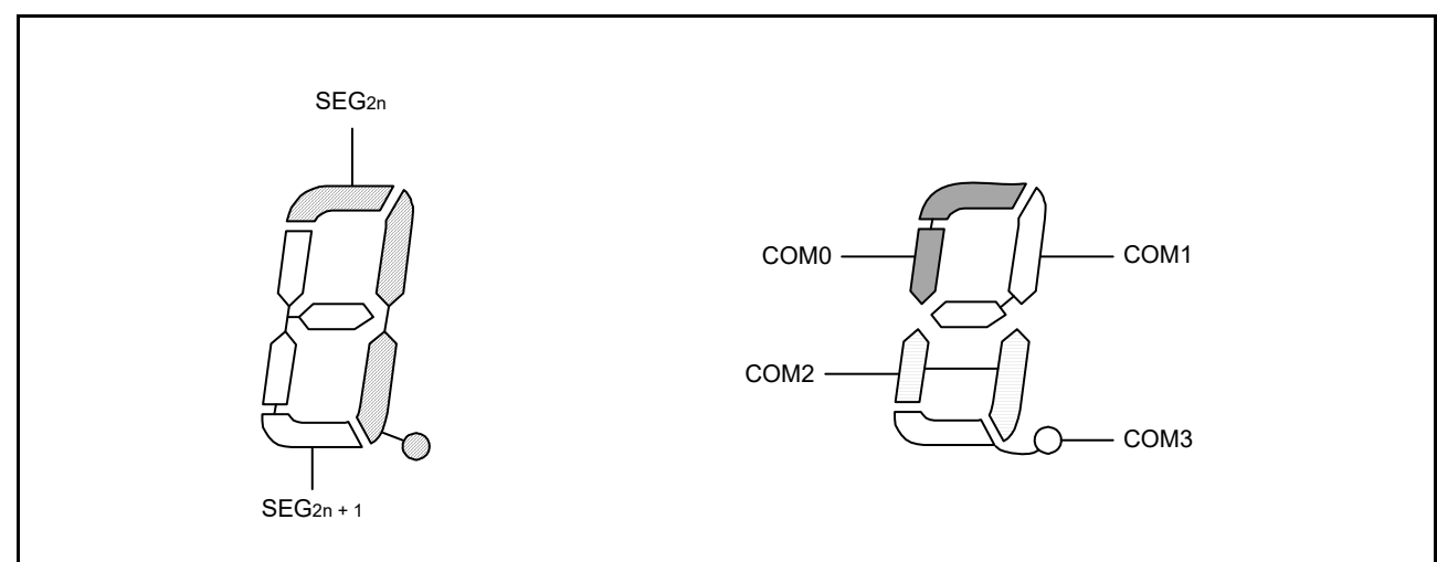
Figure 45.28 Four-time-slice LCD display pattern and electrode connections
