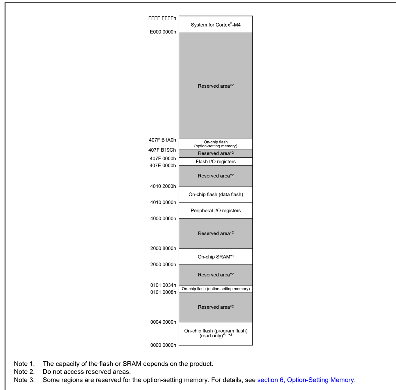
Figure 4.1 Memory map
