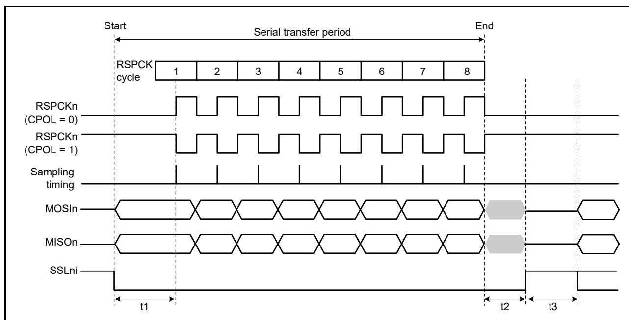
Figure 28.22 SPI transfer format when CPHA = 0
