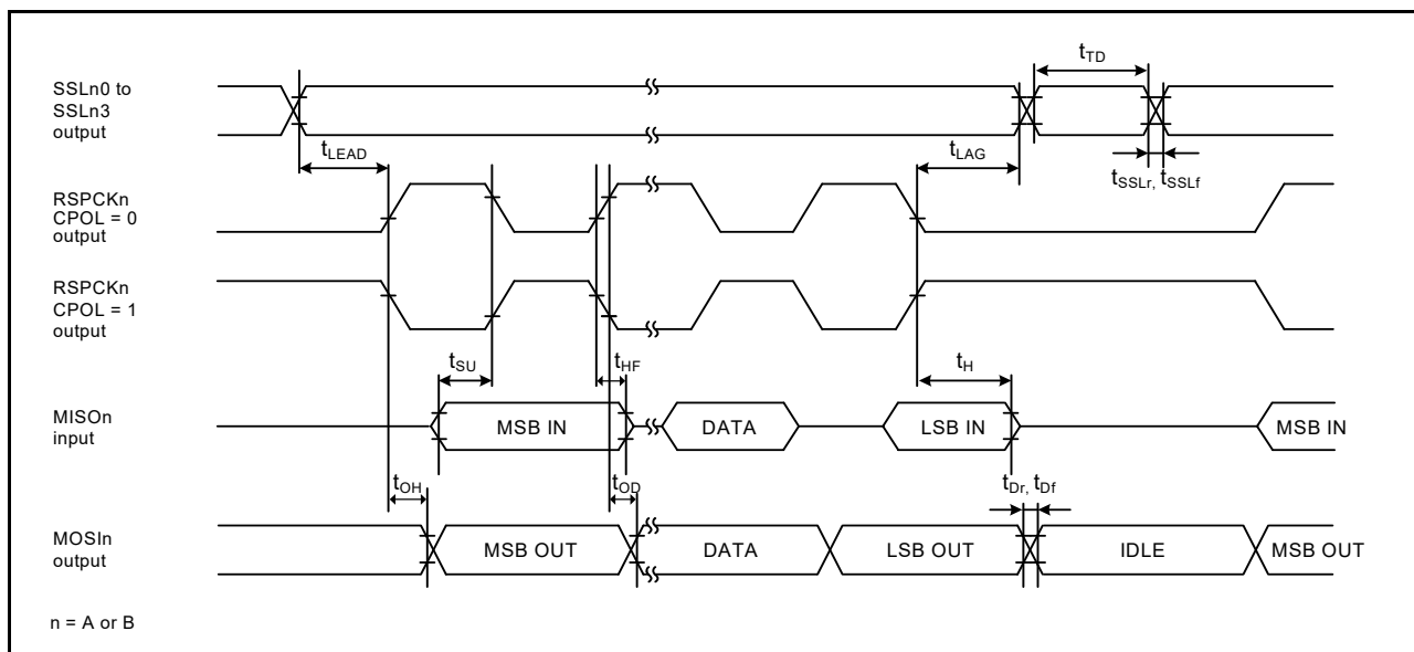
Figure 41.53 SPI timing (master, CPHA = 1) (bit rate: PCLKB division ratio is set to 1/2)
