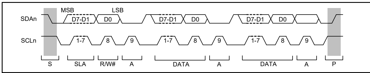
Figure 25.59 I²C bus timing when SLA is 7 bits
