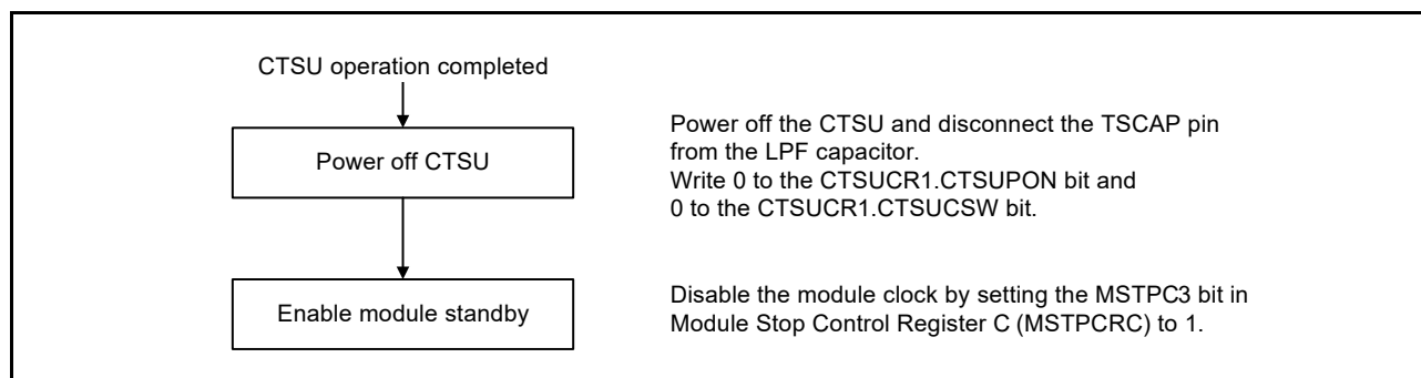
Figure 34.10 CTSU stopping flow
