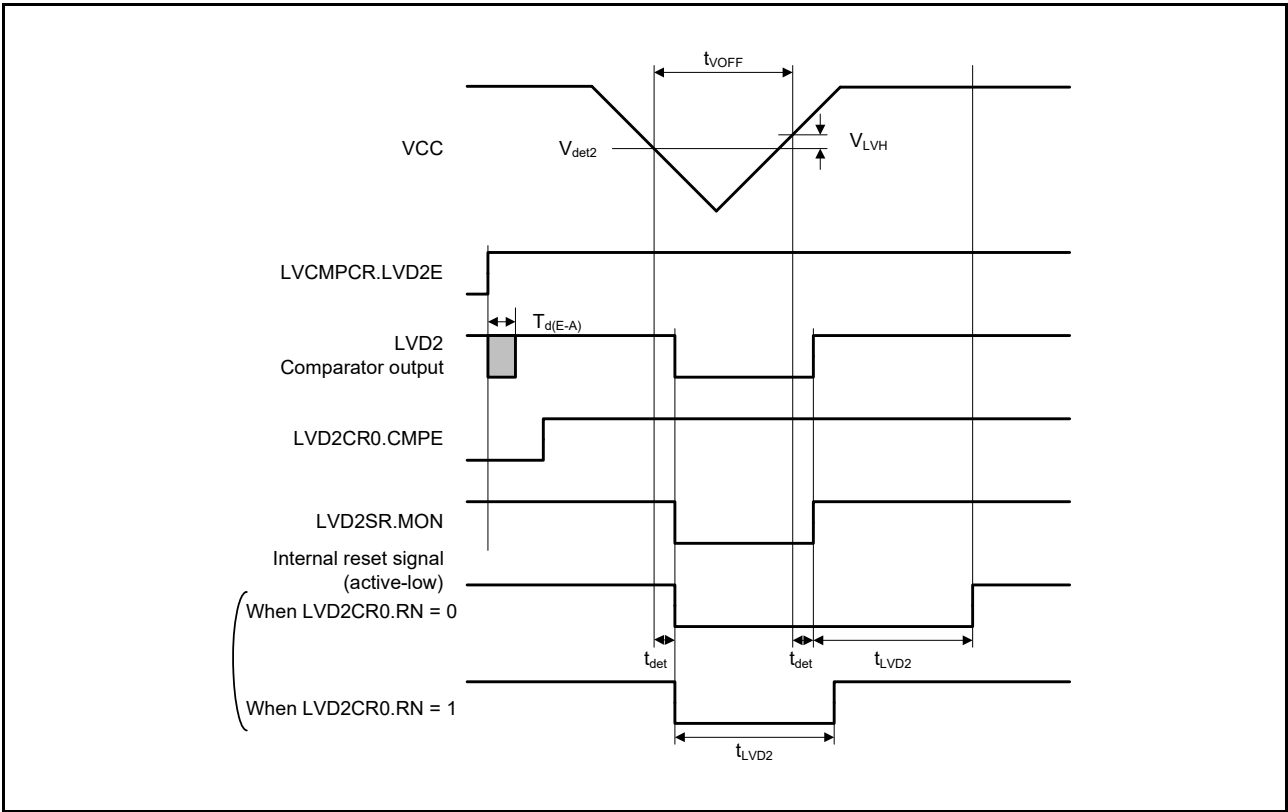
Figure 41.70 Voltage detection circuit timing ( V_{det2} )
