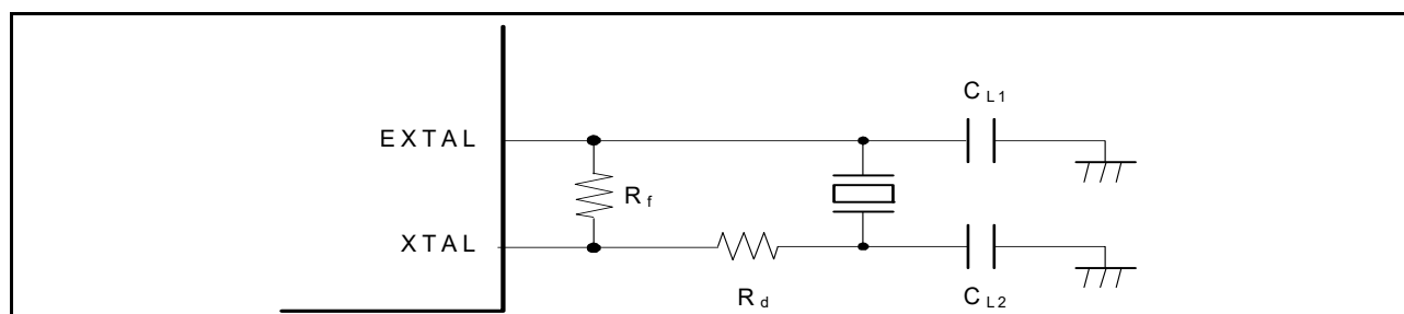
Figure 8.2 Example of crystal resonator connection
