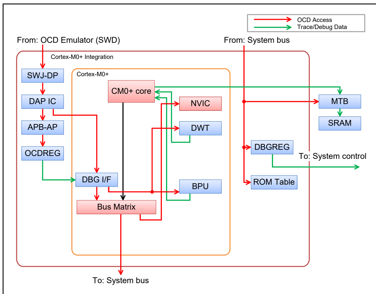
Figure 2.1 Cortex-M0+ block diagram
