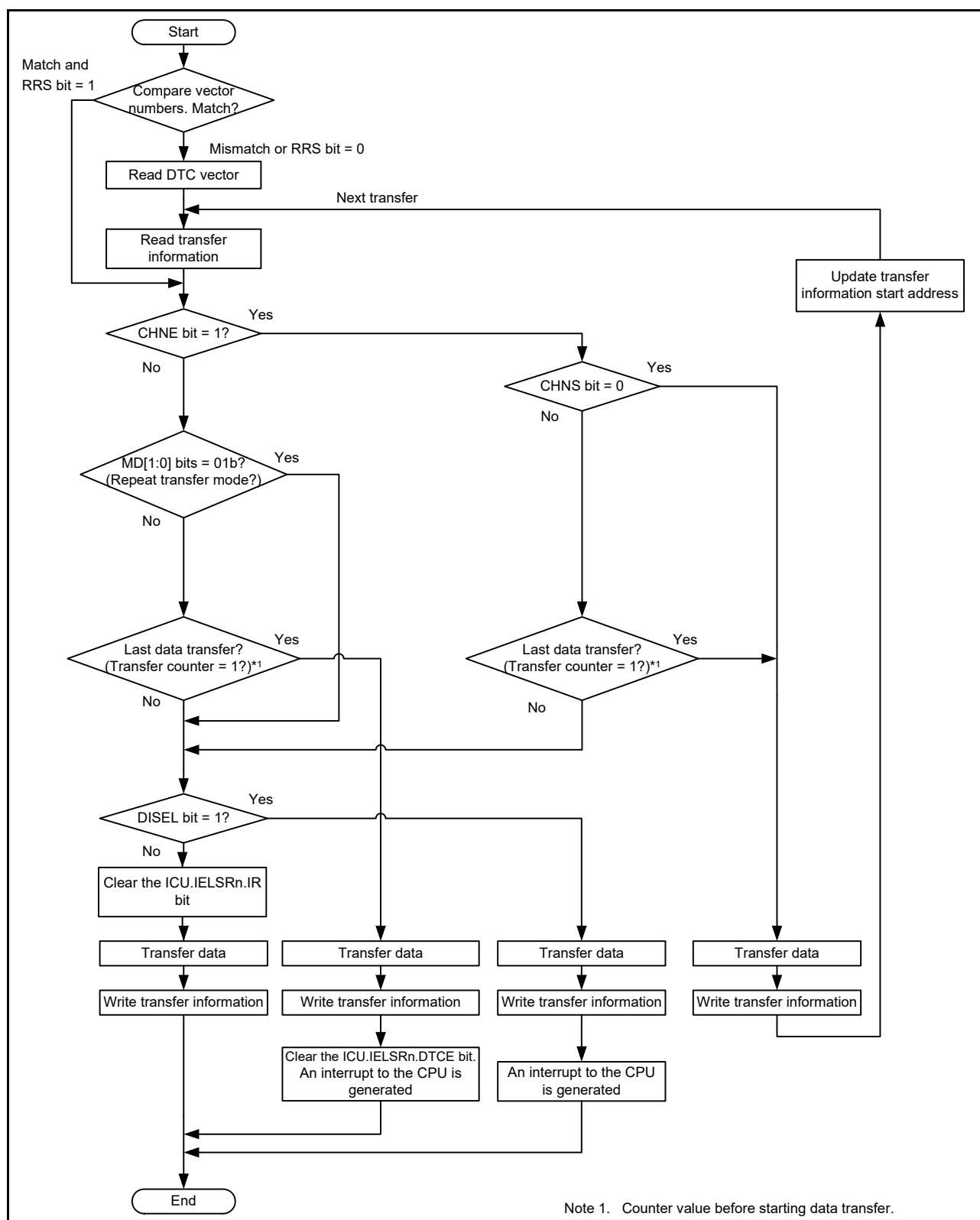
Figure 14.4 DTC operation flowchart
