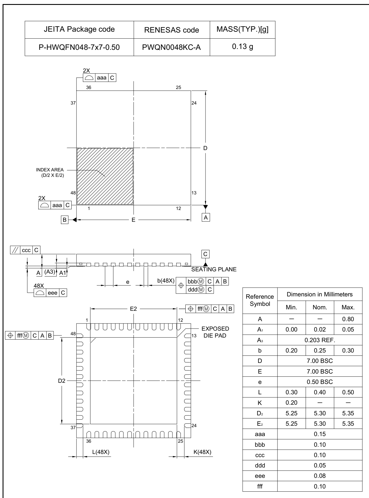
Figure 2.7 QFN 48-pin (2)
