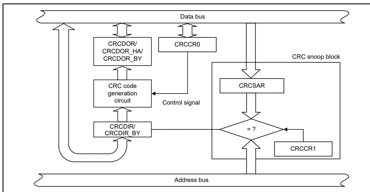
Figure 29.1 CRC calculator block diagram
