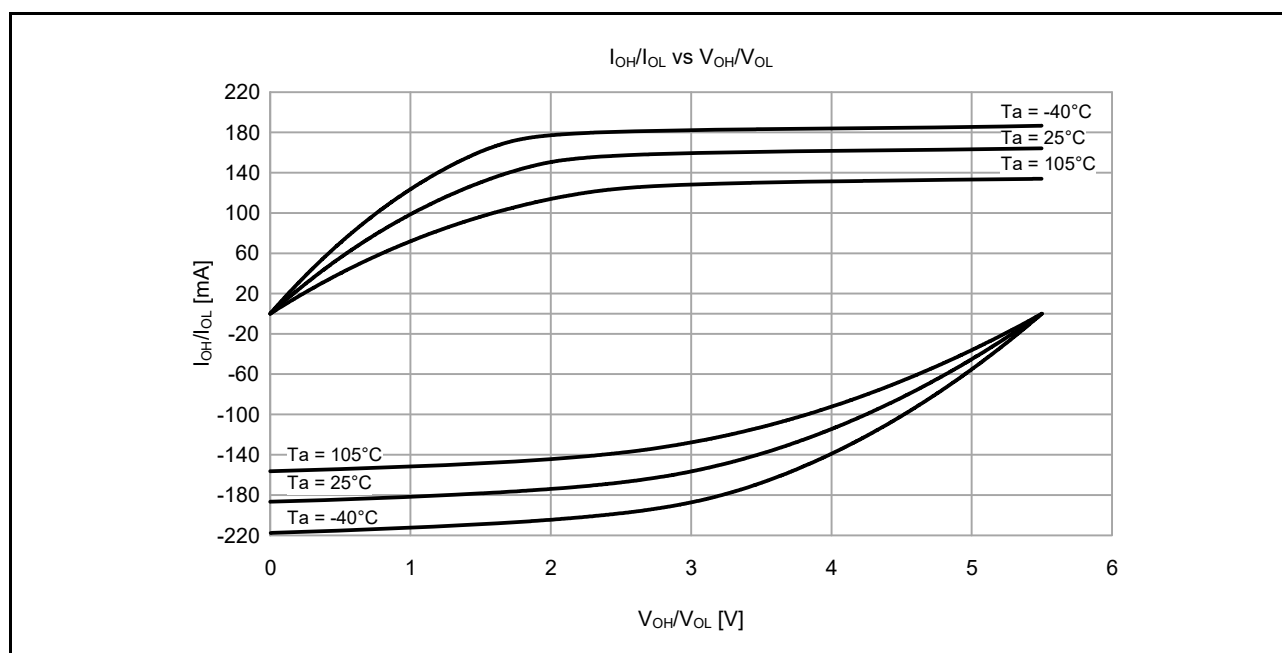
Figure 41.15 V_{OH}/V_{OL} and I_{OH}/I_{OL} temperature characteristics at V_{CC} = 5.5 V when middle drive output is selected (reference data)
