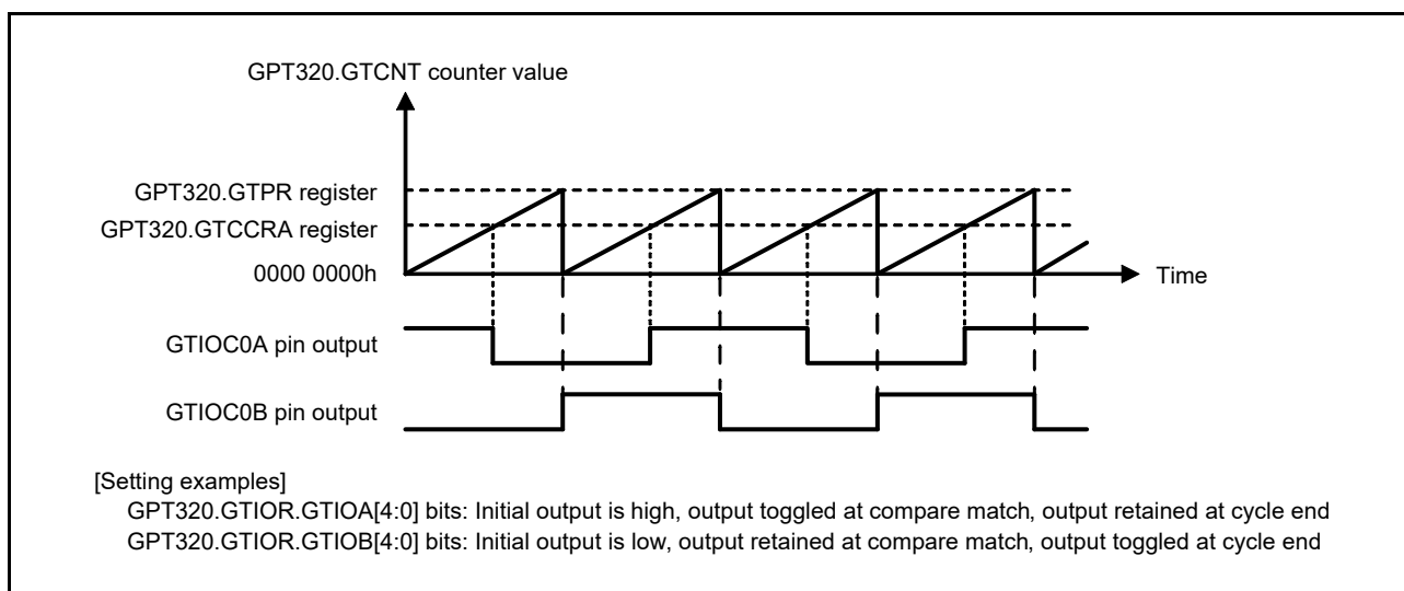
Figure 19.14 Example of toggled output operation (2)
