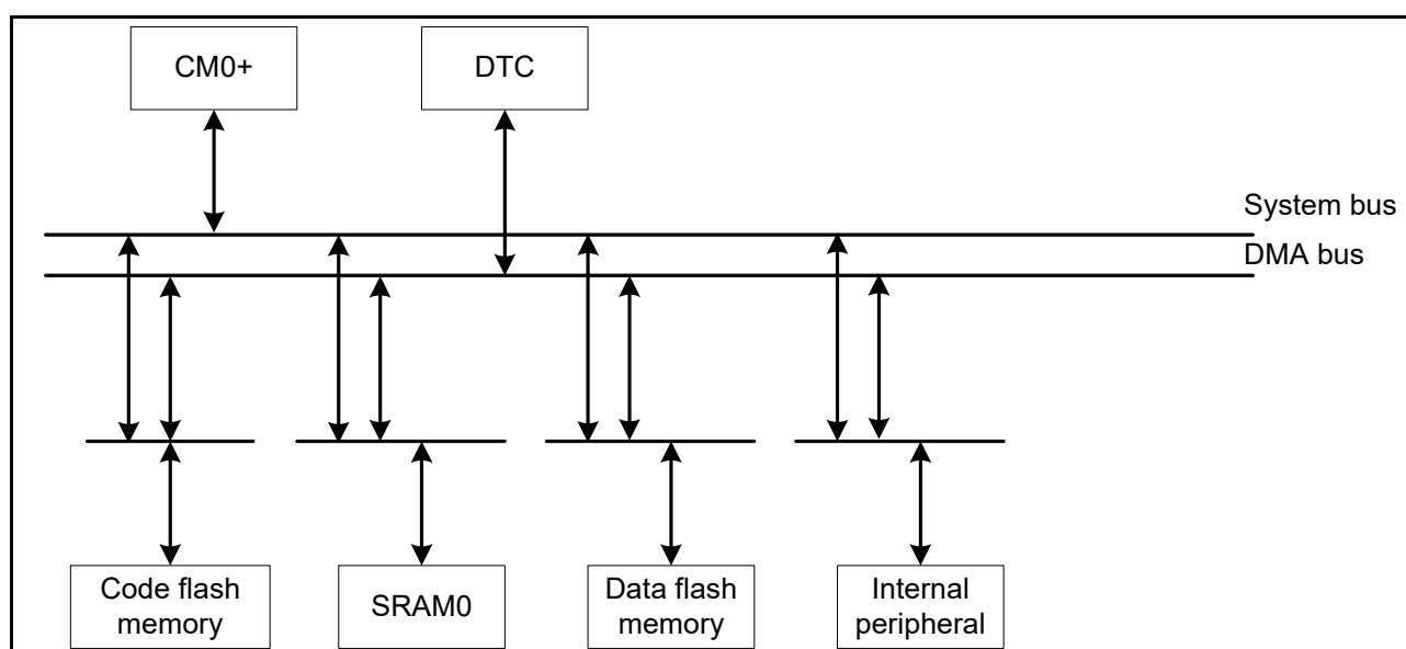
Figure 13.1 Bus configuration
