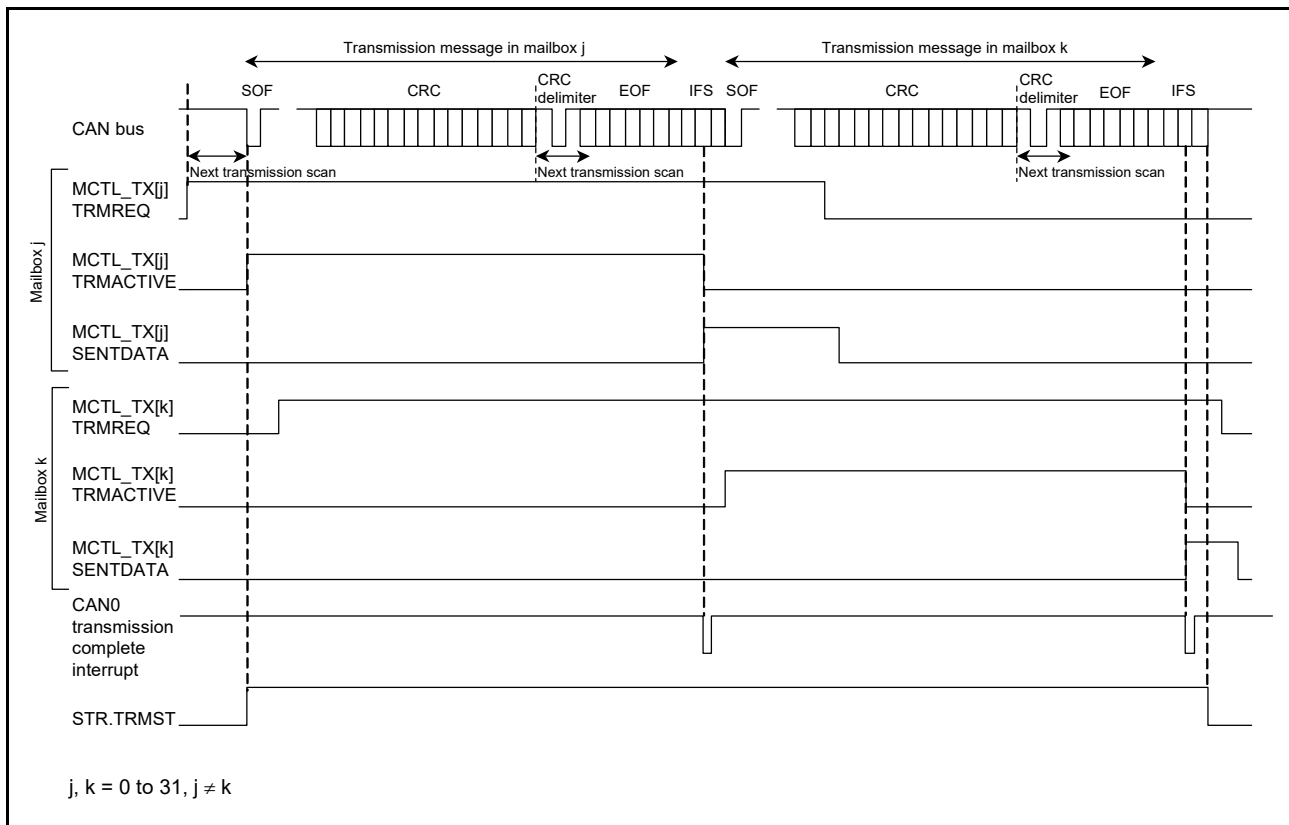
Figure 27.20 Operation example of data frame transmission
