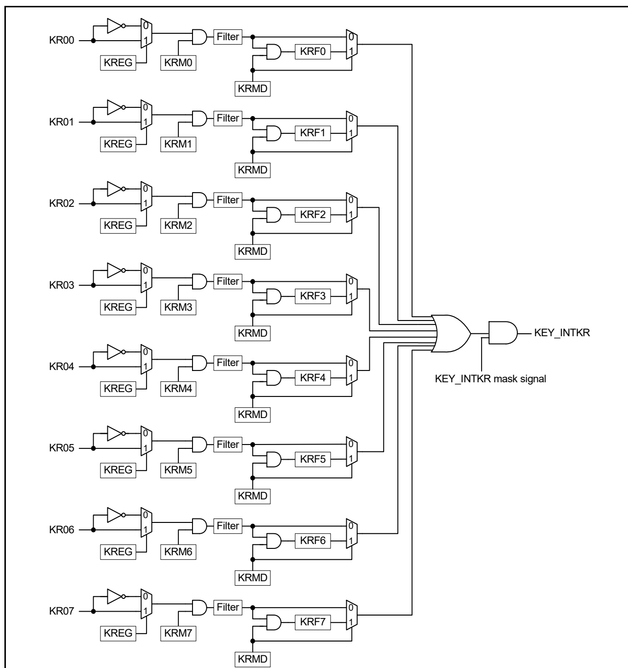
Figure 17.1 Key interrupt function block diagram
