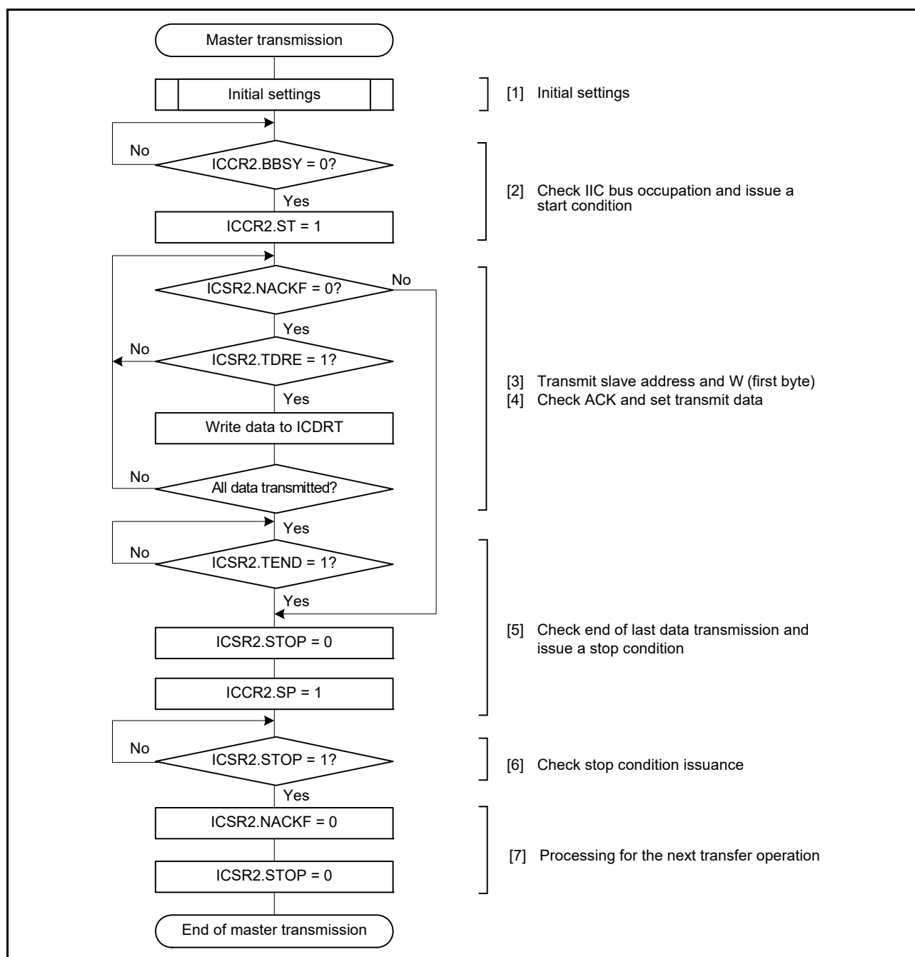
Figure 26.6 Example master transmission flow
