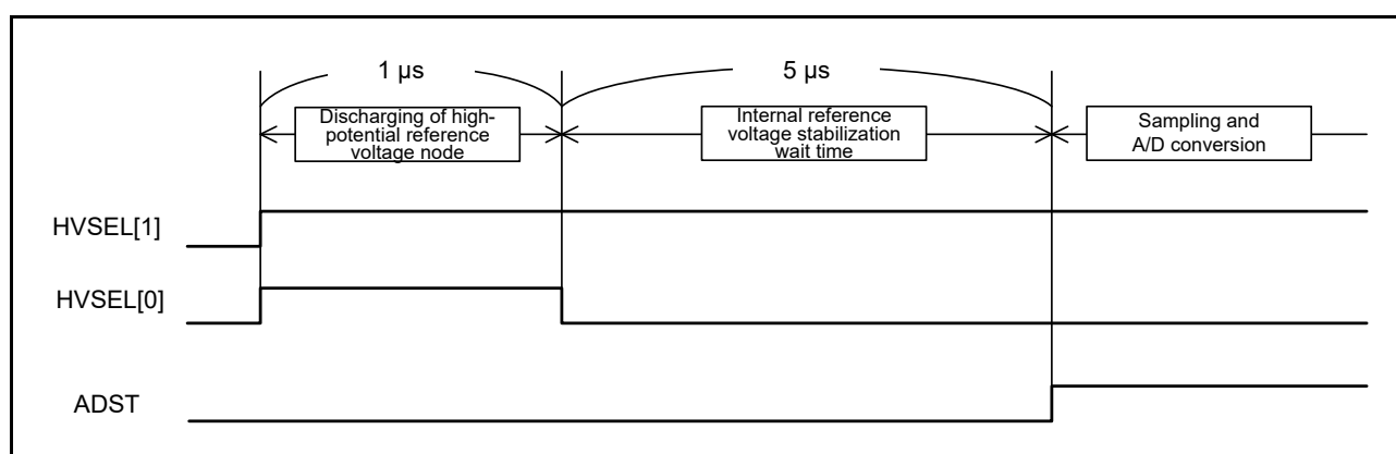
Figure 30.30 Procedure to select internal reference voltage as high-potential reference voltage
