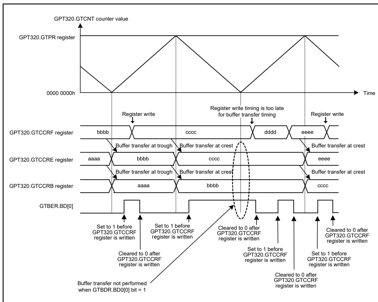
Figure 19.83 Example of operation for disabling buffer operation with triangle waves, double buffer operation, and buffer transfer at both troughs and crests
