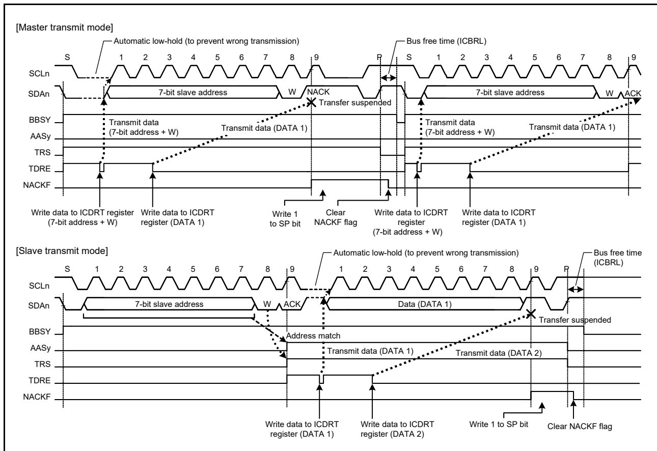
Figure 26.39 Suspension of data transfer when NACK is received (NACK = 1)
