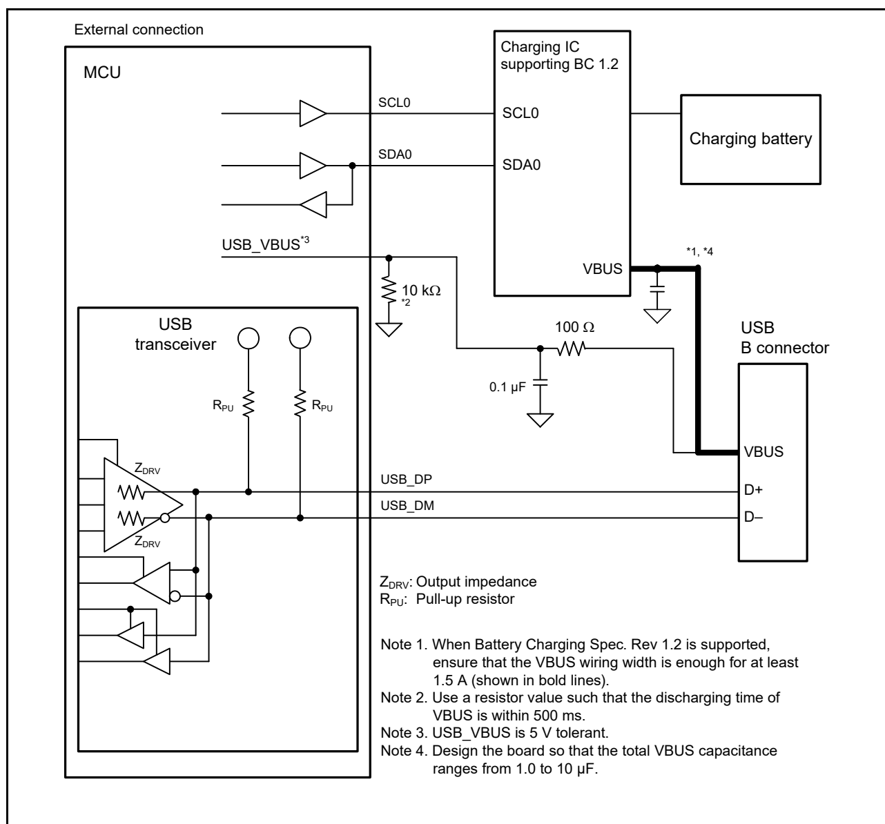
Figure 24.8 Example of functional connection with Battery Charging Rev 1.2 supported
