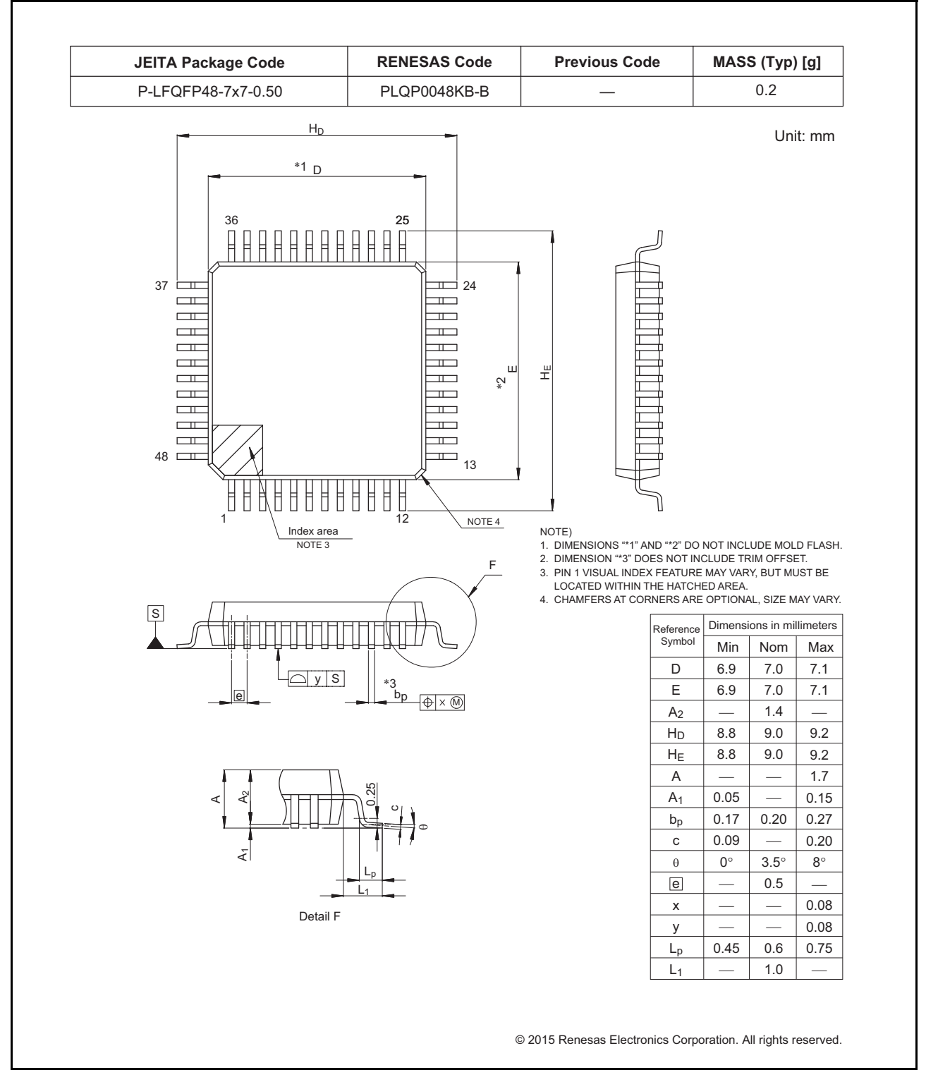
Figure 2.2 LQFP 48-pin
