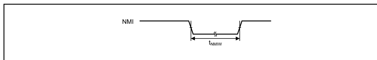
Figure 41.33 NMI interrupt input timing
