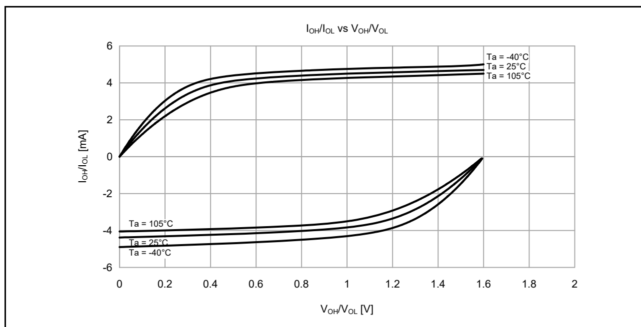
Figure 41.8 V_{OH}/V_{OL} and I_{OH}/I_{OL} temperature characteristics at V_{CC} = 1.6 V when middle drive output is selected (reference data)
