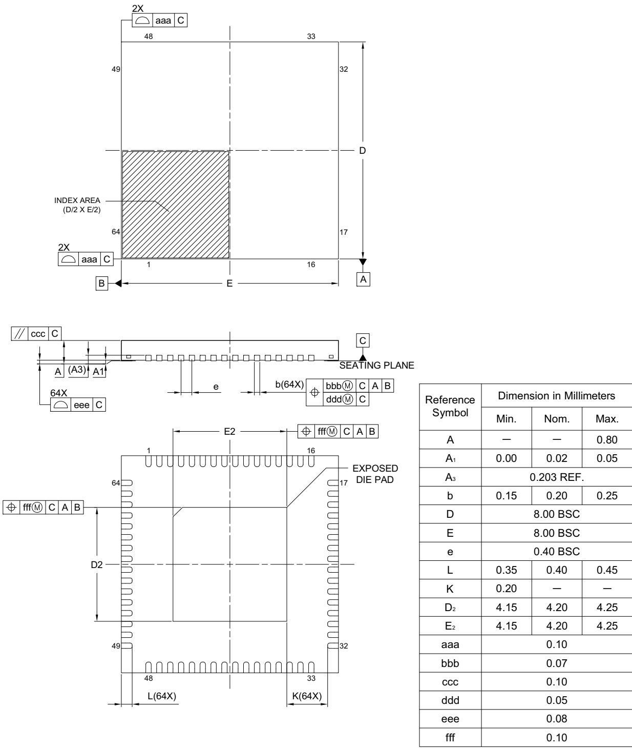
Figure 2.5 QFN 64-pin (2)
