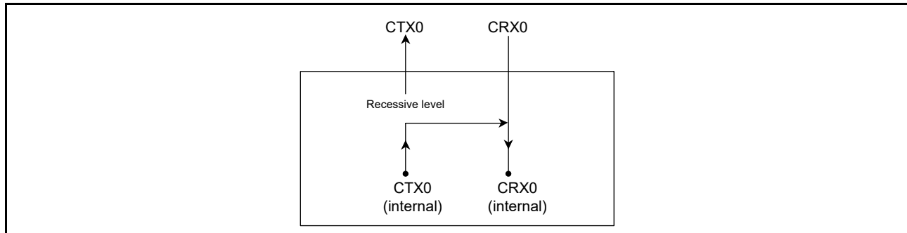
Figure 27.6 Connection when listen-only mode is selected
