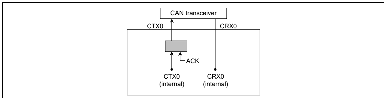
Figure 27.7 Connection when self-test mode 0 is selected
