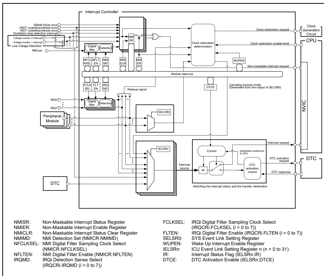
Figure 12.1 Interrupt Controller Unit block diagram
