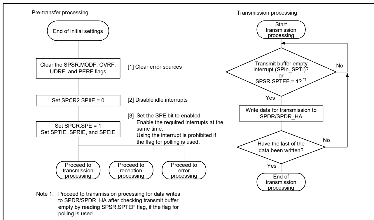
Figure 28.37 Transmission flow in slave mode
