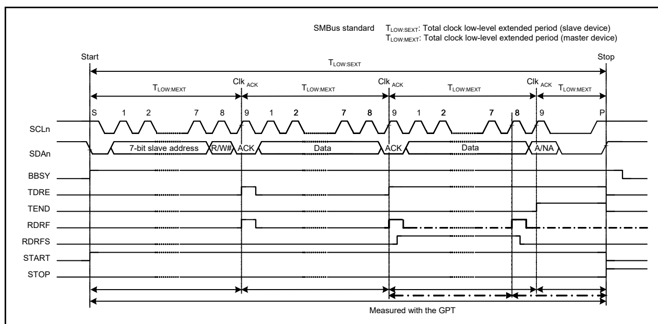
Figure 26.50 SMBus timeout measurement
