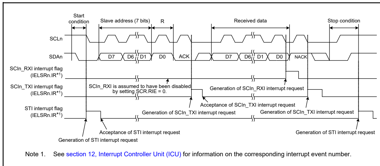
Figure 25.67 Example operation for master reception in simple IIC bus mode with 7-bit slave addresses, transmission interrupts, and reception interrupts
