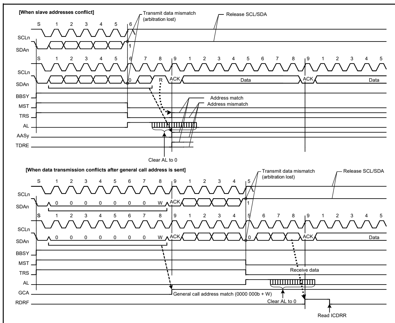
Figure 26.41 Examples of master arbitration-lost detection (MALE = 1)
