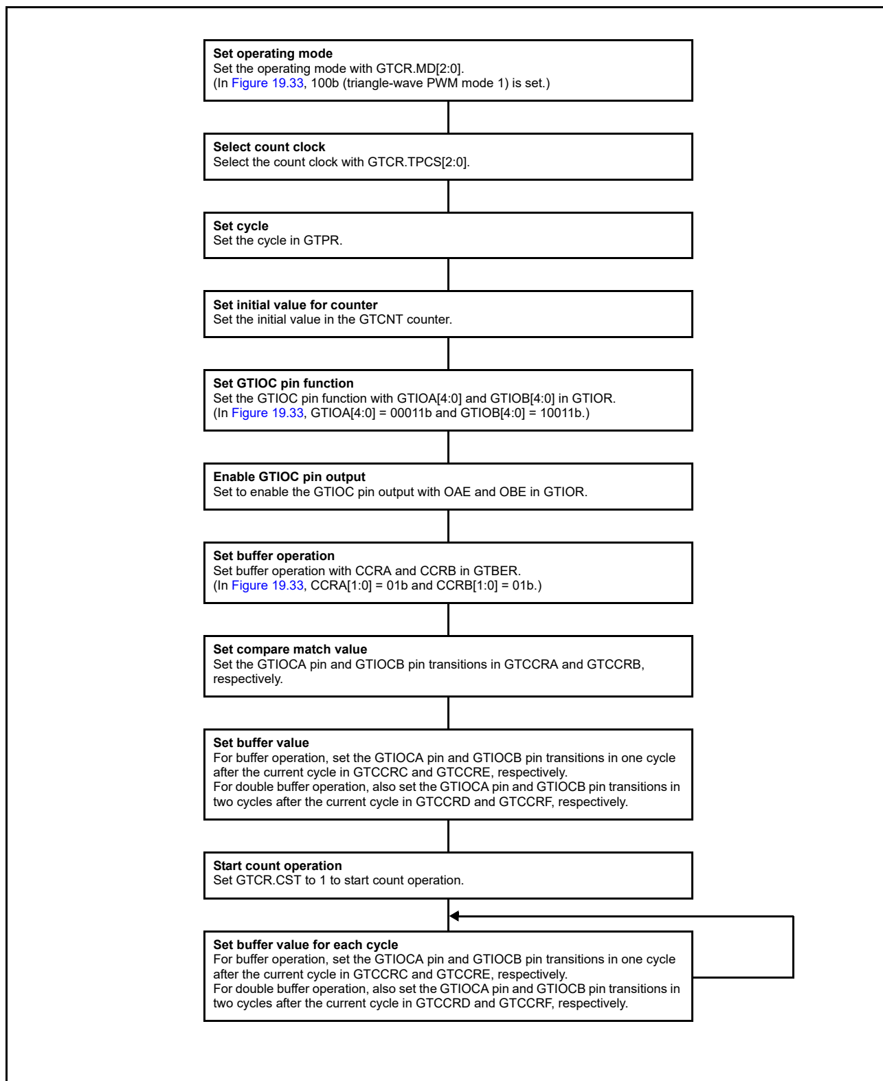
Figure 19.34 Example for setting triangle-wave PWM mode 1
