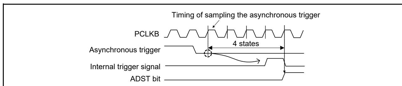
Figure 30.29 Asynchronous trigger input timing
