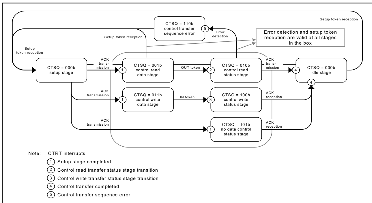
Figure 24.14 Control transfer stage transitions
