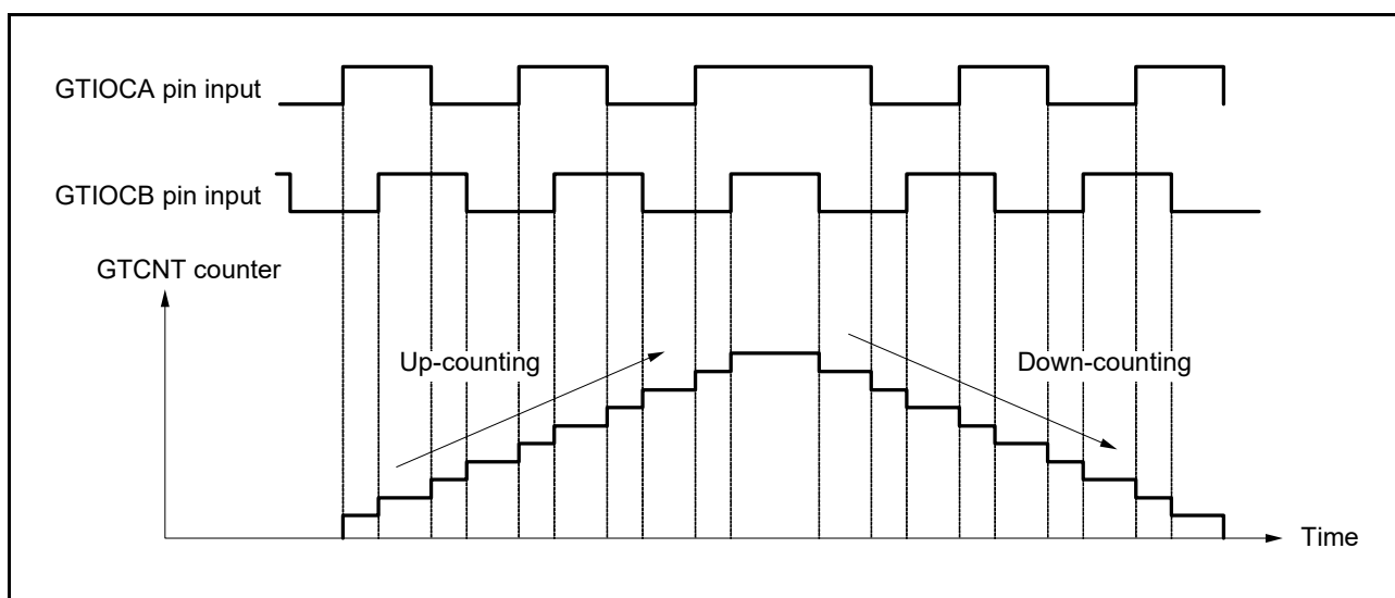
Figure 19.67 Example of phase counting mode 1
