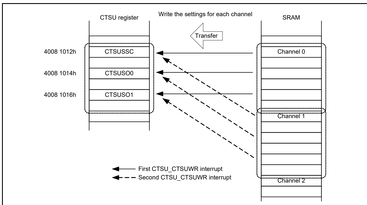
Figure 34.19 Example DTC transfer operation using the CTSU_CTSUWR interrupt
