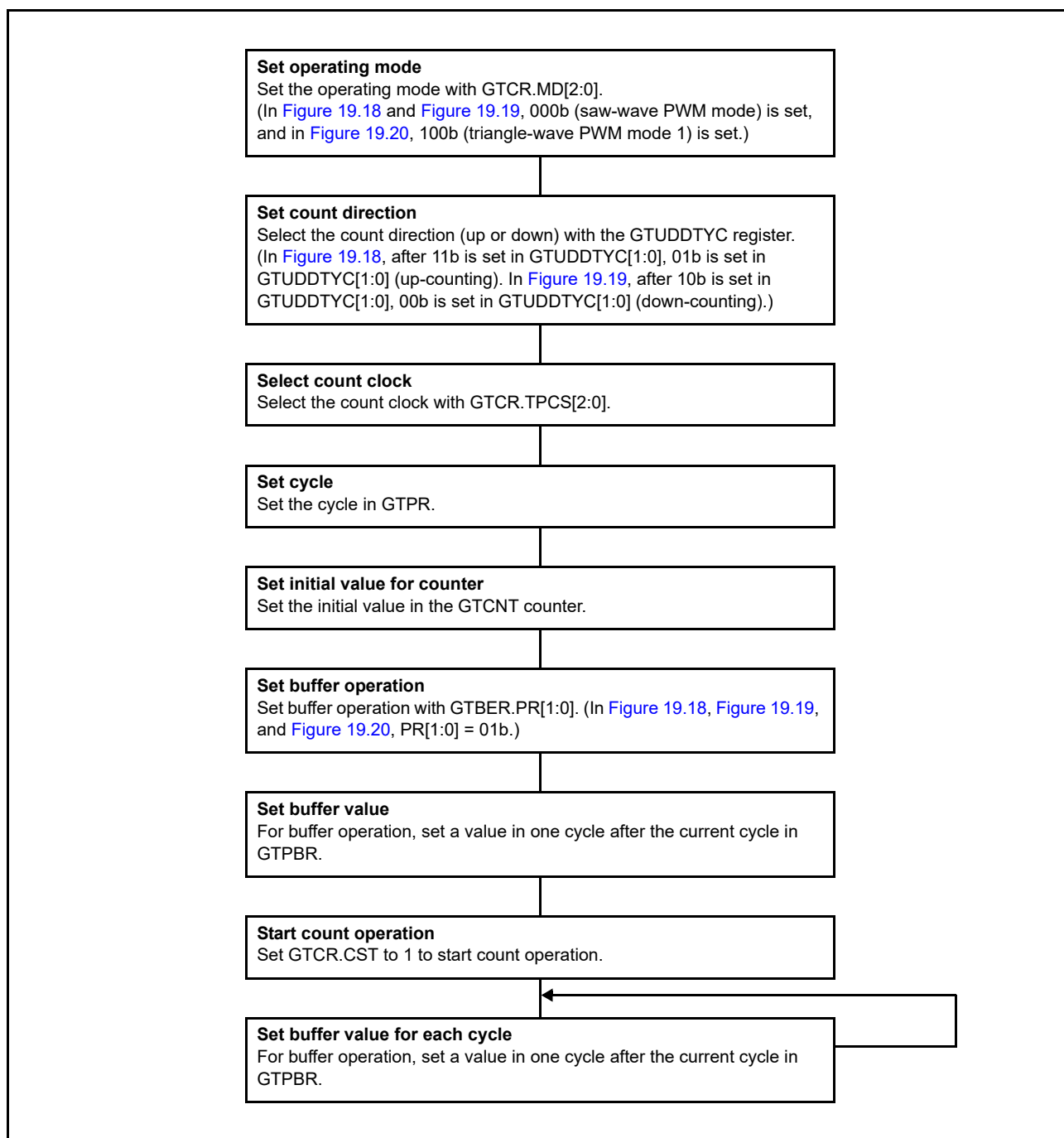
Figure 19.21 Example for setting GTPR buffer operation
