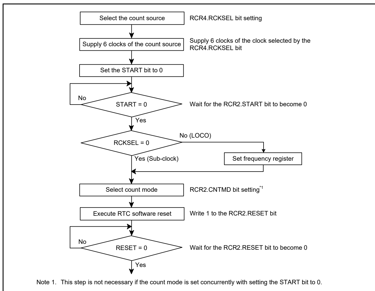
Figure 21.3 Clock and count mode setting procedure
