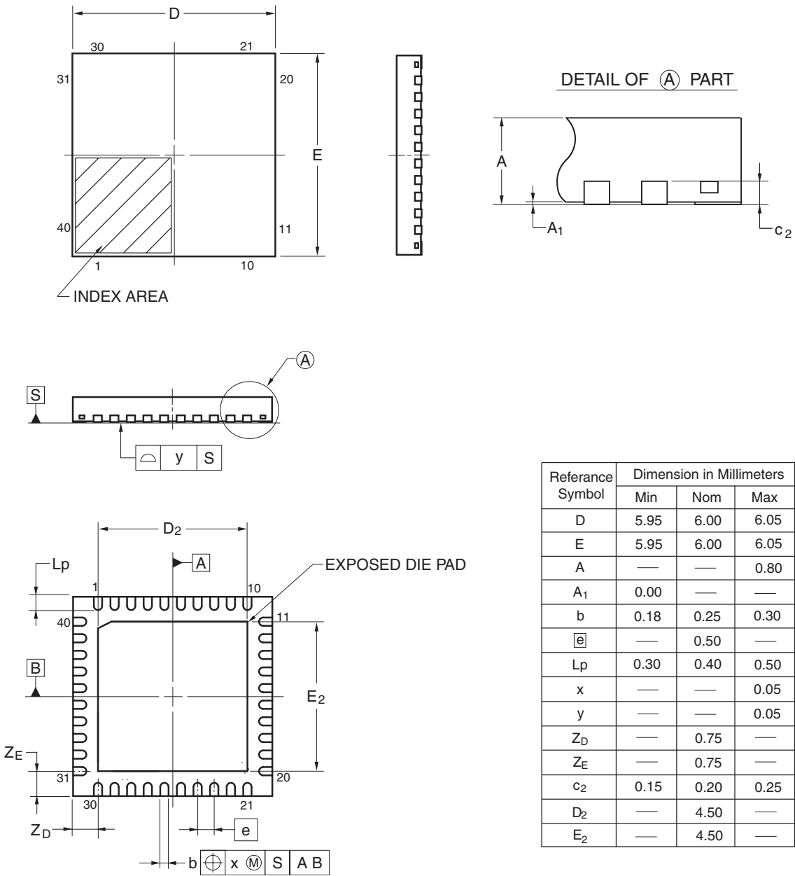
Figure 2.8 QFN 40-pin (1)
