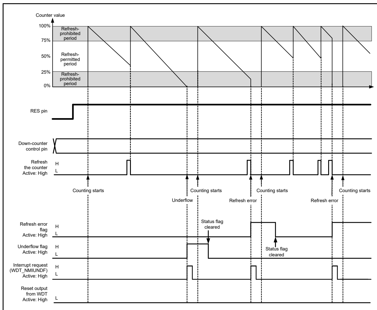
Figure 22.4 Operation example in auto start mode
