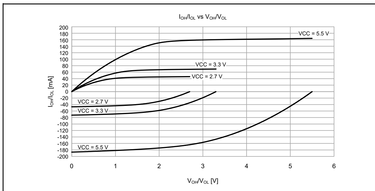
Figure 41.12 V_{OH}/V_{OL} and I_{OH}/I_{OL} voltage characteristics at T_a = 25^\circ\text{C} when middle drive output is selected (reference data)
