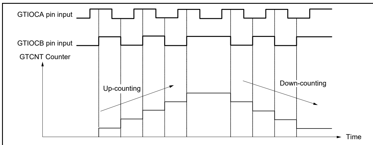
Figure 19.74 Example of phase counting mode 4
