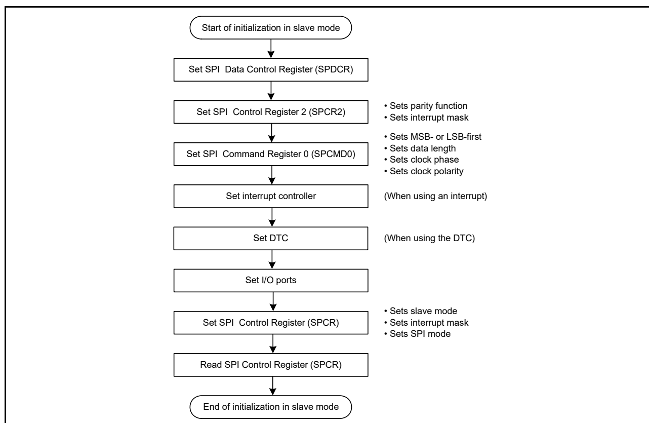
Figure 28.41 Example of initialization flow in slave mode for clock synchronous operation
