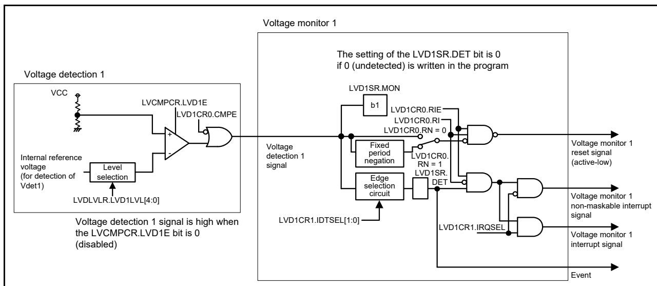
Figure 7.2 Voltage monitor 1 interrupt/reset circuit block diagram
