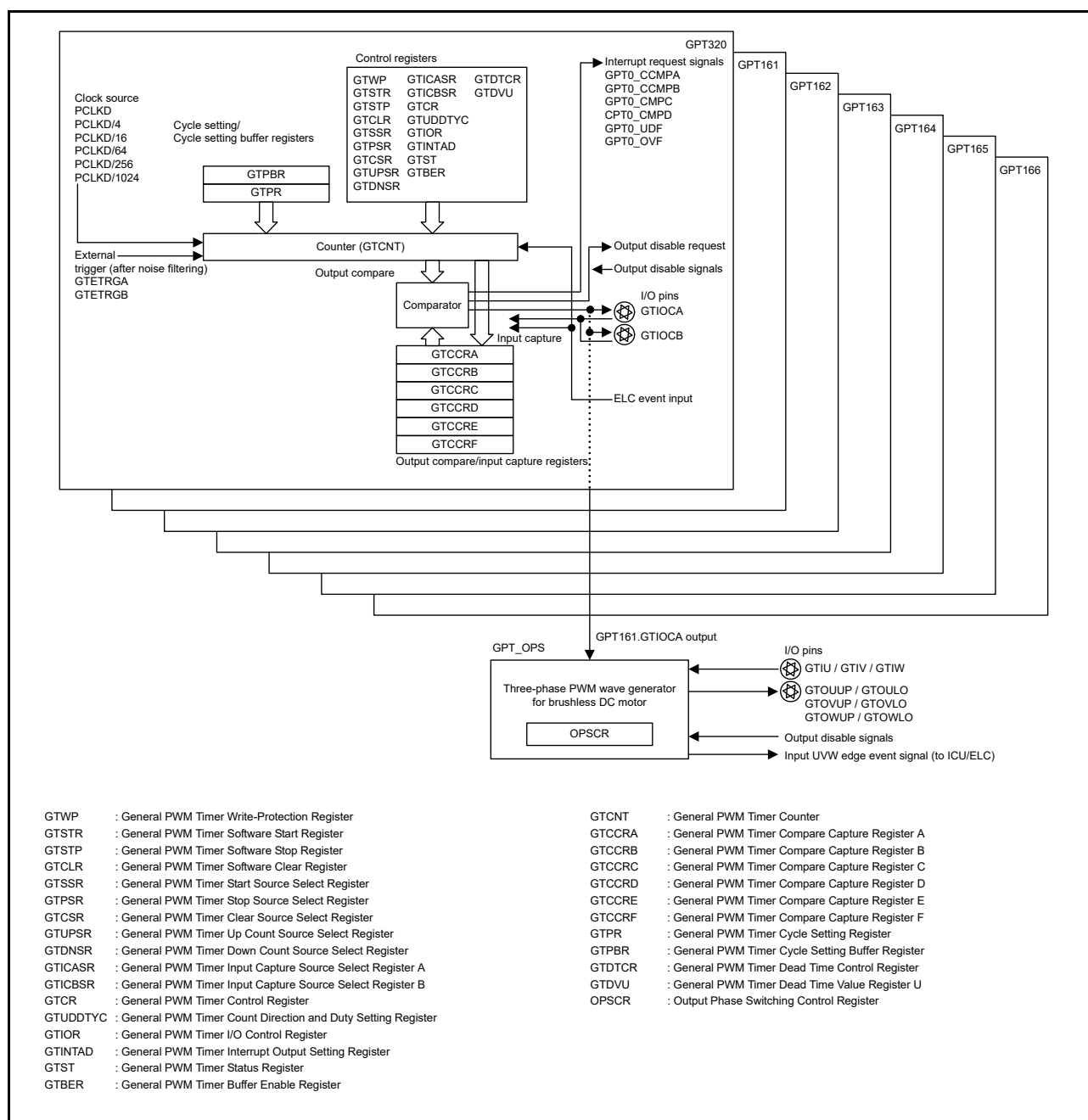
Figure 19.1 GPT block diagram
