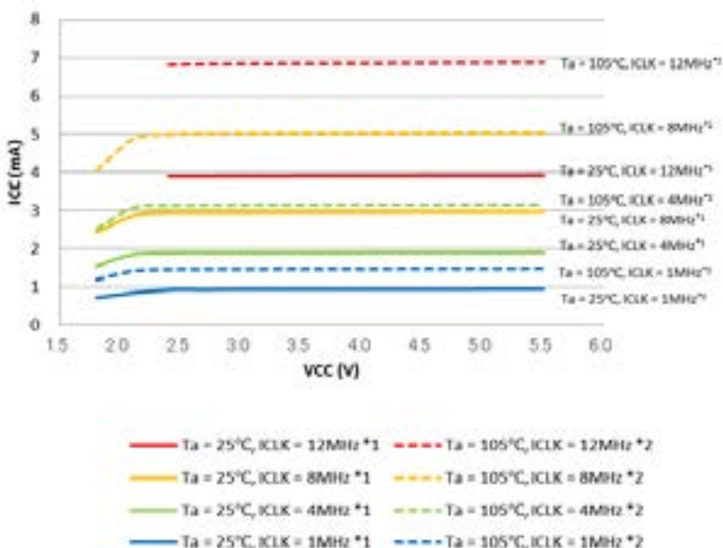
Figure 41.17 Voltage dependency in high-speed operating mode (reference data)
