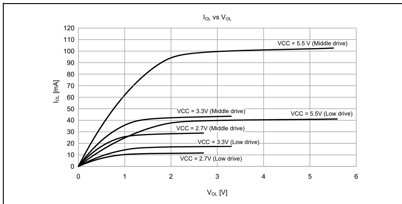
Figure 41.16 V_{OH}/V_{OL} and I_{OH}/I_{OL} voltage characteristics at T_a = 25^\circ\text{C}
