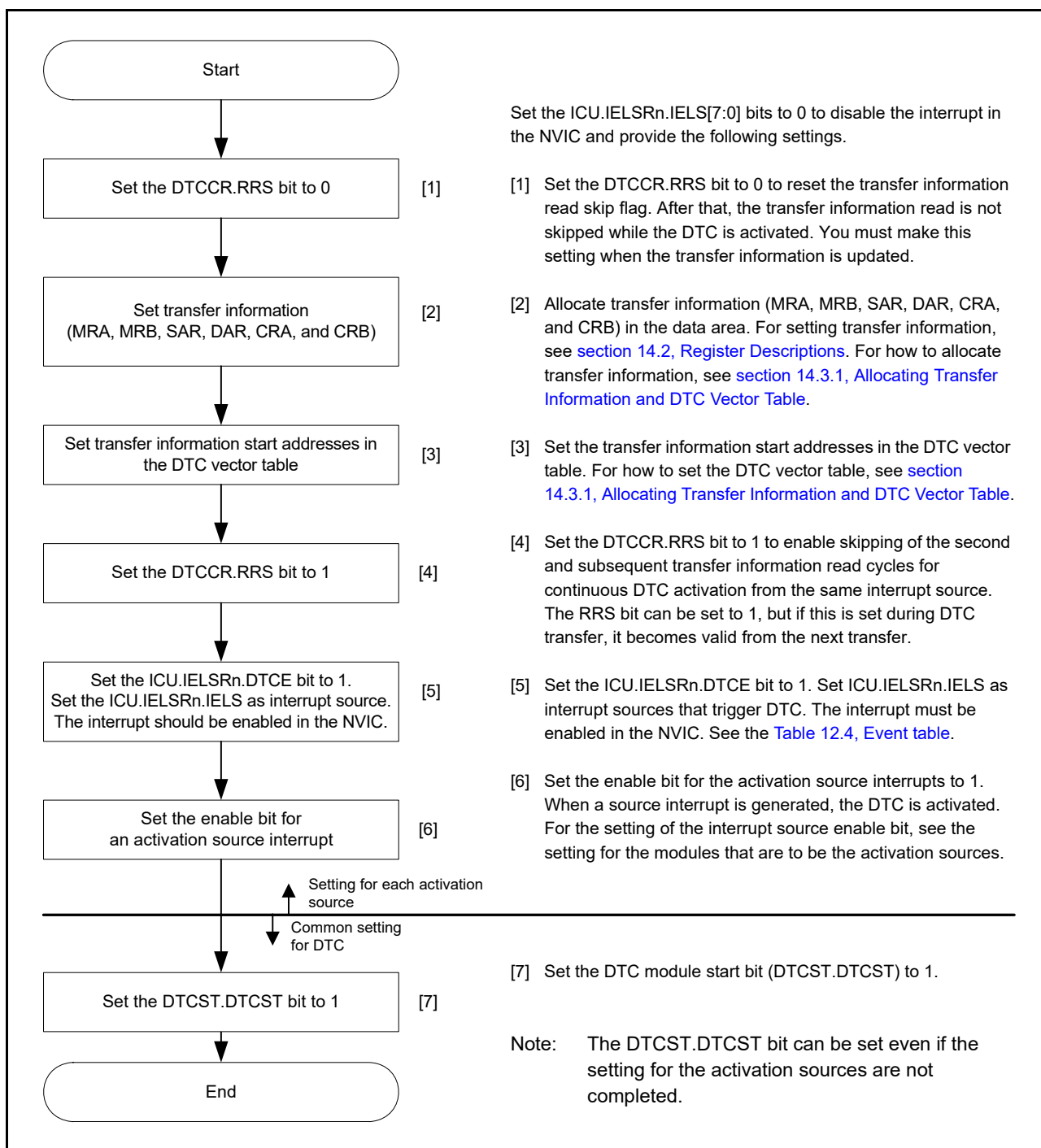
Figure 14.13 DTC setting procedure
