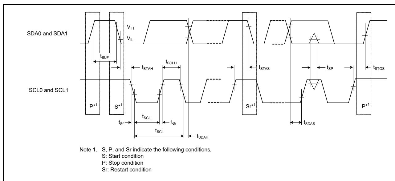
Figure 41.56 I 2 C bus interface input/output timing
