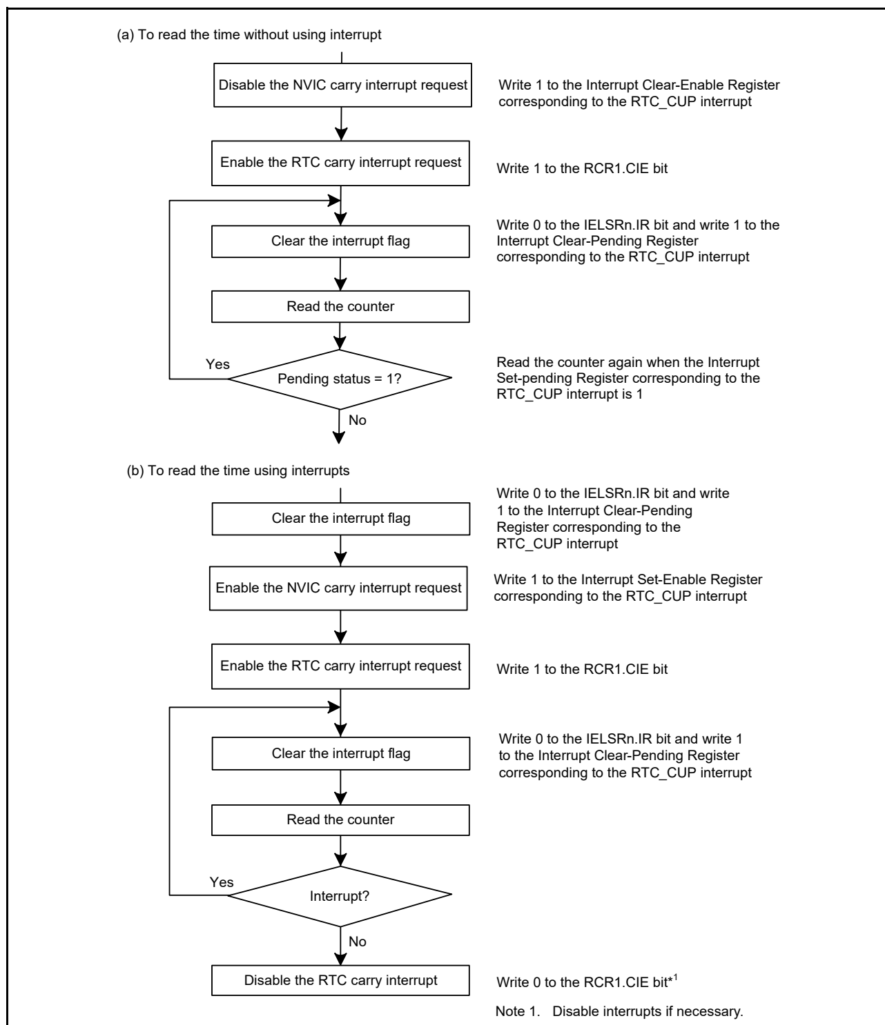
Figure 21.6 Reading time
