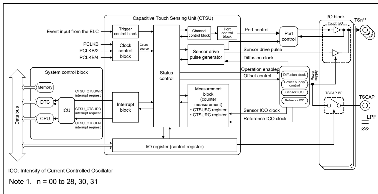
Figure 34.3 CTSU block diagram
