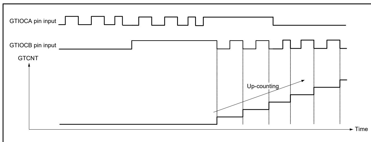
Figure 19.76 Example of phase counting mode 5 (B)
