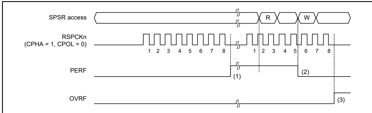
Figure 28.31 Operation example of PERF flag
