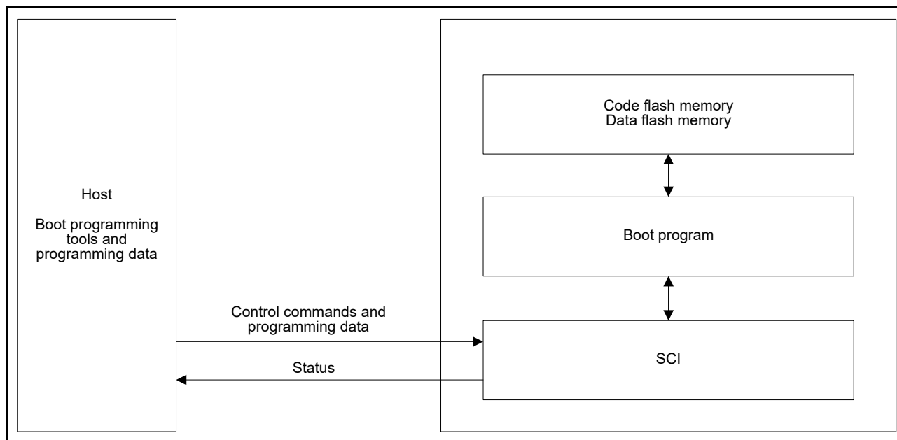
Figure 37.8 System configuration in SCI boot mode
