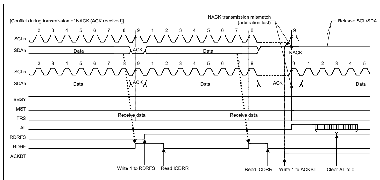
Figure 26.43 Example of arbitration-loss detection during transmission of NACK (NALE = 1)
