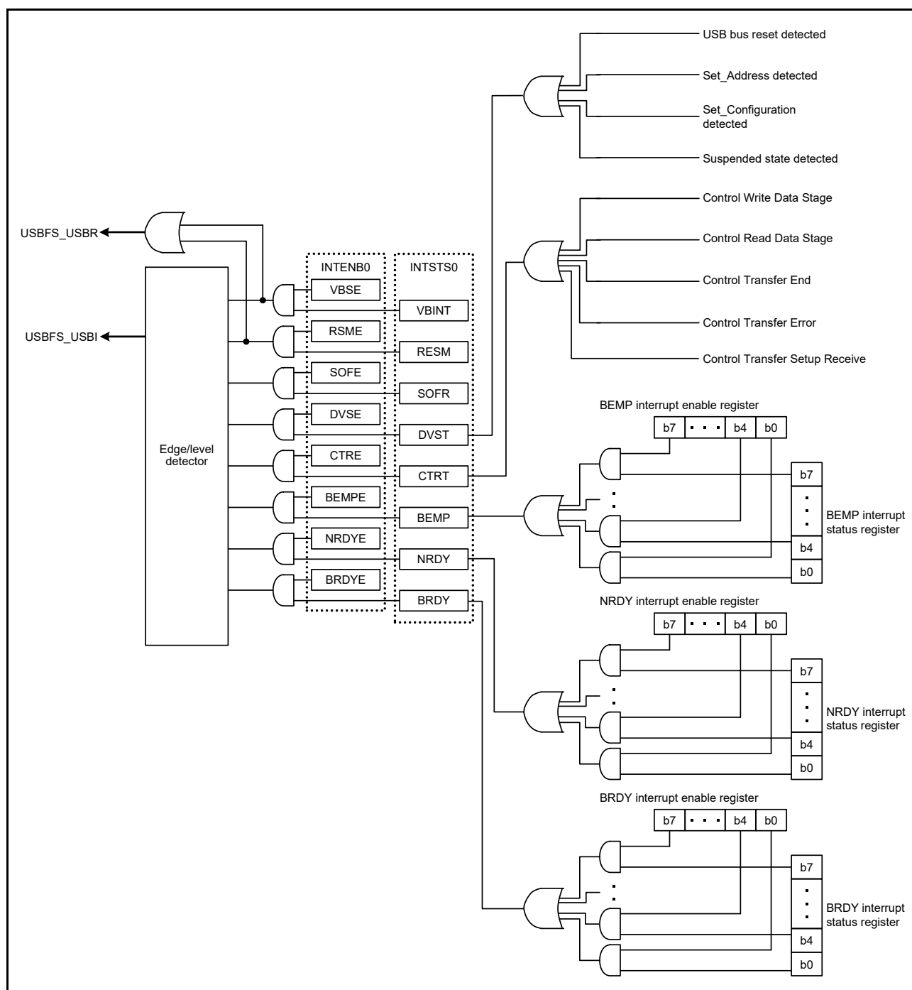
Figure 24.9 Circuits related to interrupts in USBFS
