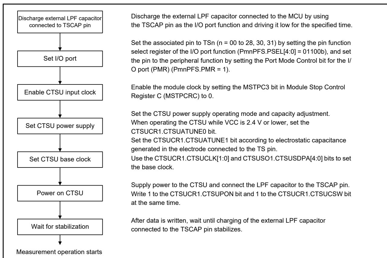
Figure 34.9 Initial CTSU settings flow
