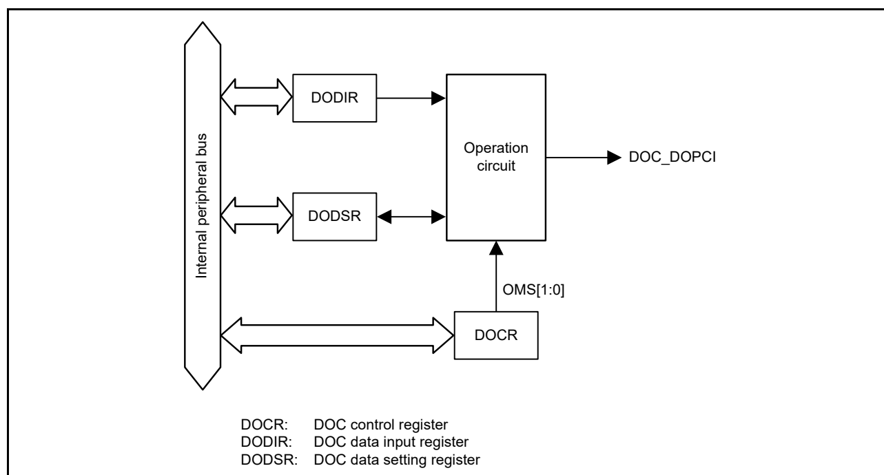
Figure 35.1 DOC block diagram
