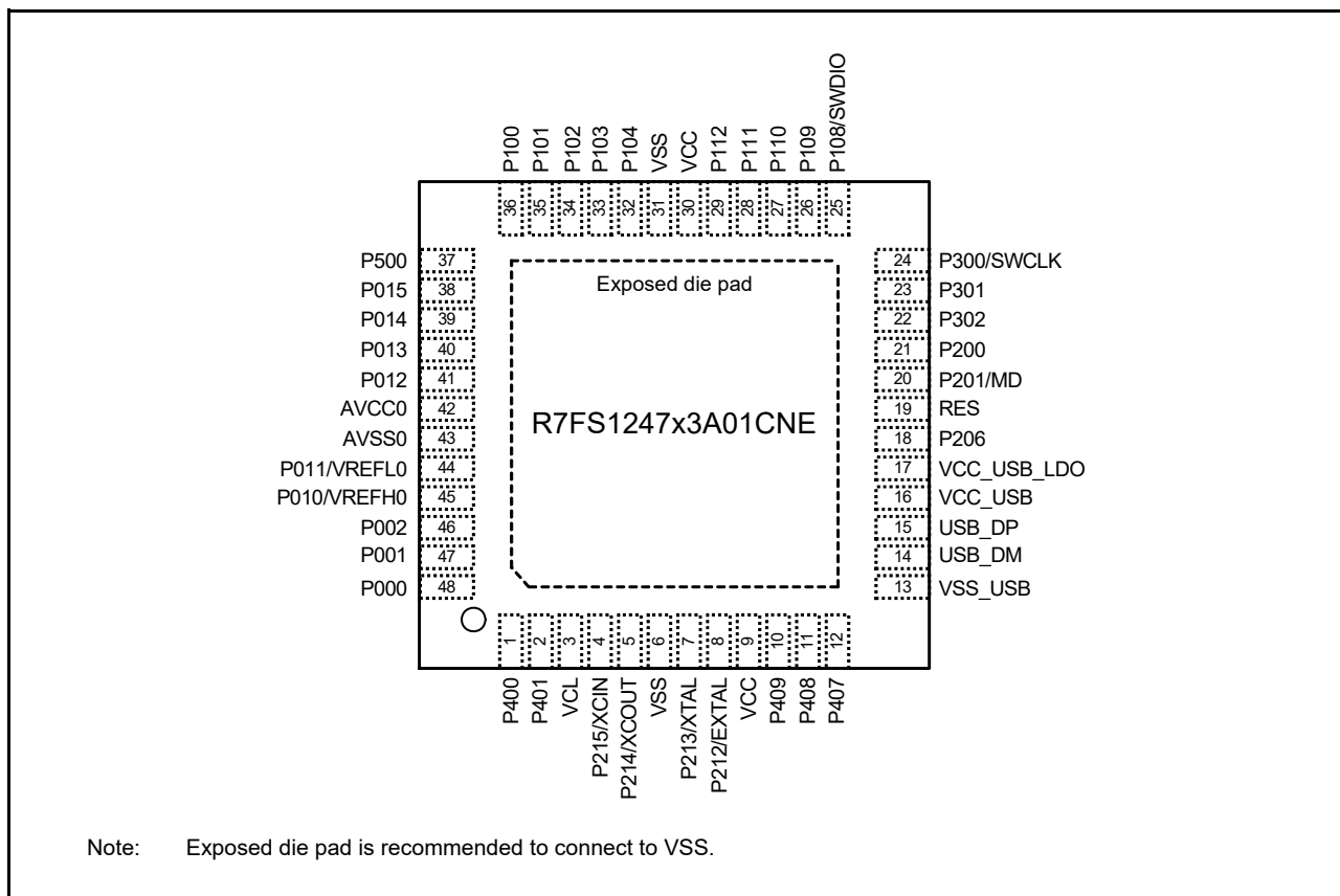
Figure 1.6 Pin assignment for QFN 48-pin (top view)
