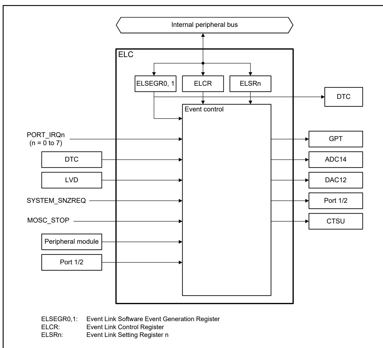
Figure 15.1 ELC block diagram when n = 0 to 3, 8, 9, 12, 14, 15, 18
