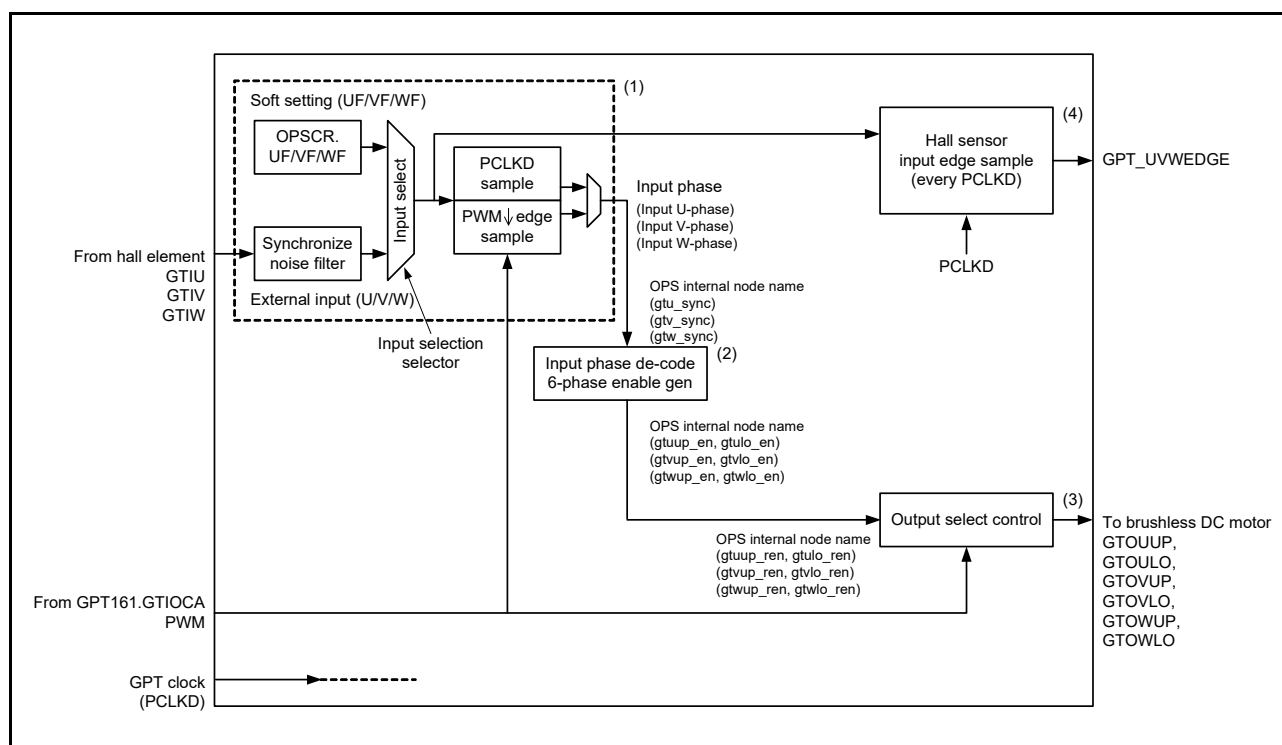
Figure 19.77 GPT_OPS control flow conceptual diagram
