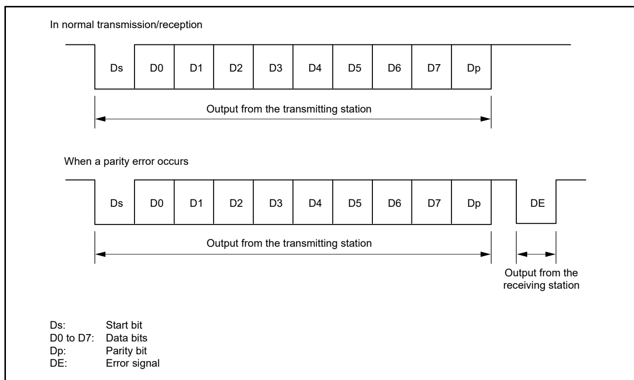
Figure 25.46 Data formats in smart card interface mode
