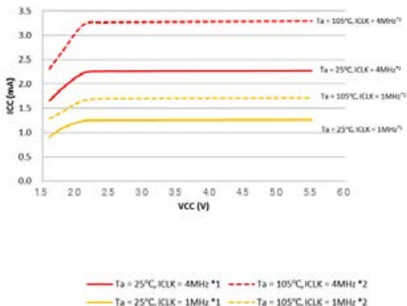
Figure 41.19 Voltage dependency in low-speed operating mode (reference data)
