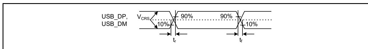
Figure 41.58 USB_DP and USB_DM output timing
