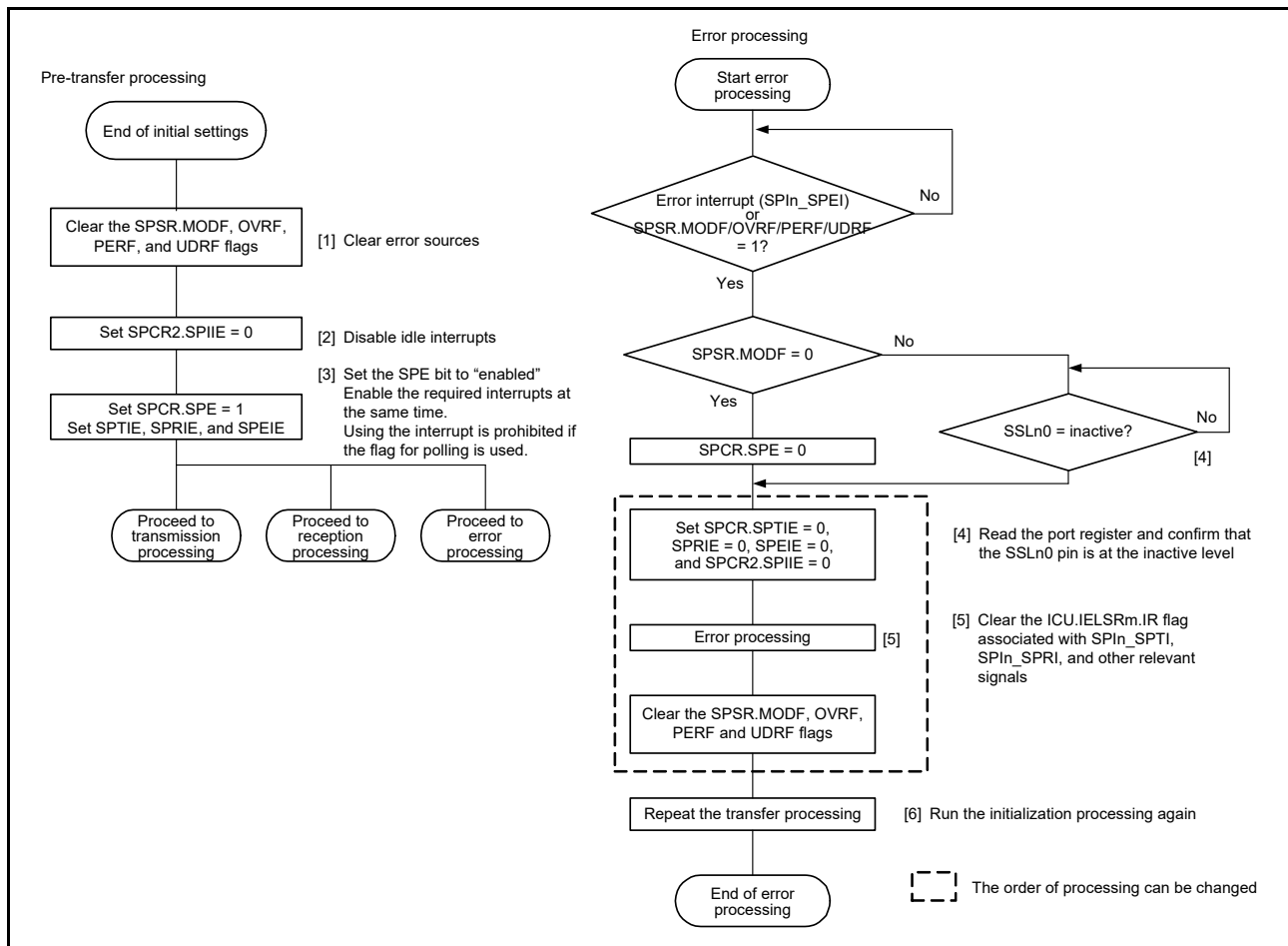
Figure 28.35 Error processing flow in master mode
