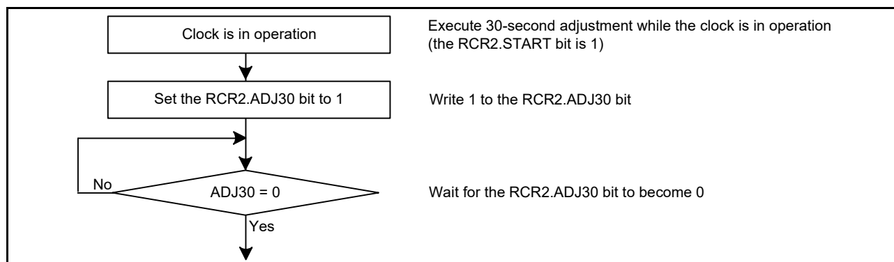
Figure 21.5 30-second adjustment
