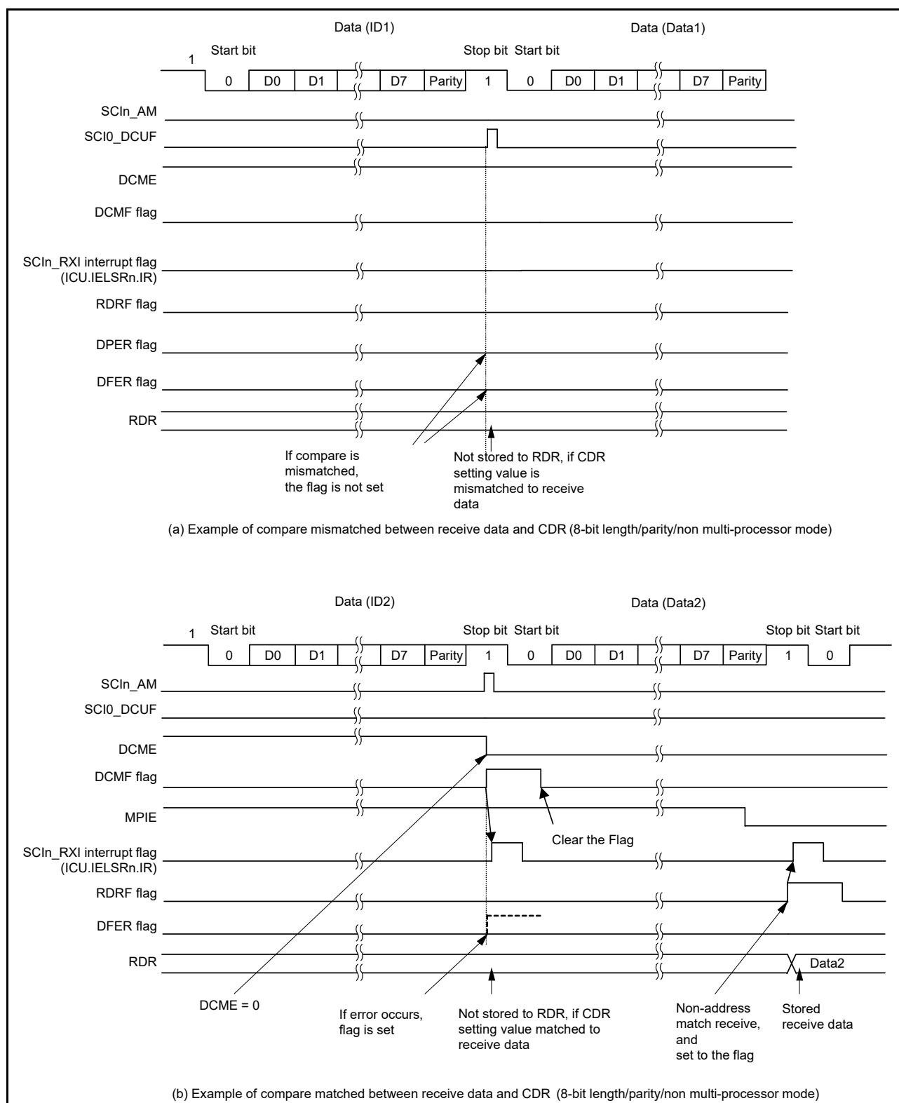
Figure 25.5 Example of address match (1) non multi-processor mode
