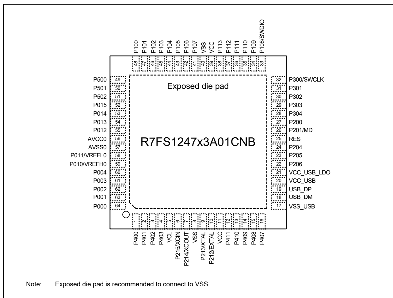
Figure 1.4 Pin assignment for QFN 64-pin (top view)
