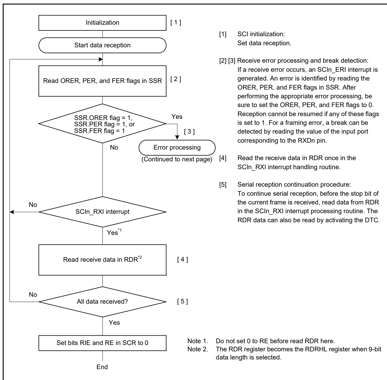
Figure 25.17 Example flow of serial reception in asynchronous mode with non-FIFO selected (1)
