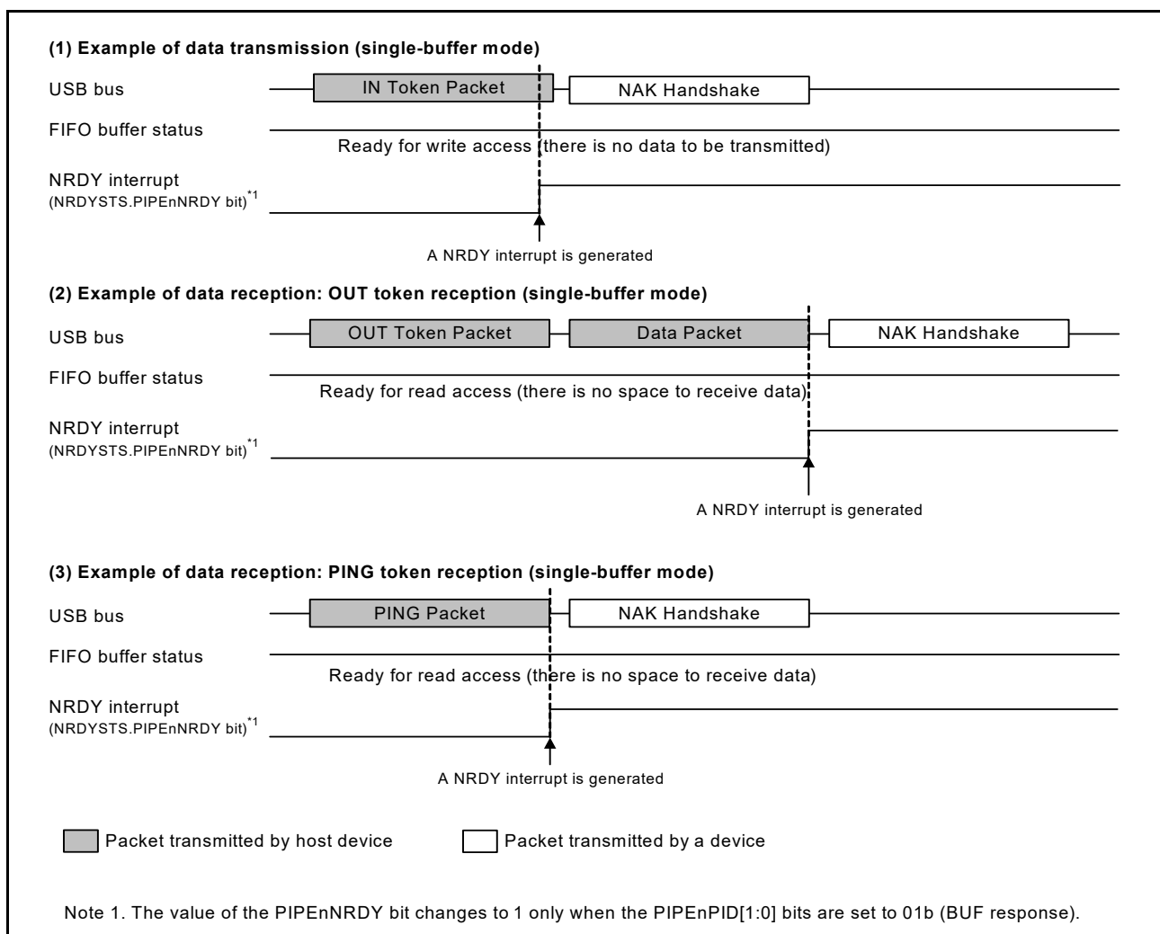
Figure 24.11 Timing of NRDY interrupt generation
