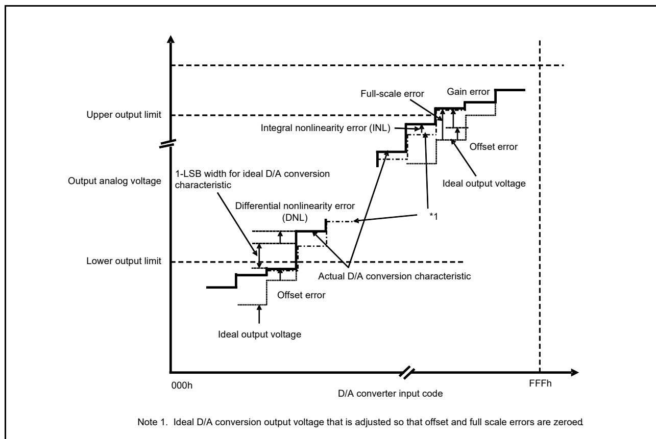
Figure 41.64 Illustration of D/A converter characteristic terms
