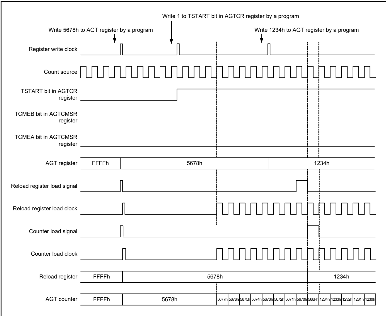
Figure 20.2 Timing of rewrite operation with TSTART, TCMEA and TCMEB bit values when compare match A register and compare match B register are invalid
