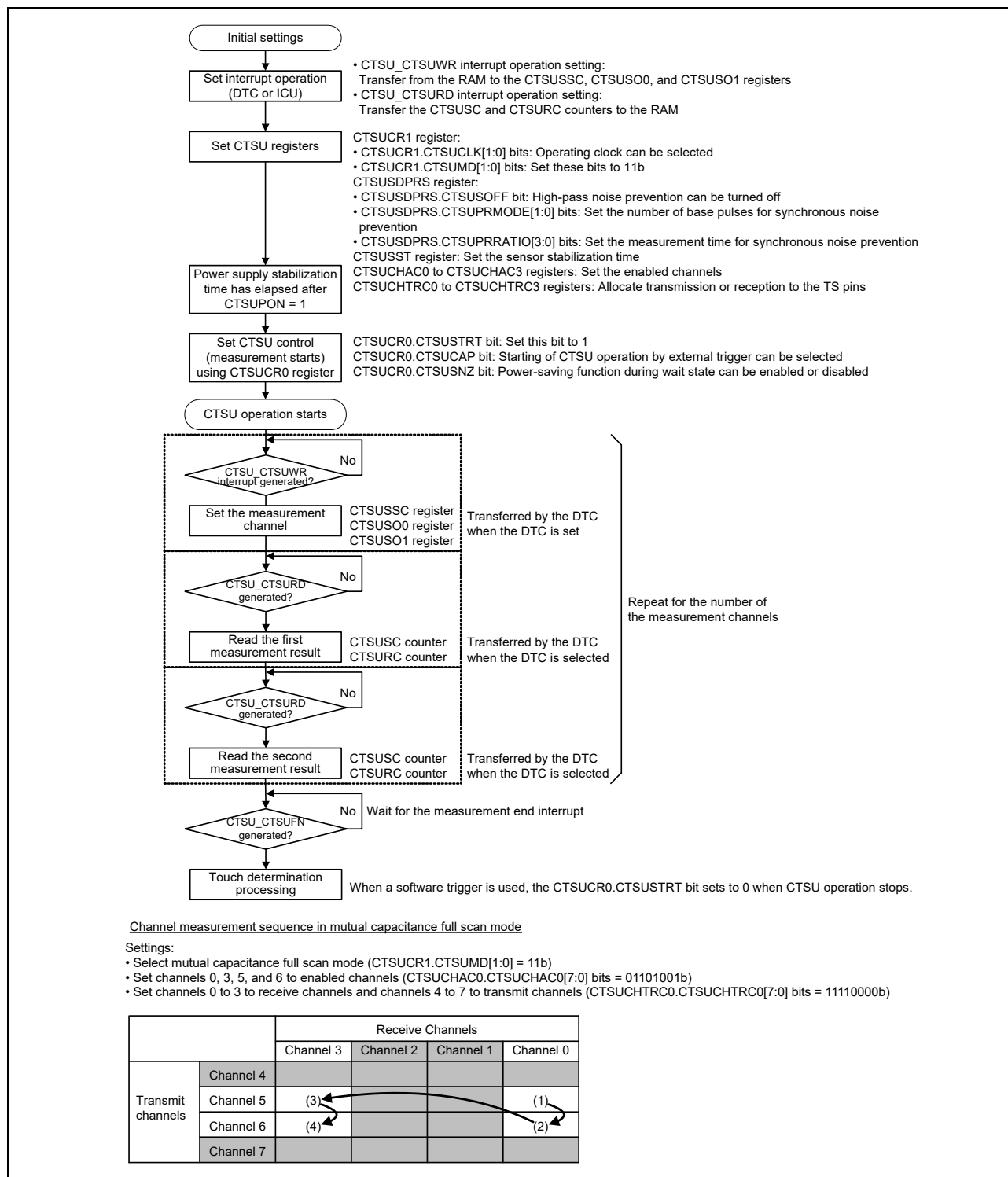
Figure 34.16 Software flow and operation example of mutual capacitance full scan mode
