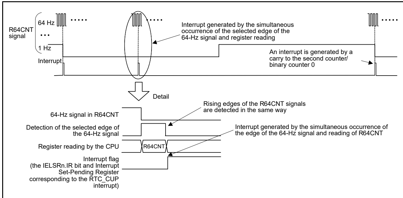
Figure 21.10 Timing of the carry interrupt (RTC_CUP)
