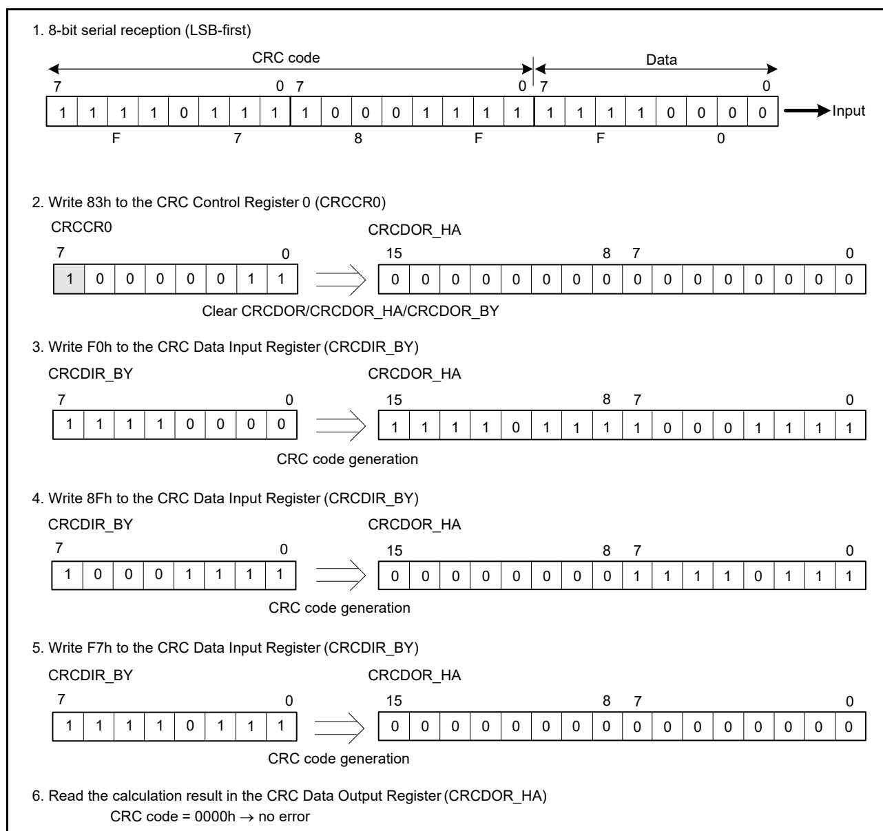
Figure 29.4 LSB-first data reception
