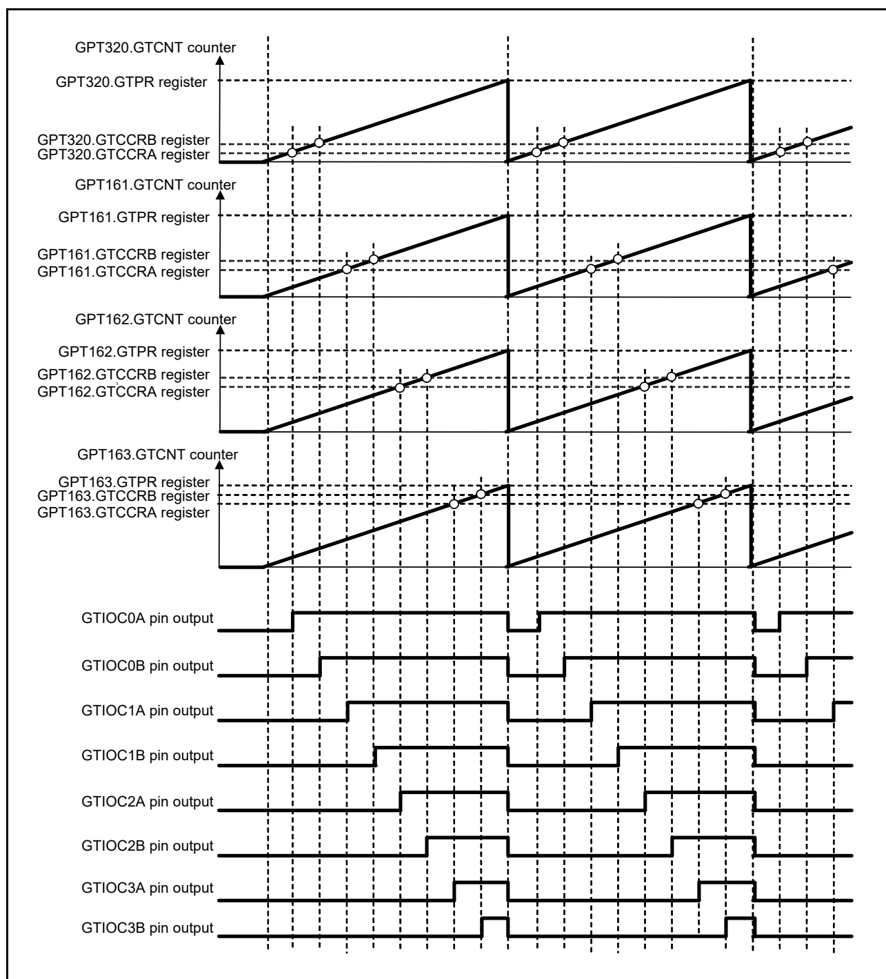
Figure 19.61 Example of synchronized PWM output
