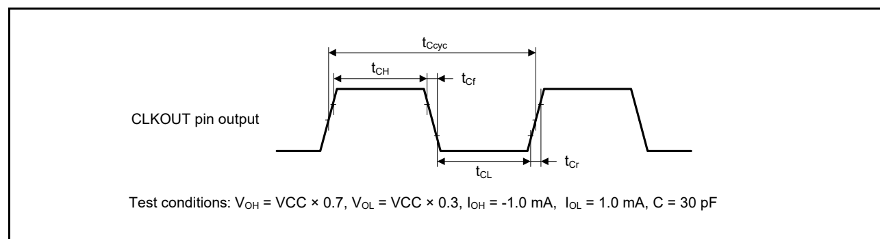
Figure 41.57 CLKOUT output timing
