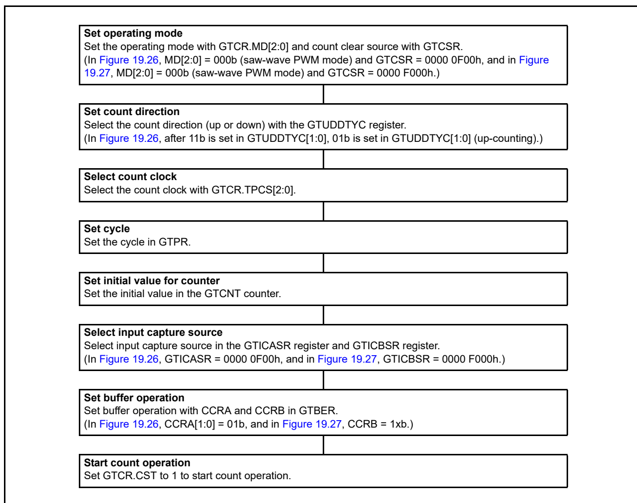
Figure 19.28 Example for setting GTCCRA and GTCCRB buffer operation for input capture
