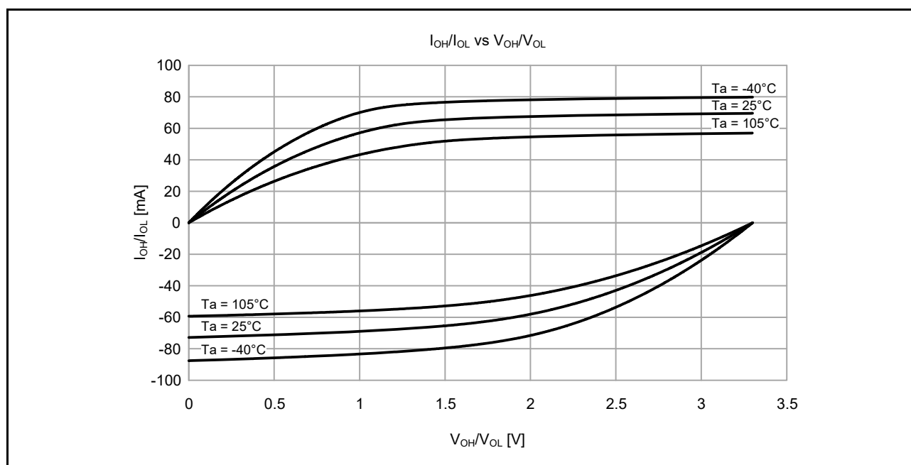
Figure 41.14 V_{OH}/V_{OL} and I_{OH}/I_{OL} temperature characteristics at V_{CC} = 3.3 V when middle drive output is selected (reference data)
