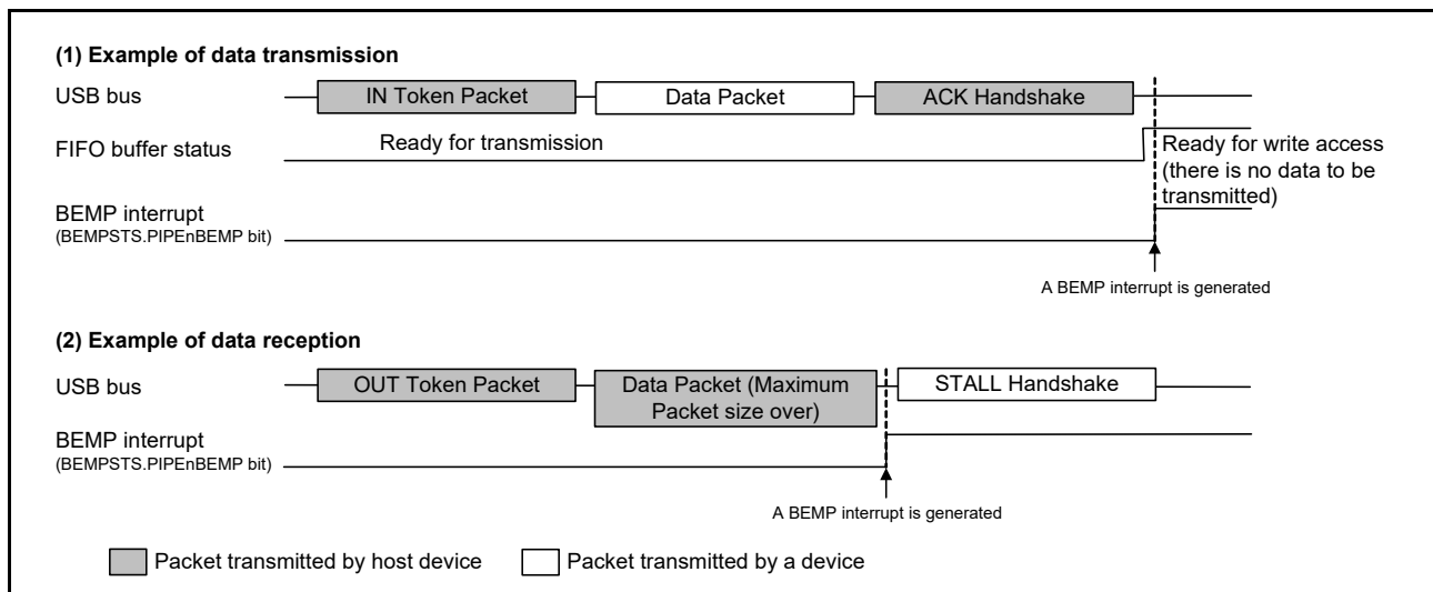
Figure 24.12 Timing of BEMP interrupt generation
