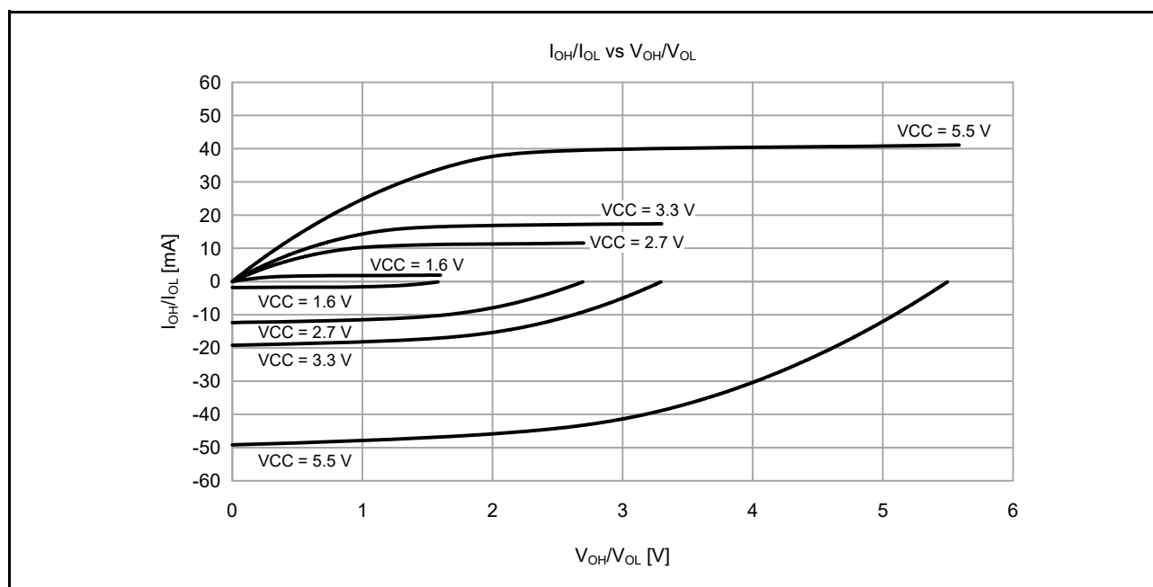
Figure 41.2 V_{OH}/V_{OL} and I_{OH}/I_{OL} voltage characteristics at T_a = 25^\circ\text{C} when low drive output is selected (reference data)
