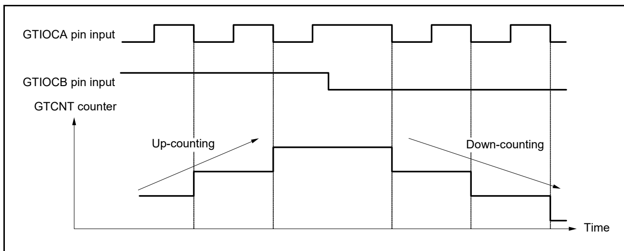
Figure 19.68 Example of phase counting mode 2 (A)
