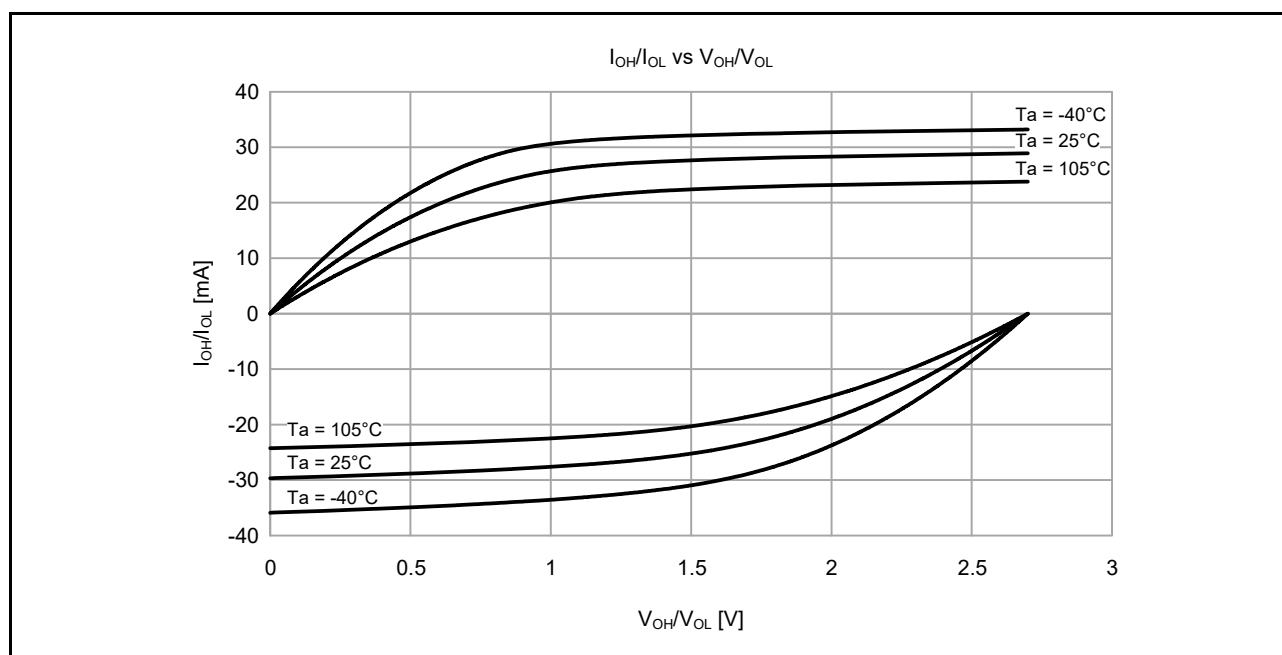
Figure 41.9 V_{OH}/V_{OL} and I_{OH}/I_{OL} temperature characteristics at V_{CC} = 2.7 V when middle drive output is selected (reference data)
