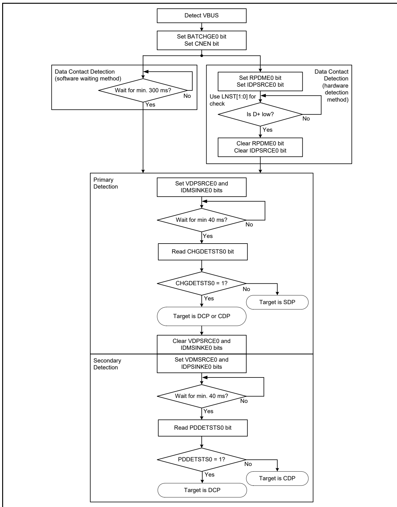
Figure 24.15 Process flow for operating as portable device
