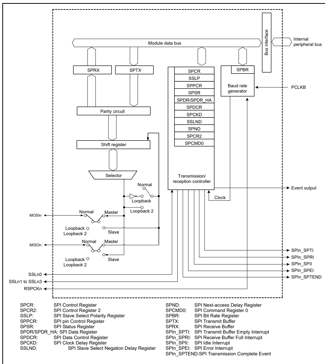
Figure 28.1 SPI block diagram
