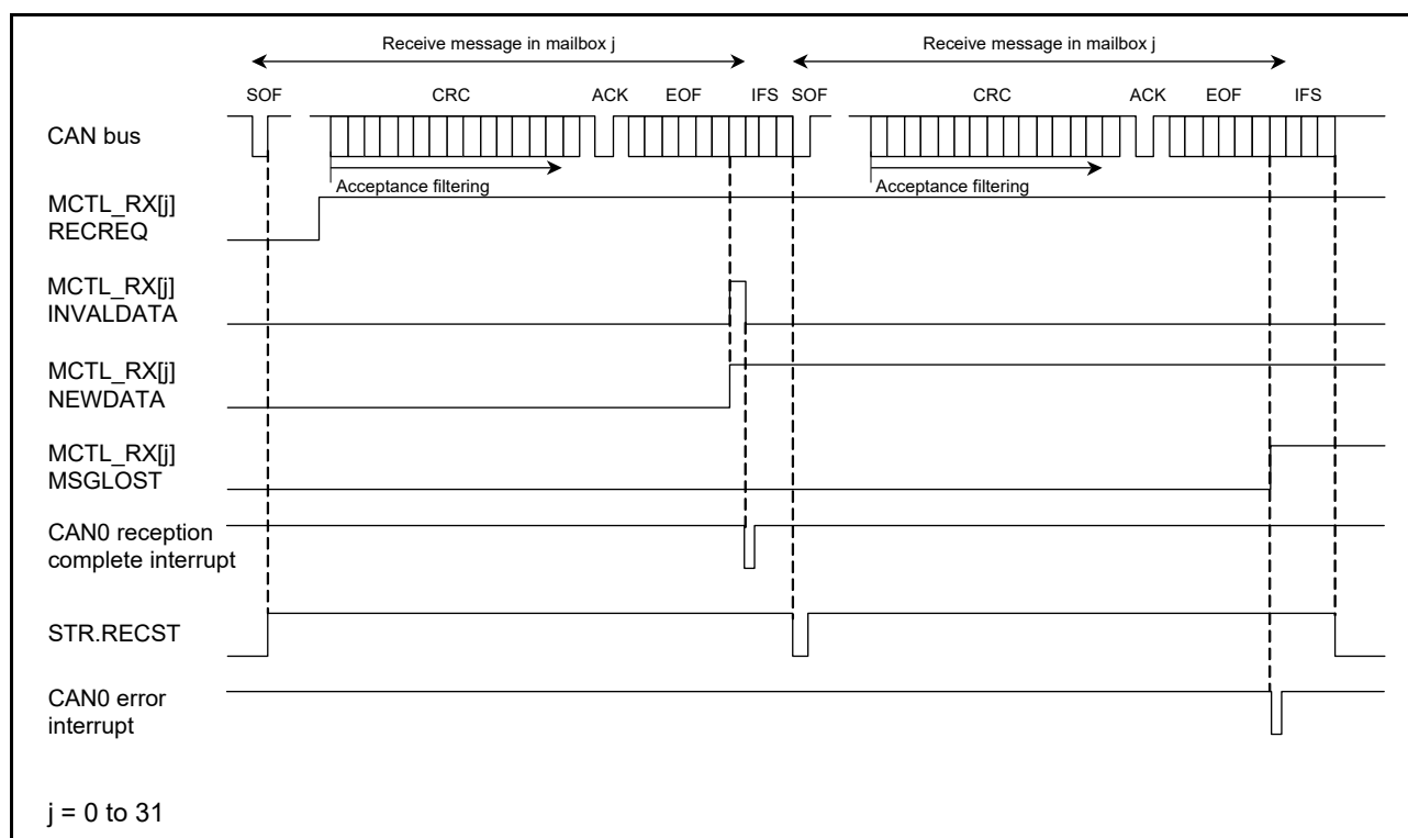
Figure 27.19 Operation example of data frame reception in overrun mode
