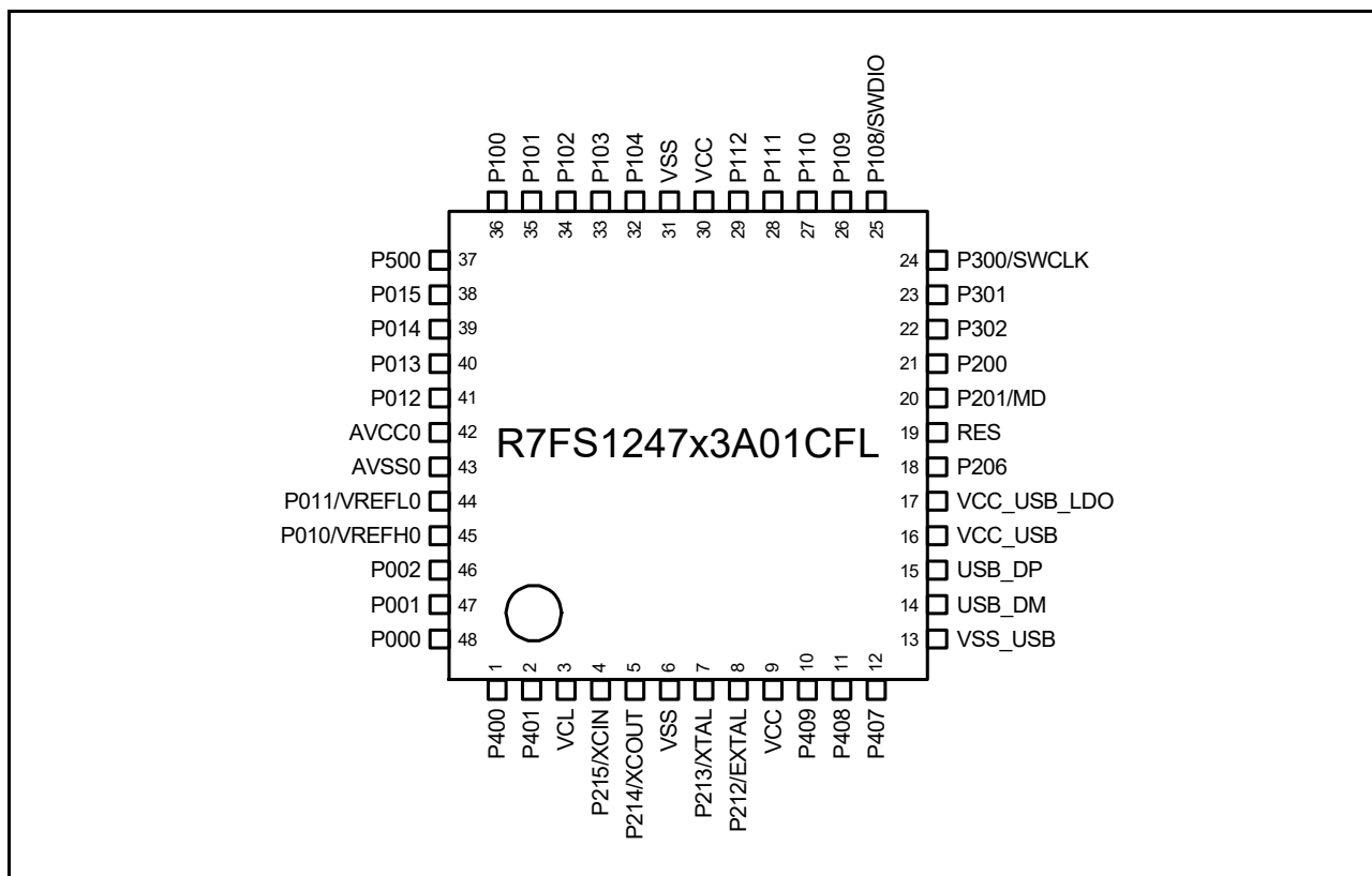
Figure 1.5 Pin assignment for LQFP 48-pin (top view)
