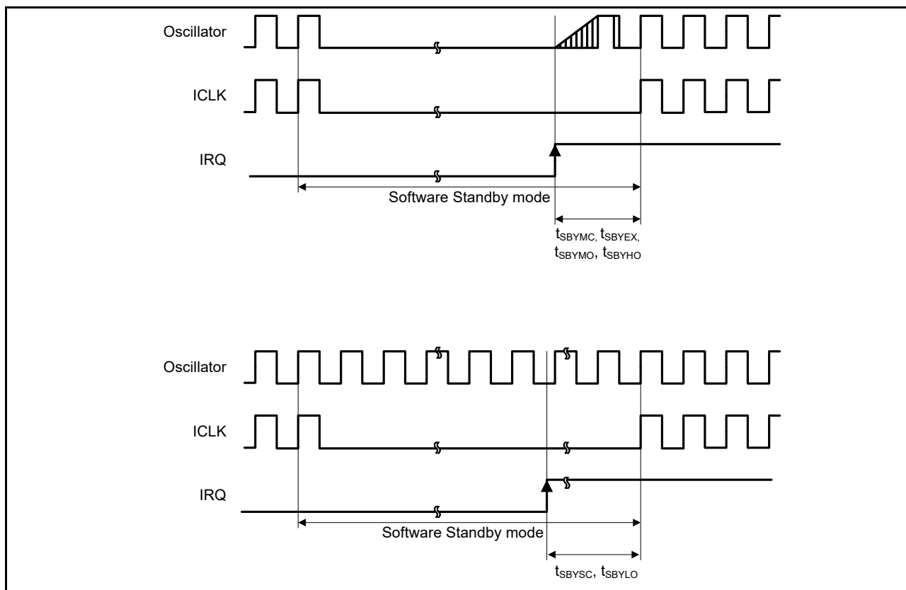
Figure 41.31 Software Standby mode cancellation timing
