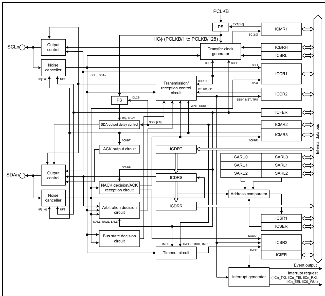
Figure 26.1 IIC block diagram
