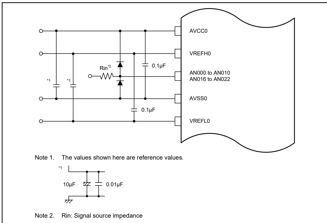
Figure 30.32 Example protection circuit for analog inputs
