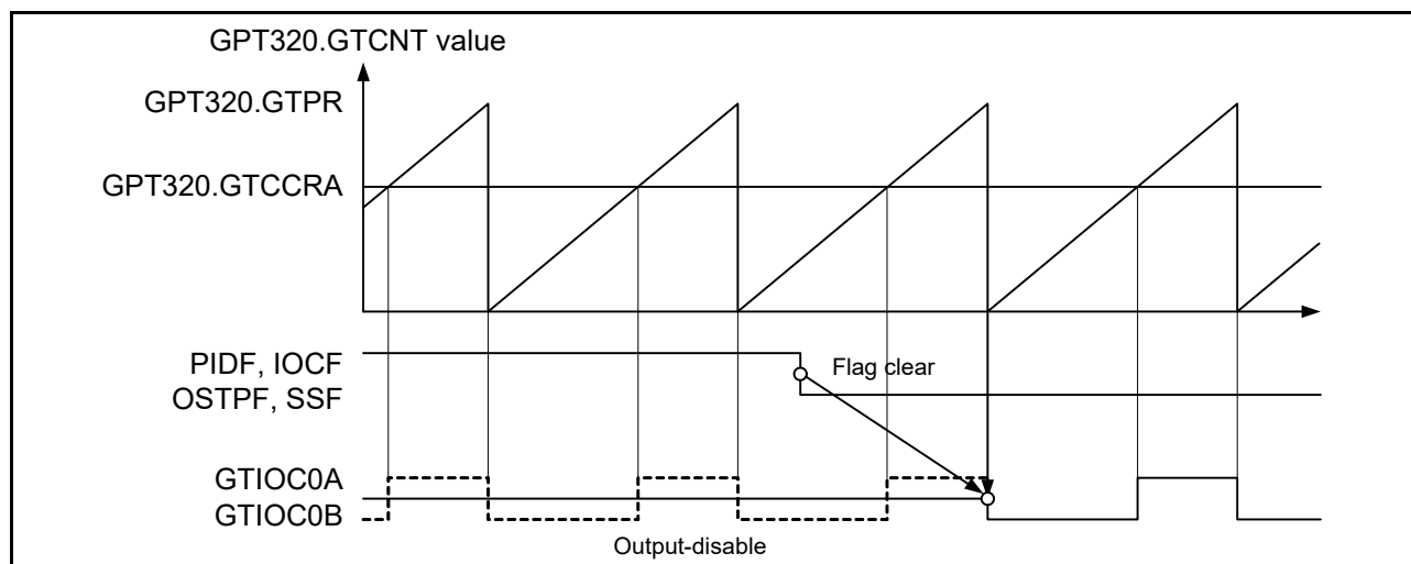
Figure 18.3 Released timing of GPT pin output from output disable
