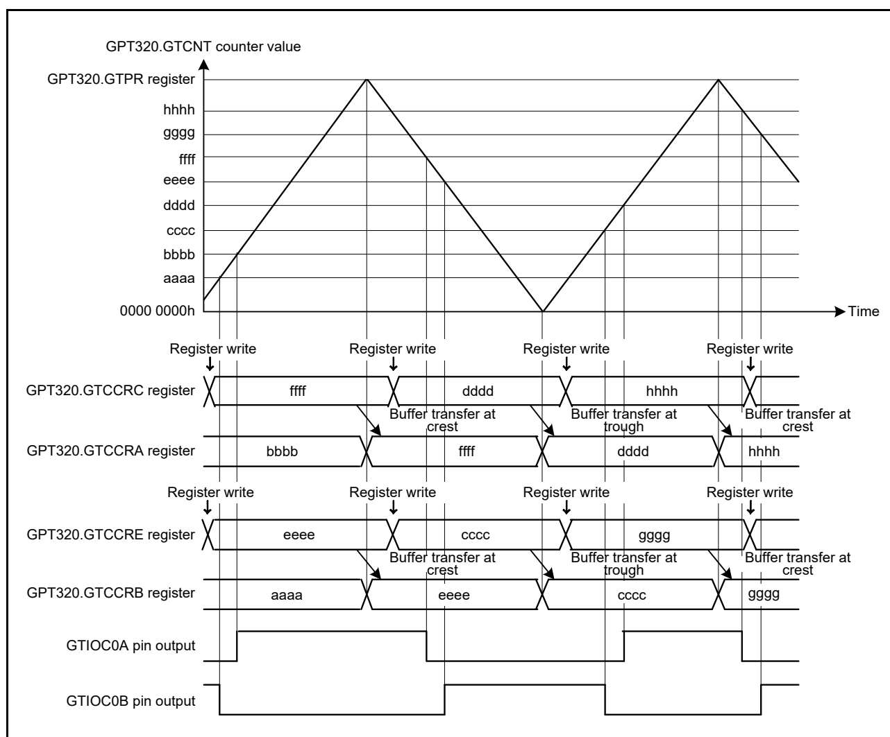
Figure 19.35 Example of triangle-wave PWM mode 2 operation with buffer operation, low output from the GTIOC0A pin and high output from the GTIOC0B pin at count start, output toggled at GTCCRA/GTCCRB compare match, and output retained at cycle end
