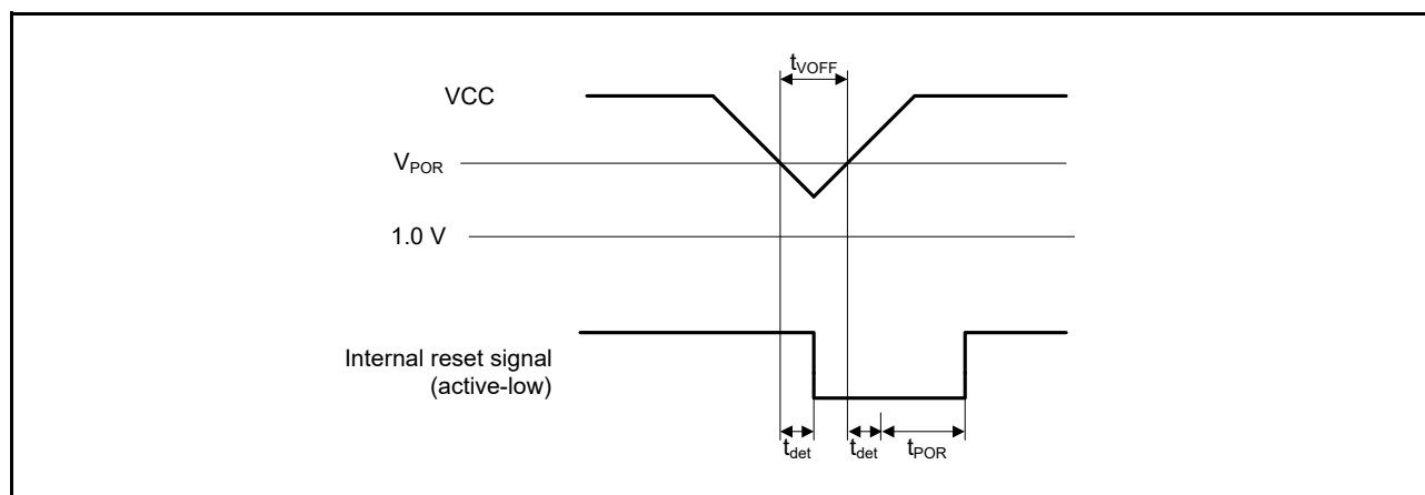
Figure 41.66 Voltage detection reset timing
