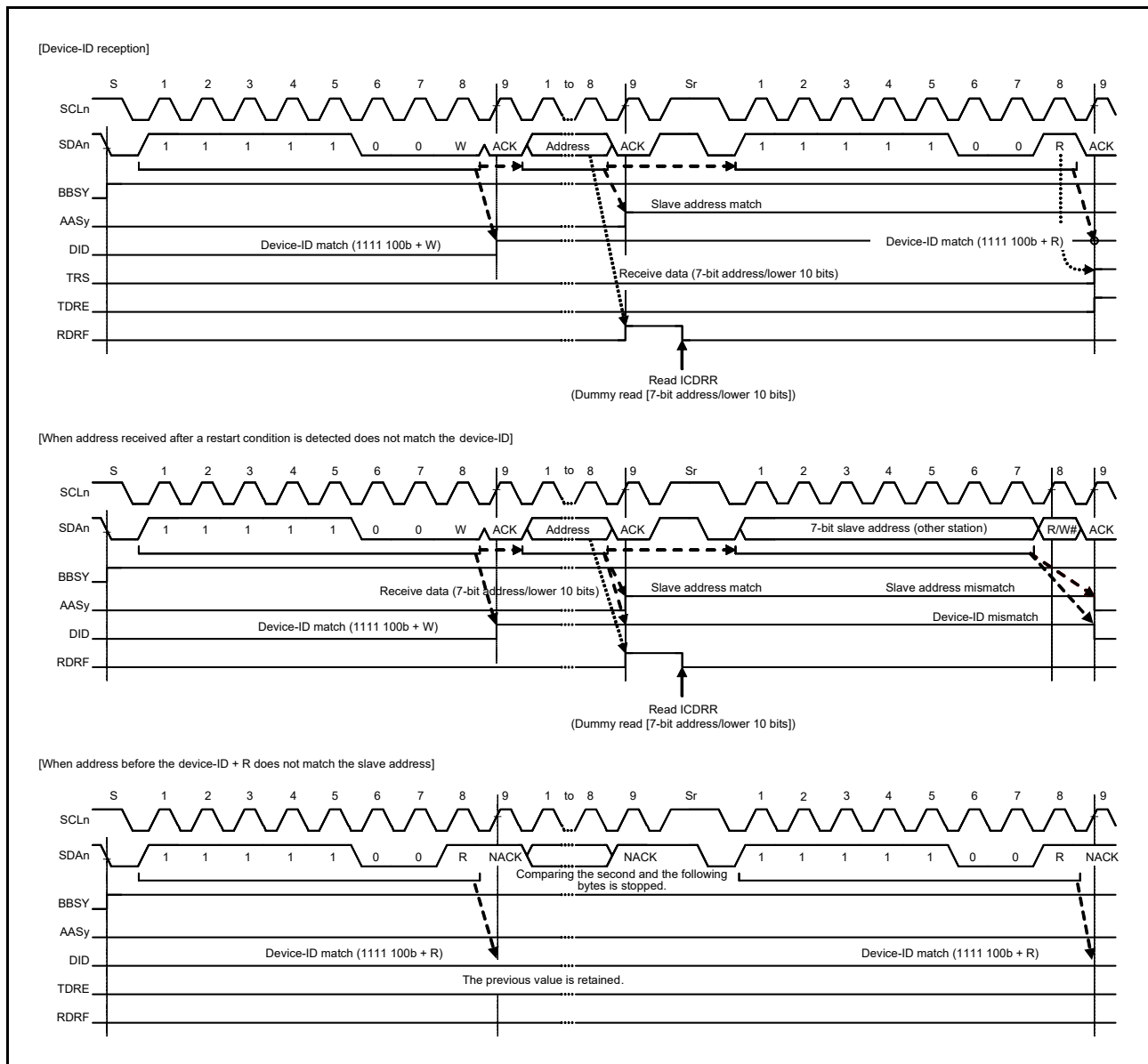
Figure 26.28 AASy/DID flag set and clear timing during reception of device ID
