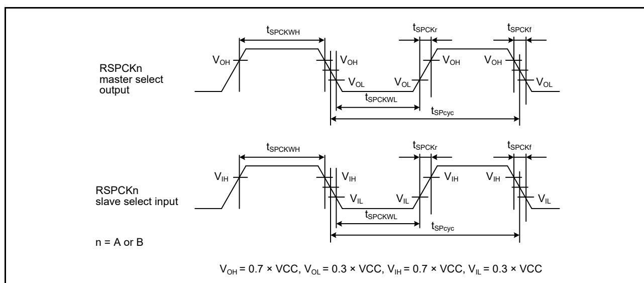
Figure 41.49 SPI clock timing
