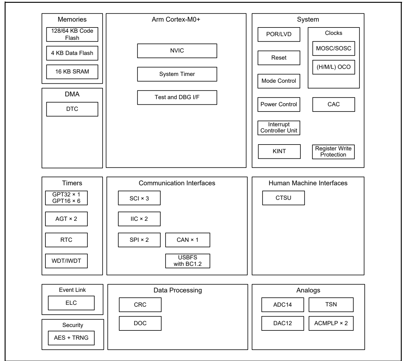
Figure 1.1 Block diagram
