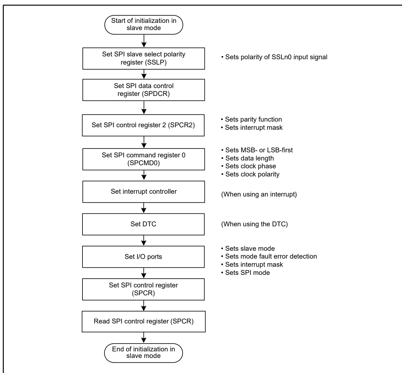
Figure 28.36 Example of initialization flow in slave mode for SPI operation
