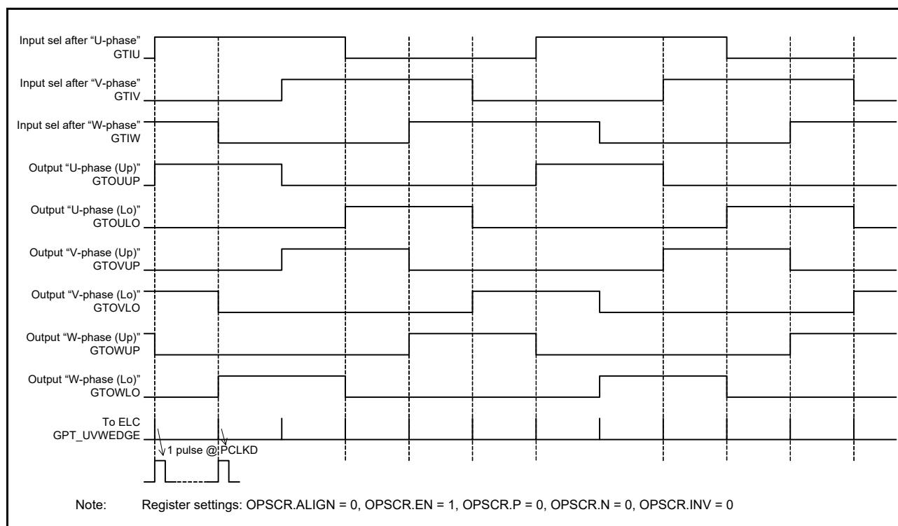
Figure 19.78 6-phase level output operation example
