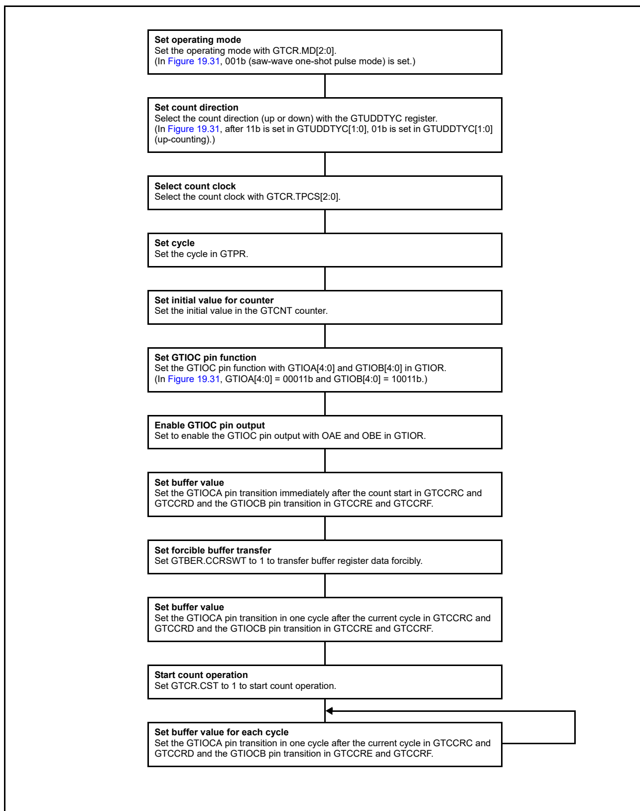
Figure 19.32 Example for setting saw-wave one-shot pulse mode
