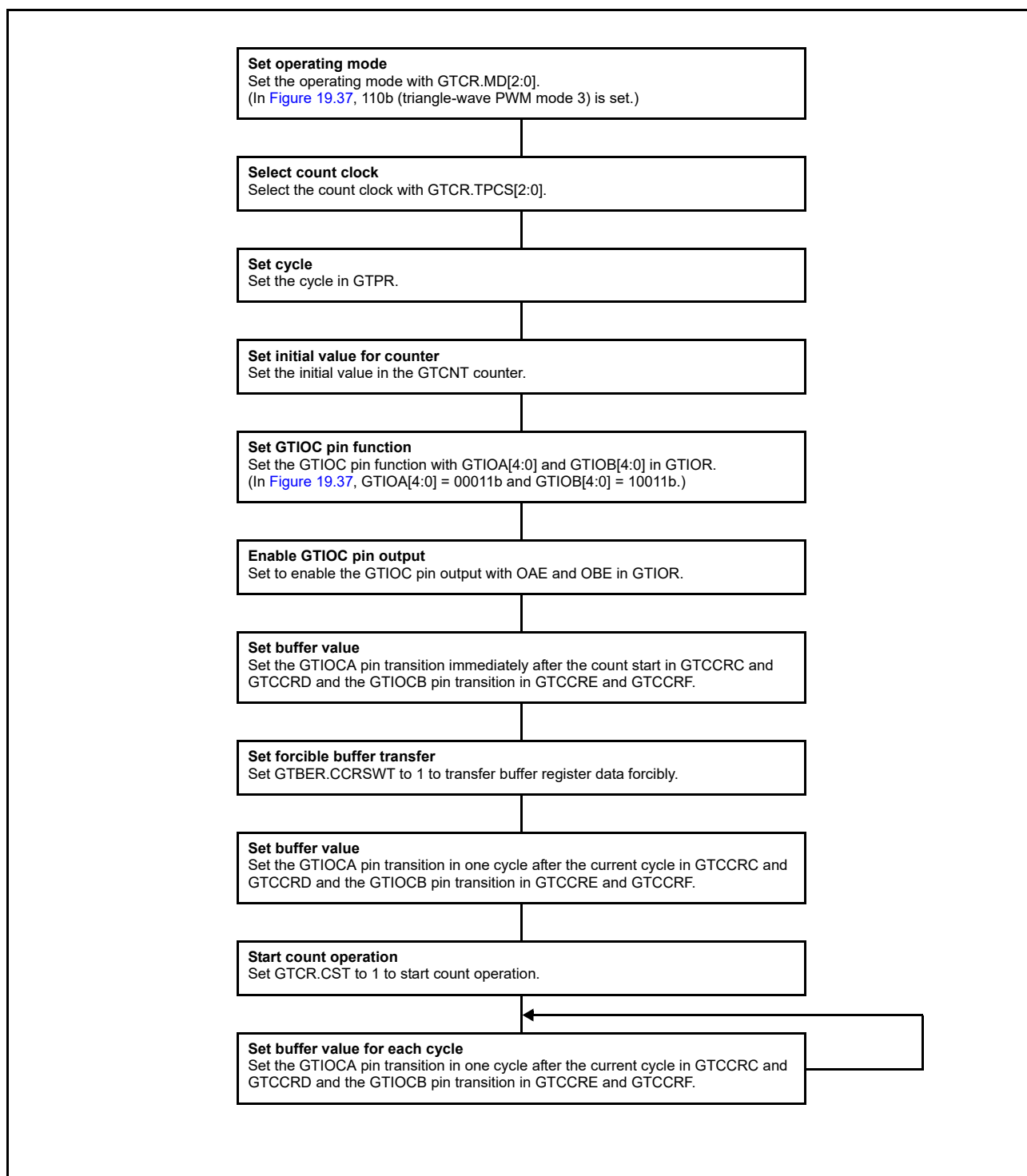
Figure 19.38 Example for setting triangle-wave PWM mode 3
