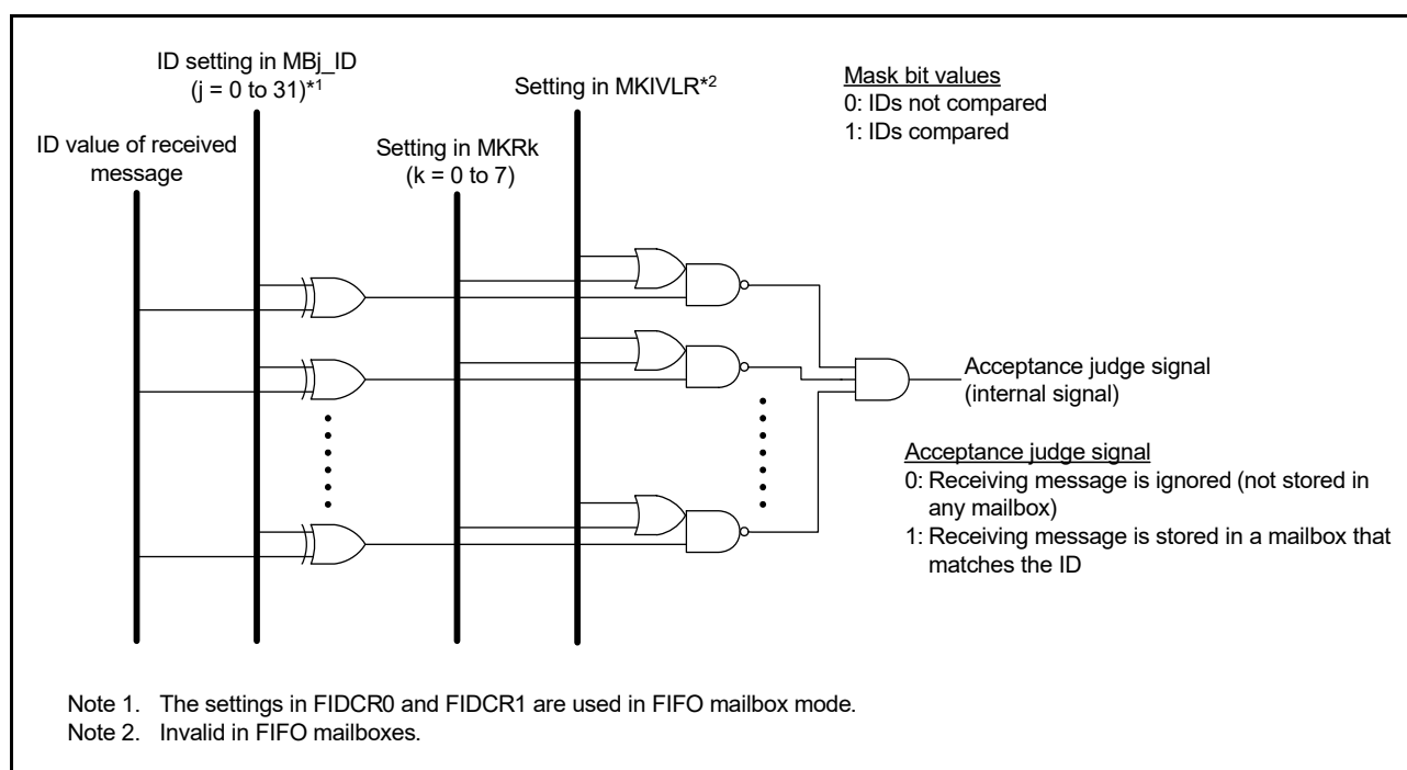
Figure 27.17 Acceptance filtering
