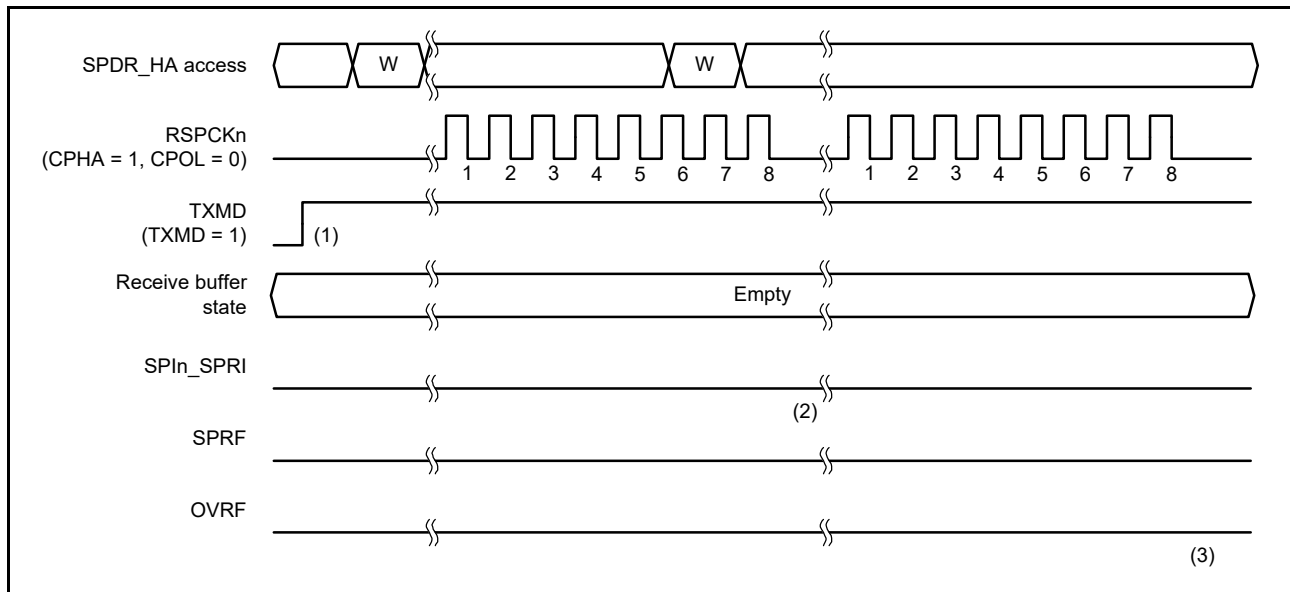
Figure 28.25 Operation example when SPCR.TXMD = 1
