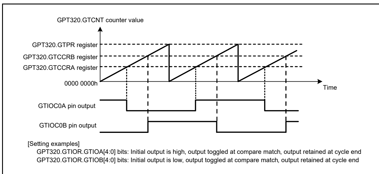
Figure 19.13 Example of toggled output operation (1)
