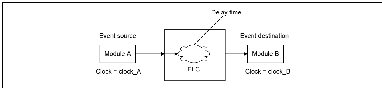
Figure 15.2 ELC delay time
