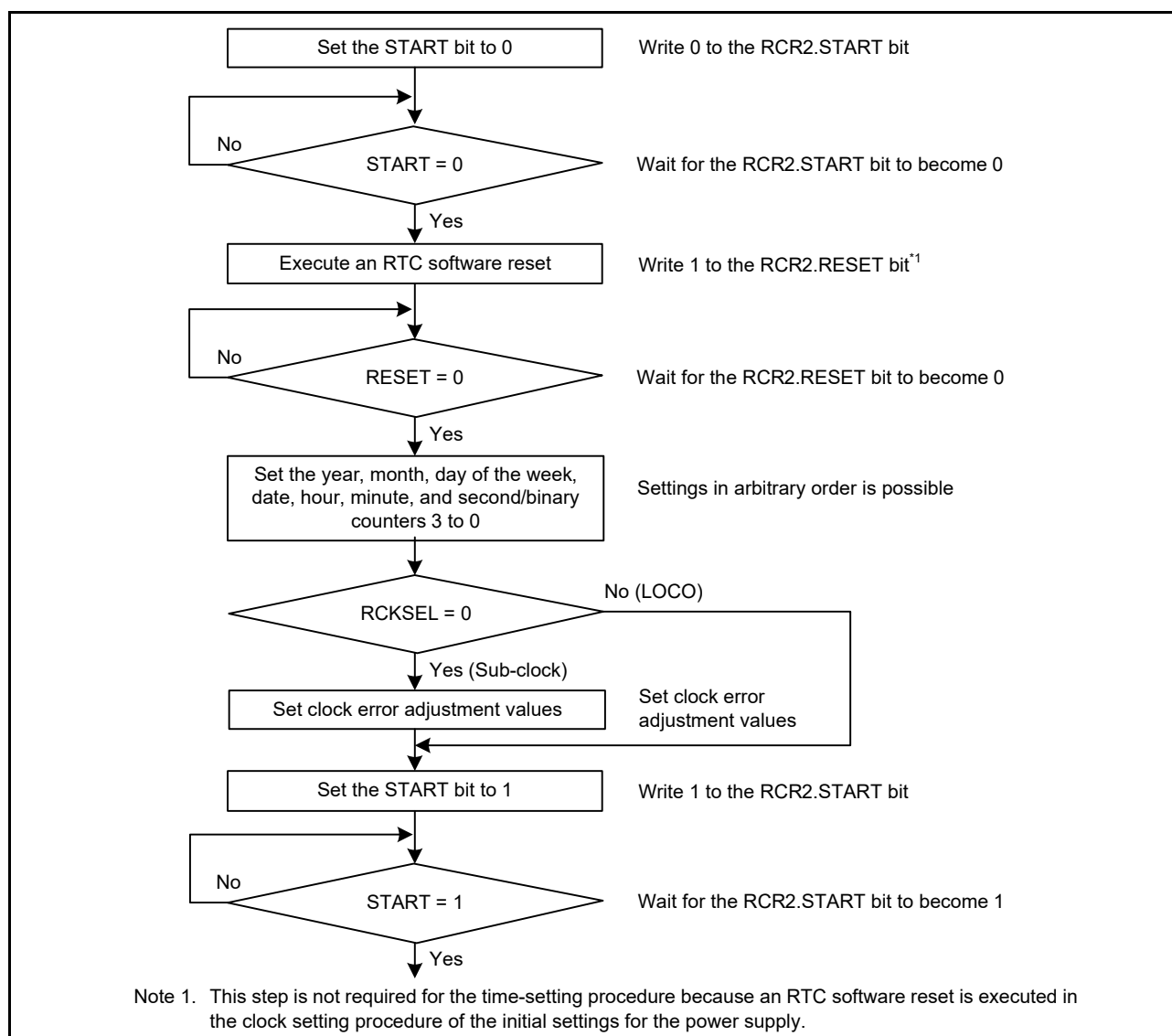
Figure 21.4 Setting the time
