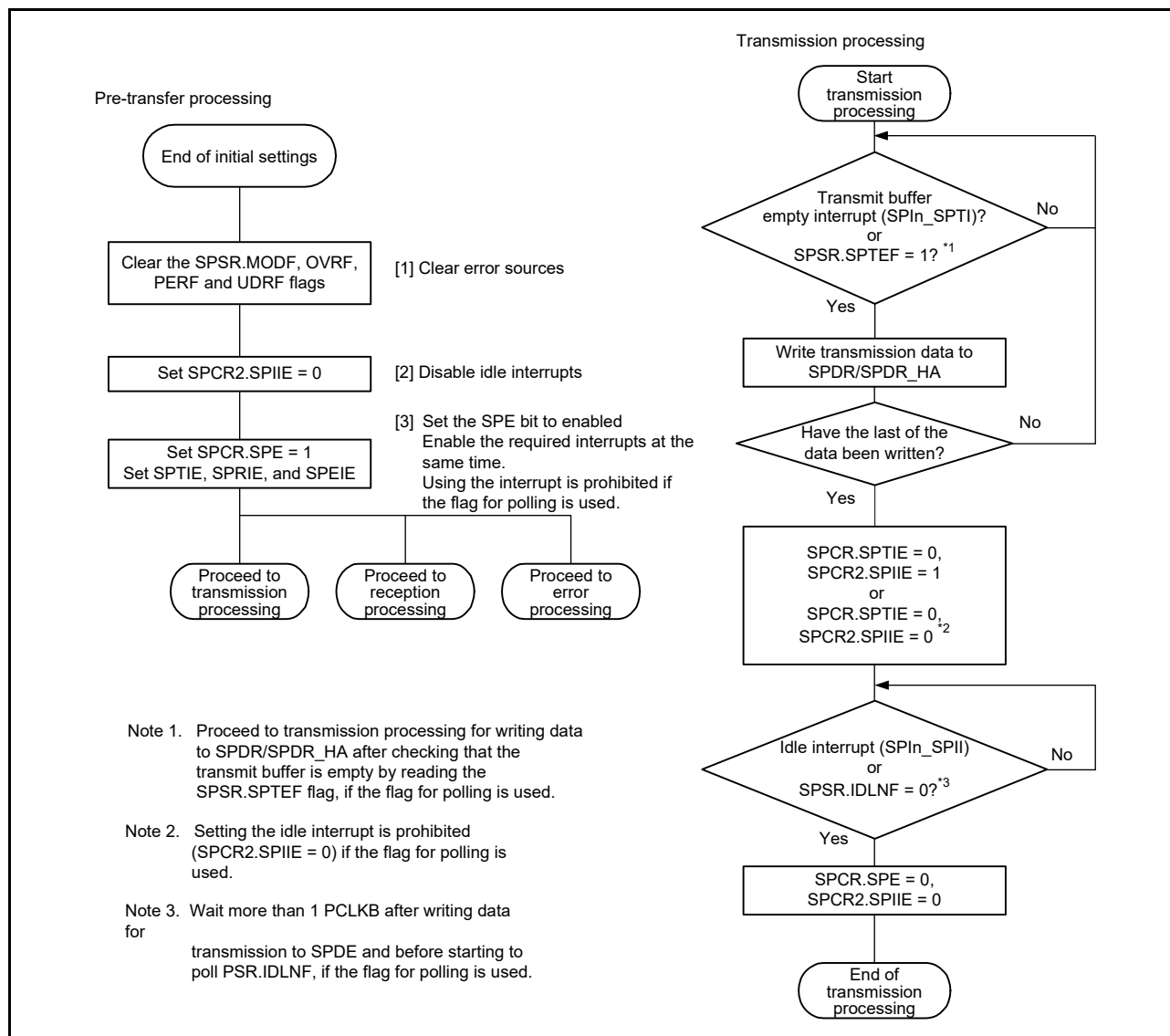
Figure 28.33 Transmission flow in master mode
