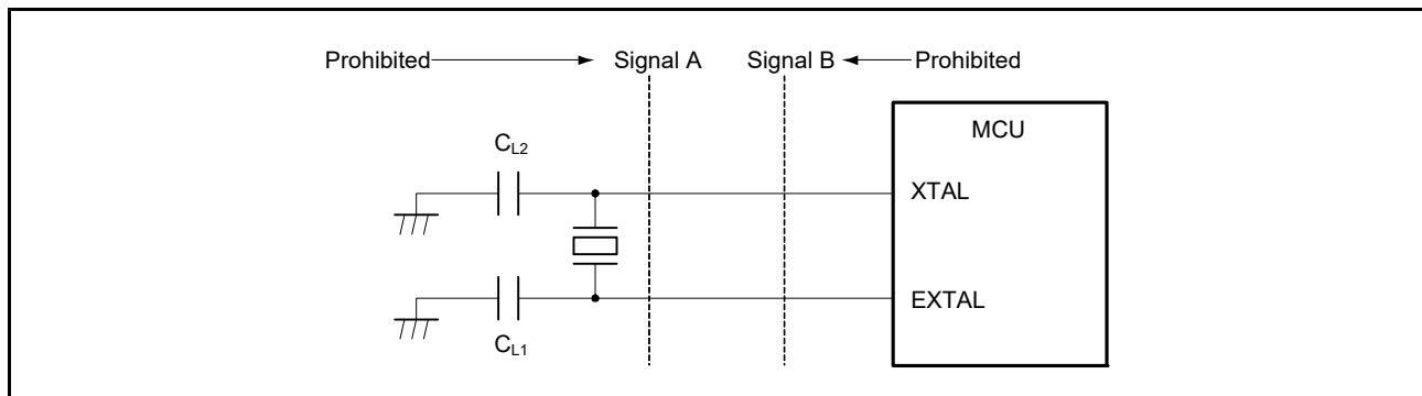
Figure 8.6 Signals routing in board design for oscillation circuit (applies to the sub-clock oscillator for the main clock oscillator)
