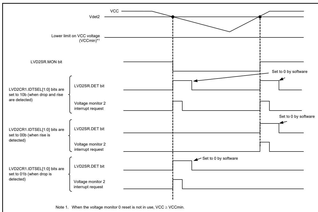
Figure 7.6 Example of voltage monitor 2 interrupt operation
