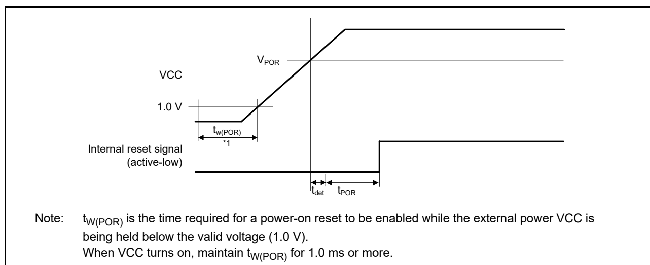
Figure 41.67 Power-on reset timing
