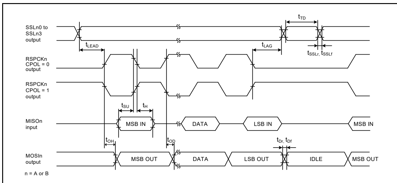
Figure 41.52 SPI timing (master, CPHA = 1) (bit rate: PCLKB division ratio is set to any value other than 1/2)
