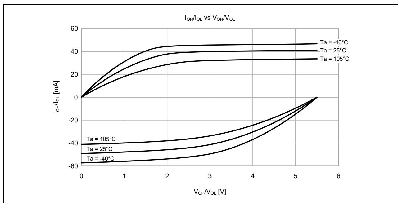
Figure 41.6 V_{OH}/V_{OL} and I_{OH}/I_{OL} temperature characteristics at V_{CC} = 5.5 V when low drive output is selected (reference data)
