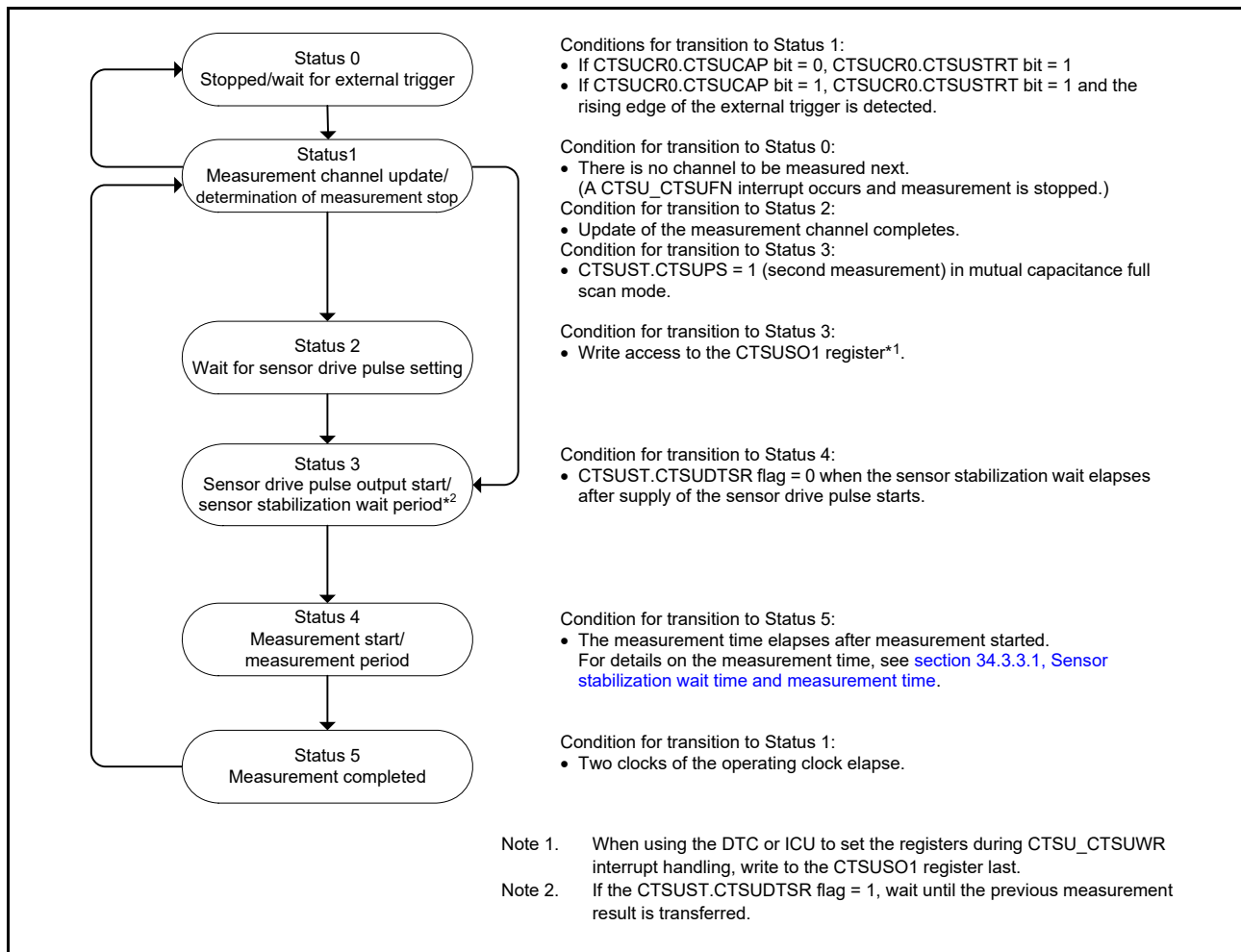
Figure 34.11 Status operation transitions
