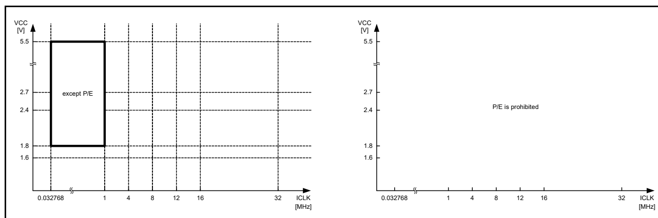
Figure 10.5 Operating voltages and frequencies in low-speed mode
