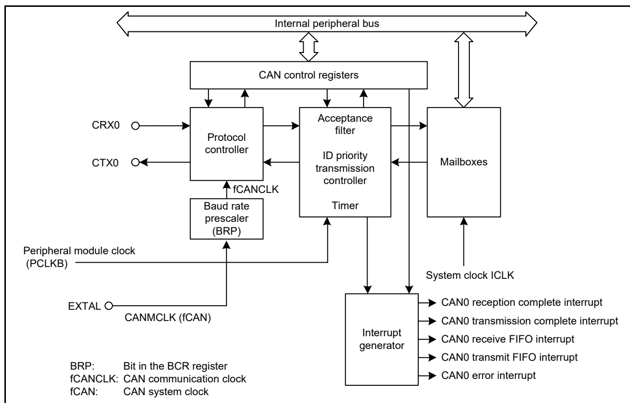
Figure 27.1 CAN module block diagram
