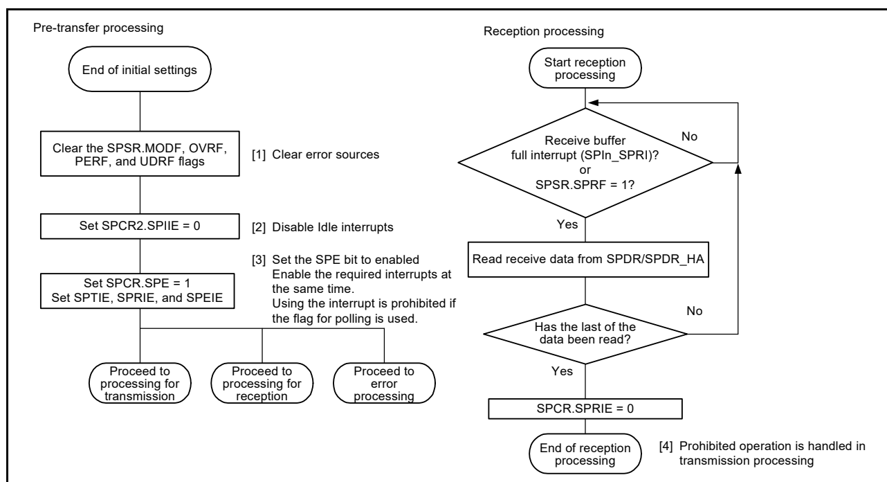
Figure 28.34 Reception flow in master mode
