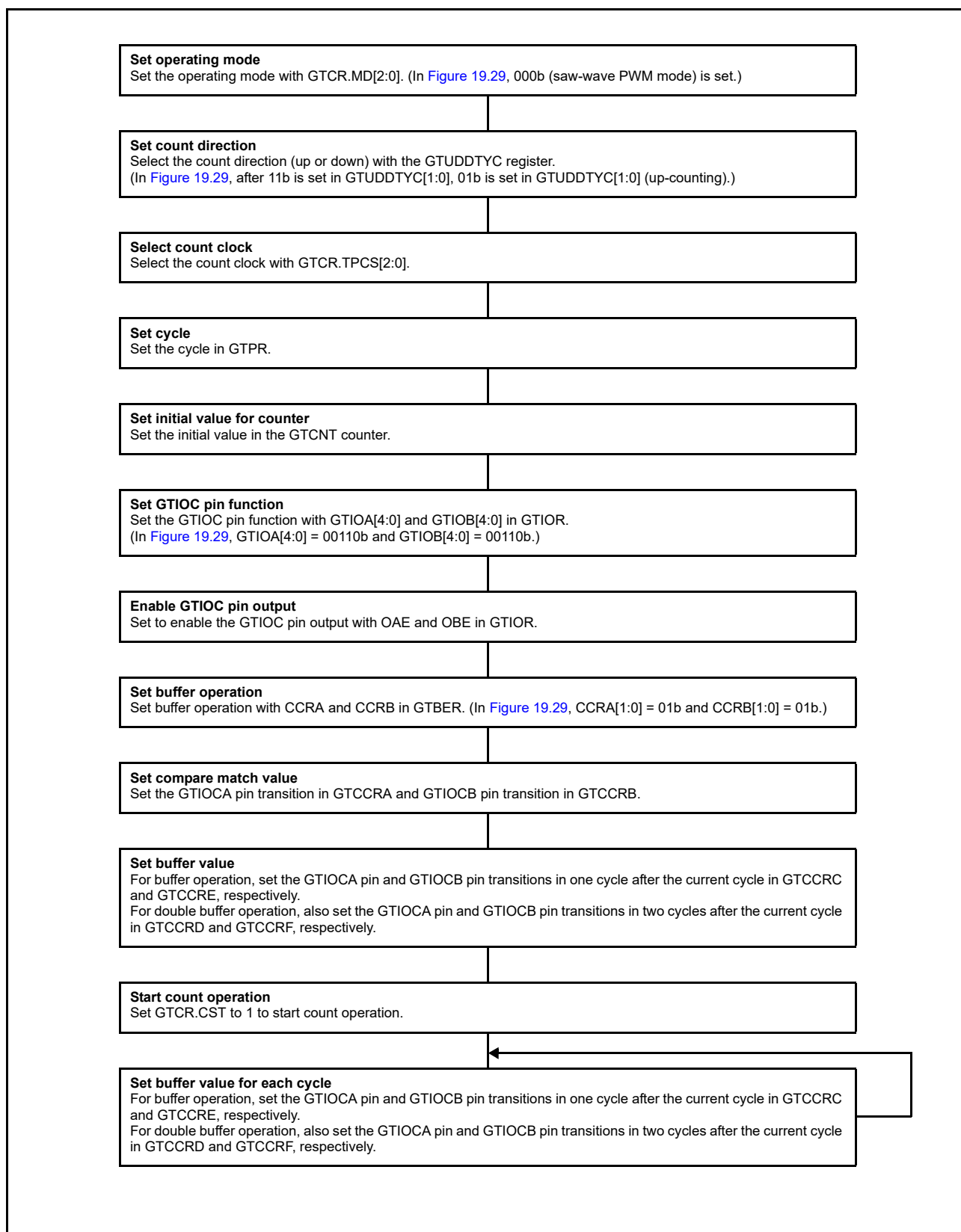
Figure 19.30 Example for setting saw-wave PWM mode
