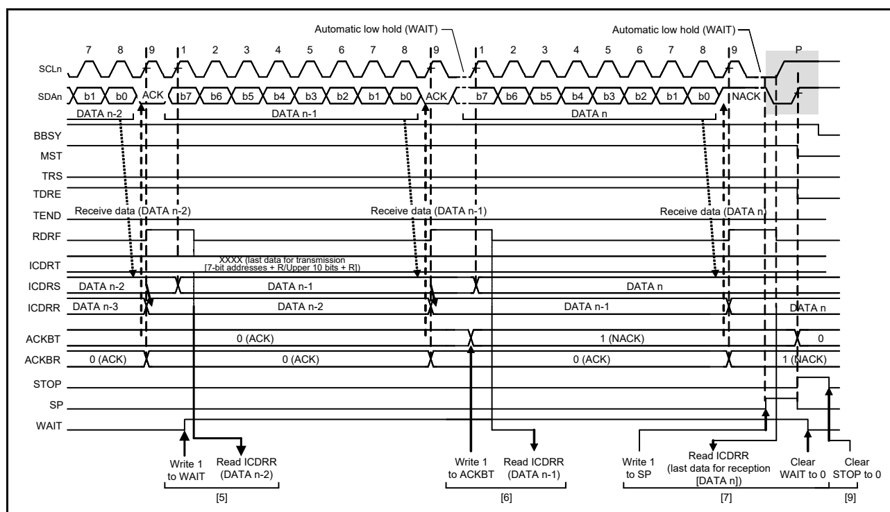
Figure 26.14 Master receive operation timing (3) when RDRFS = 0
