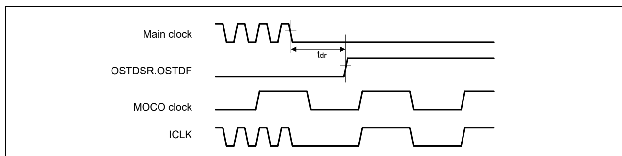
Figure 41.65 Oscillation stop detection timing
