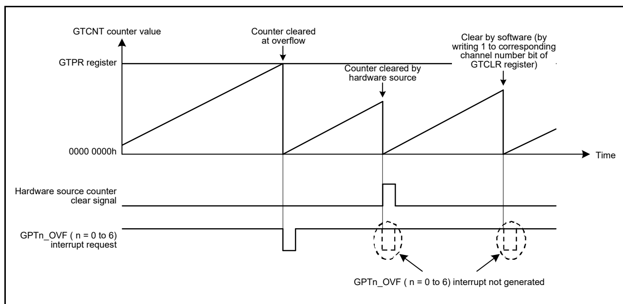
Figure 19.56 Relationship between counter clearing by hardware source and GPTn_OVF (n = 0 to 6) interrupt
