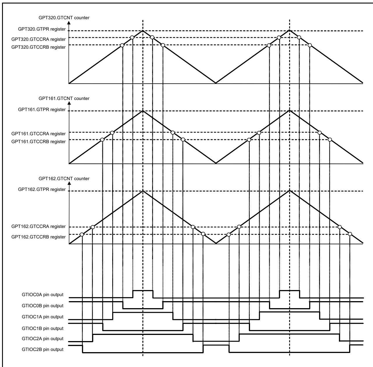
Figure 19.64 Example of 3-phase triangle-wave complementary PWM output
