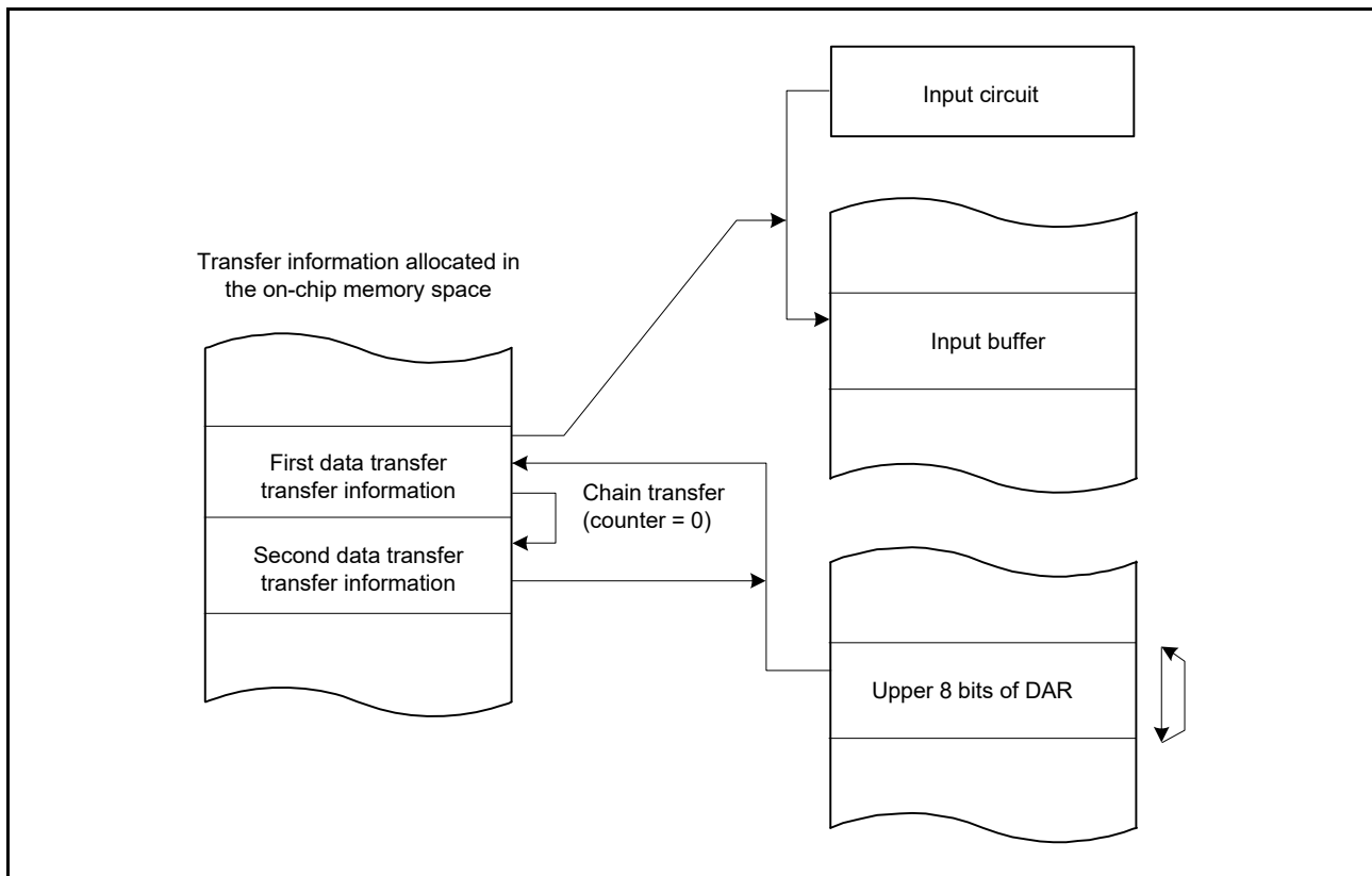
Figure 14.14 Chain transfer when counter = 0
