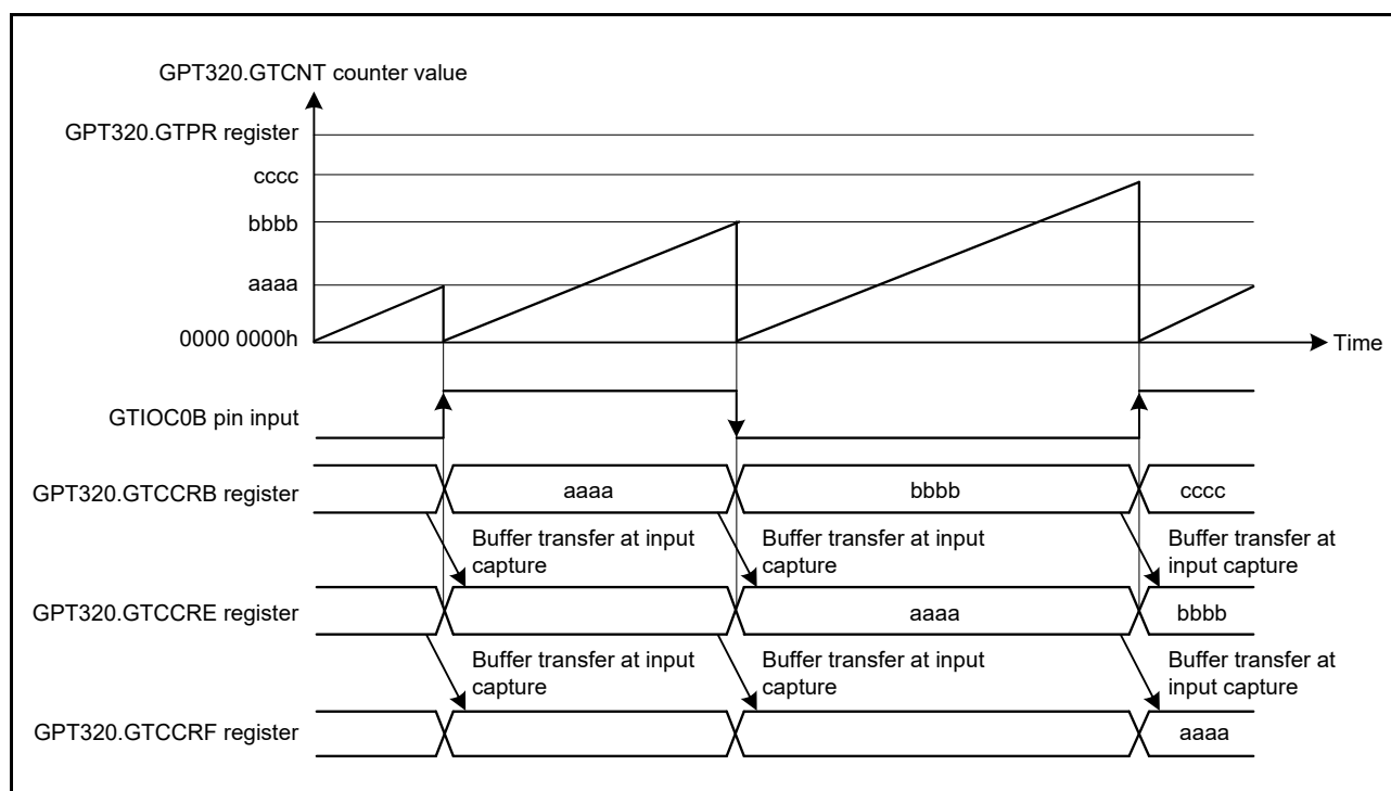
Figure 19.27 Example of GTCCRA and GTCCRB double buffer operation with input capture at both edges of GTIOC0B input, saw waves in up-counting, and GTCNT counter cleared at both edges of GTIOC0B input
