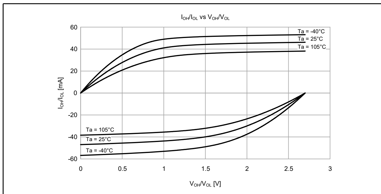
Figure 41.13 V_{OH}/V_{OL} and I_{OH}/I_{OL} temperature characteristics at V_{CC} = 2.7\text{ V} when middle drive output is selected (reference data)
