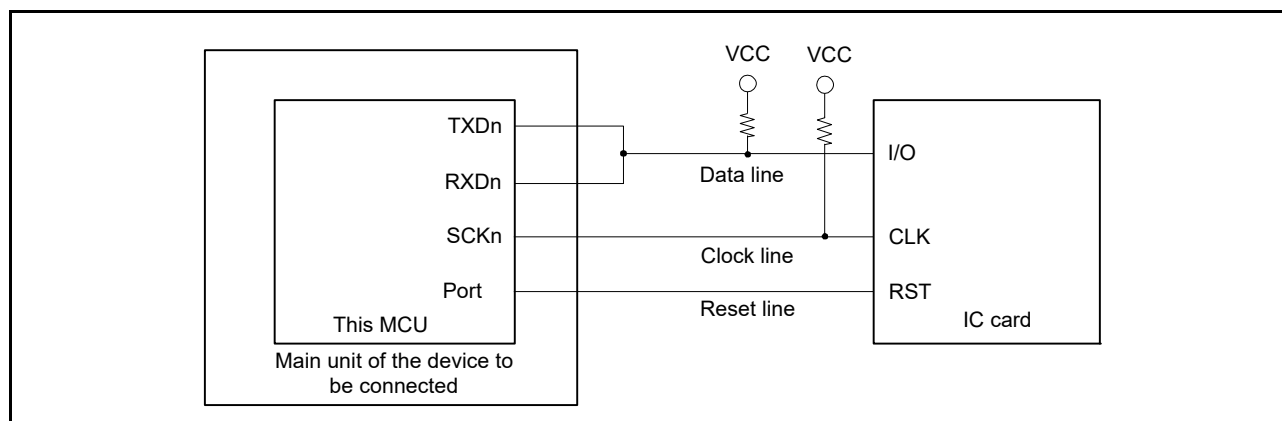
Figure 25.45 Example connection with a Smart Card (IC Card)
