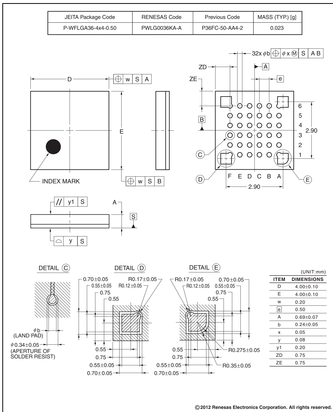
Figure 2.3 LGA 36-pin
