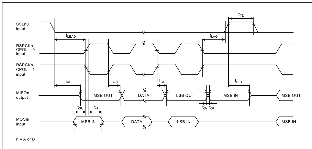
Figure 41.54 SPI timing (slave, CPHA = 0)
