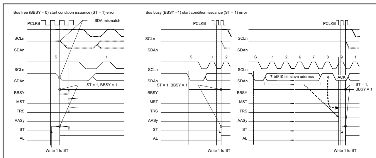
Figure 26.42 Arbitration-loss when start condition is issued (MALE = 1)
