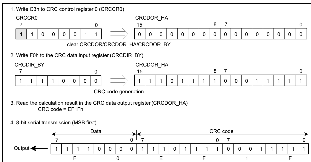
Figure 29.3 MSB-first data transmission
