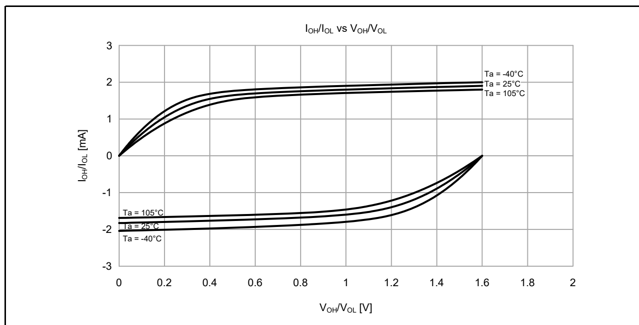
Figure 41.3 V_{OH}/V_{OL} and I_{OH}/I_{OL} temperature characteristics at V_{CC} = 1.6\text{ V} when low drive output is selected (reference data)
