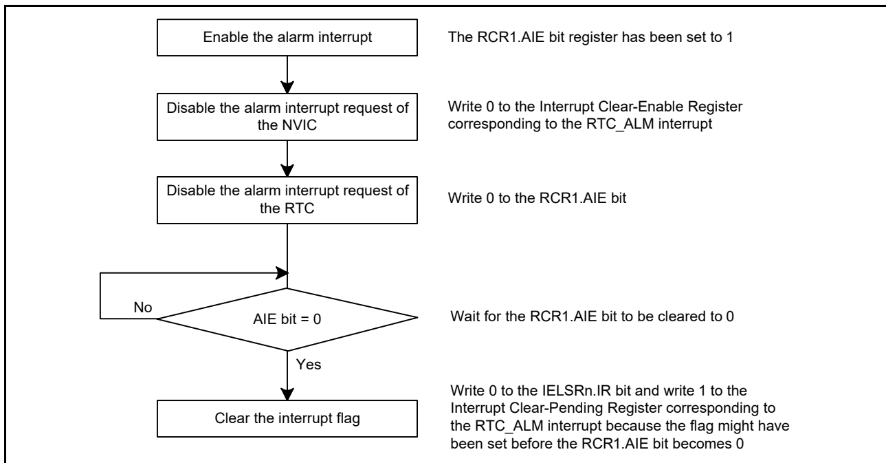
Figure 21.8 Procedure for disabling alarm interrupt request
