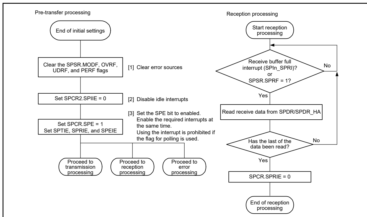
Figure 28.38 Reception flow in slave mode
