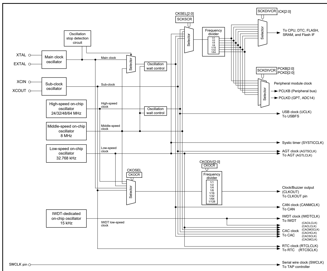
Figure 8.1 Clock generation circuit block diagram
