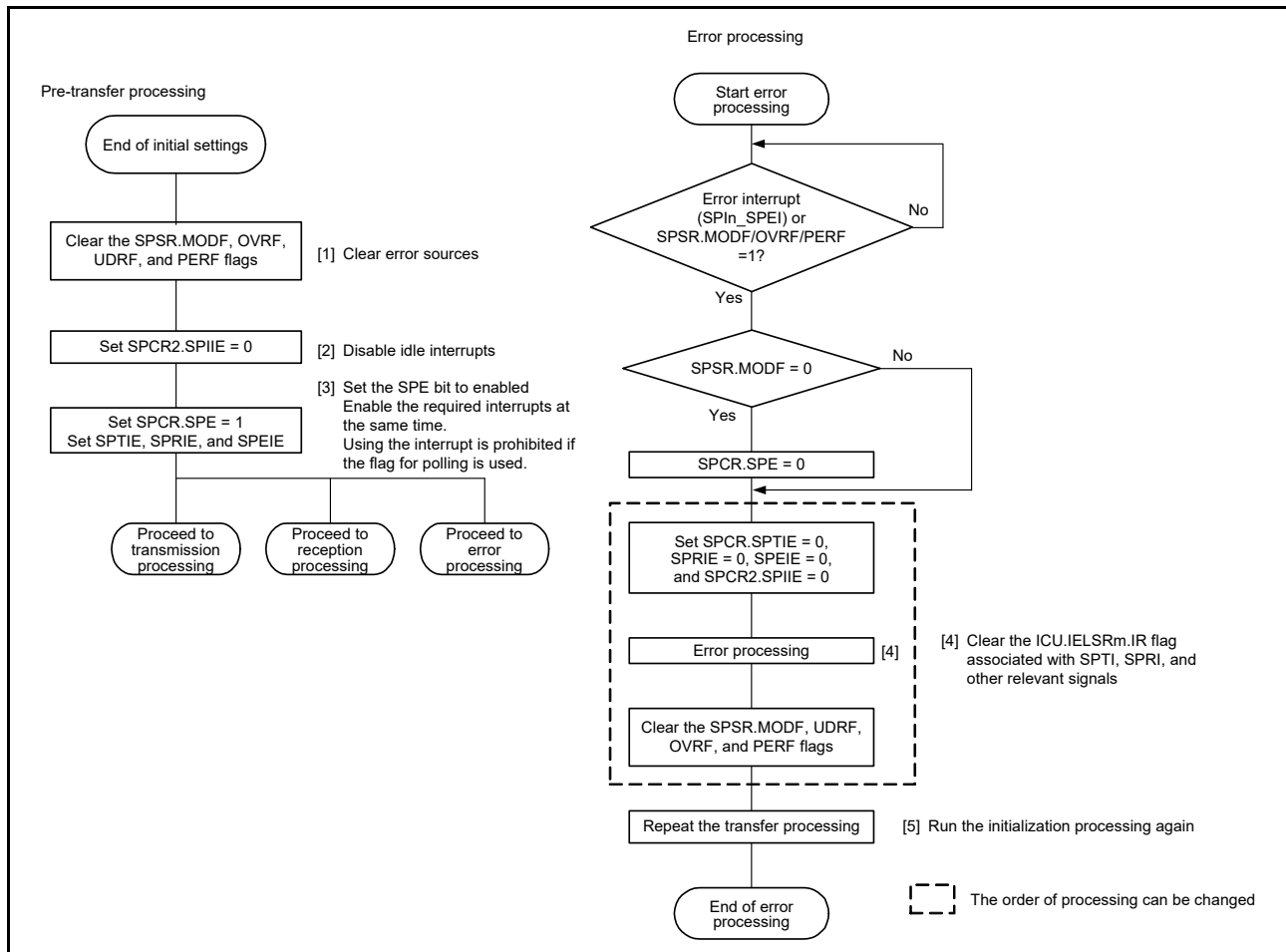
Figure 28.39 Error processing flow for slave mode
