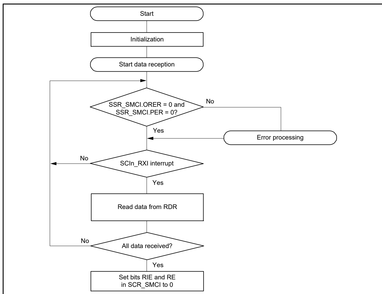
Figure 25.56 Example flow of smart card interface reception
