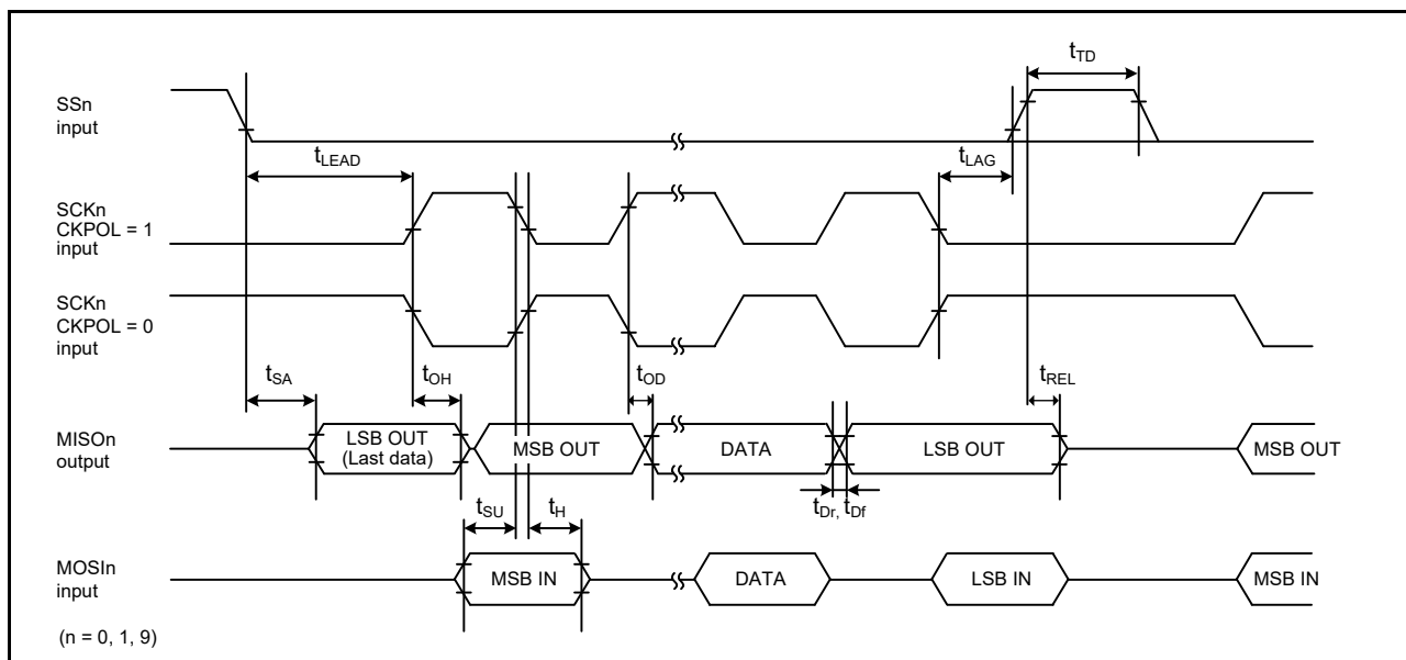
Figure 41.47 SCI simple SPI mode timing (slave, CKPH = 0)
