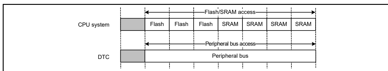
Figure 13.2 Example of parallel operations
