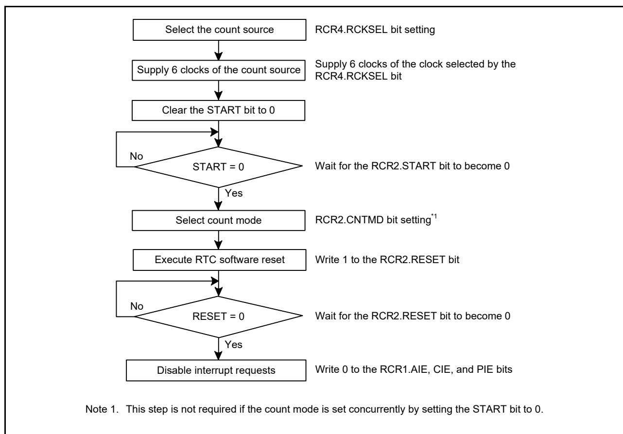
Figure 21.12 Initialization procedure
