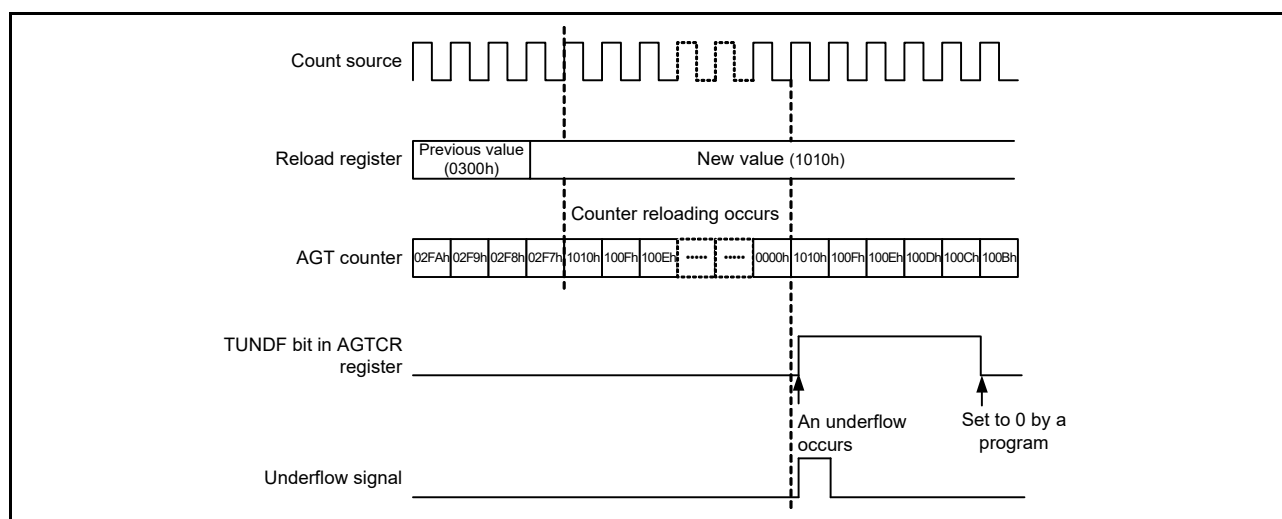
Figure 20.5 Operation example in timer mode
