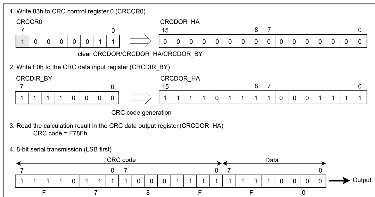
Figure 29.2 LSB-first data transmission
