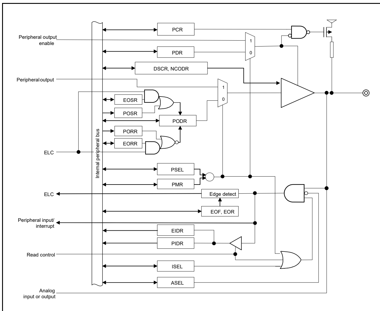
Figure 16.1 I/O Ports Registers connection diagram
