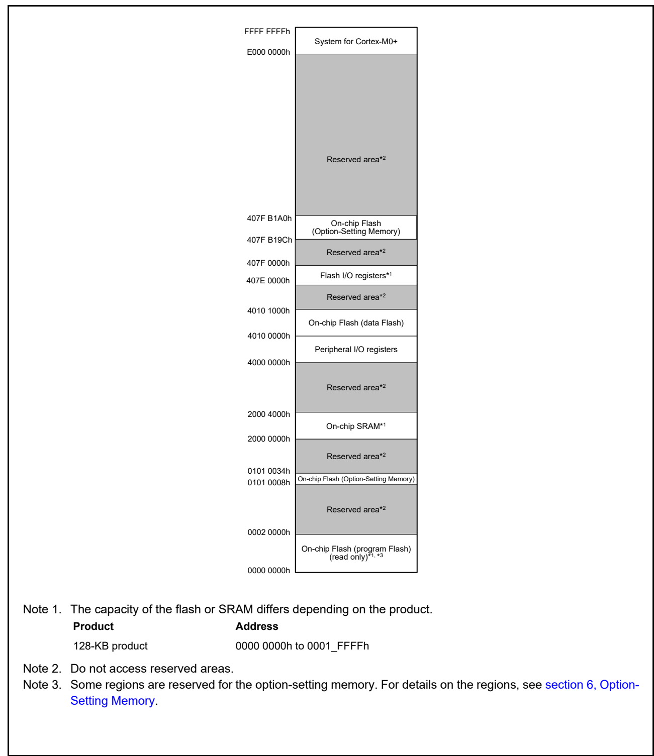
Figure 4.1 Memory map
