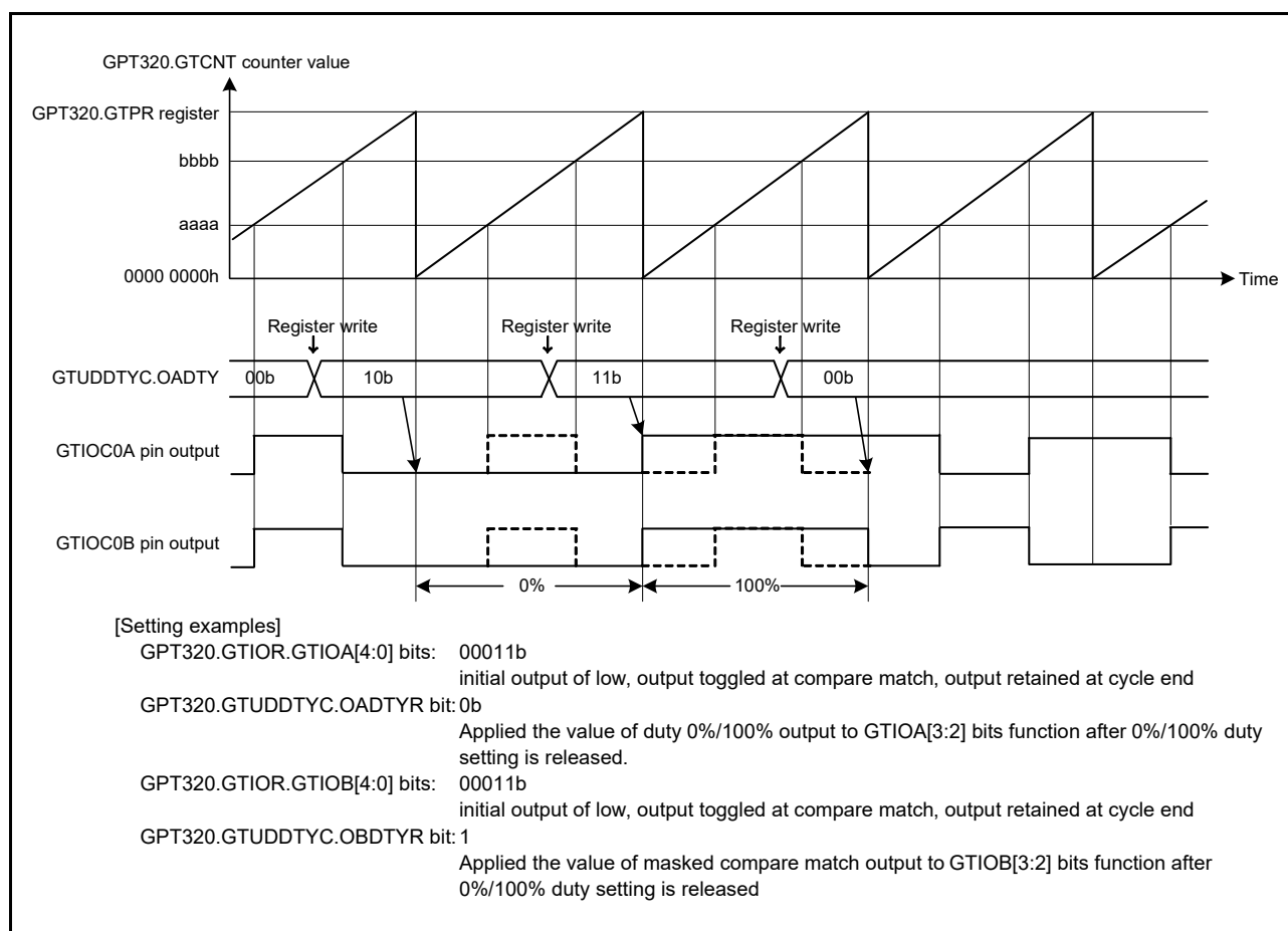
Figure 19.46 Example of output duty 0% and 100% function
