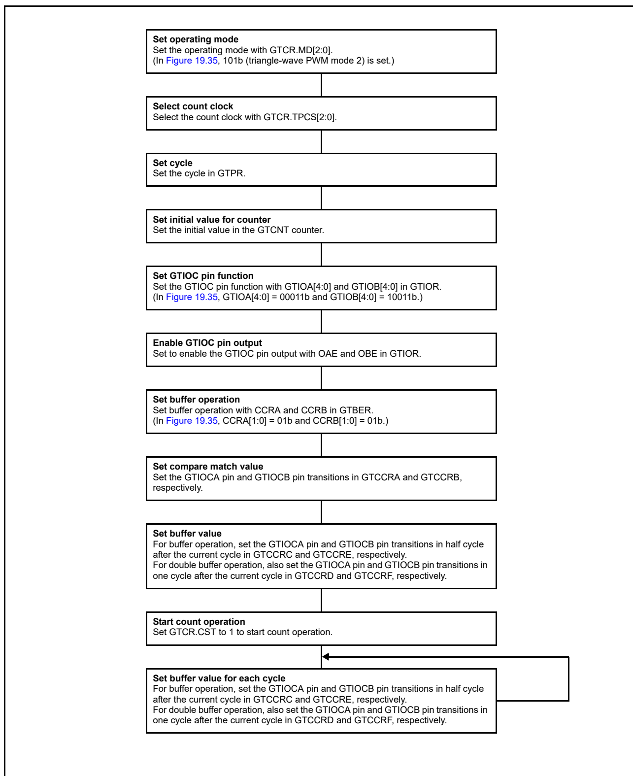
Figure 19.36 Example for setting triangle-wave PWM mode 2
