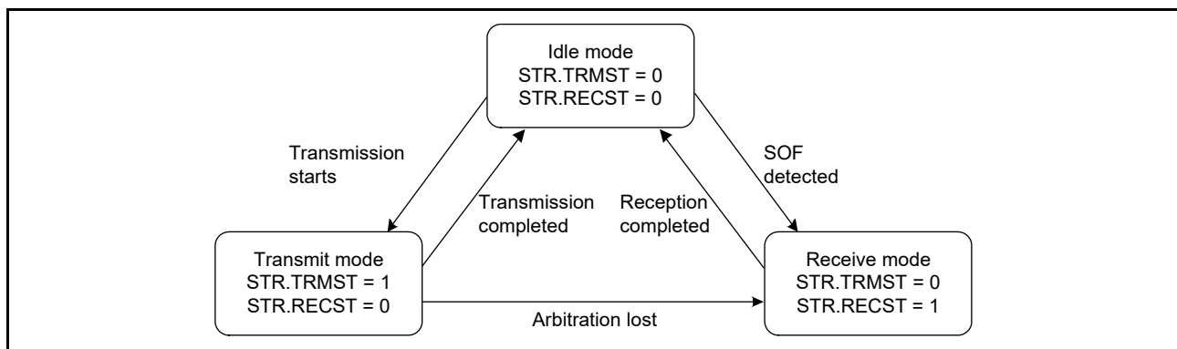
Figure 27.10 Sub-modes of CAN operation mode
