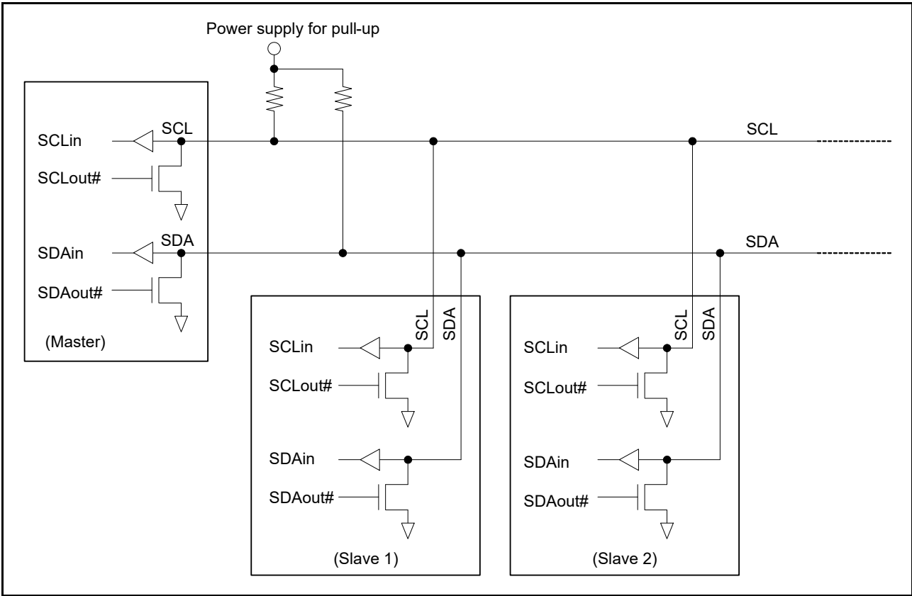
Figure 26.2 I/O pin connection to the external circuit (I 2 C bus configuration example)
