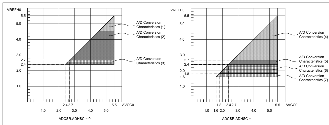
Figure 41.61 AVCC0 to VREFH0 voltage range
