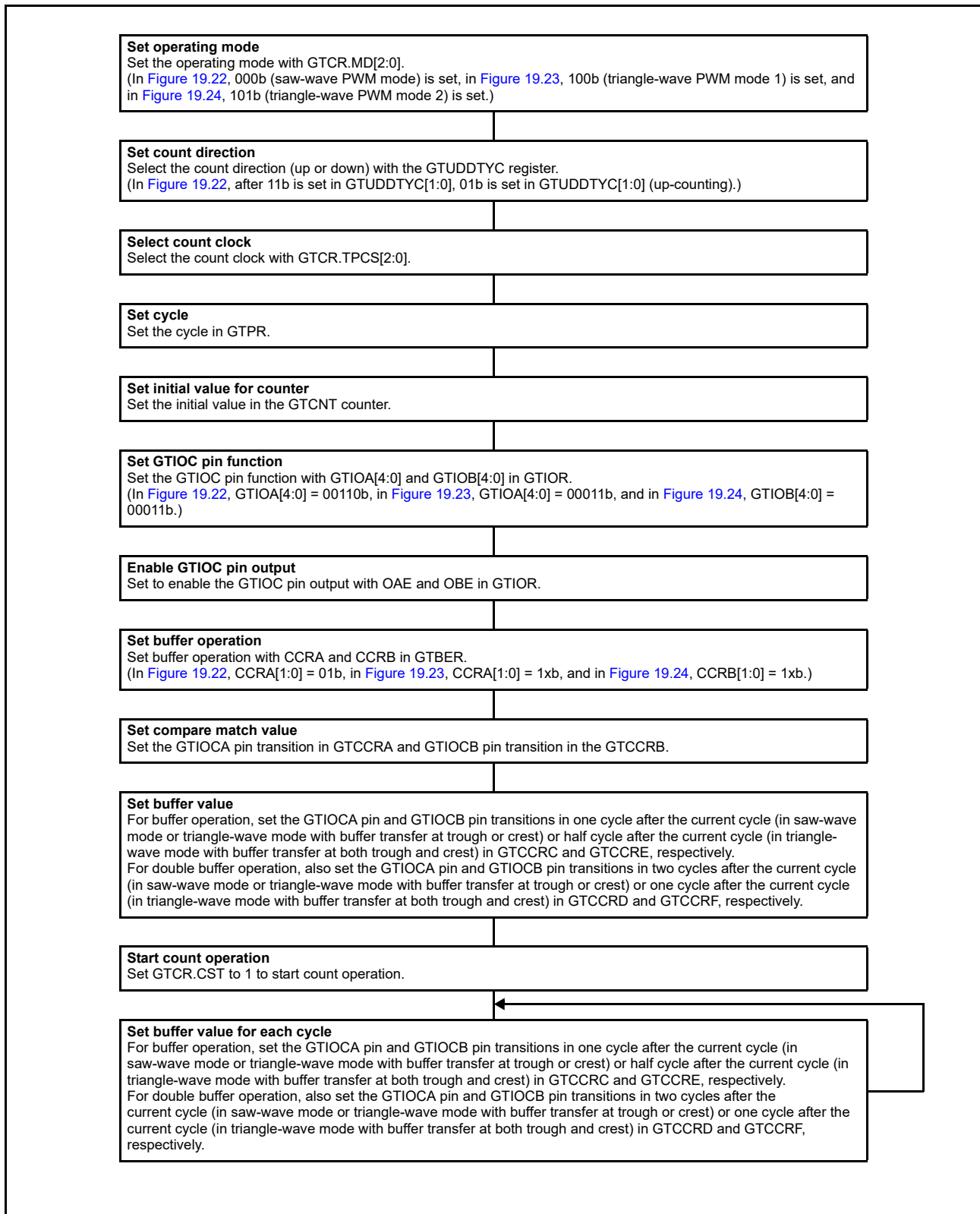
Figure 19.25 Example for setting GTCCRA and GTCCRB buffer operation for output compare
