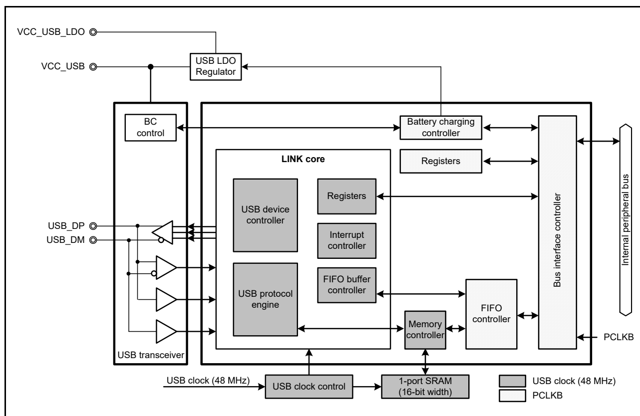
Figure 24.1 USBFS block diagram
