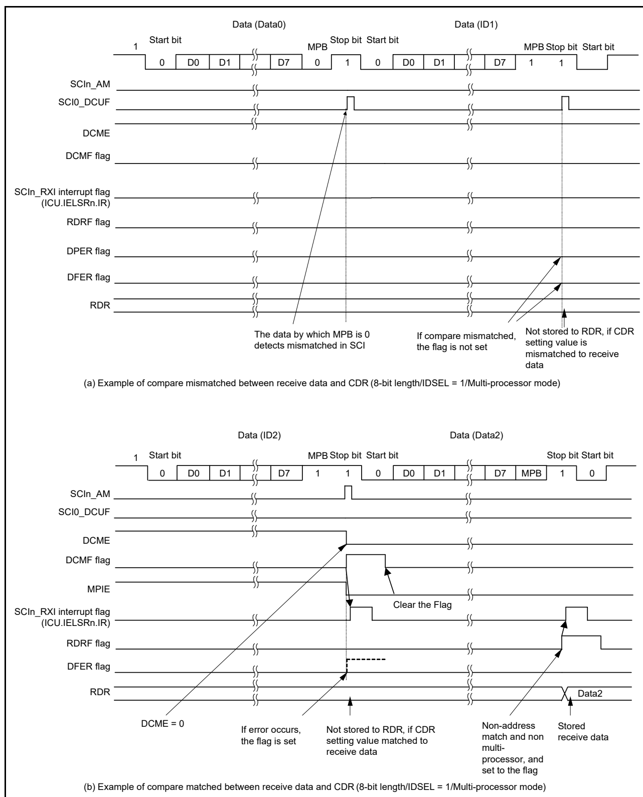
Figure 25.6 Example of address match (2) multi-processor mode
