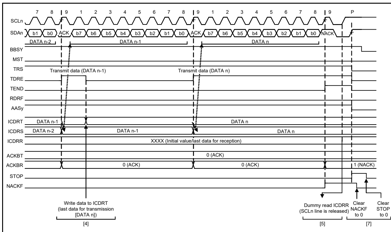
Figure 26.17 Slave transmit operation timing (2)
