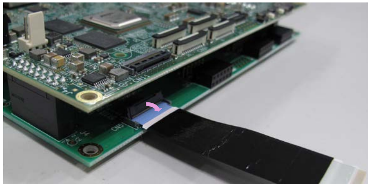
Figure 2.1-1 Connect FFC to RZ/V2H EVK Expansion Board
