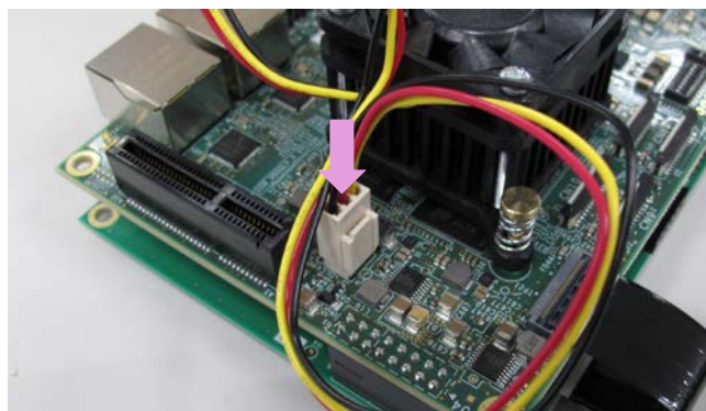
Figure 5.2-2 Connecting Power Supply of Heat-sink Fan
