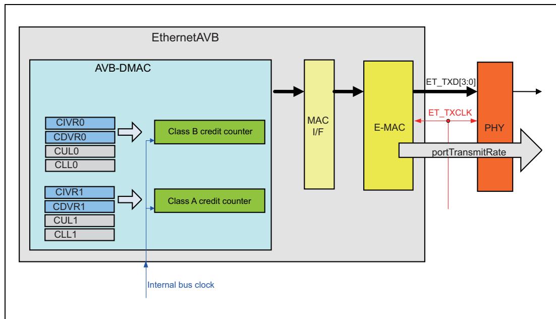
Figure 45.42 CBS (Credit-Based Shaping) Operation in the AVB-DMAC
