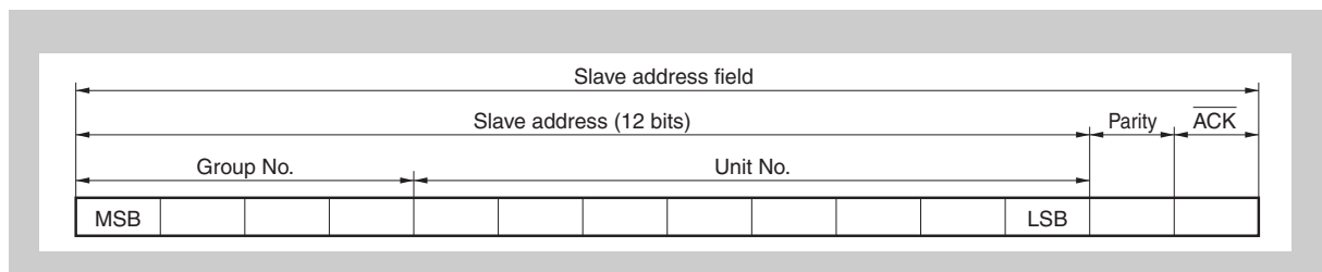
Figure 22-58 Slave address field
