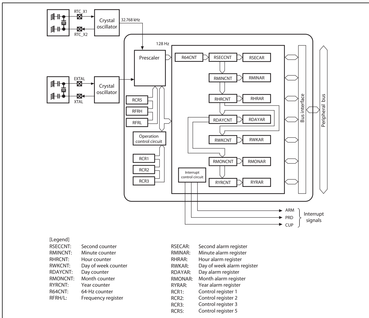
Figure 13.1 Block Diagram
