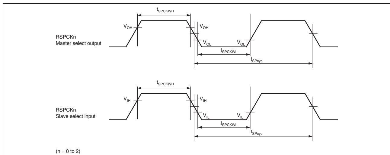
Figure 47.41 Clock Timing
