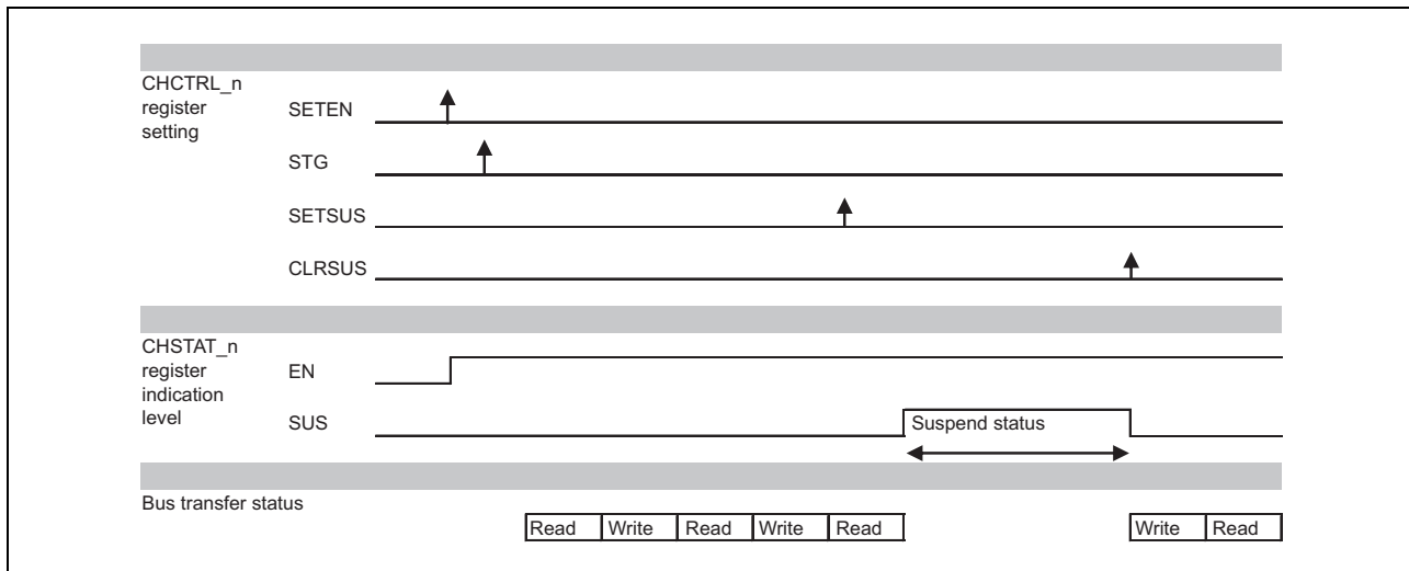
Figure 9.28 DMAC Suspend Status (Auto Request/Block Transfer)
