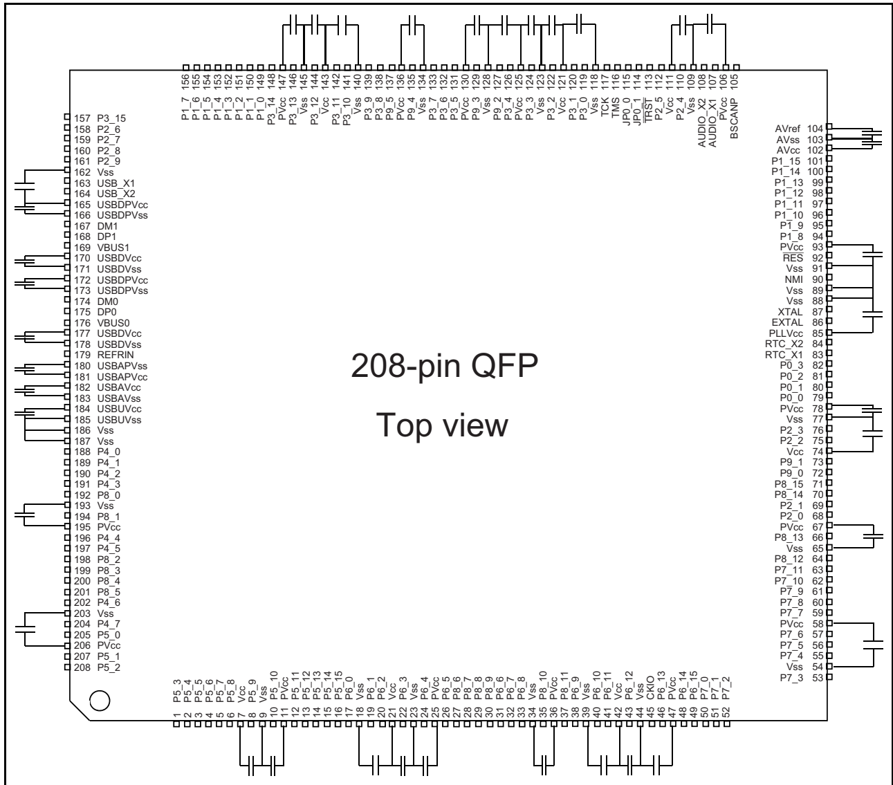
Figure 48.1 Example of Externally Allocated Capacitors in the Products in 208-Pin QFP Packages
