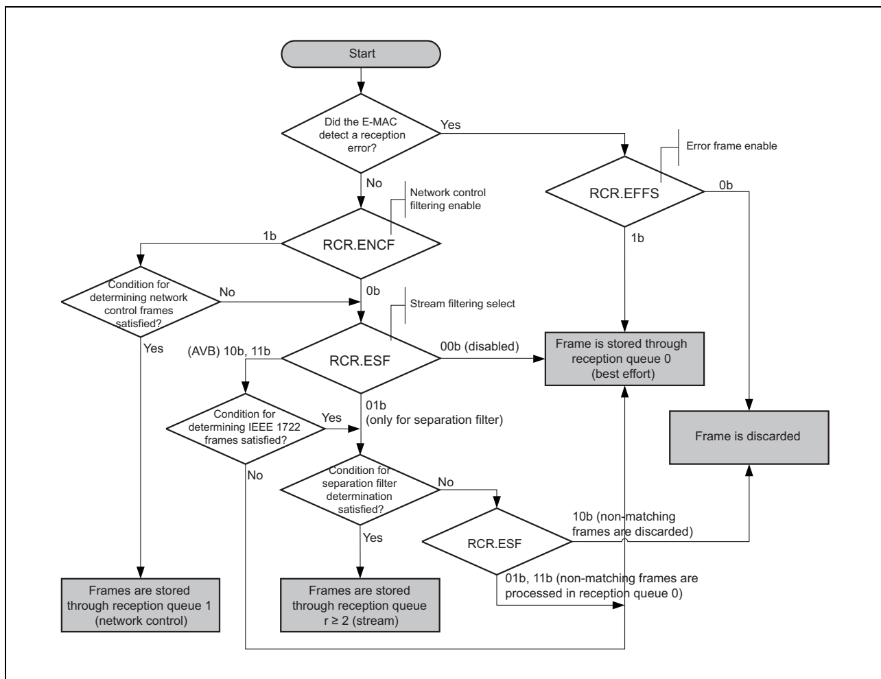
Figure 45.20 Flow of Reception Queue Selection
