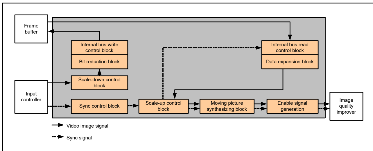
Figure 31.18 Signal Paths for Displaying Input Video Image
