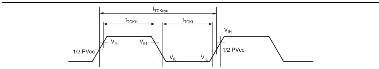
Figure 47.82 TCK Input Timing
