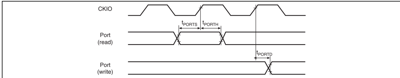
Figure 47.81 General I/O Ports Timing
