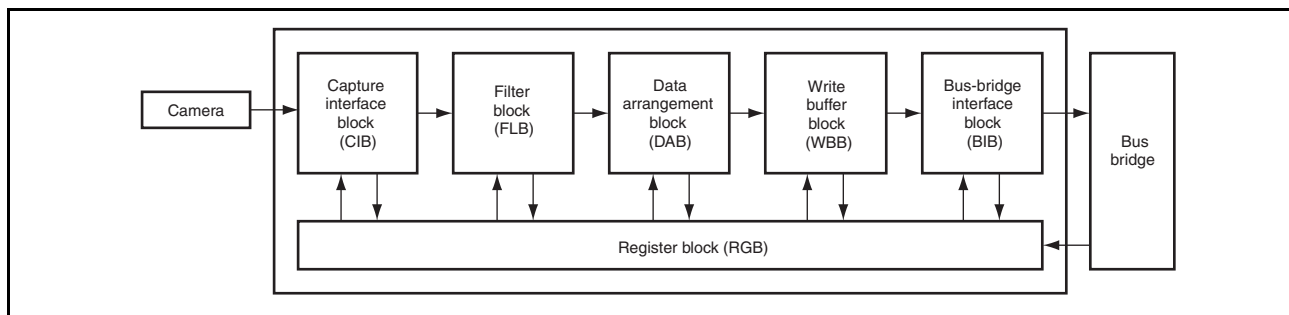
Figure 36.1 Block Diagram of CEU
