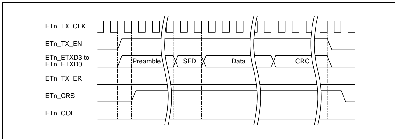
Figure 35.6 MII Frame Transmit Timing During Normal Transmission
