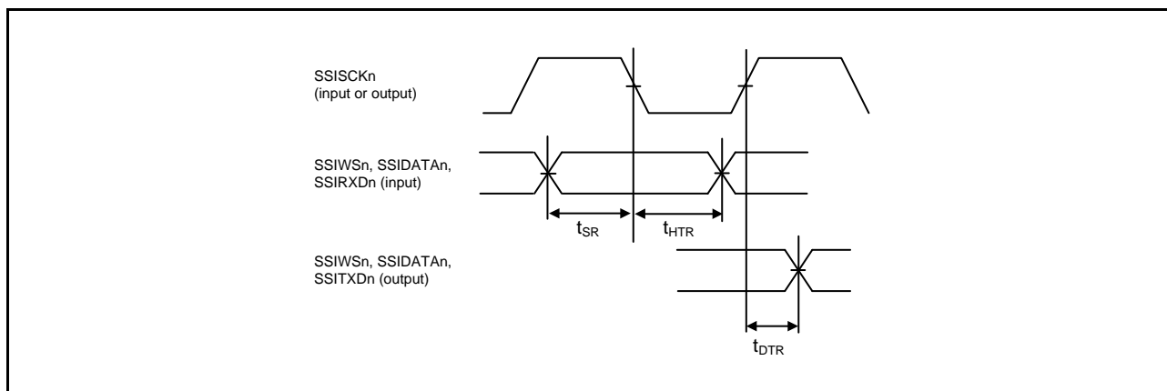
Figure 64.68 Transmit/Receive Timing (SSISCKn Falling Synchronous)
