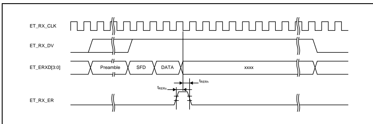
Figure 64.80 MII Reception Timing (Error Occurrence)
