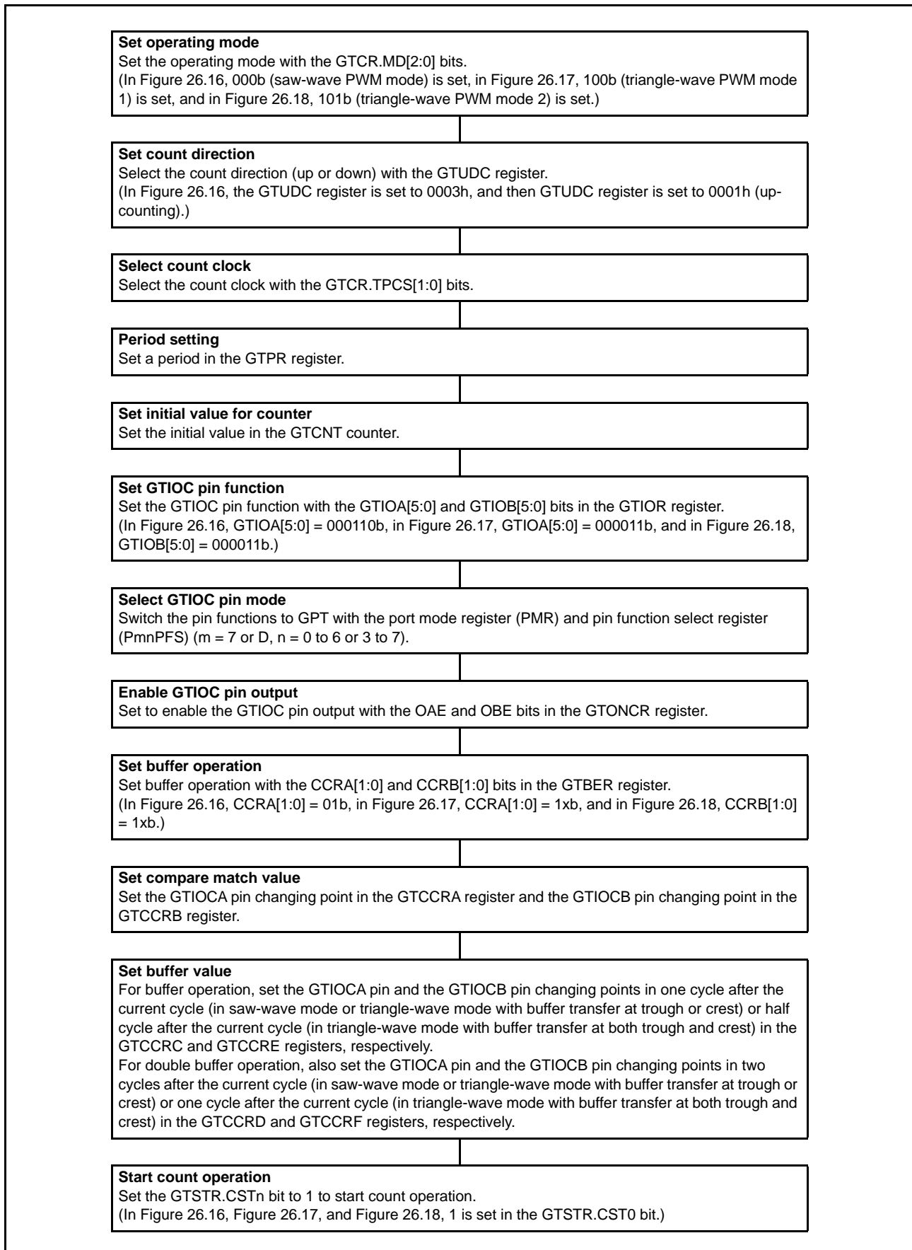
Figure 26.19 Example for Setting GTCRA and GTCRB Buffer Operation (for Output Compare)
