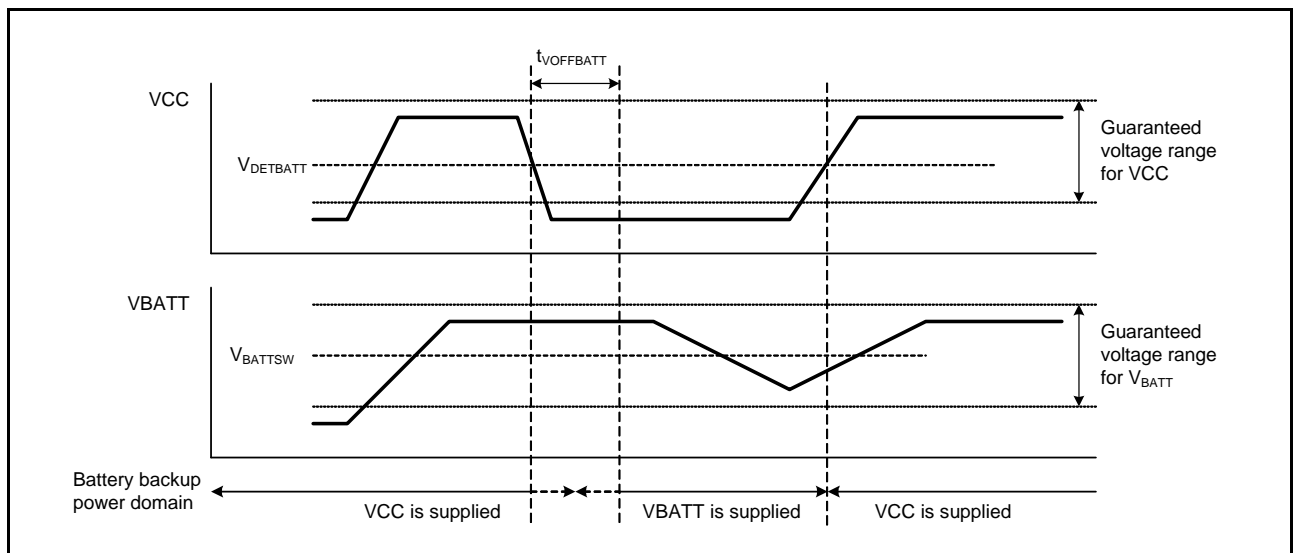
Figure 64.95 Battery Backup Function Characteristics
