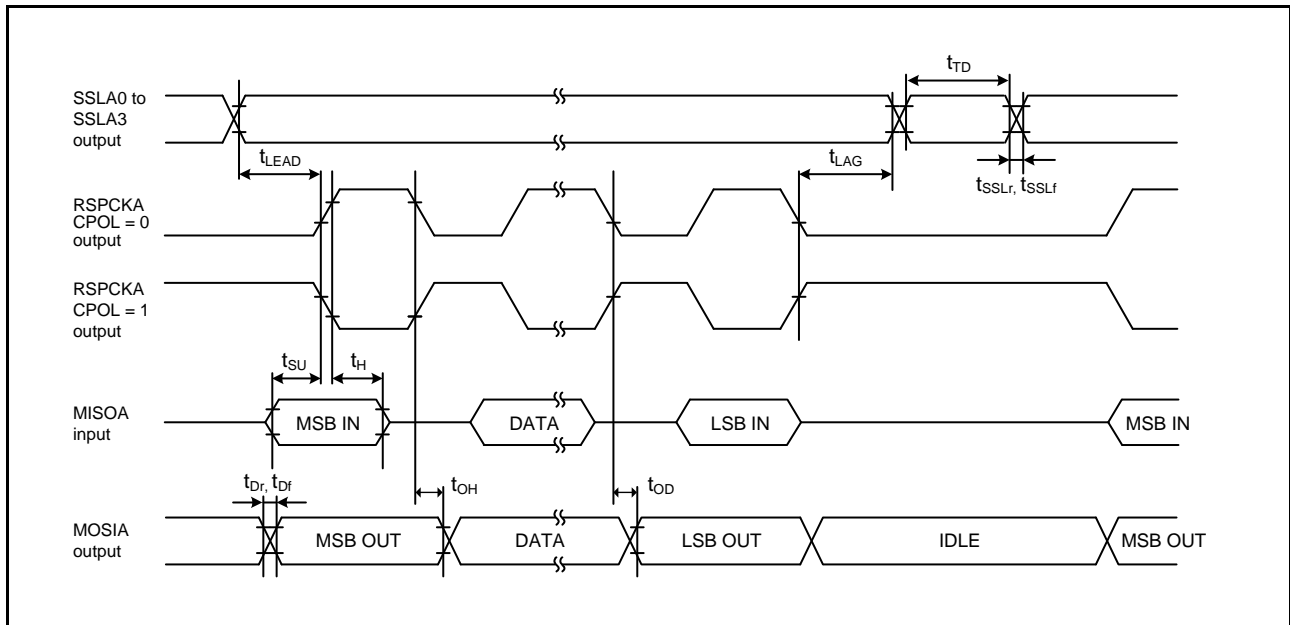
Figure 64.57 RSPCKA Timing (Master, CPHA = 0) (Bit Rate: PCLKB Division Ratio Set to a Value Other Than 1/2)
