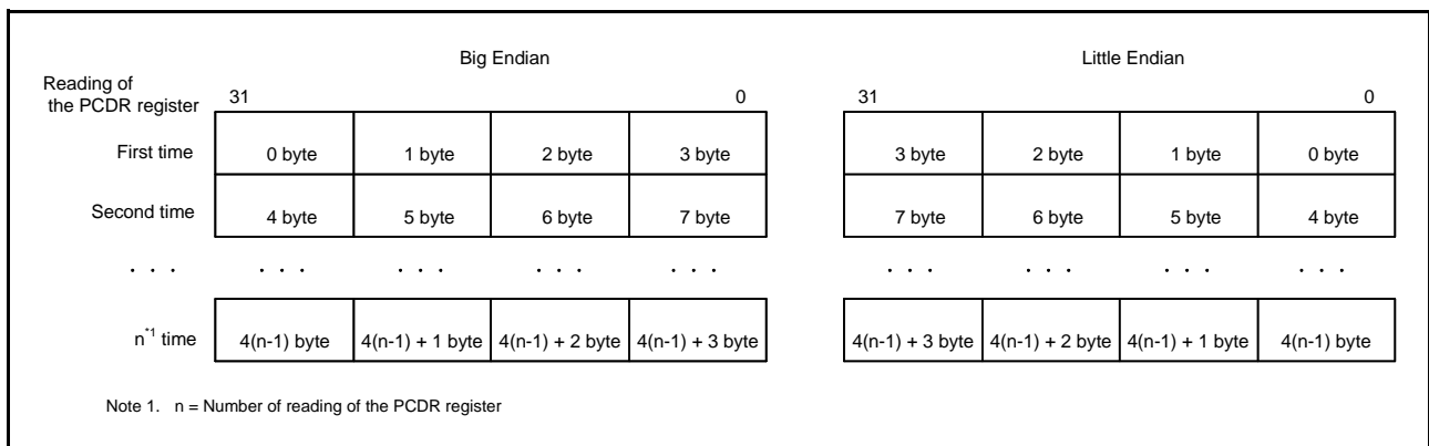
Figure 51.3 Endian Formats
