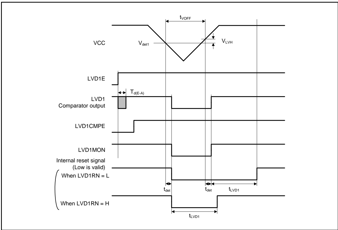
Figure 64.92 Voltage Detection Circuit Timing (V det1 )
