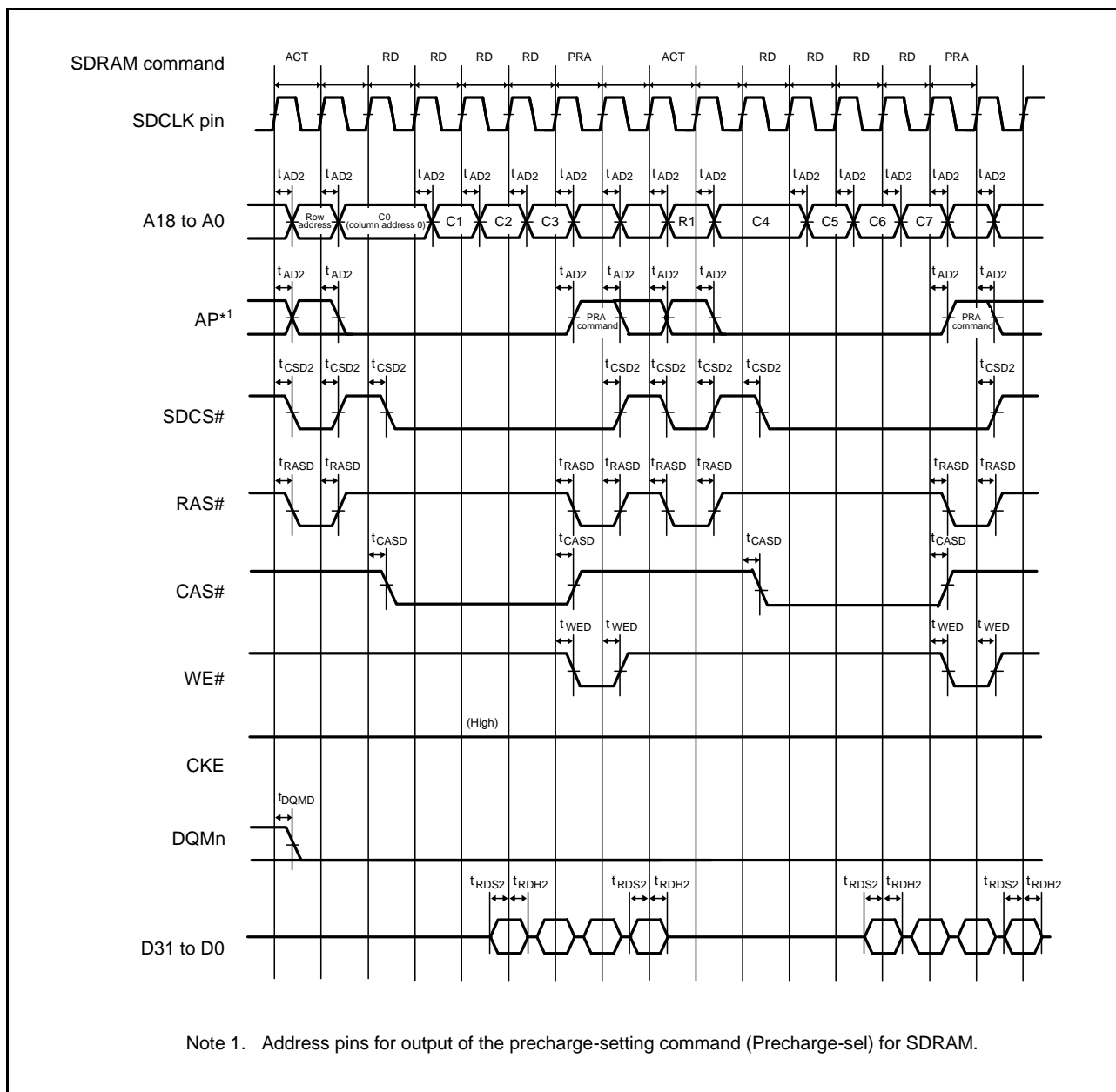
Figure 64.27 SDRAM Space Multiple Read Line Stride Bus Timing
