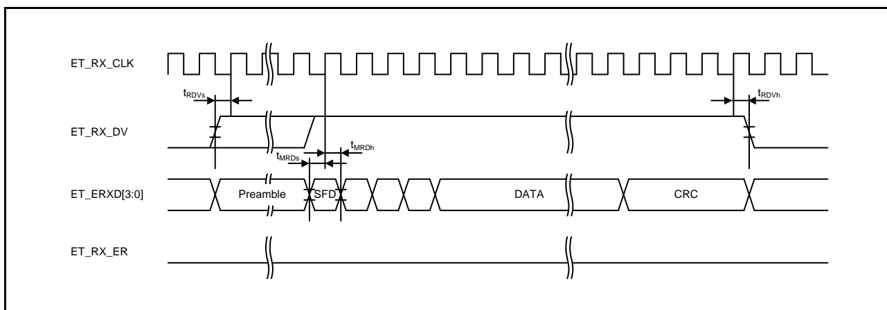
Figure 64.79 MII Reception Timing (Normal Operation)
