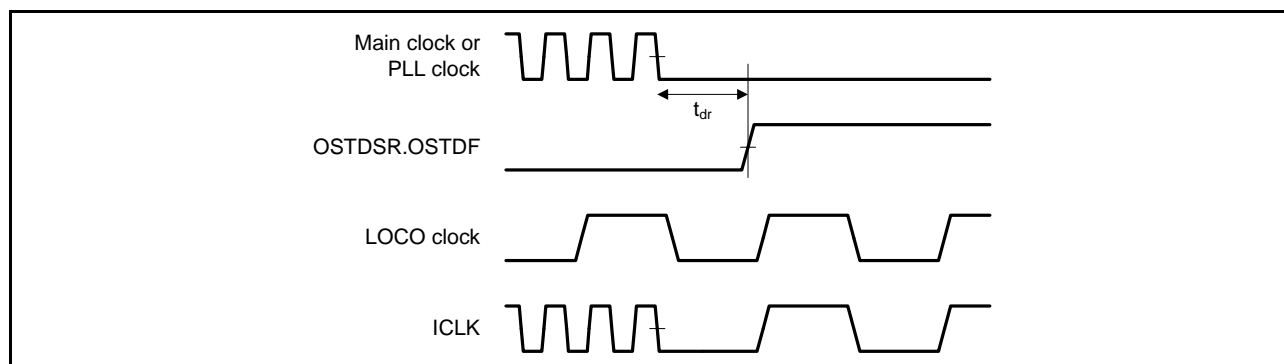
Figure 64.94 Oscillation Stop Detection Timing
