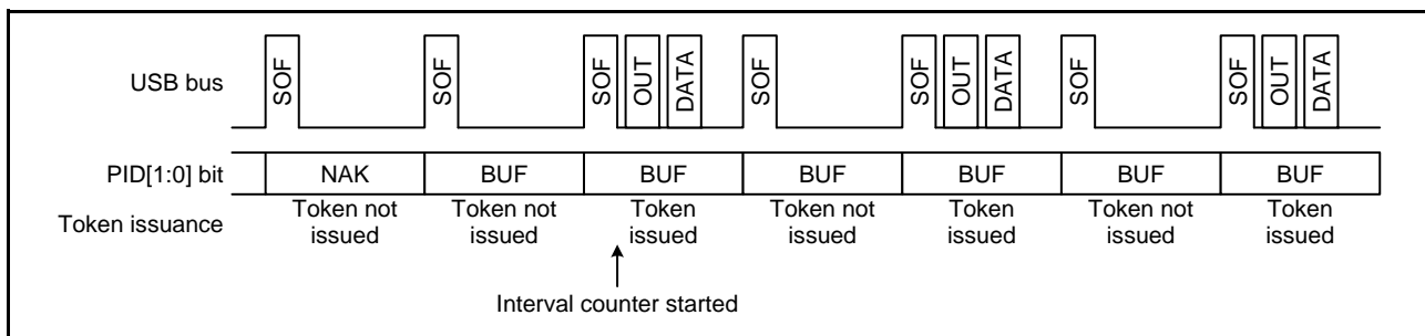
Figure 39.14 Token Issuance When IITV[2:0] Bits are 001b
