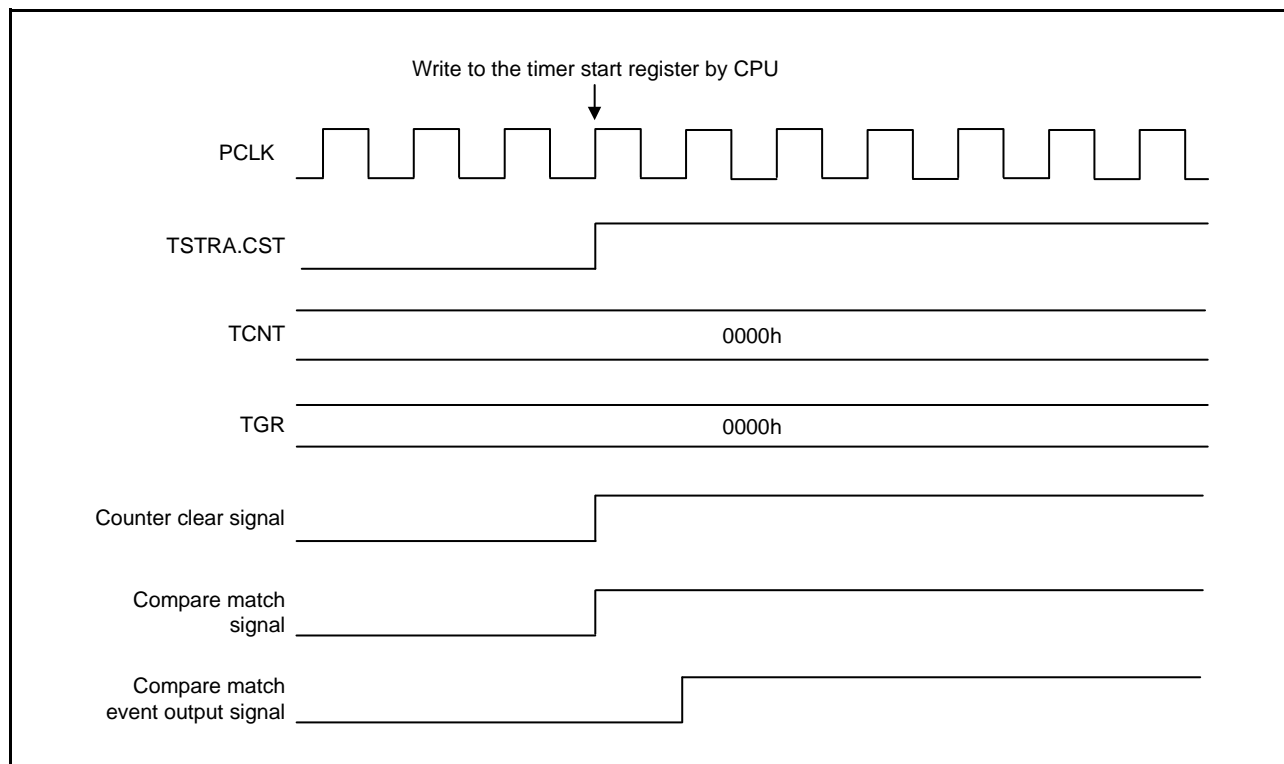
Figure 27.63 Continuous Output of the Compare Match Event Output Signal
