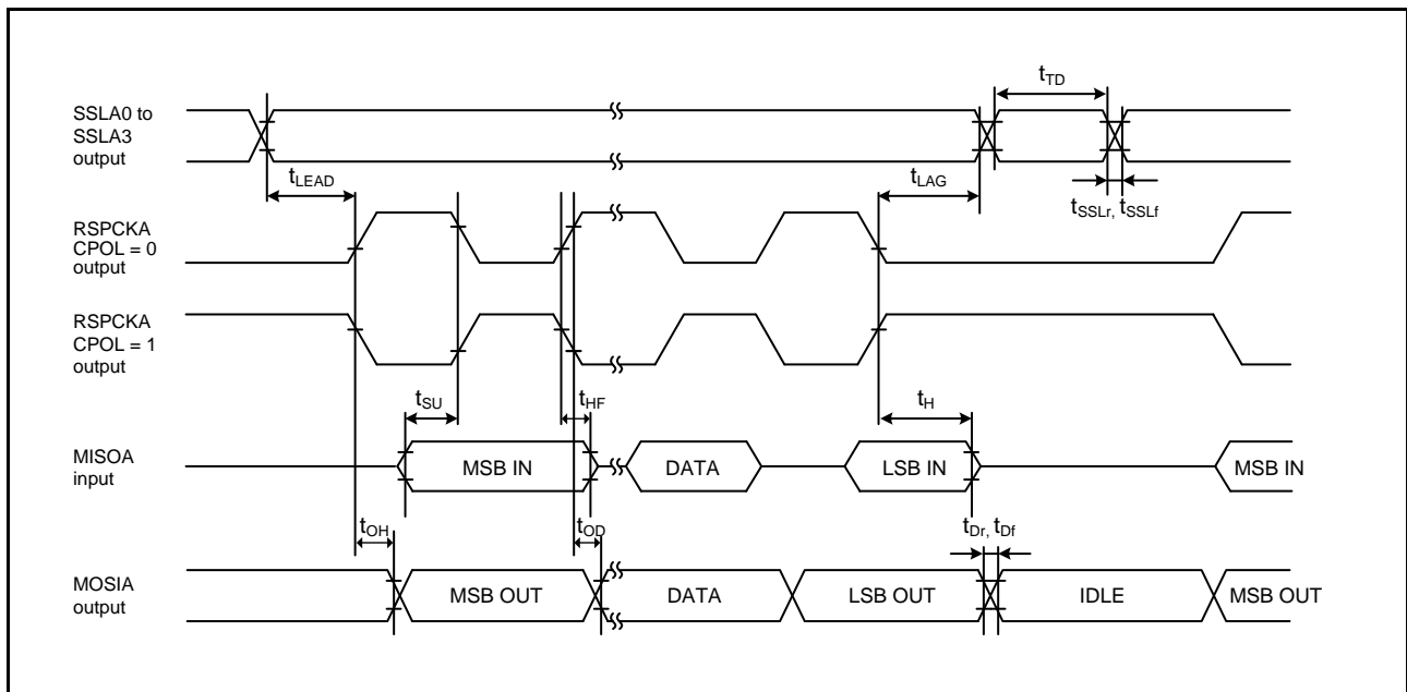
Figure 64.60 RSPI Timing (Master, CPHA = 1) (Bit Rate: PCLKB Division Ratio Set to 1/2)
