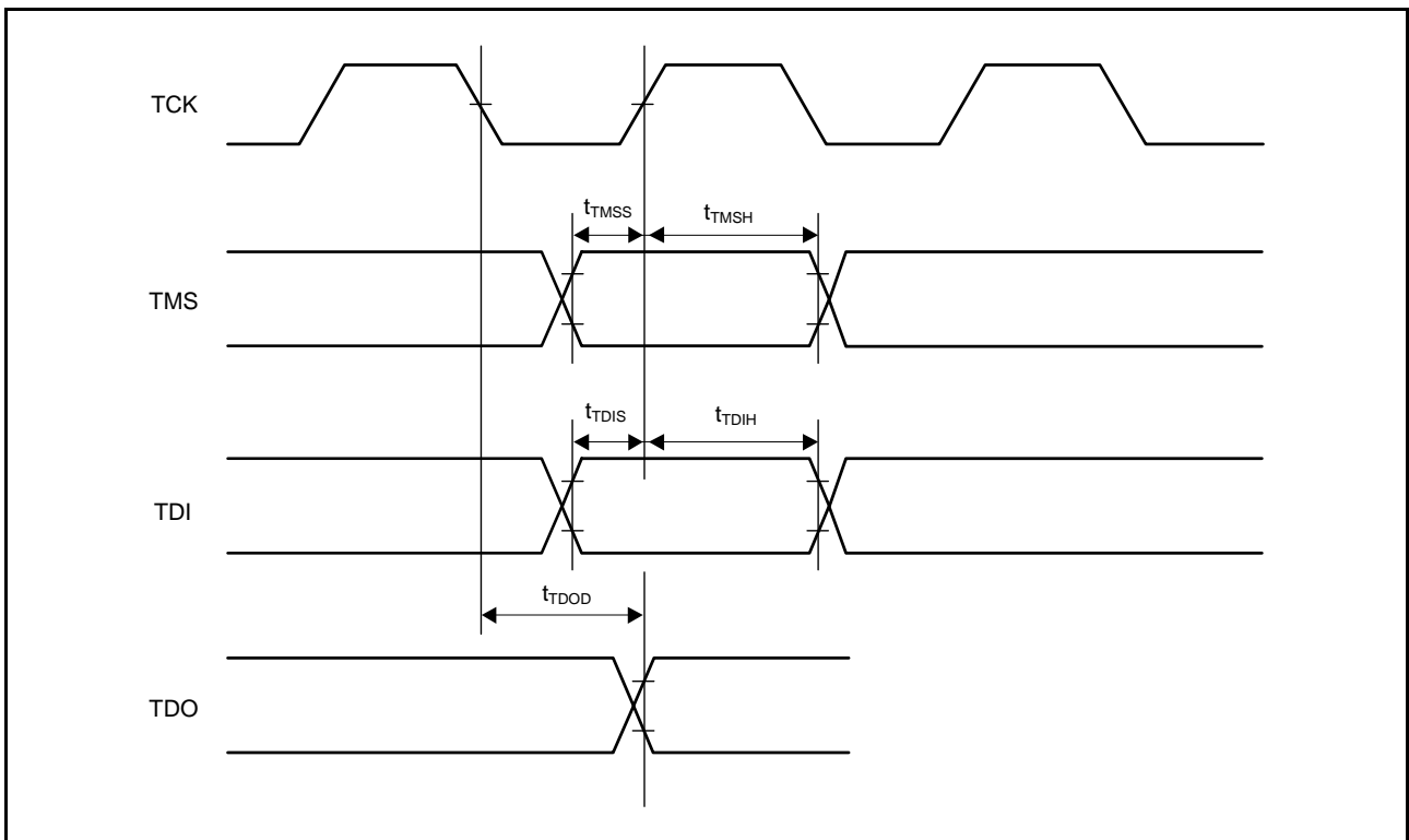
Figure 64.99 Boundary Scan Input/Output Timing
