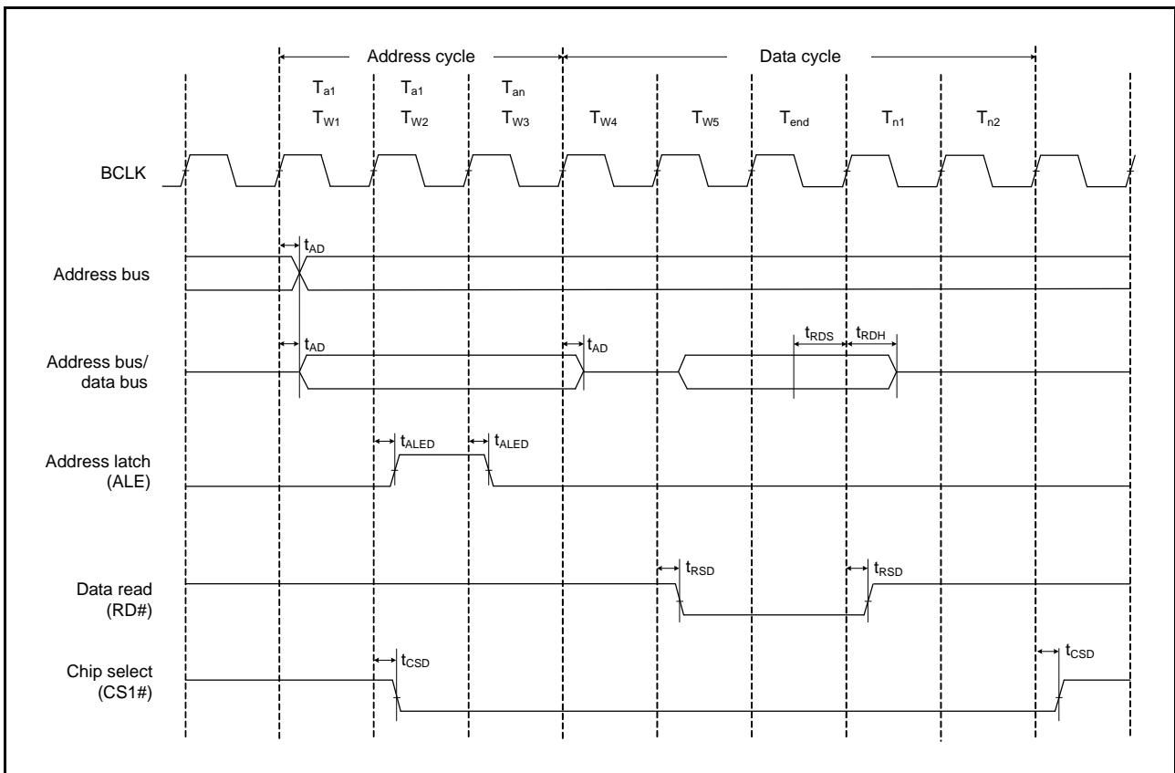
Figure 64.16 Address/Data Multiplexed Bus Read Access Timing
