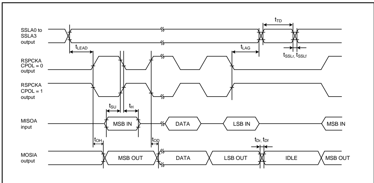
Figure 64.59 RSPI Timing (Master, CPHA = 1) (Bit Rate: PCLKB Division Ratio Set to a Value Other Than 1/2)
