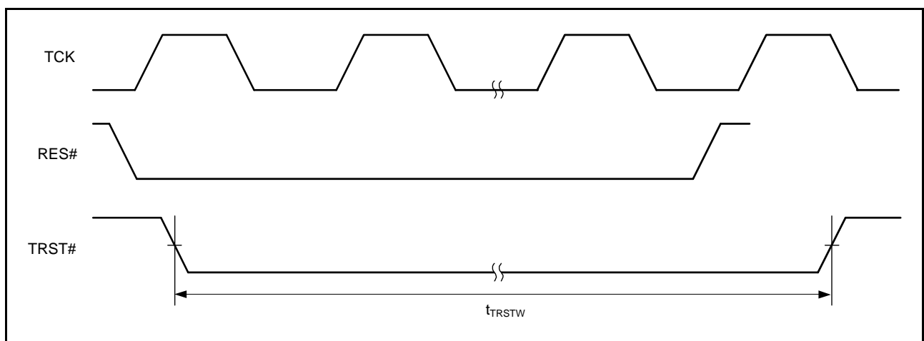
Figure 64.98 Boundary Scan TRST# Timing
