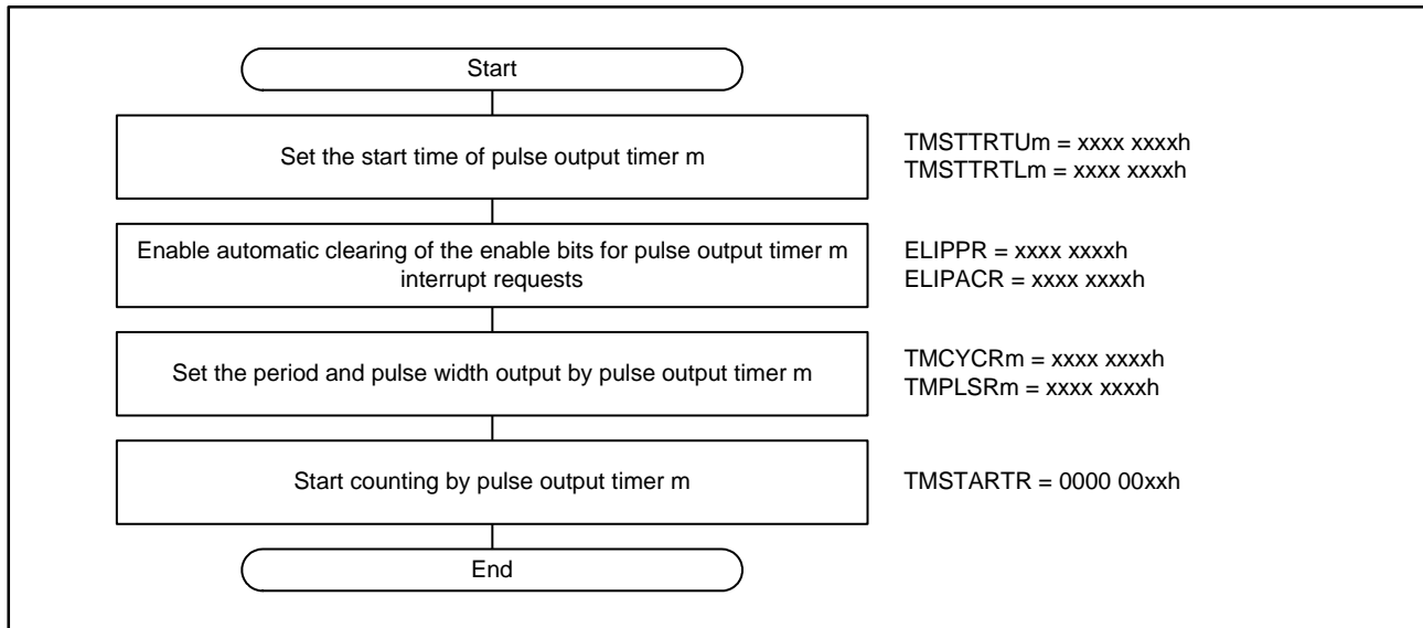
Figure 36.33 Procedure for Setting a Pulse Output Timer
