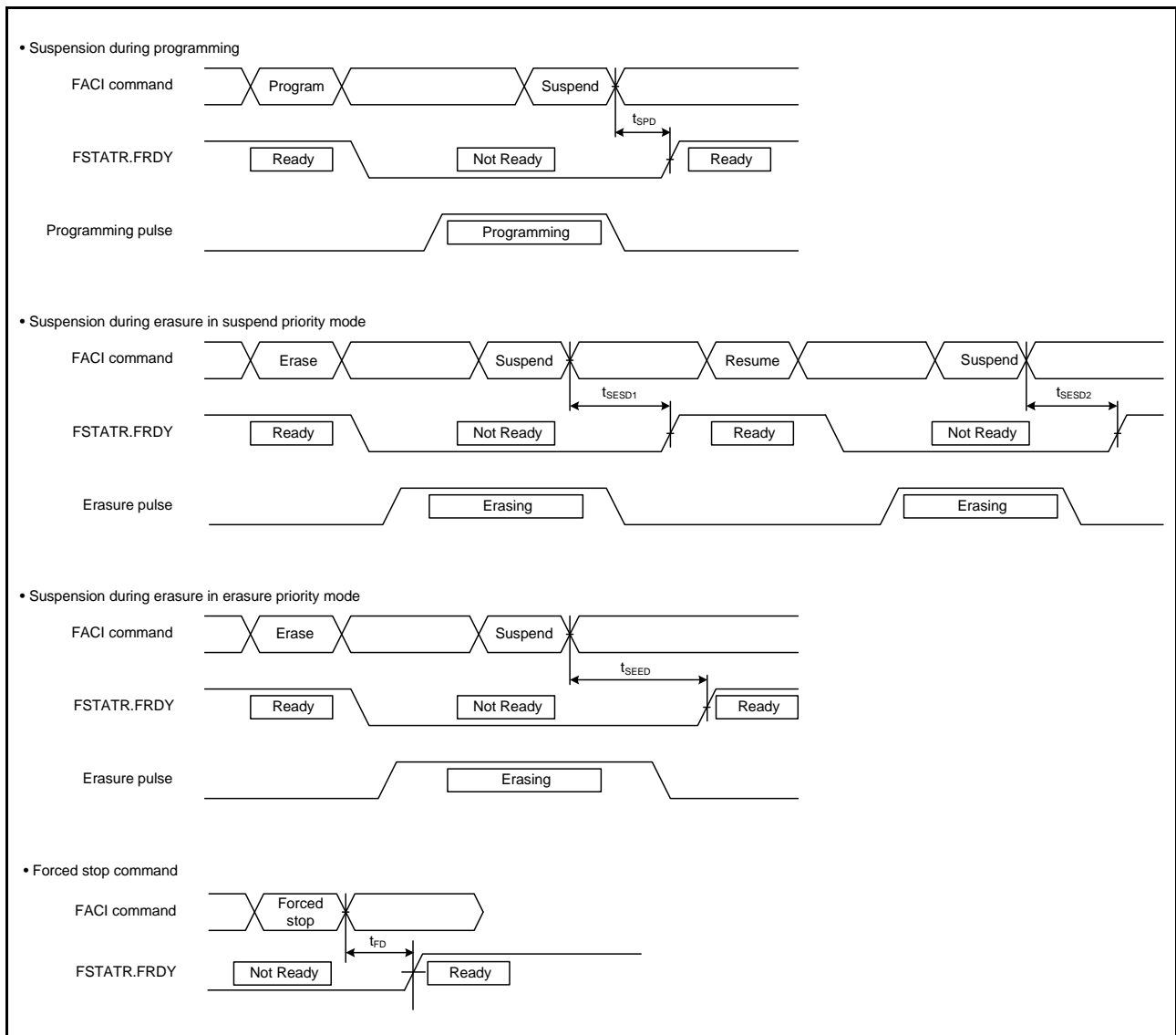
Figure 64.96 Flash Memory Programming/Erasure Suspension Timing
