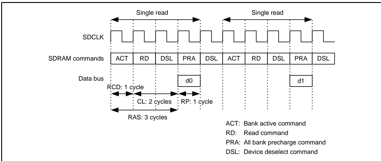
Figure 16.71 Timing Example of Single Read (4)
