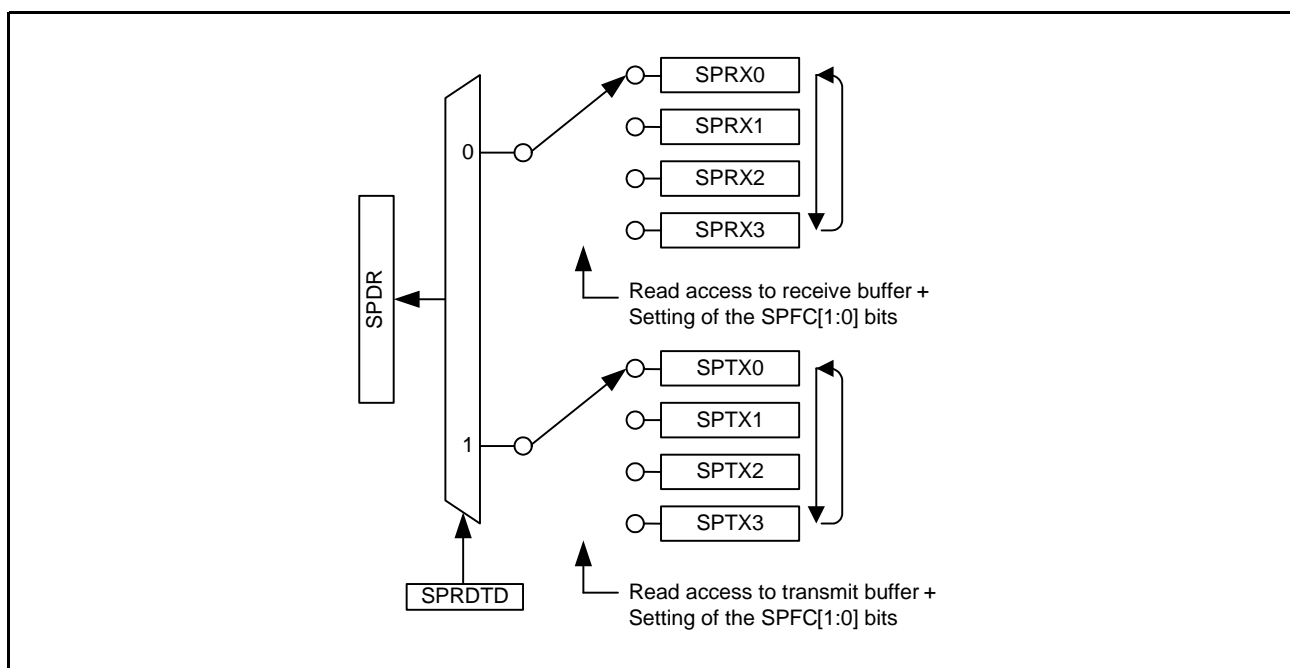
Figure 44.4 Configuration of the SPDR Register (Reading)
