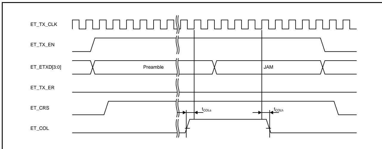
Figure 64.78 MII Transmission Timing (Conflict Occurrence)
