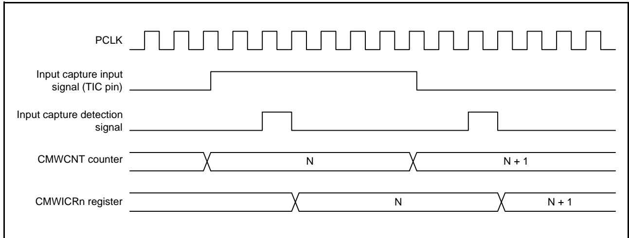
Figure 31.12 Input Capture Timing (Unit 0, Both-Edge Detection) (n = 0, 1)
