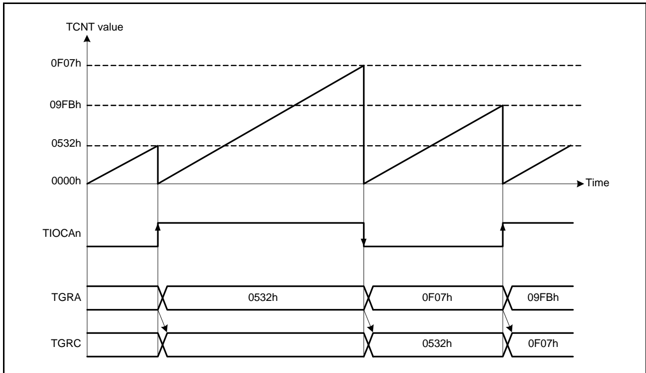
Figure 27.16 Example of Buffer Operation (2) (n = 0 to 5)
