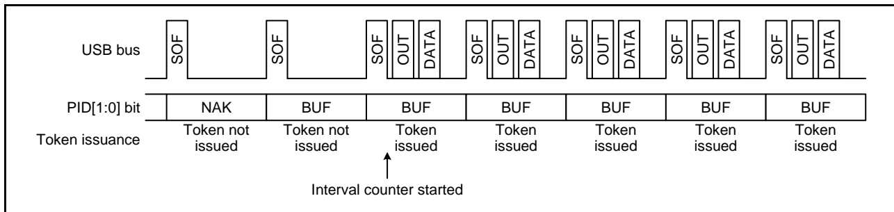
Figure 39.13 Token Issuance When IITV[2:0] Bits are 000b
