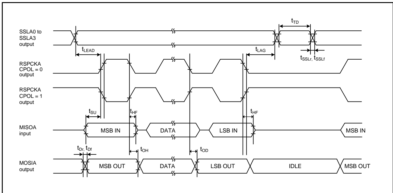
Figure 64.58 RSPI Timing (Master, CPHA = 0) (Bit Rate: PCLKB Division Ratio Set to 1/2)
