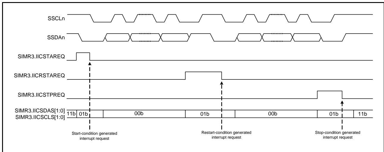
Figure 40.48 Timing of Operations in the Generation of Start, Restart, and Stop Conditions
