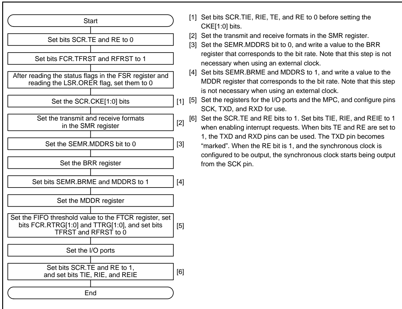
Figure 41.13 SCIFA Initialization in Clock Synchronous Mode
