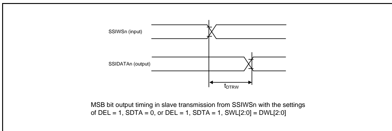
Figure 64.69 SSIDATA Output Delay from SSIWSn Change Edge
