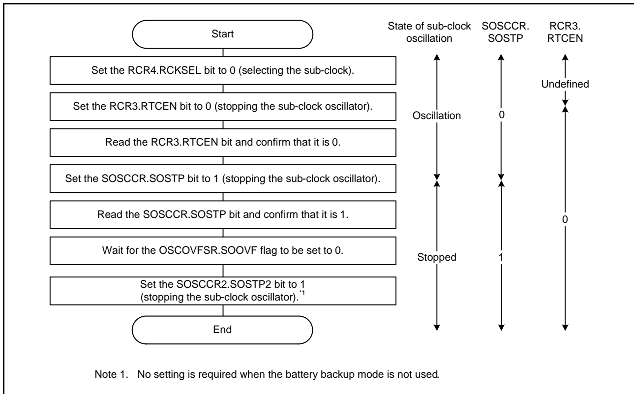
Figure 9.13 Example Flowchart for when the Sub-Clock is not to be Used
