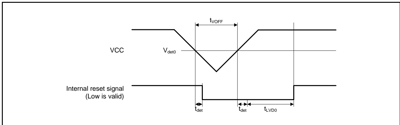
Figure 64.91 Voltage Detection Circuit Timing ( V_{det0} )
