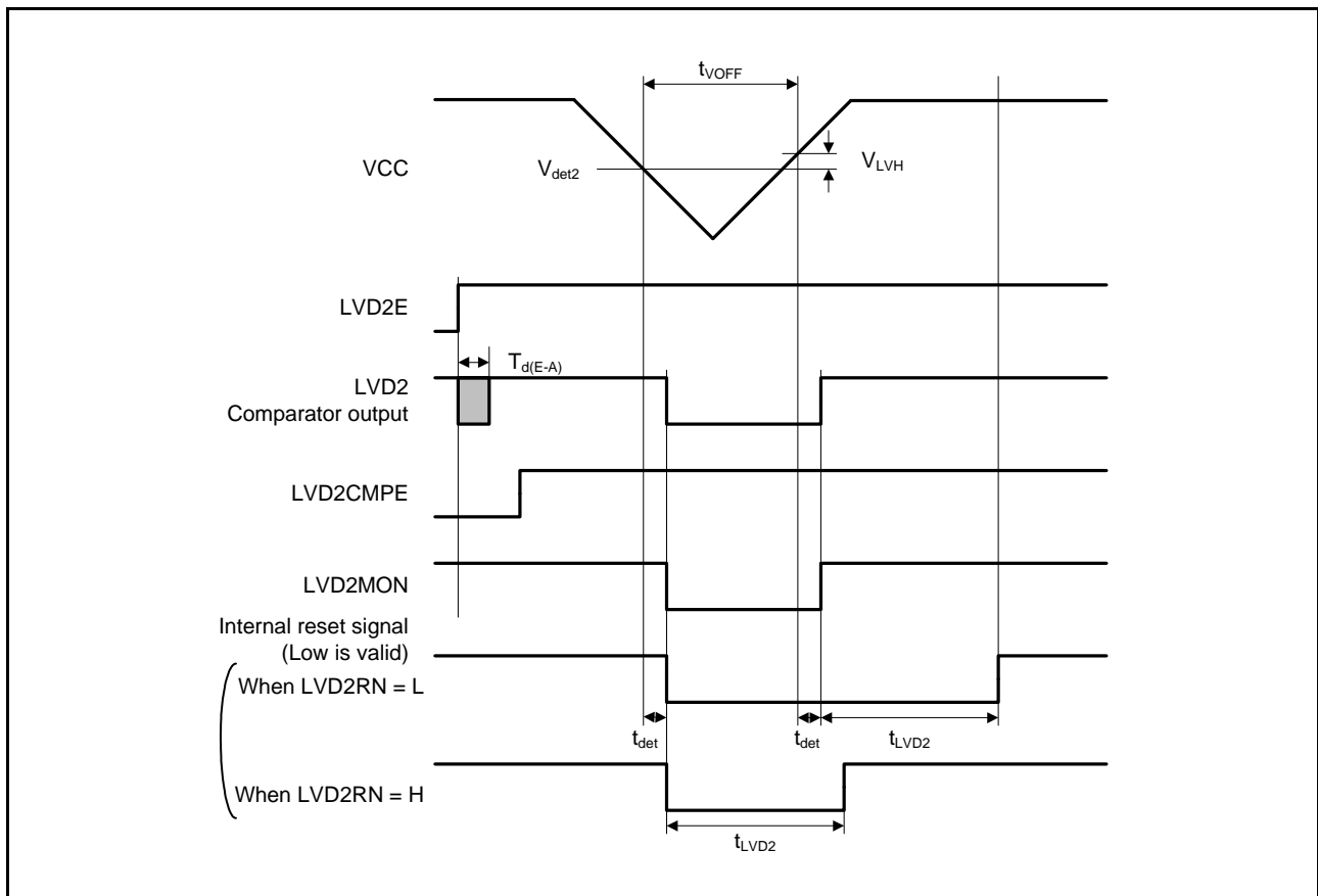
Figure 64.93 Voltage Detection Circuit Timing (V det2 )
