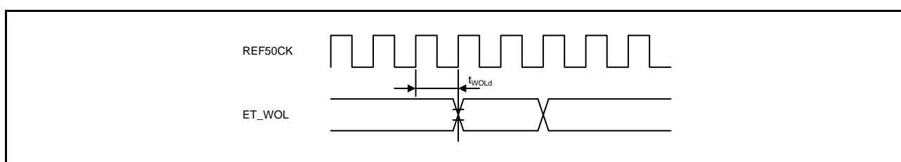
Figure 64.76 WOL Output Timing (RMII)
