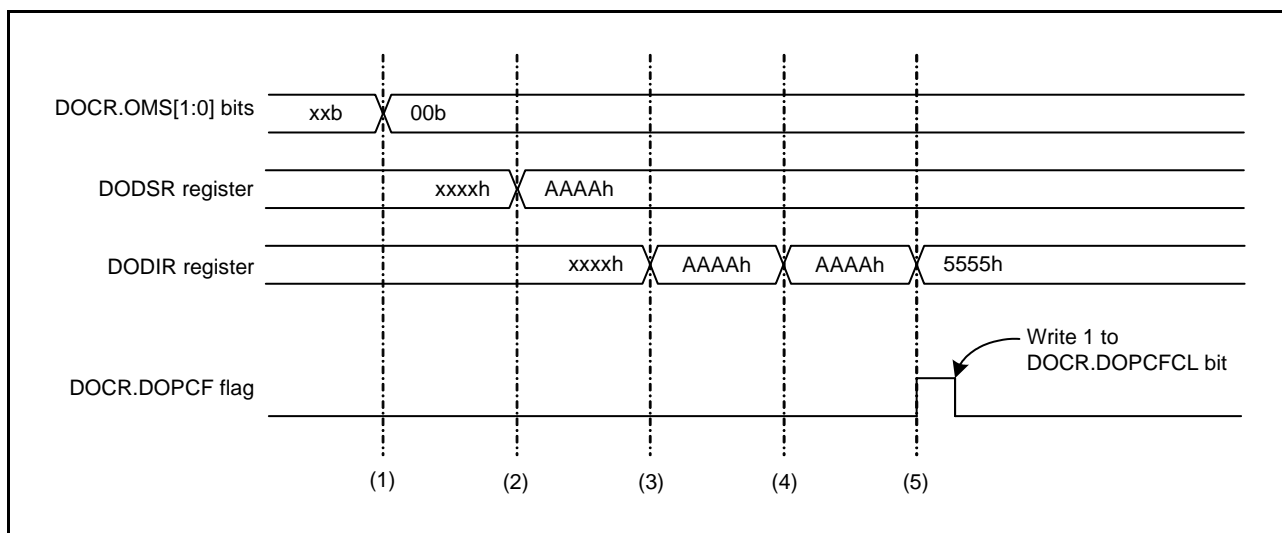
Figure 60.2 Example of Operation in Data Comparison Mode
