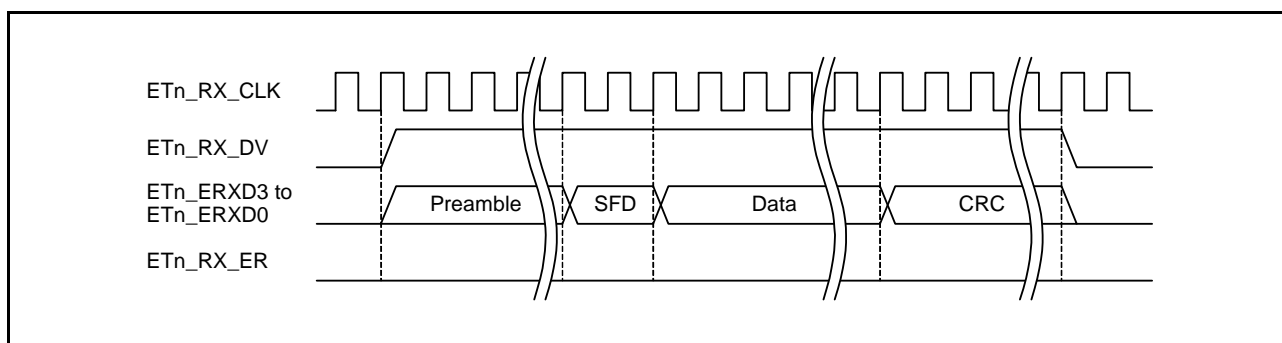
Figure 35.8 MII Frame Receive Timing During Normal Reception
