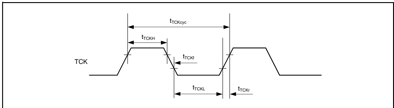
Figure 64.97 Boundary Scan TCK Timing
