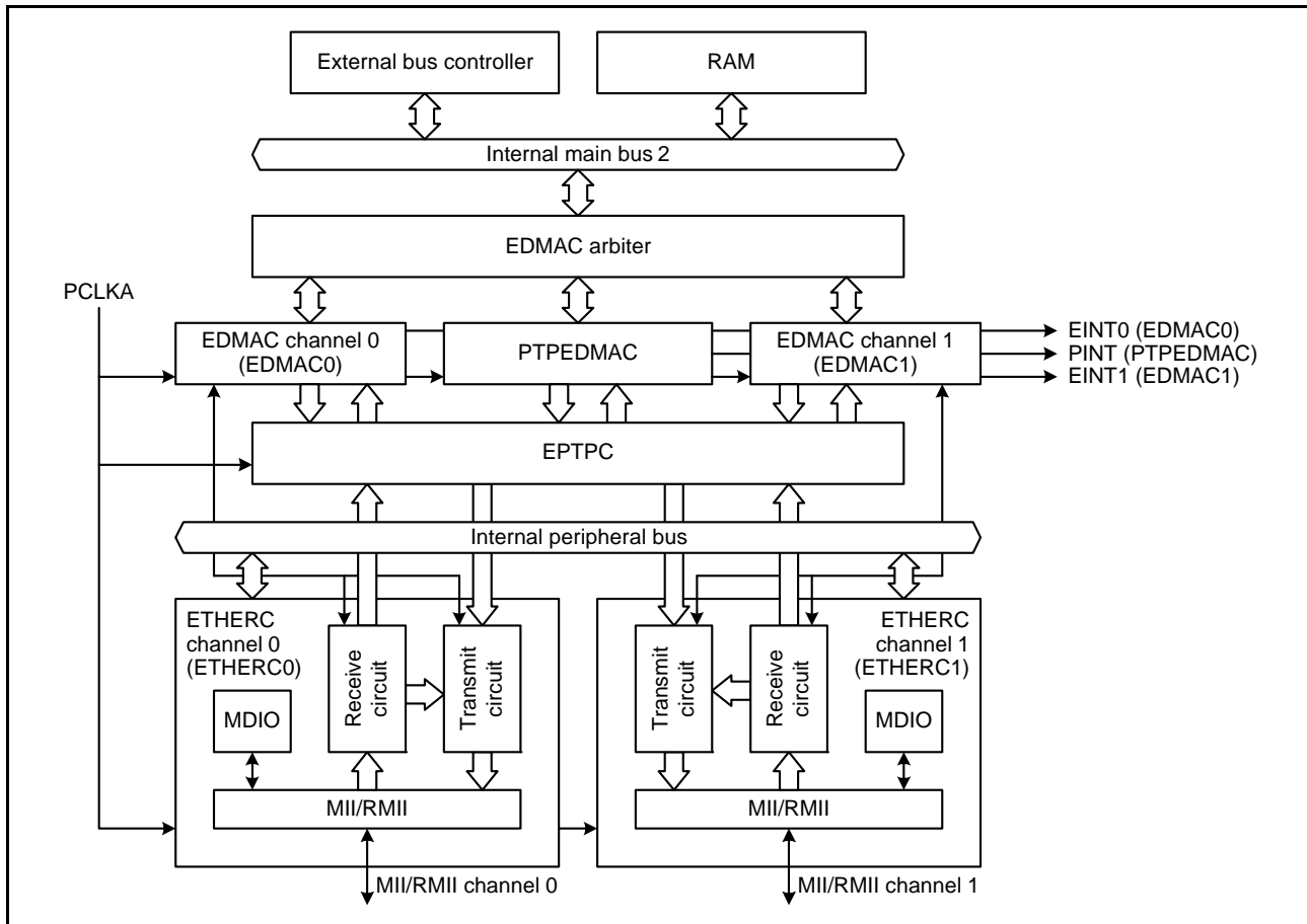
Figure 35.1 ETHERC Configuration
