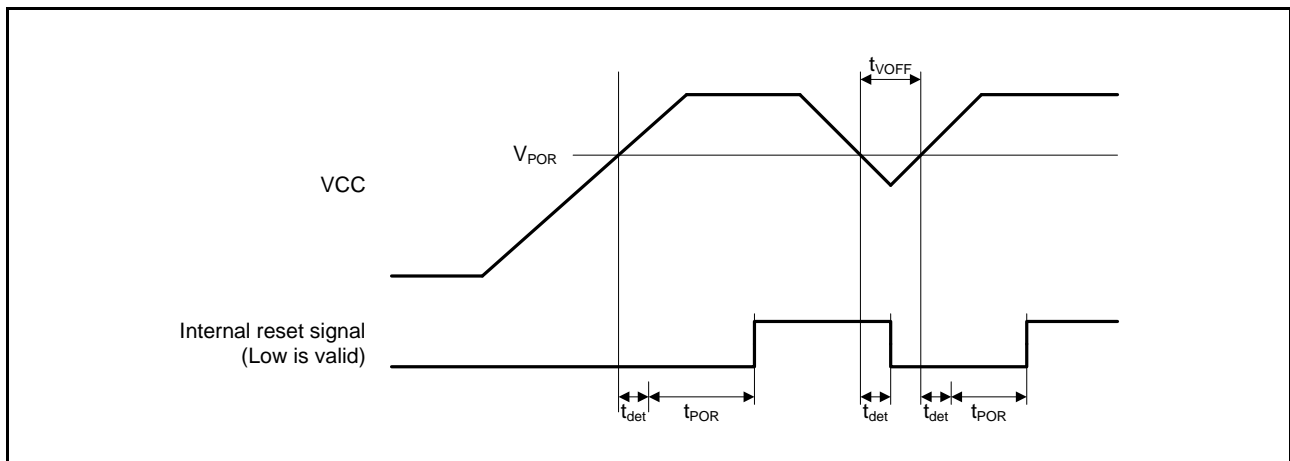
Figure 64.90 Power-on Reset Timing
