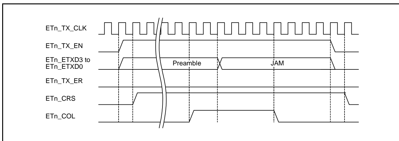
Figure 35.7 MII Frame Transmit Timing When Collision Occurs
