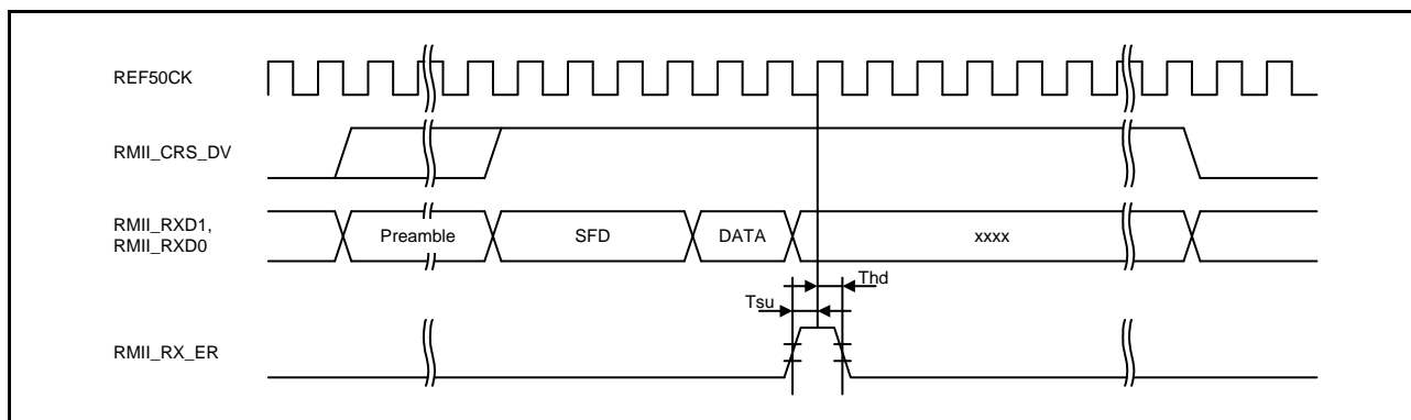
Figure 64.75 RMI Reception Timing (Error Occurrence)
