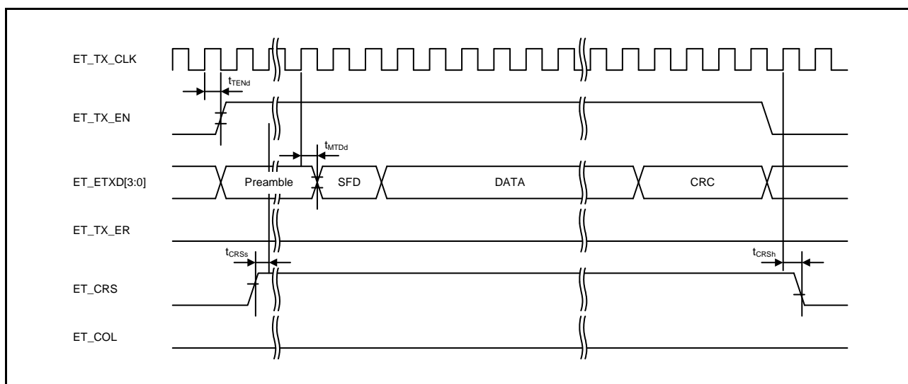
Figure 64.77 MII Transmission Timing (Normal Operation)
