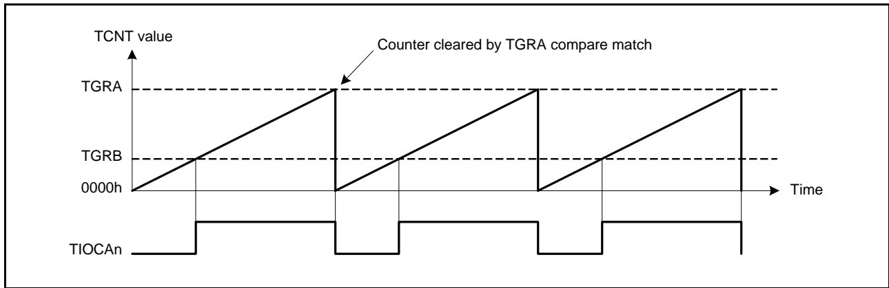
Figure 27.21 Example of PWM Mode Operation (1) (n = 0 to 5)
