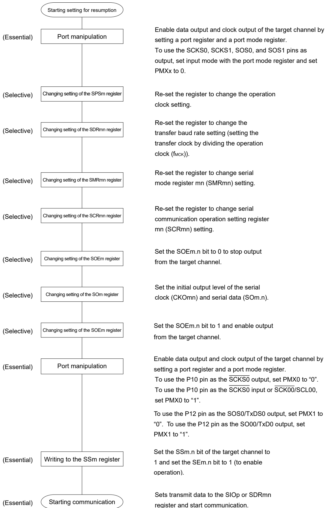
Figure 13-34. Procedure for Resuming Master Transmission
