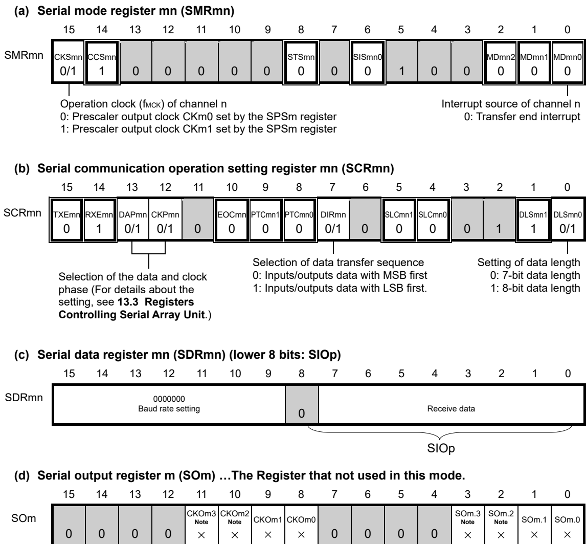
Figure 13-66. Example of Contents of Registers for Slave Reception of 3-Wire Serial I/O (CSI00, CSI01, CSI10, CSI11, CSI20, CSI21)
