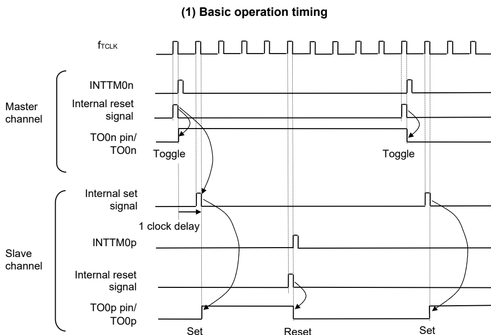
Figure 6-43. Set/Reset Timing Operating Statuses
