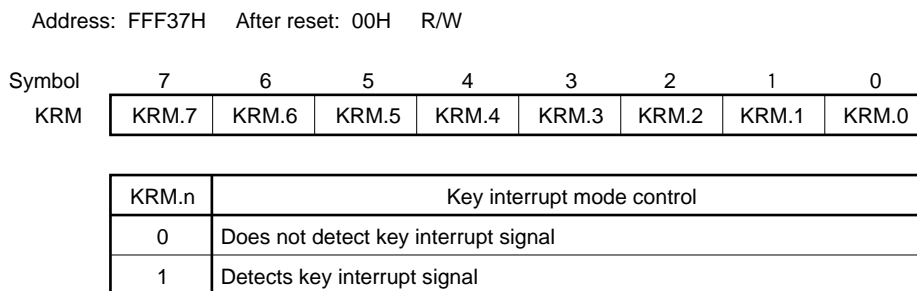
Figure 19-2. Format of Key Return Mode Register (KRM)
