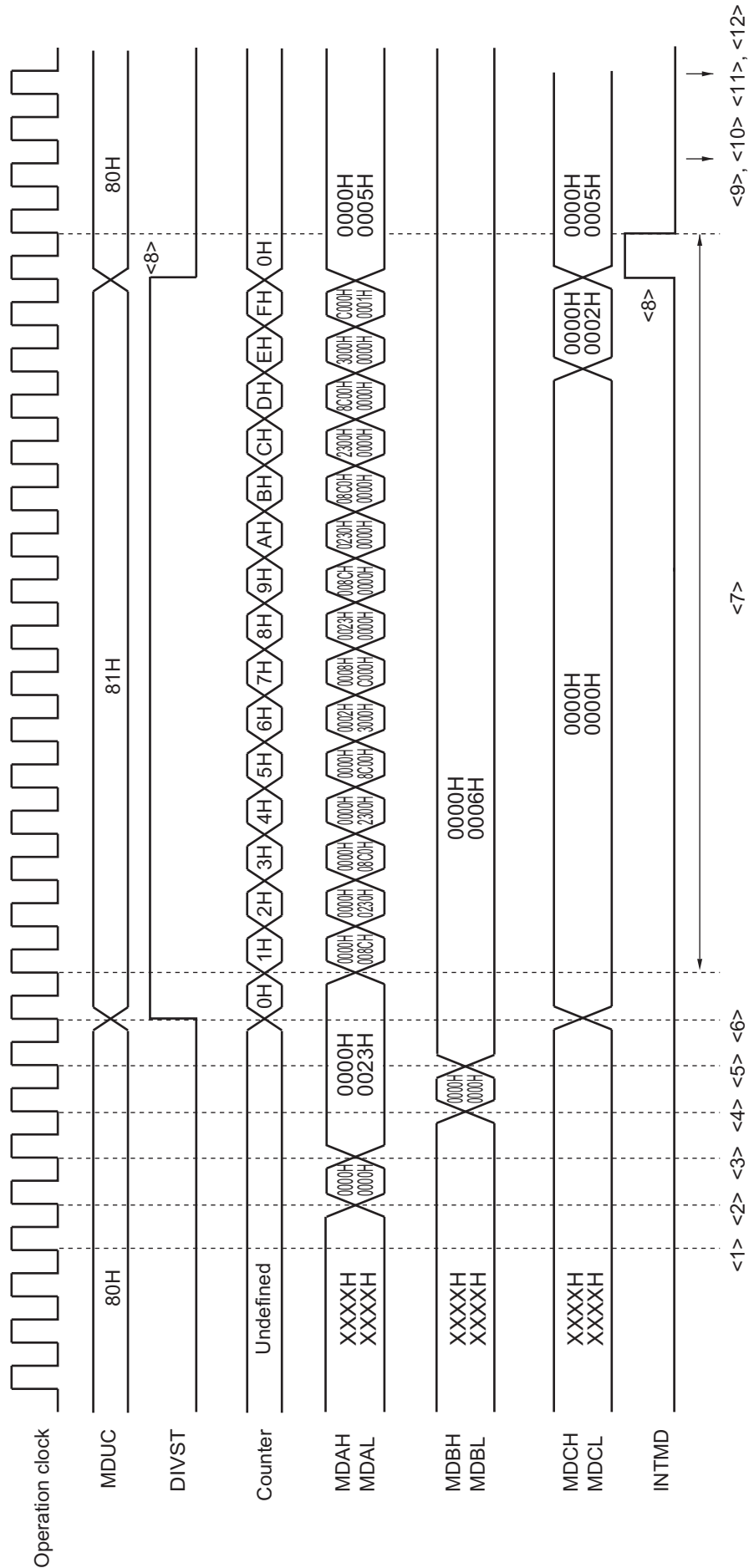
Figure 16-10. Timing Diagram of Division Operation (Example: 35 ÷ 6 = 5, Remainder 5)
