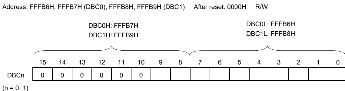
Figure 17-3. Format of DMA Byte Count Register n (DBCn)
