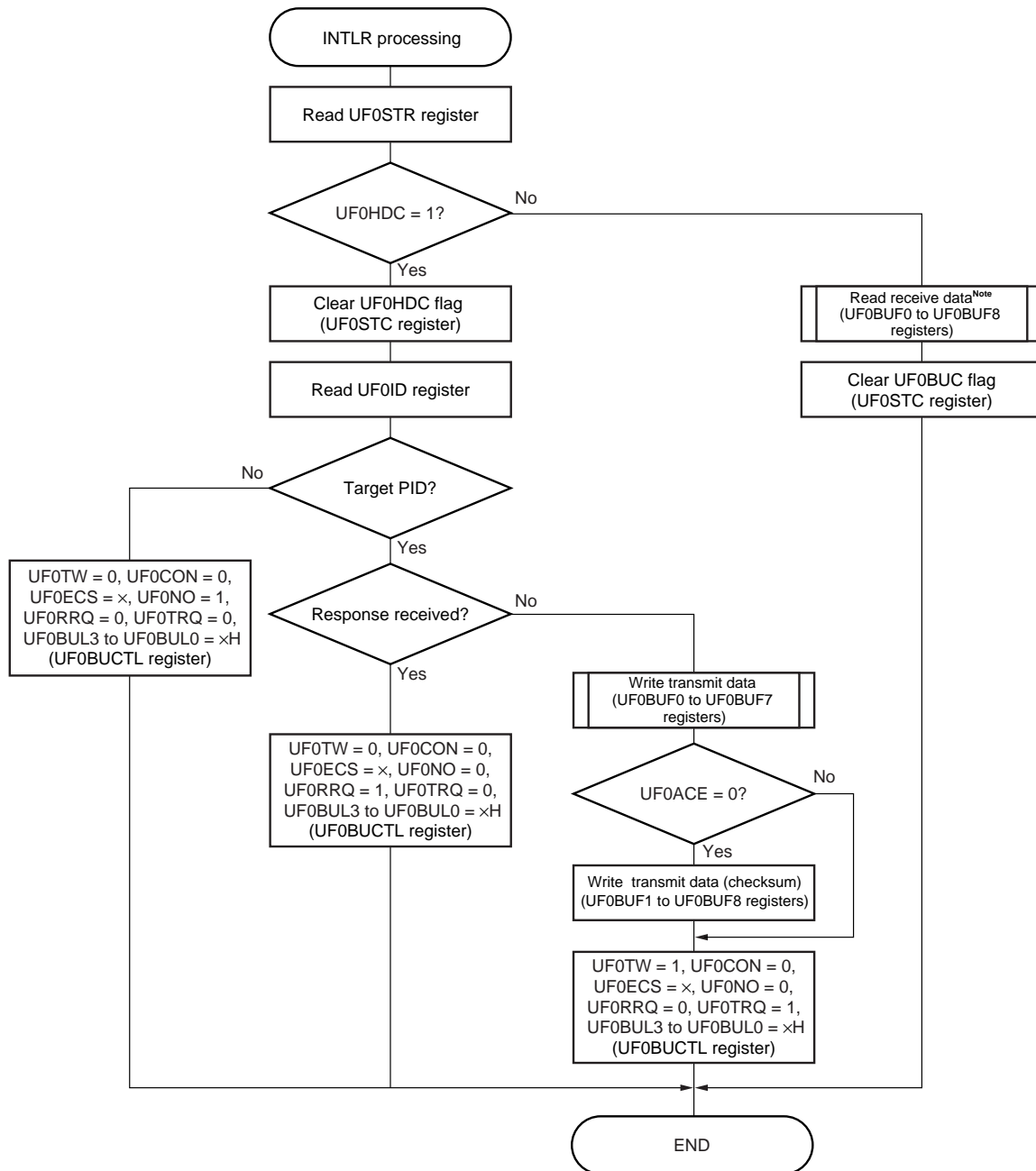
Figure 14-50. Basic Processing Flow Example of LIN Communication Automatic Baud Rate Mode (2/2)
