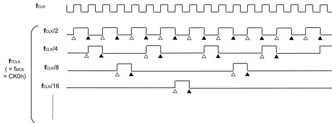
Figure 6-31. Timing of f CLK and count clock (f CLK ) (When CCS0n = 0)
