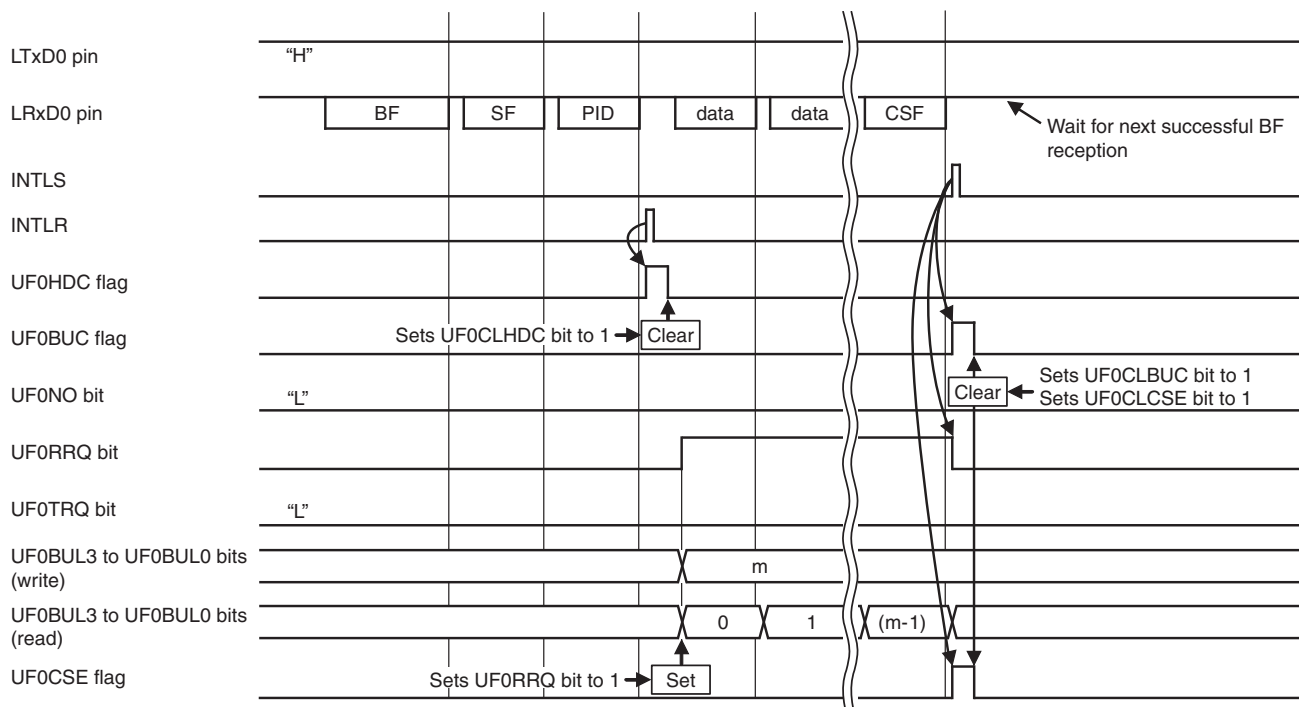
Figure 14-61. Automatic Checksum Error Occurrence Example (Response Reception)
