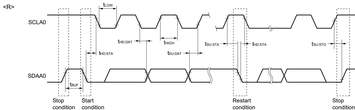
IICA serial transfer timing
