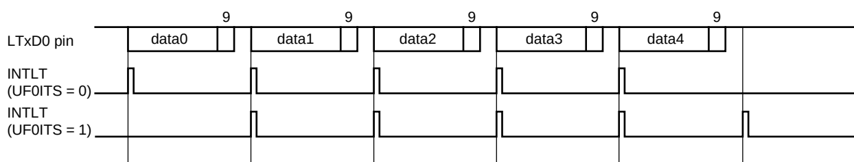
Figure 14-65. Expansion Bit Mode Transmission Example (LSB First)
