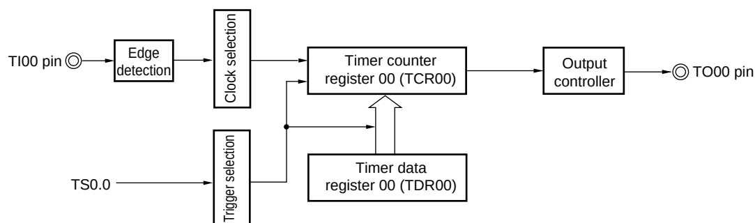
Figure 6-56. Block Diagram of Operation as Frequency Divider
