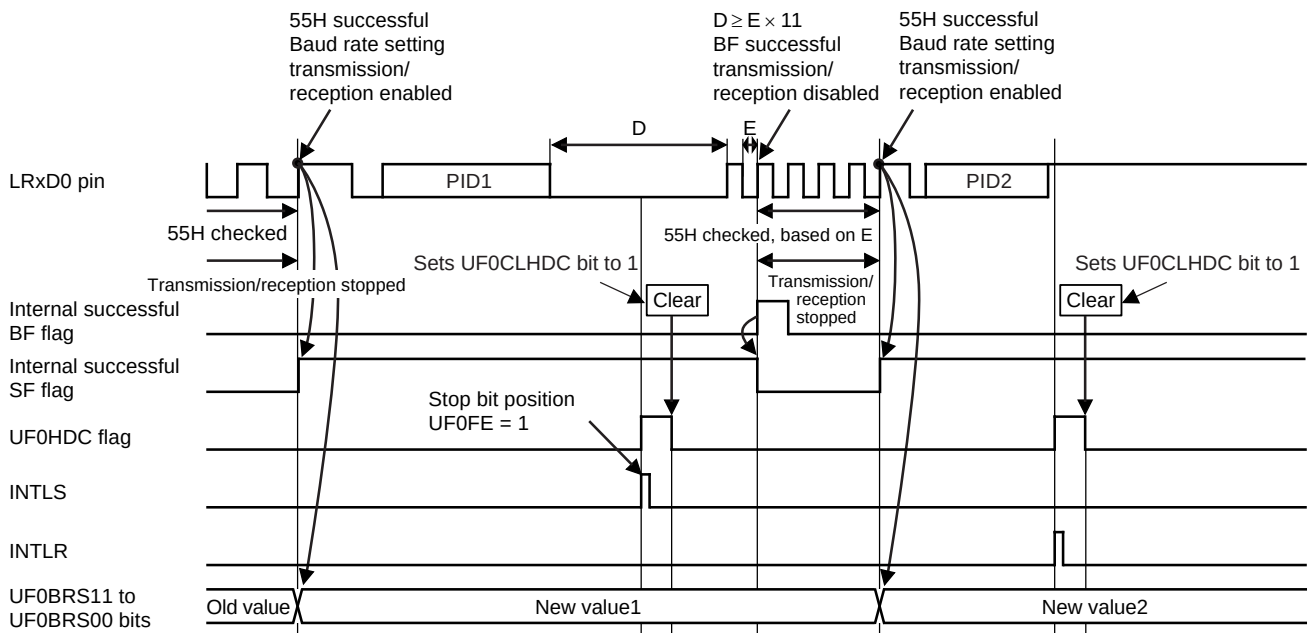
Figure 14-57. Example of Successful BF Reception During PID Reception (No PID2 Reception Error)
