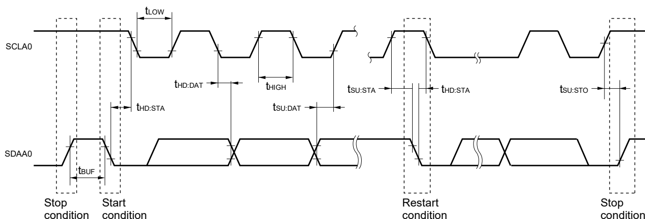
IICA serial transfer timing
