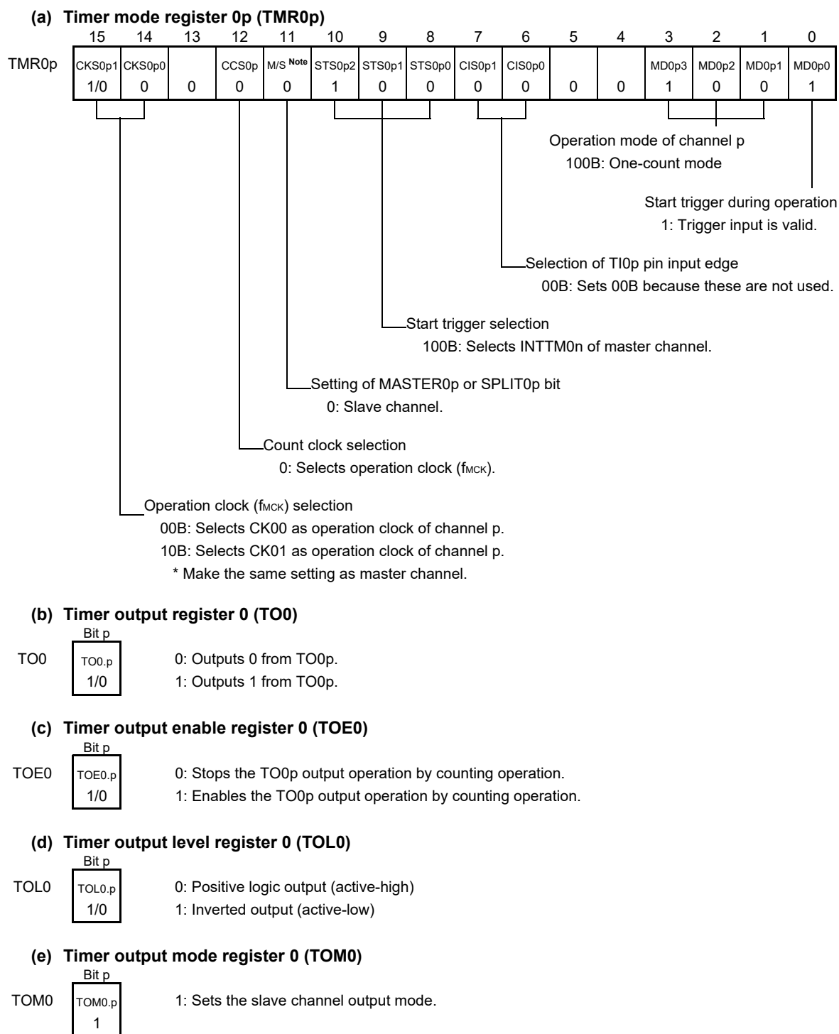
Figure 6-80. Example of Set Contents of Registers When PWM Function (Slave Channel) Is Used
