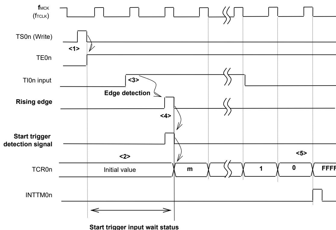
Figure 6-36 Operation Timing (In One-count Mode)
