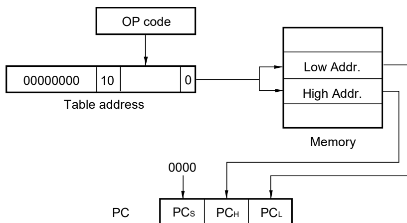
Figure 3-29. Outline of Table Indirect Addressing
