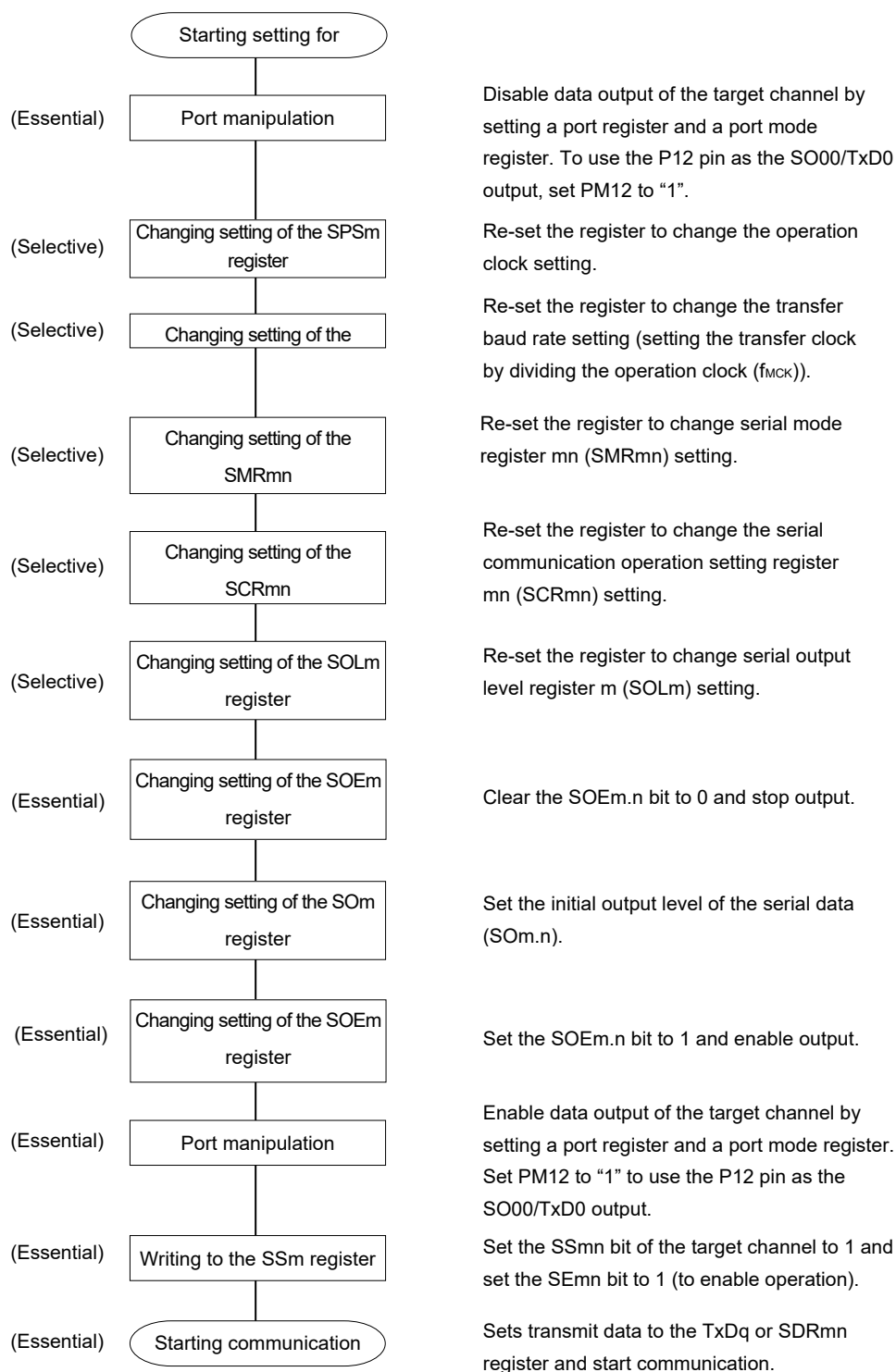
Figure 12-77. Procedure for Resuming UART Transmission
