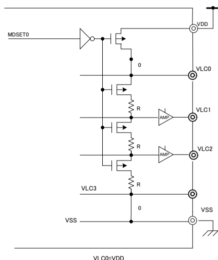
(a) 1/3 bias method and static display mode (MDSET1, MDSET0 = 0, 1) (example of V DD = 5 V, V LC0 = 5 V)
