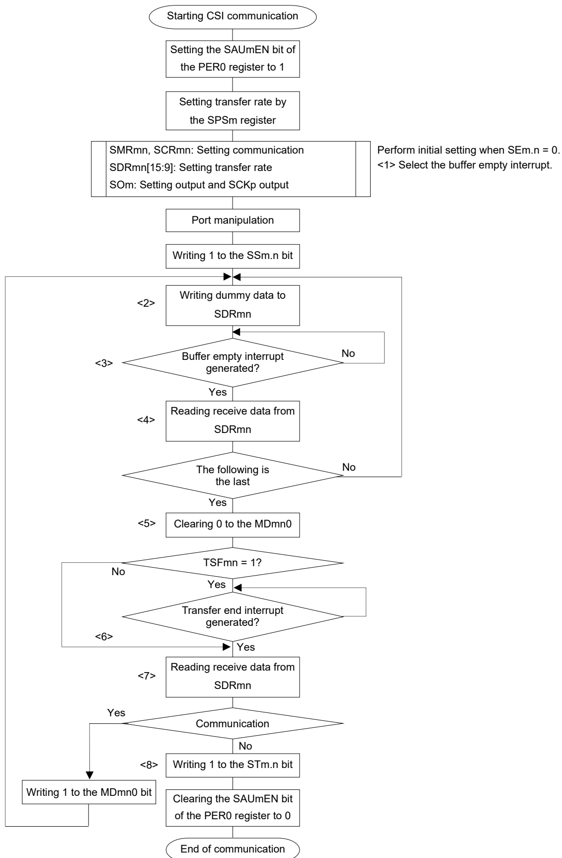
Figure 12-42. Flowchart of Master Reception (in Continuous Reception Mode)
