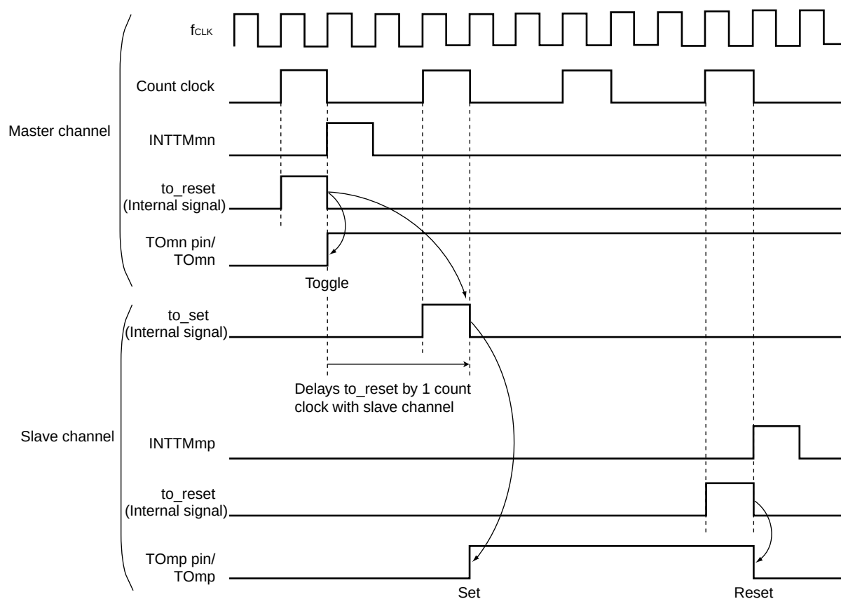
Figure 6-45. Set/Reset Timing Operating Statuses
