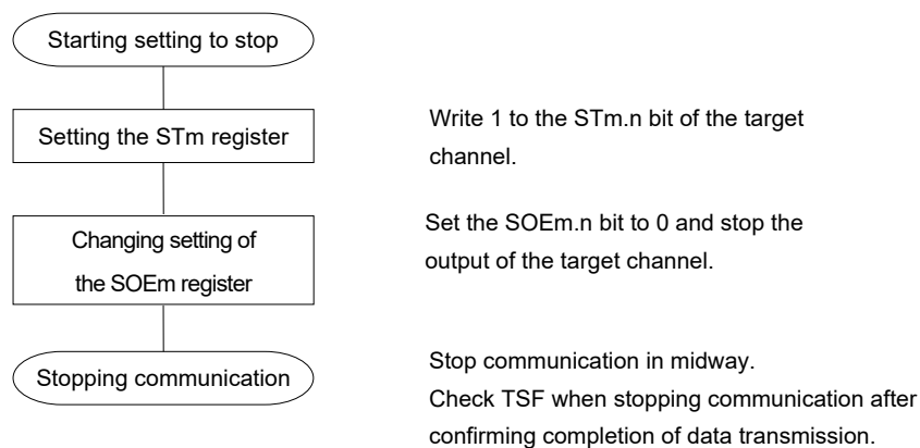
Figure 12-53. Procedure for Stopping Slave Transmission
