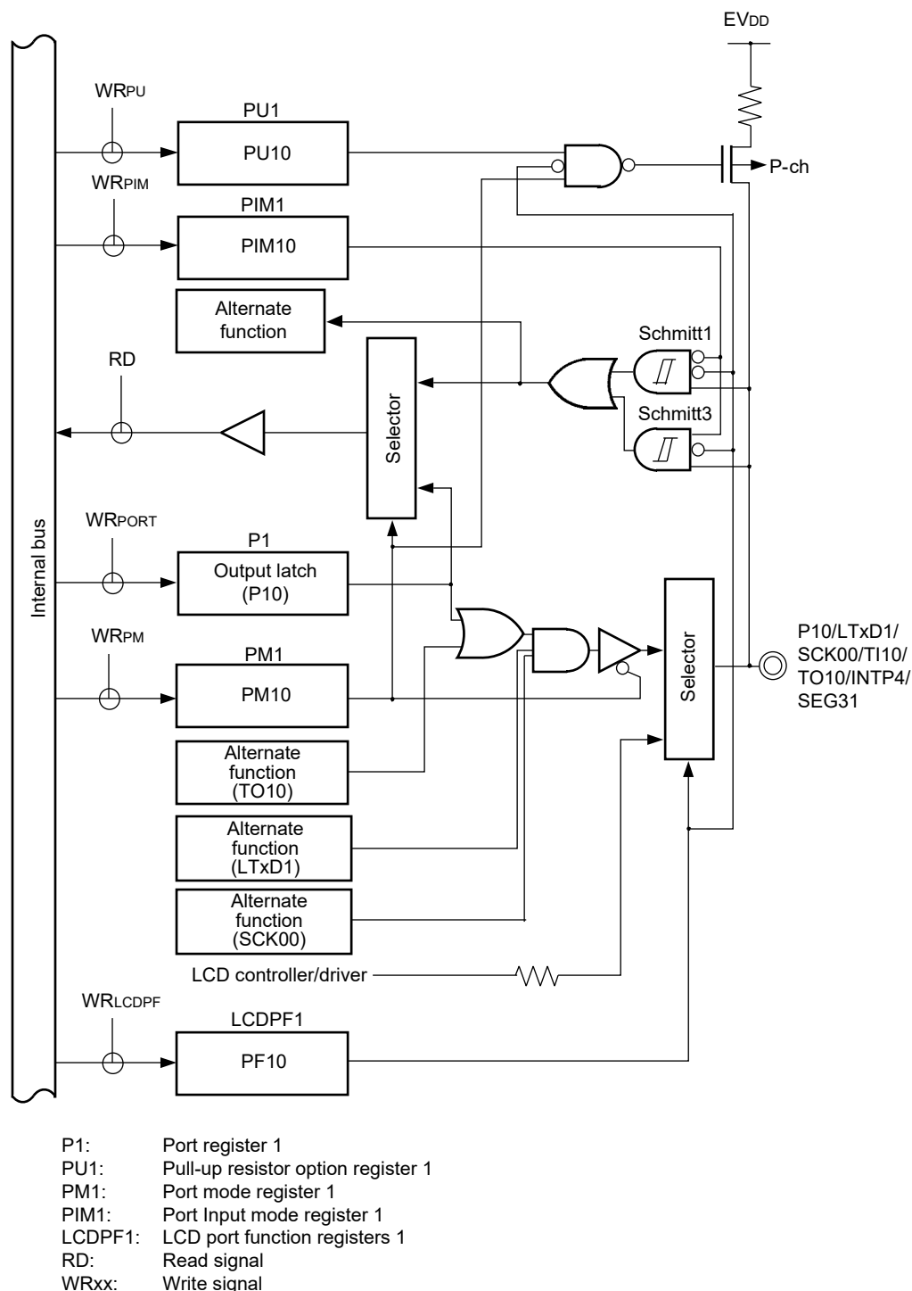
Figure 4-7. Block Diagram of P10
