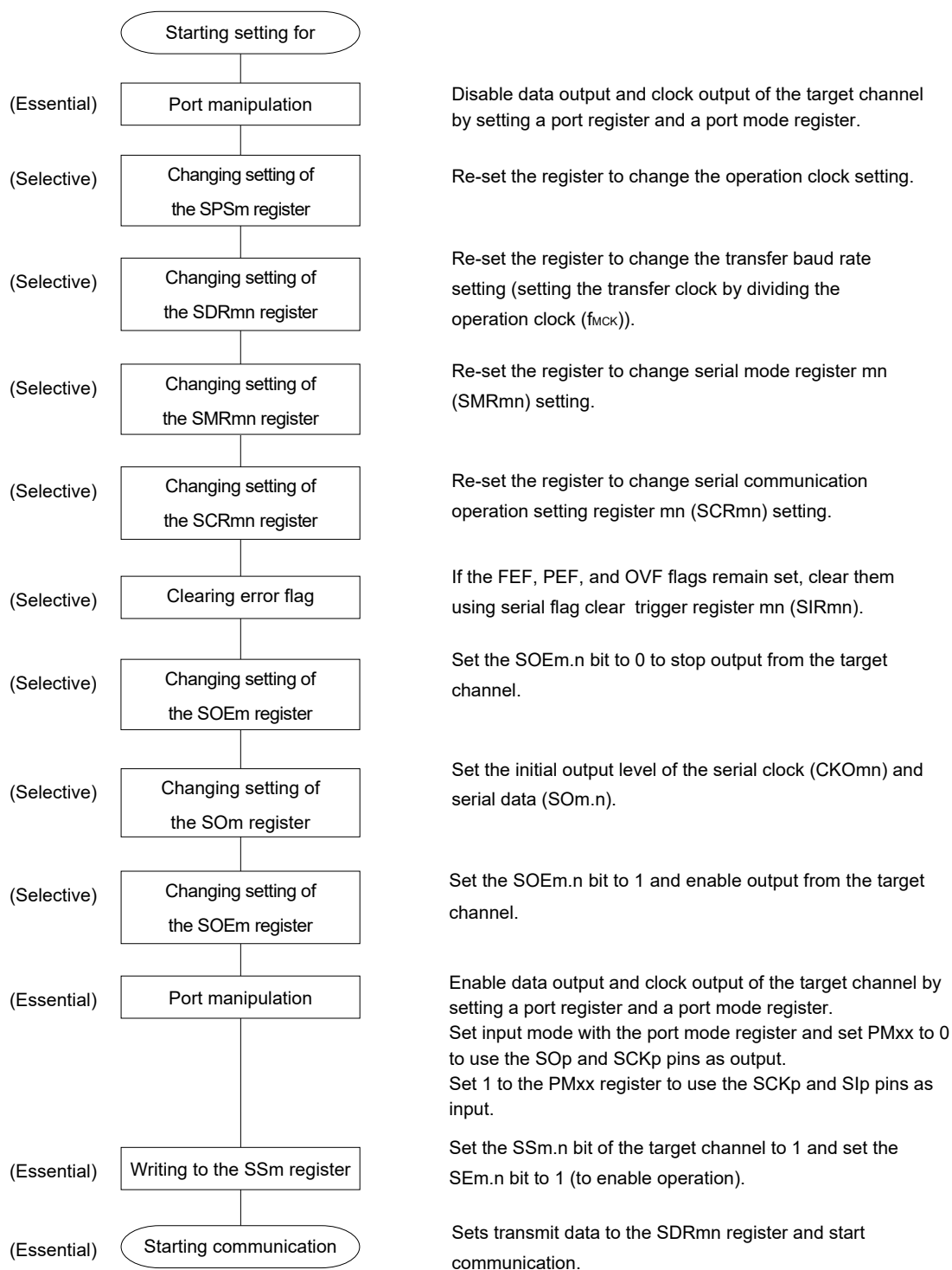
Figure 12-46. Procedure for Resuming Master Transmission/Reception
