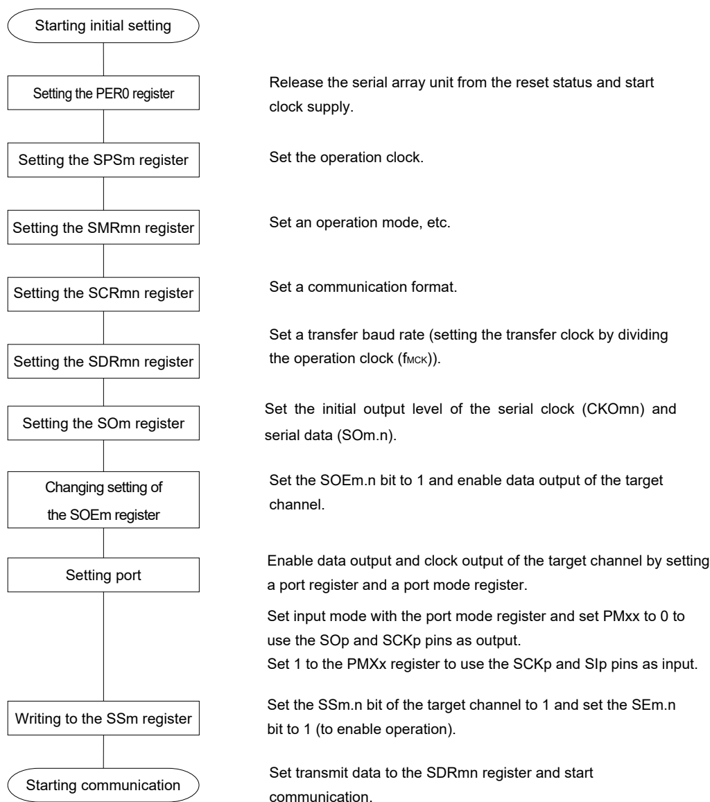
Figure 12-44. Initial Setting Procedure for Master Transmission/Reception
