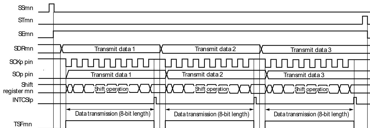
Figure 12-31. Timing Chart of Master Transmission (in Single-Transmission Mode) (Type 1: DAPmn = 0, CKPmn = 0)
