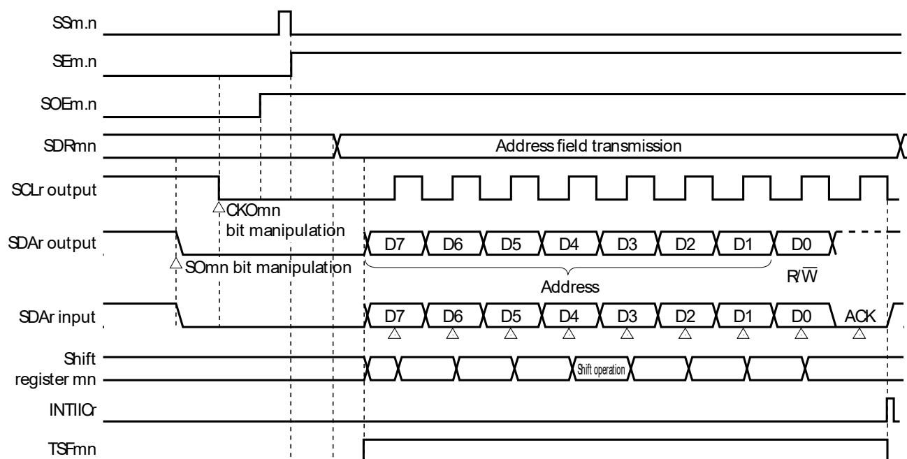
Figure 12-93. Timing Chart of Address Field Transmission
