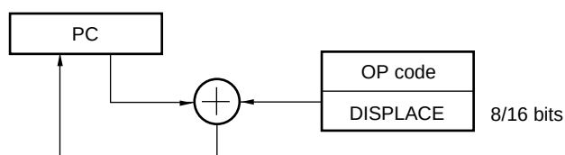
Figure 3-26. Outline of Relative Addressing
