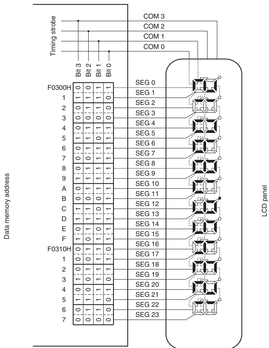
Figure 16-25. Example of Connecting Four-Time-Slice LCD Panel
