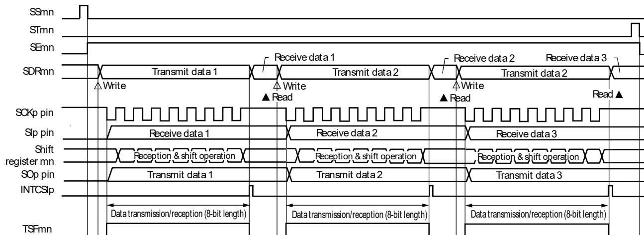
Figure 12-47. Timing Chart of Master Transmission/Reception (in Single-Transmission/Reception Mode) (Type 1: DAPmn = 0, CKPmn = 0)
