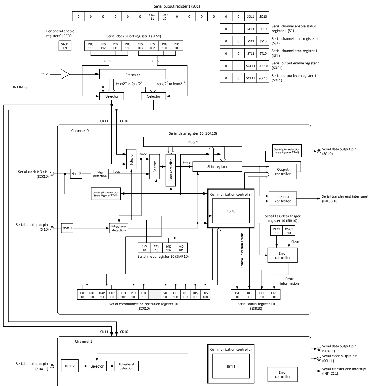
Figure 12-3. Block Diagram of Serial Array Unit 1
