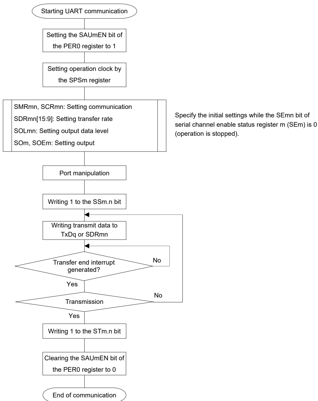
Figure 12-79. Flowchart of UART Transmission (in Single-Transmission Mode)
