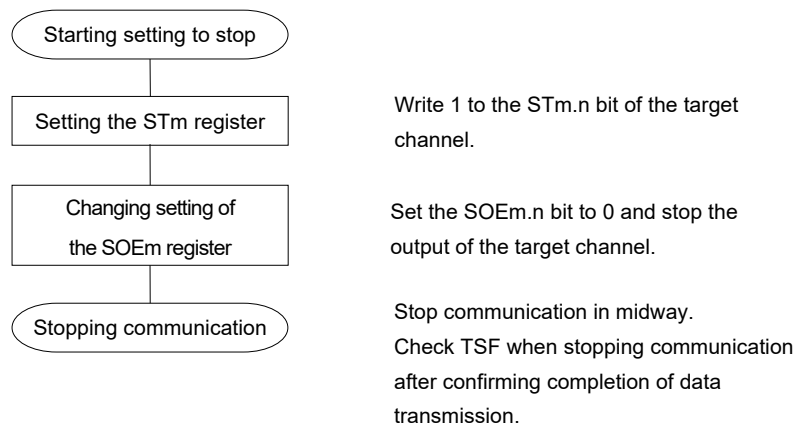
Figure 12-67. Procedure for Stopping Slave Transmission/Reception
