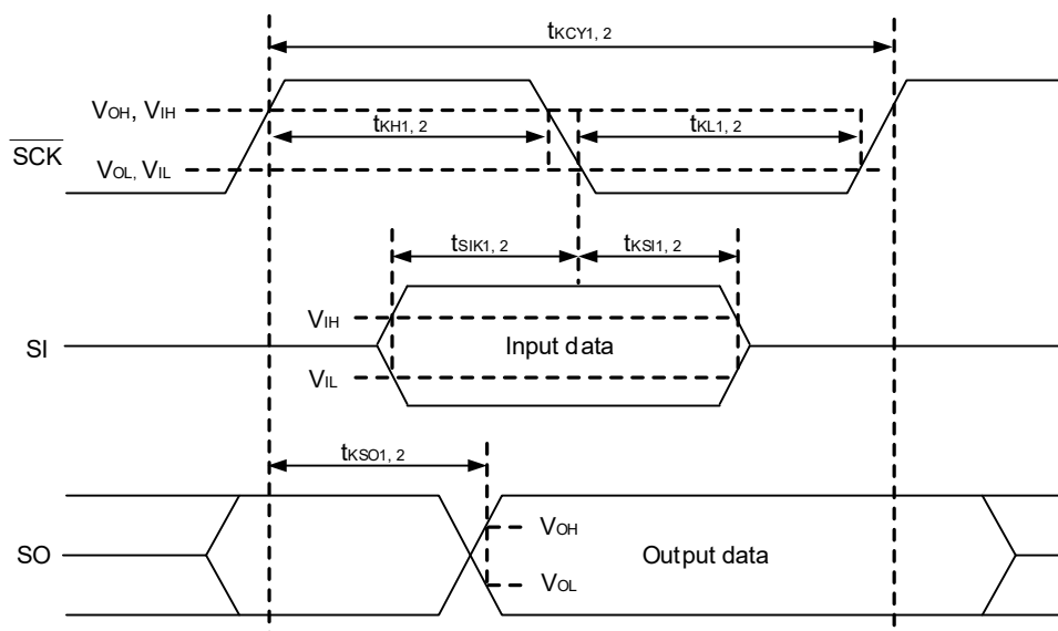
<R> Figure 33-8. CSI mode serial transfer timing (When DAPmn = 0 and CKPmn = 1, or DAPmn = 1 and CKPmn = 0.)
