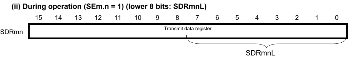
Figure 12-27. Example of Contents of Registers for Master Transmission of 3-Wire Serial I/O (CSI00, CSI01, CSI10) (2/2)
