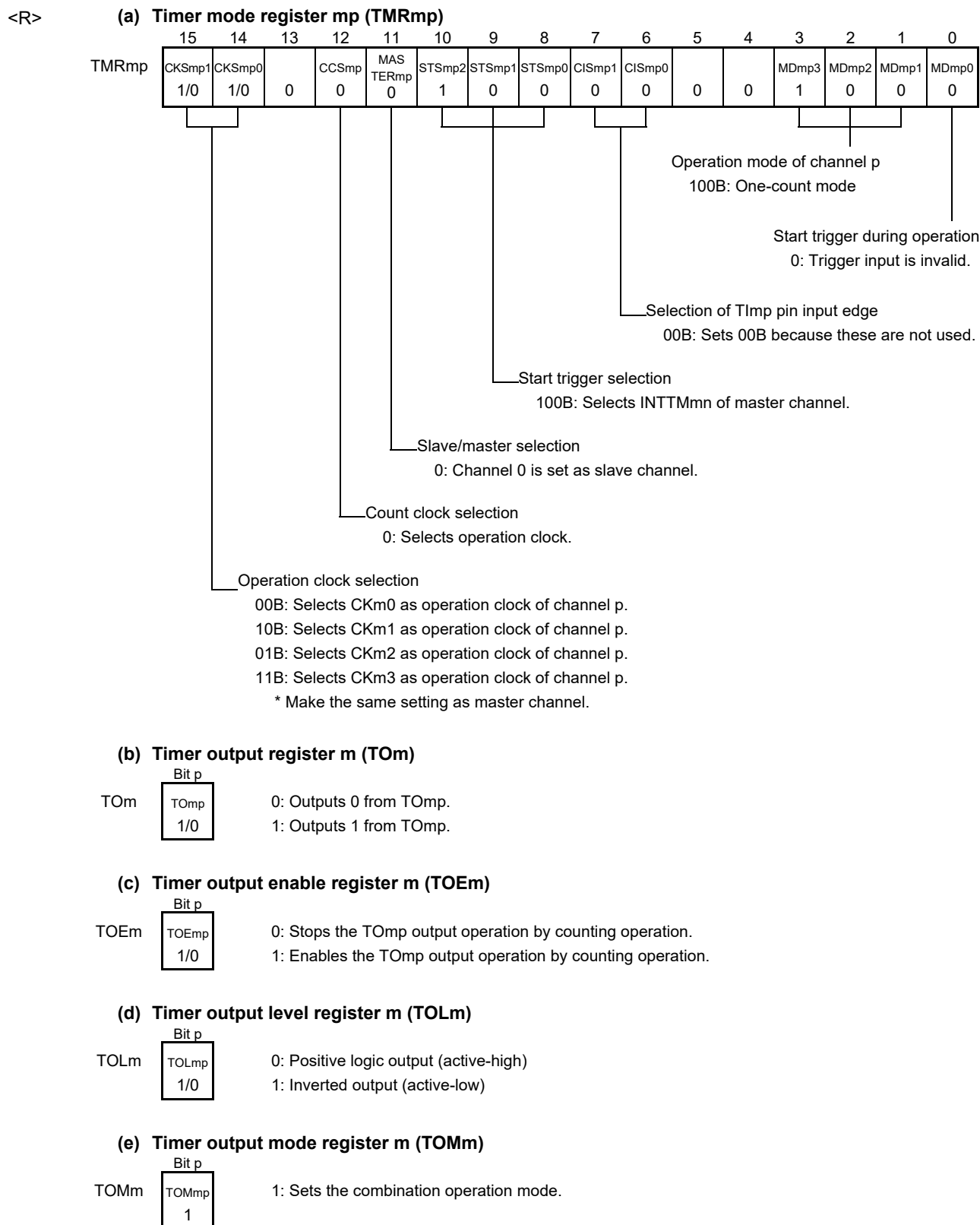
Figure 6-79. Example of Set Contents of Registers When One-Shot Pulse Output Function Is Used (Slave Channel)
