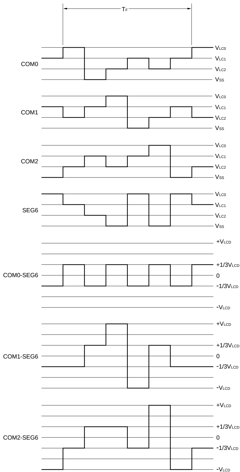
Figure 16-23. Three-Time-Slice LCD Drive Waveform Examples (1/3 Bias Method)
