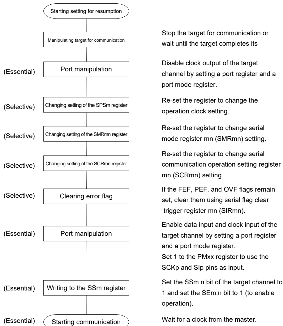
Figure 12-62. Procedure for Resuming Slave Reception
