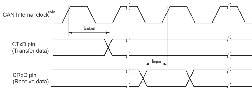
Figure 34-13. Internal delay time of CAN
