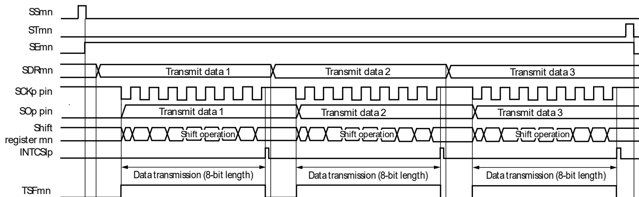
Figure 12-55. Timing Chart of Slave Transmission (in Single-Transmission Mode) (Type 1: DAPmn = 0, CKPmn = 0)
