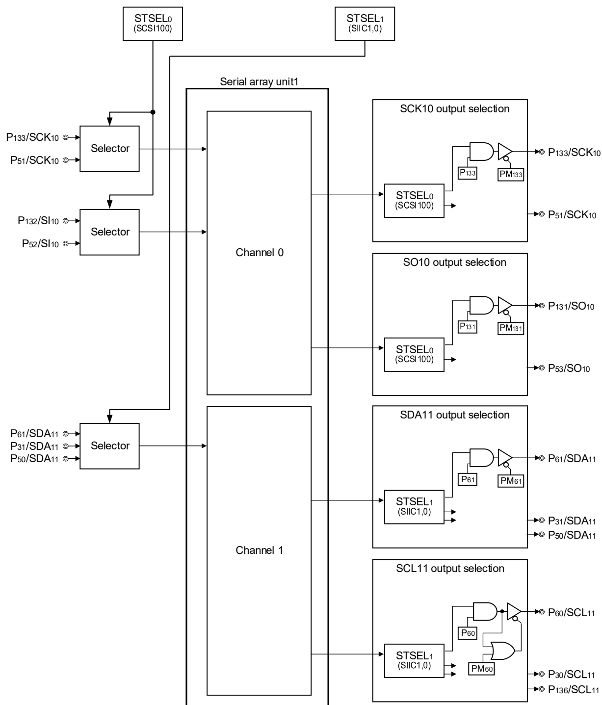
Figure 12-4. Port Configuration Diagram of Serial Array Unit 1
