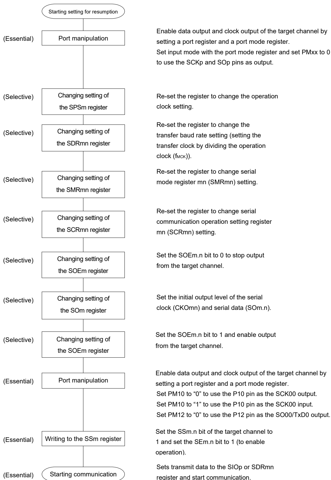
Figure 12-30. Procedure for Resuming Master Transmission
