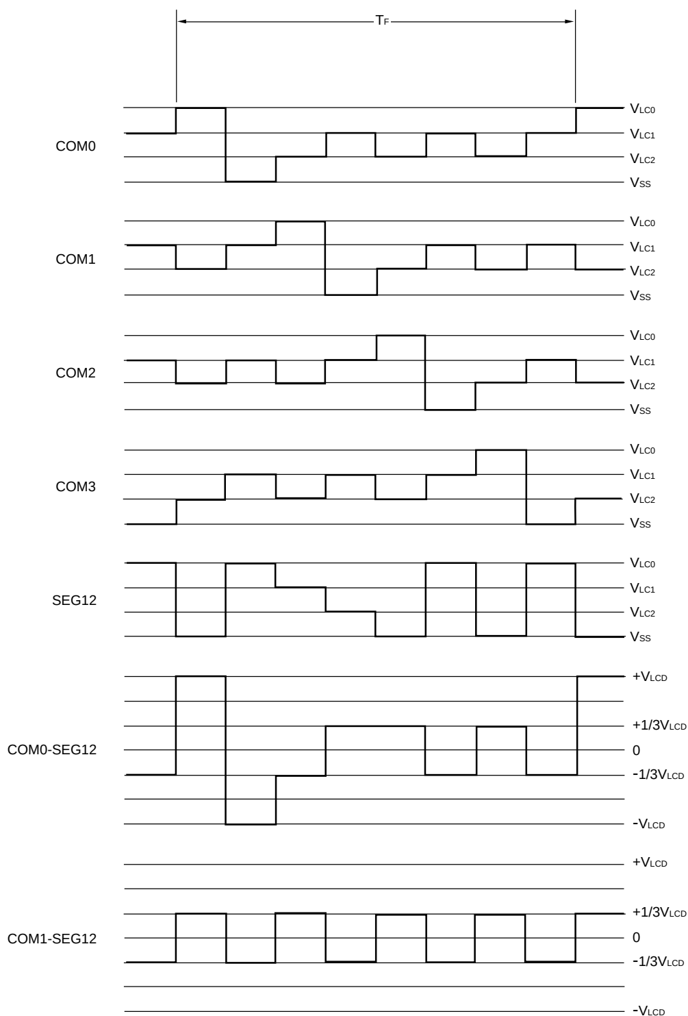
Figure 16-26. Four-Time-Slice LCD Drive Waveform Examples (1/3 Bias Method)
