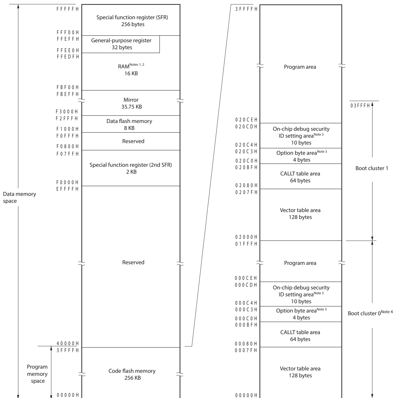
<R> Figure 3-7. Memory Map (R5F10DMJ, R5F10TPJ, R5F10DPJ, R5F10DSJ)
