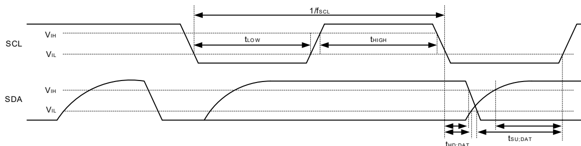
Figure 34-12. Simplified I 2 C mode serial transfer timing
