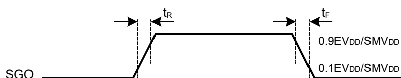
Sound Generator Output Timing
