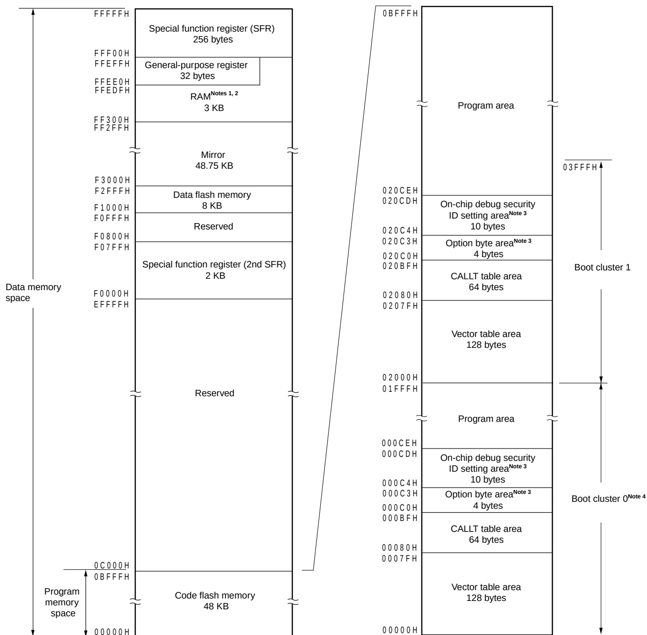
<R> Figure 3-3. Memory Map (R5F10CGD, R5F10DGD, R5F10CLD, R5F10DLD, R5F10CMD, R5F10DMD)
