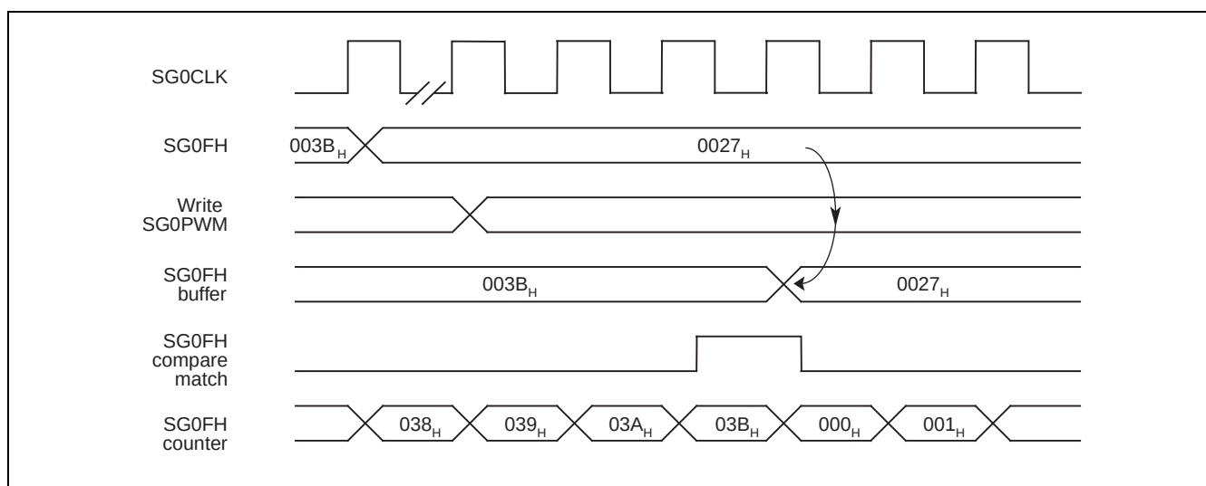
Figure 18-5. Update Timing of the Frequency Buffers
