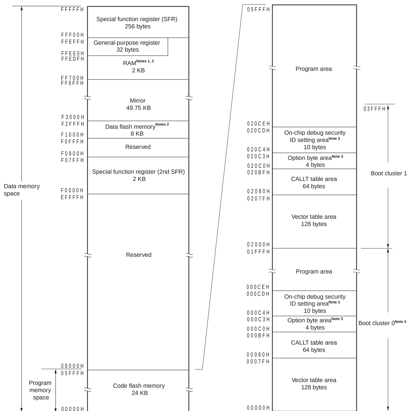
Figure 3-1. Memory Map (R5F10CGB)
