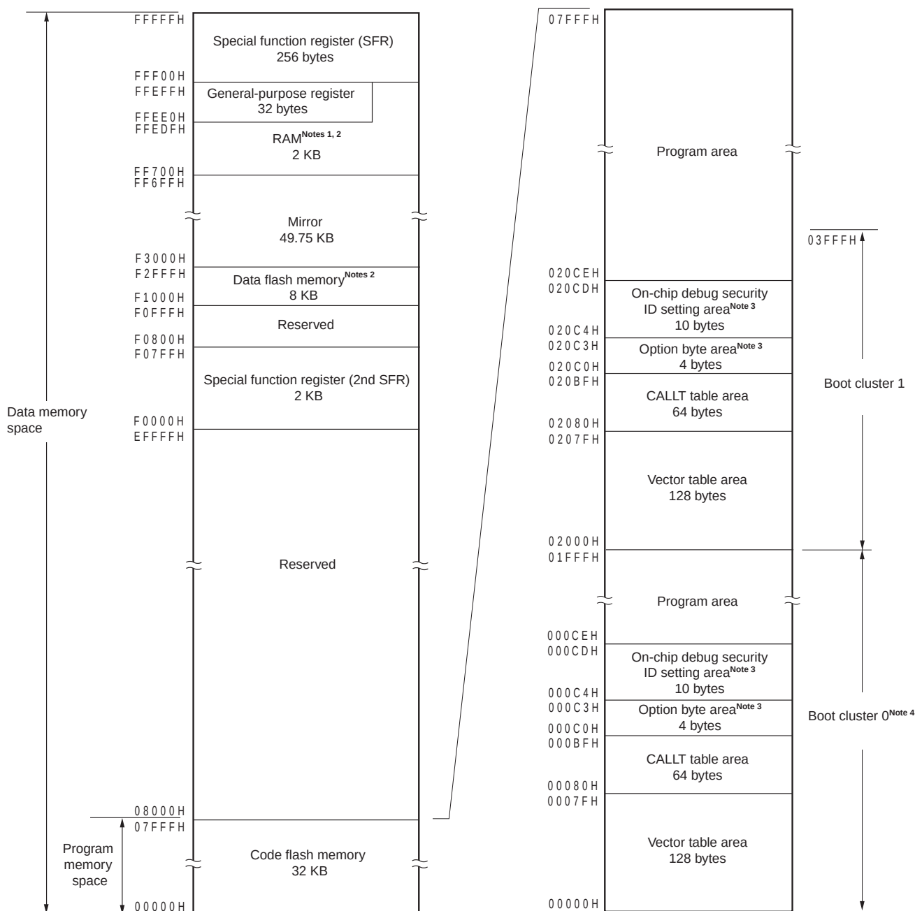
Figure 3-2. Memory Map (R5F10CGC, R5F10DGC)
