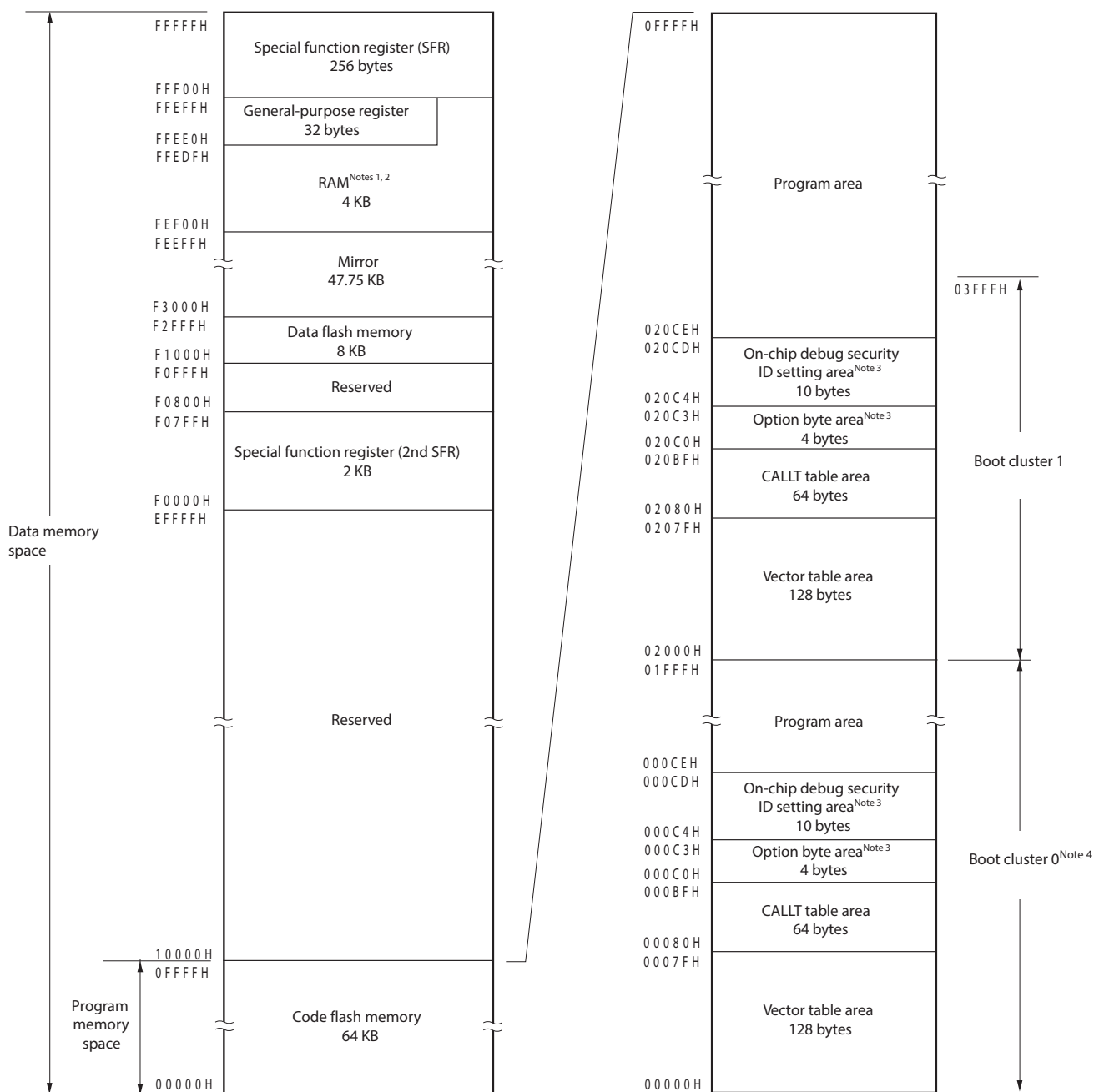
Figure 3-4. Memory Map (R5F10DGE, R5F10DLE, R5F10CME, R5F10DME, R5F10DPE)
