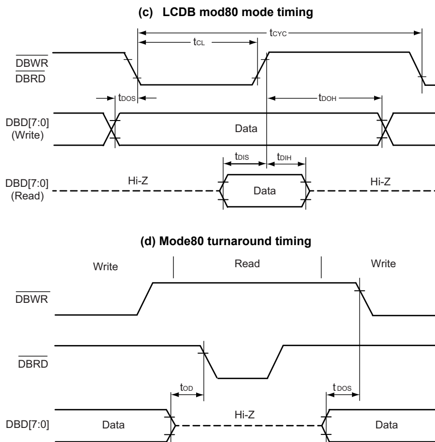
Figure 33-14. LCD Bus Interface AC timing (2/2)
