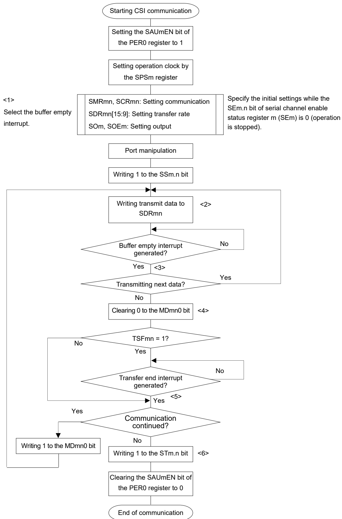
Figure 12-34. Flowchart of Master Transmission (in Continuous Transmission Mode)
