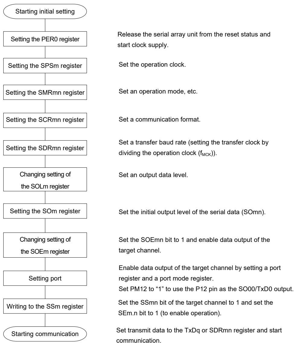
Figure 12-75. Initial Setting Procedure for UART Transmission
