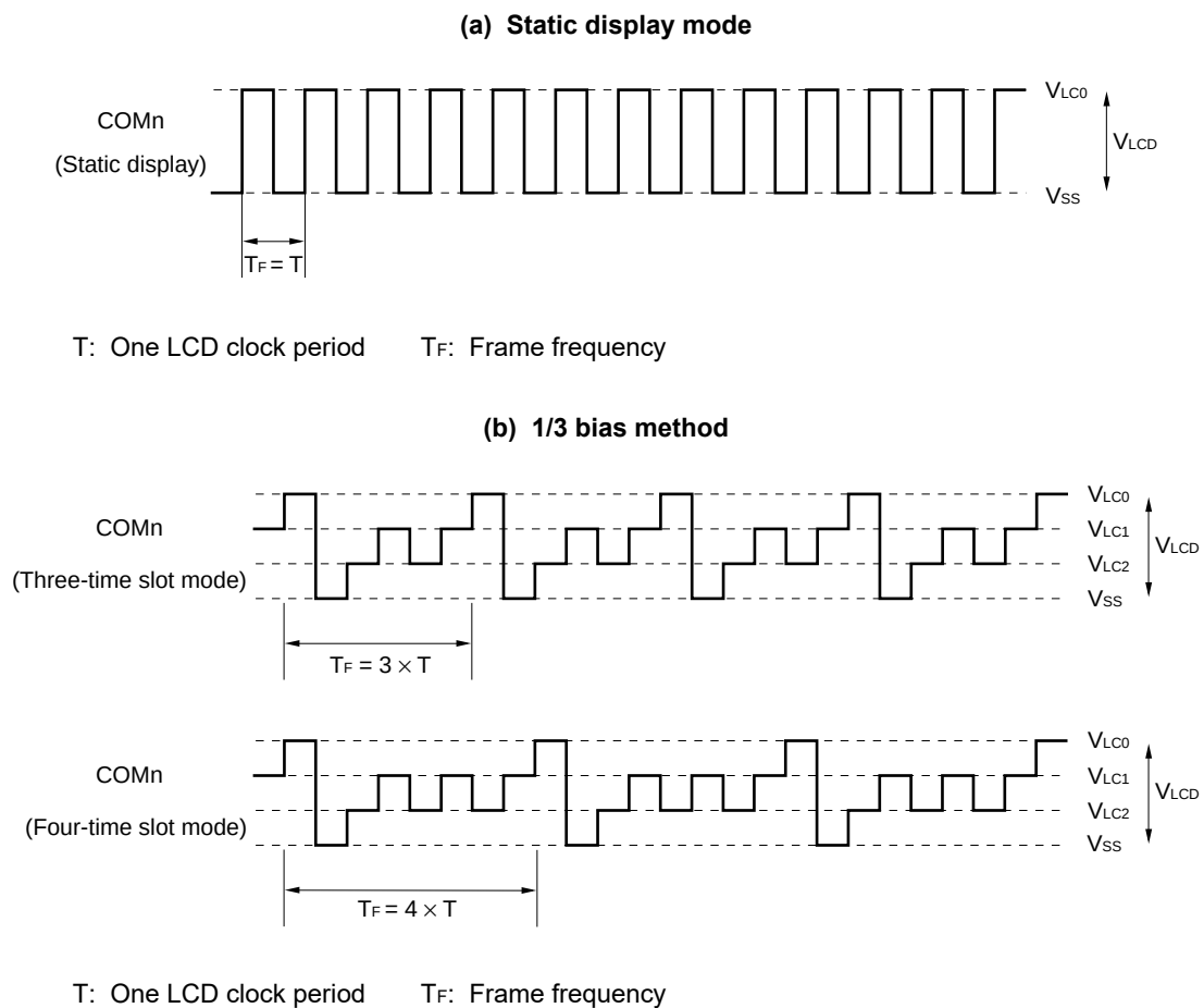
Figure 16-16. Common Signal Waveforms
