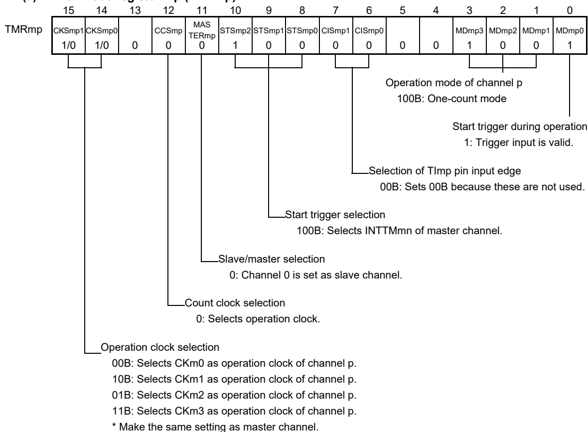
Figure 6-74. Example of Set Contents of Registers When PWM Function (Slave Channel) Is Used
