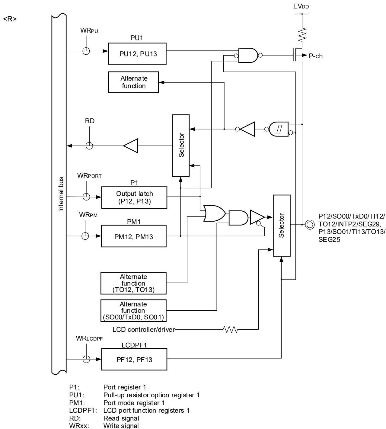
Figure 4-9. Block Diagram of P12, P13
