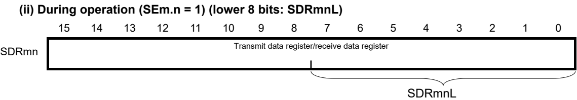
Figure 12-43. Example of Contents of Registers for Master Transmission/Reception of 3-Wire Serial I/O (CSI00, CSI01, CSI10) (2/2)
