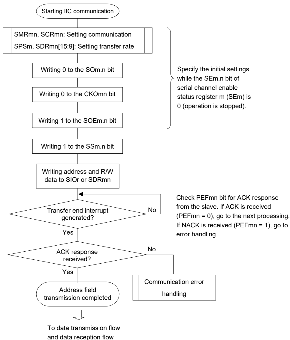
Figure 12-94. Flowchart of Address Field Transmission
