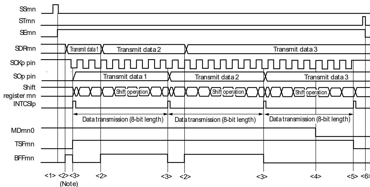
Figure 12-57. Timing Chart of Slave Transmission (in Continuous Transmission Mode) (Type 1: DAPmn = 0, CKPmn = 0)
