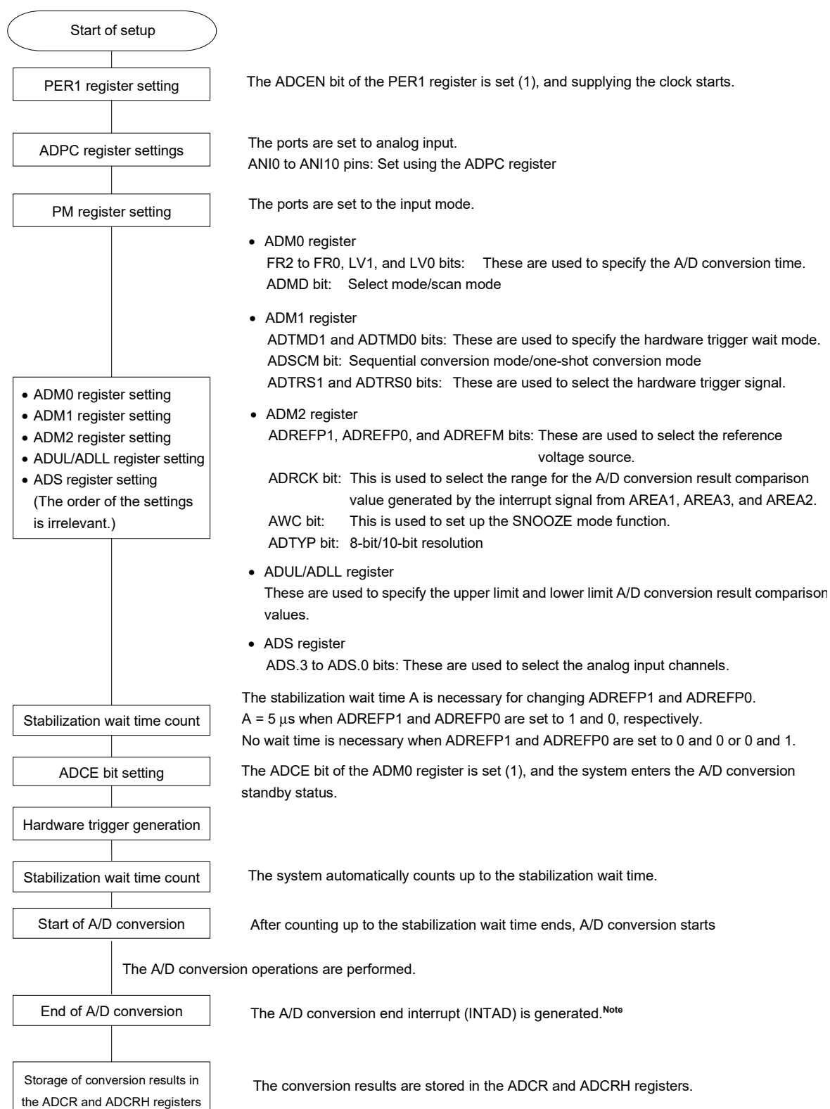
Figure 11-33. Setting up Hardware Trigger Wait Mode
