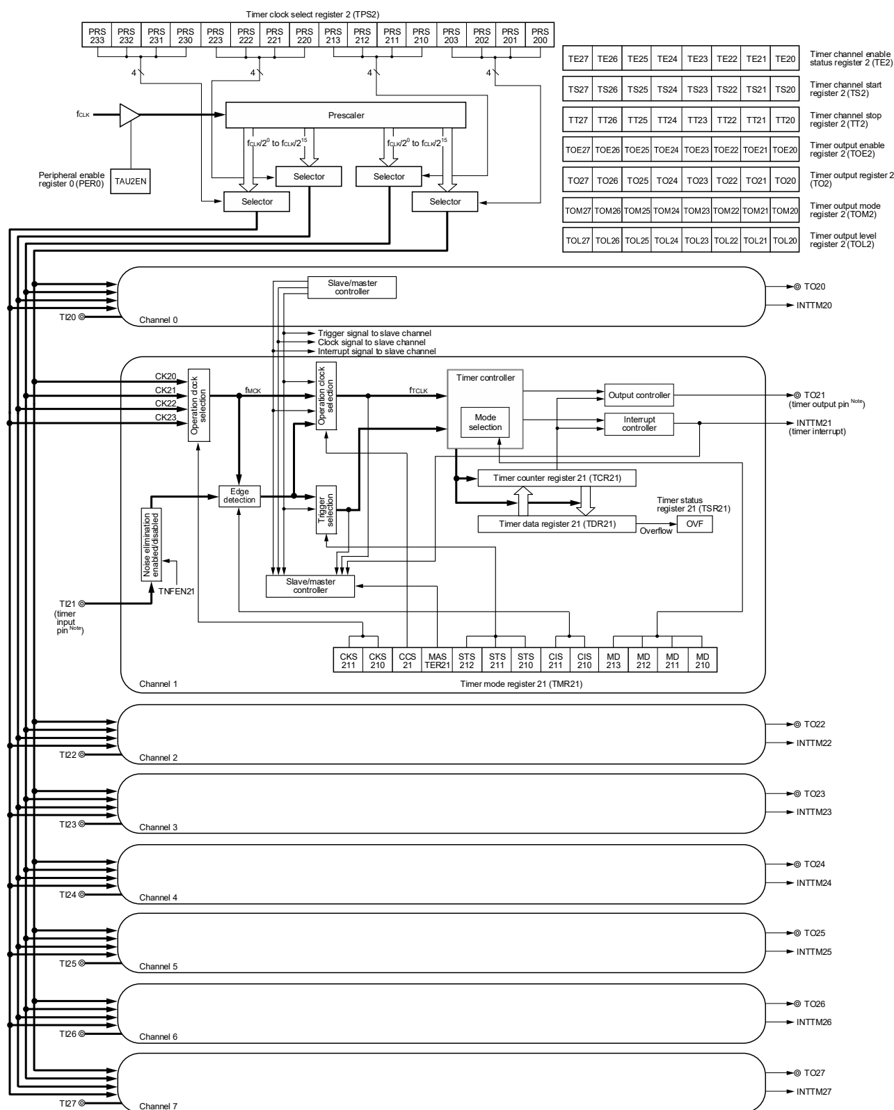
Figure 6-5. Block Diagram of Timer Array Unit 2
