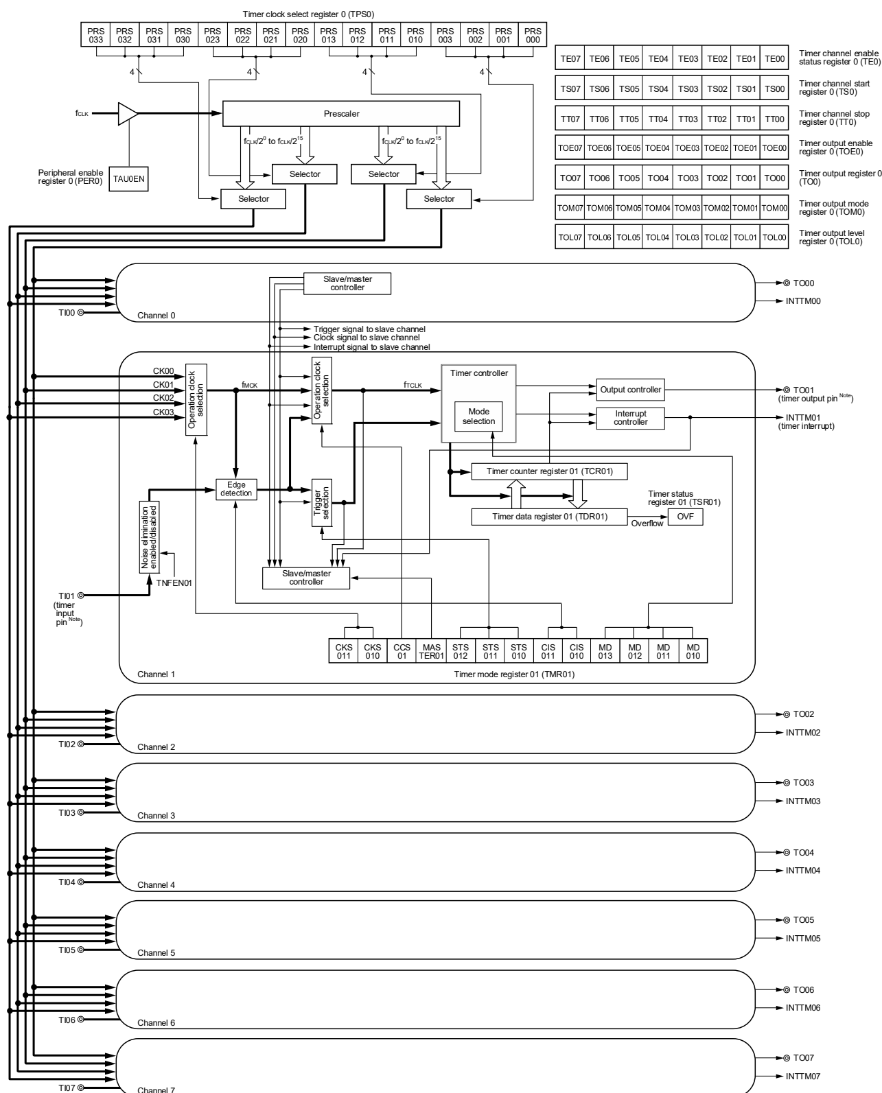
Figure 6-1. Block Diagram of Timer Array Unit 0
