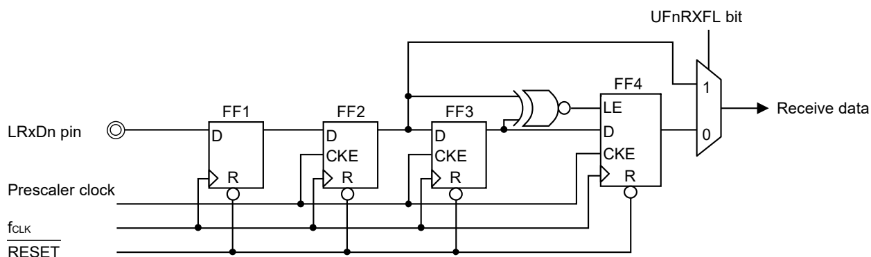
Figure 13-70. Noise Filter Circuit Example
