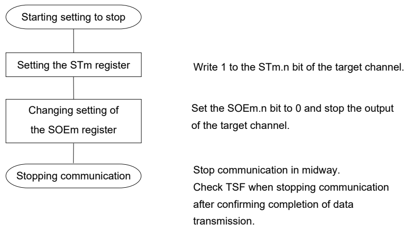
Figure 12-29. Procedure for Stopping Master Transmission
