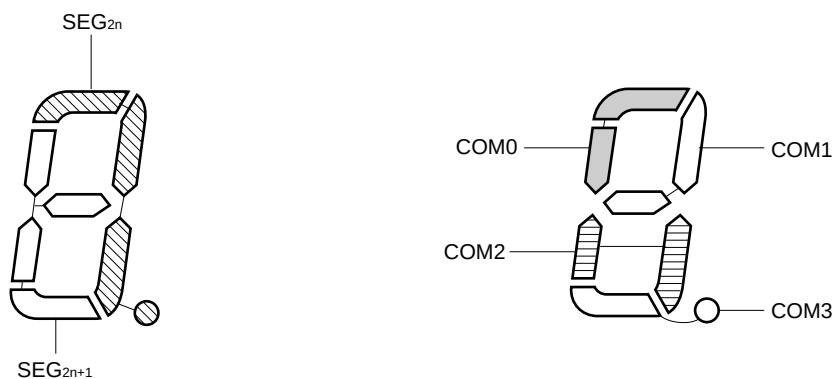
Figure 16-24. Four-Time-Slice LCD Display Pattern and Electrode Connections
