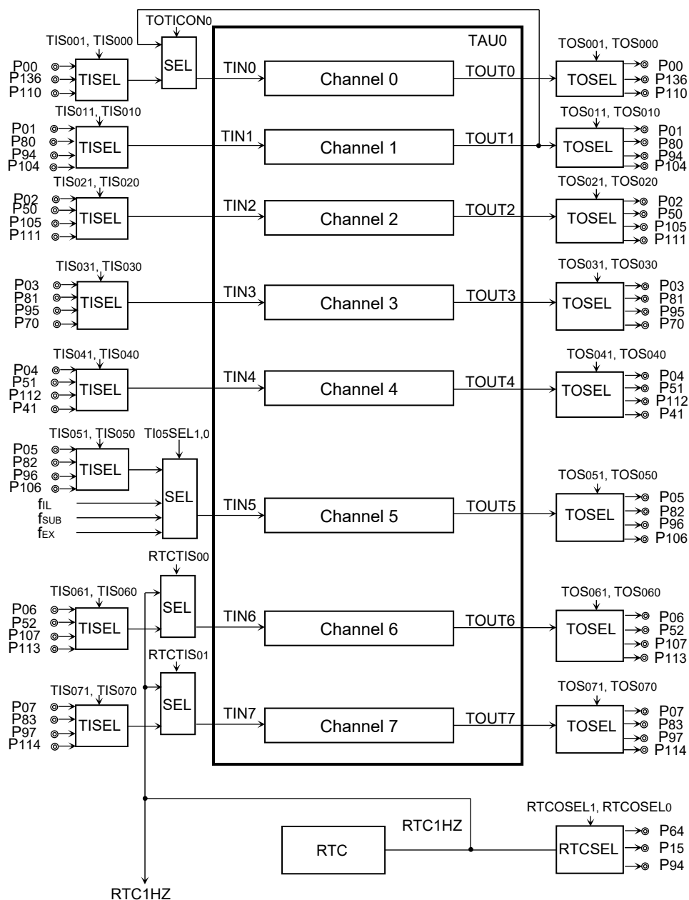
<R> Figure 4-66. Timer Array unit and RTC I/O connection (128-pin products) (1/3)
