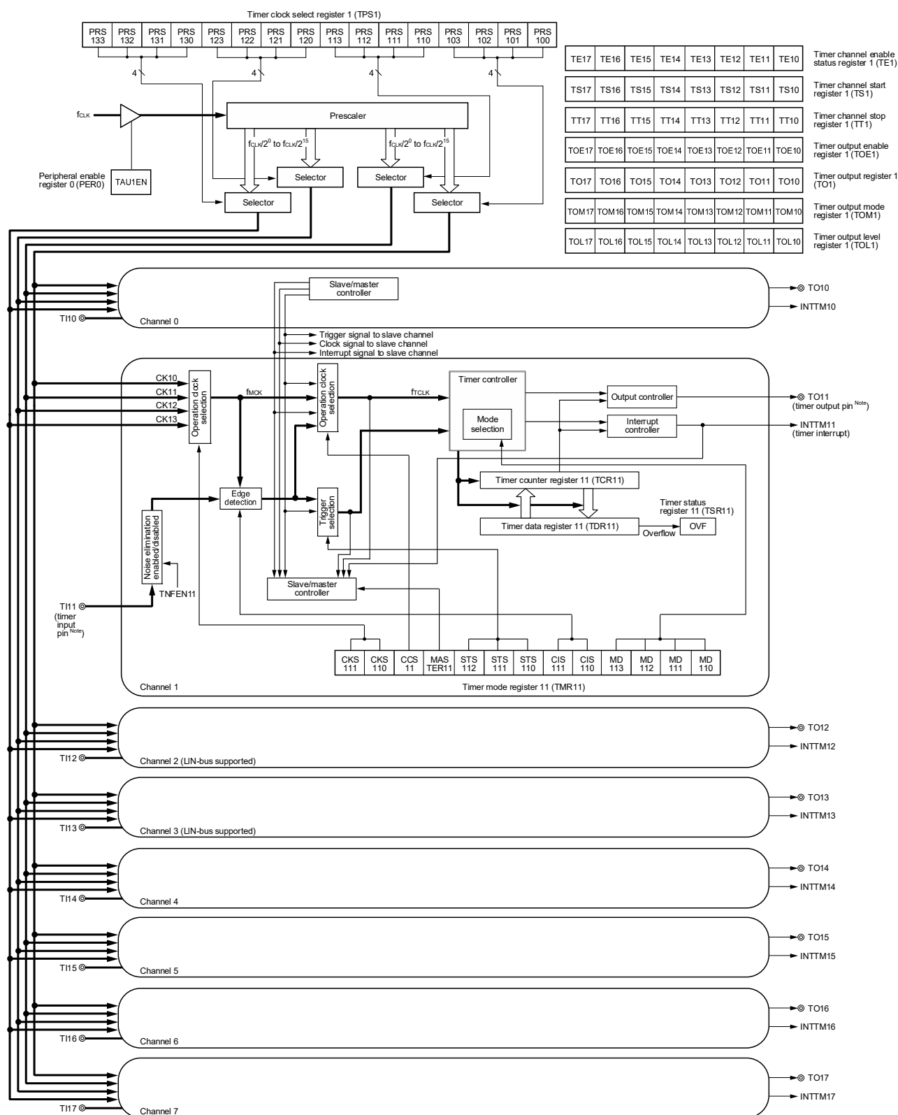
Figure 6-3. Block Diagram of Timer Array Unit 1
