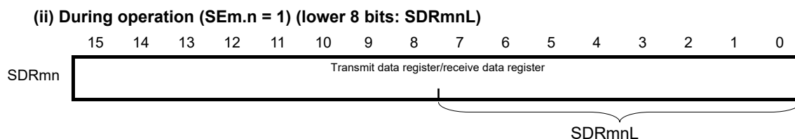
Figure 12-65. Example of Contents of Registers for Slave Transmission/Reception of 3-Wire Serial I/O (CSI00, CSI01, CSI10) (2/2)
