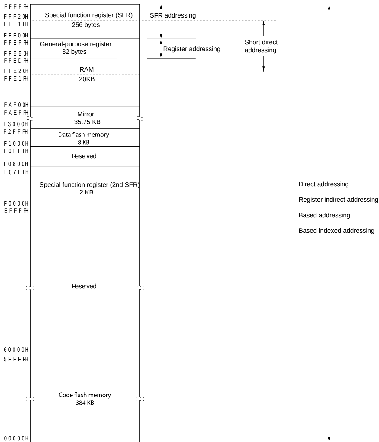
Figure 3-18. Correspondence Between Data Memory and Addressing (R5F10DPK, R5F10DSK)
