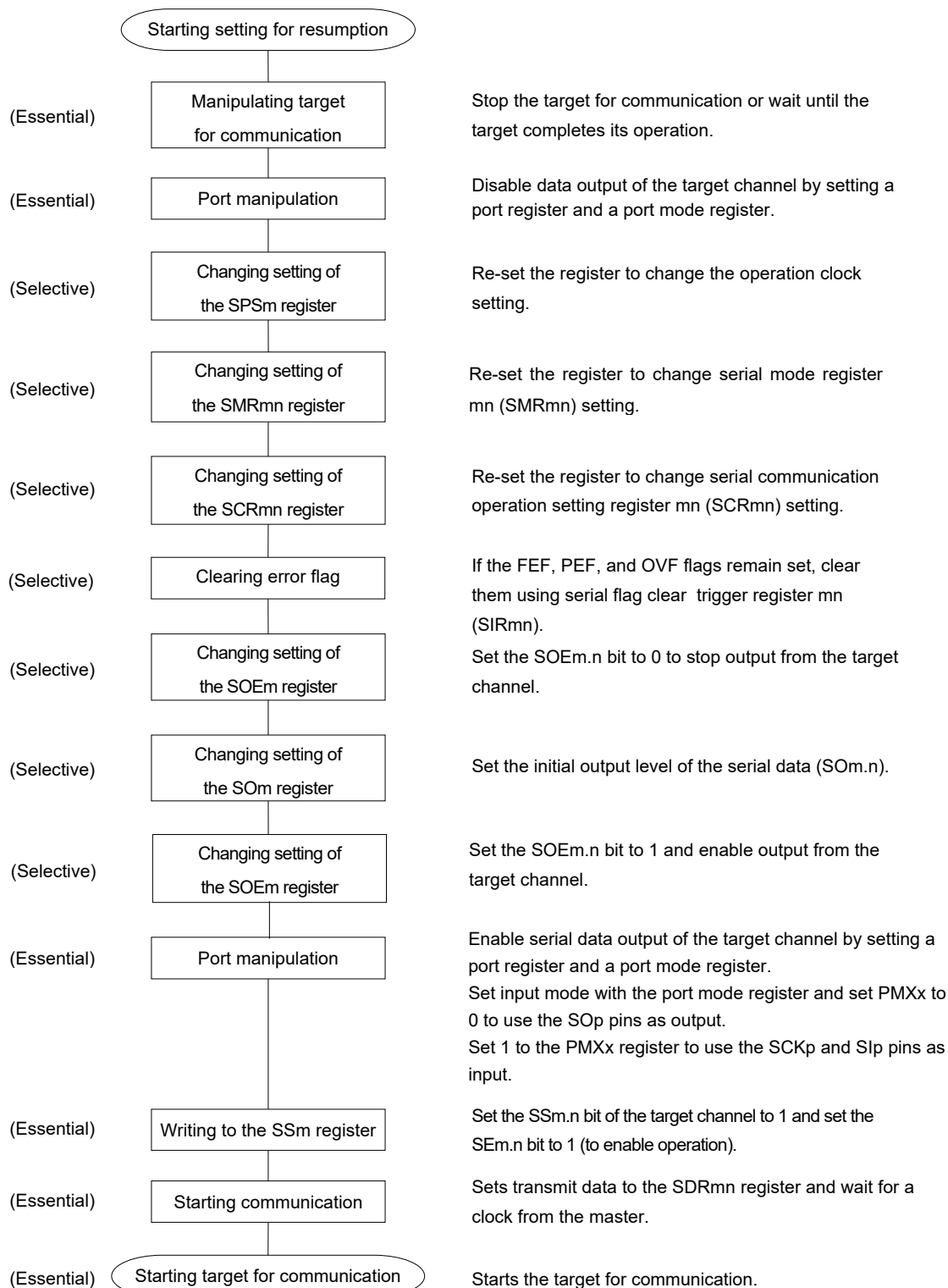
Figure 12-68. Procedure for Resuming Slave Transmission/Reception
