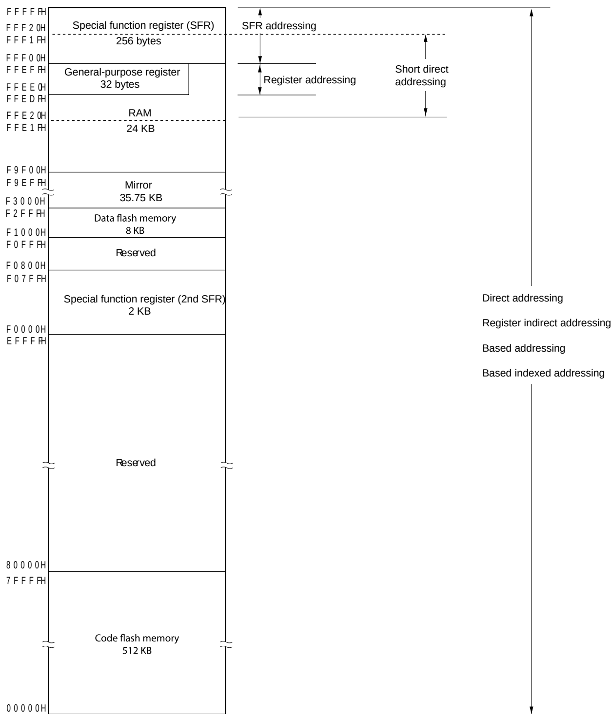
Figure 3-19. Correspondence Between Data Memory and Addressing (R5F10DPL, R5F10DSL)
