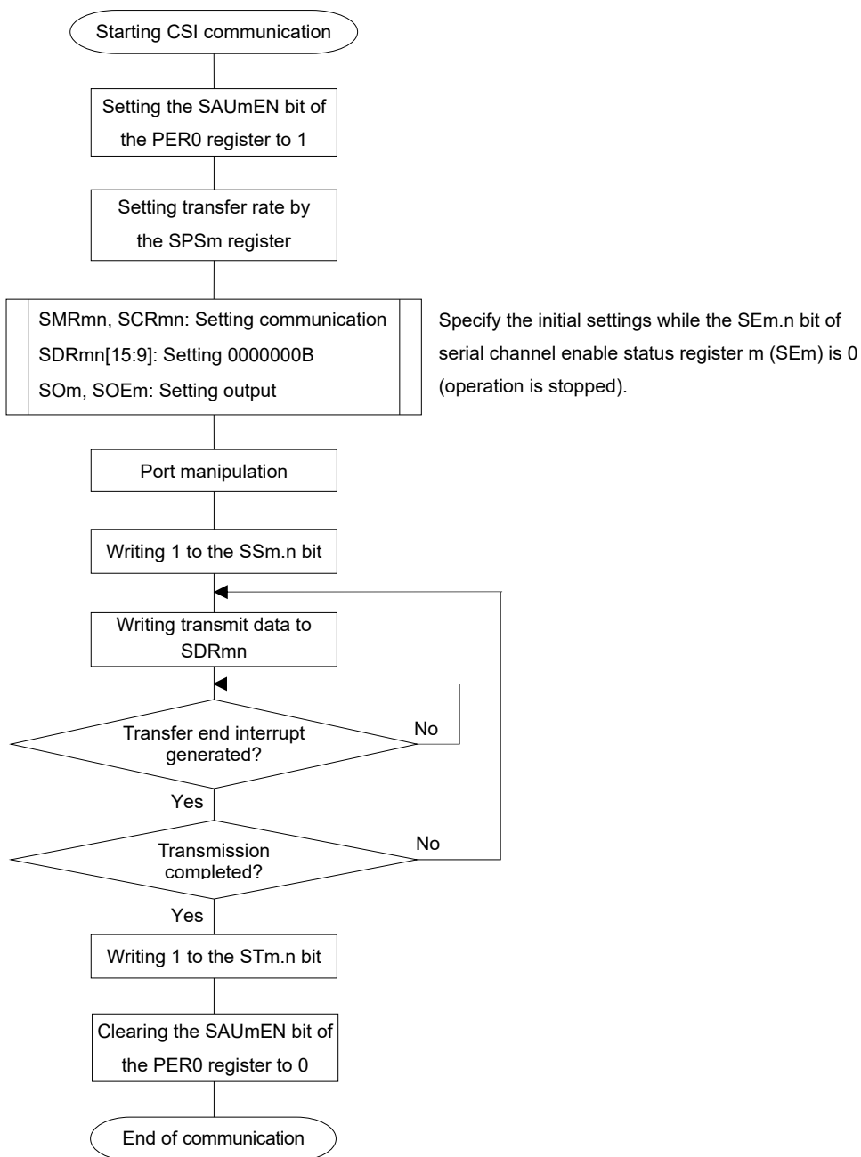
Figure 12-56. Flowchart of Slave Transmission (in Single-Transmission Mode)
