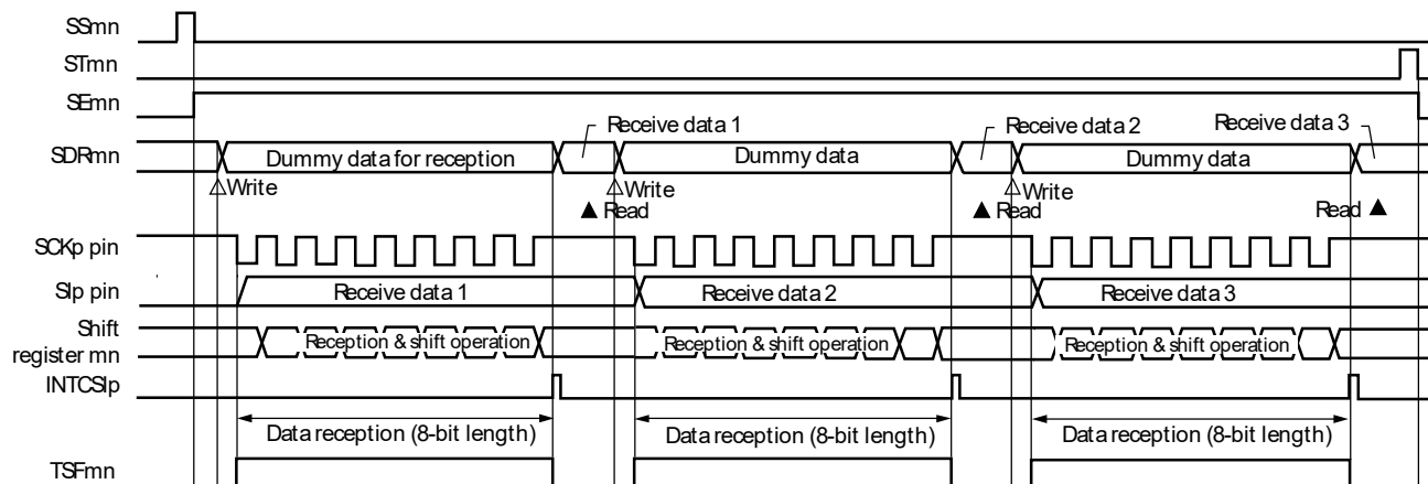
Figure 12-39. Timing Chart of Master Reception (in Single-Reception Mode) (Type 1: DAPmn = 0, CKPmn = 0)
