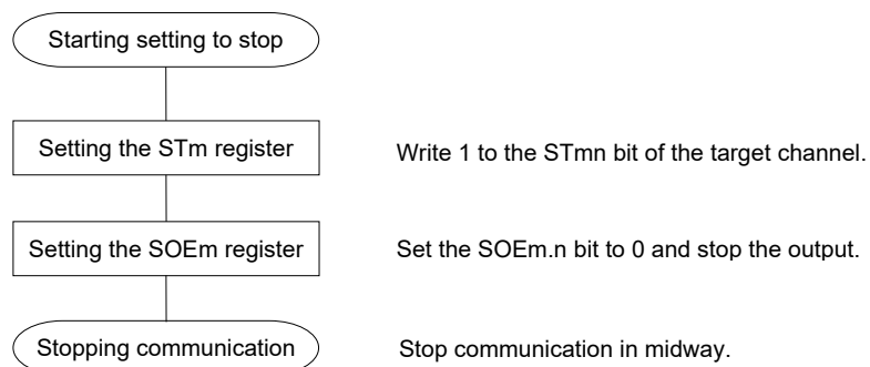
Figure 12-76. Procedure for Stopping UART Transmission
