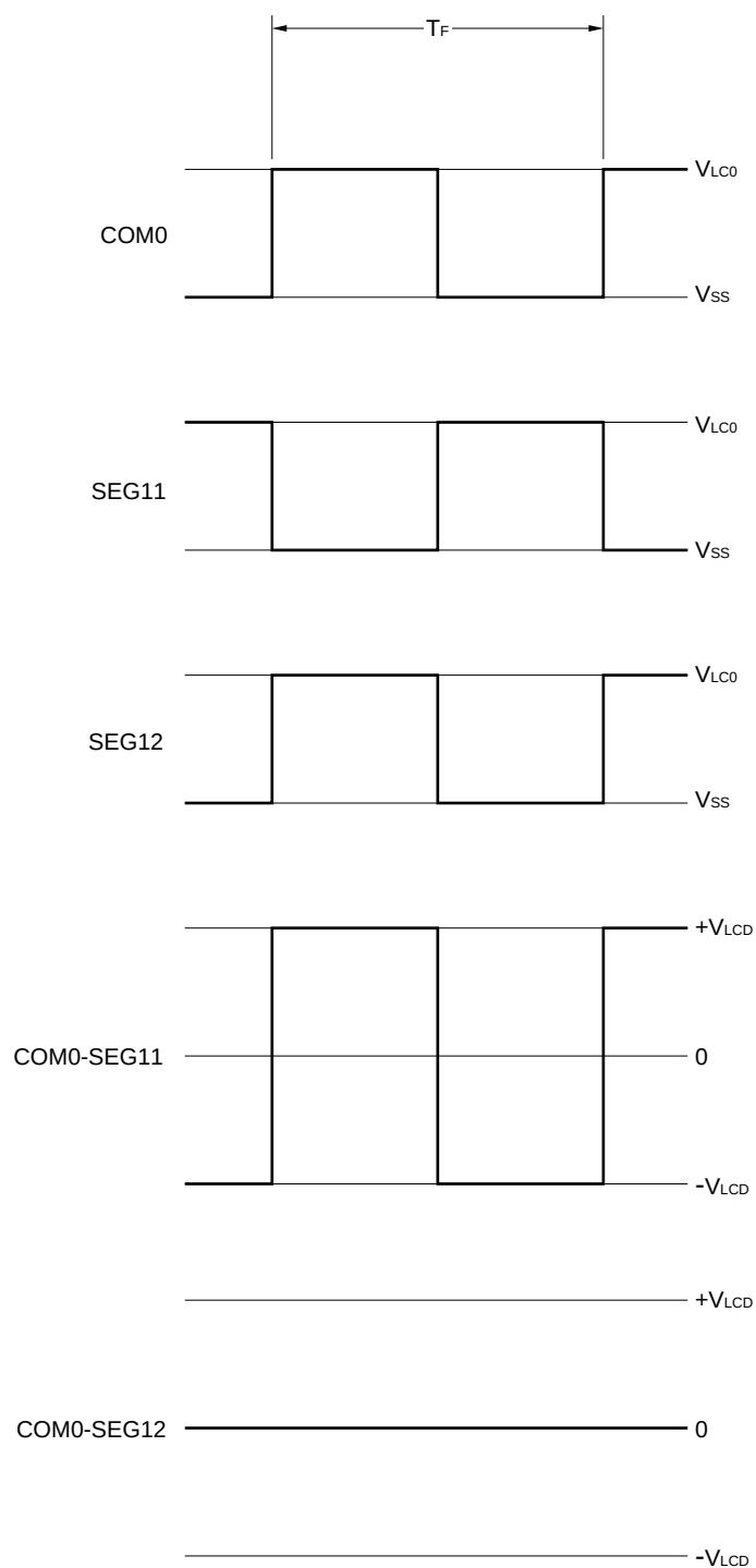
Figure 16-20. Static LCD Drive Waveform Examples
