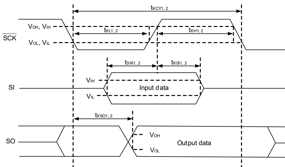
<R> Figure 33-8. CSI mode serial transfer timing (When DAPmn = 0 and CKPmn = 1, or DAPmn = 1 and CKPmn = 0.)
