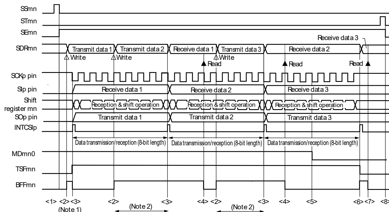
Figure 12-49. Timing Chart of Master Transmission/Reception (in Continuous Transmission/Reception Mode) (Type 1: DAPmn = 0, CKPmn = 0)
