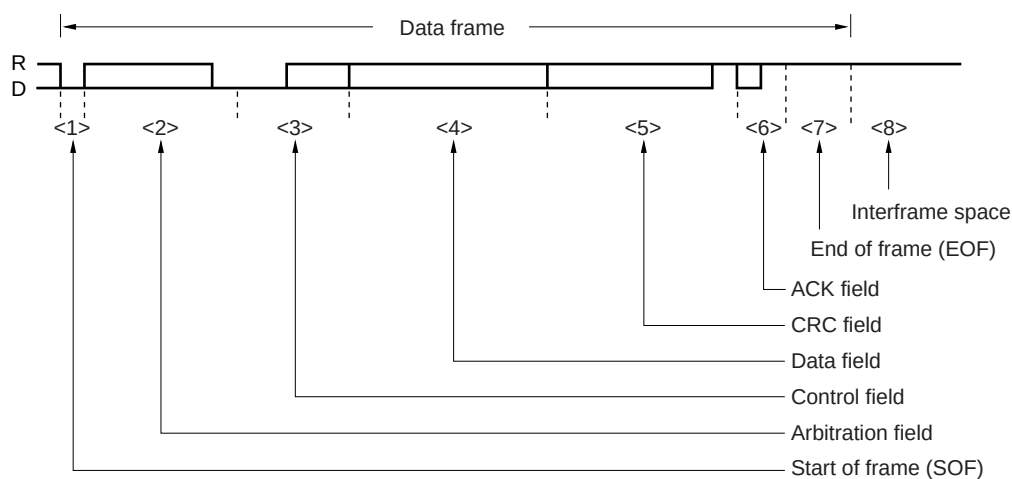
Figure 14-3. Data Frame
