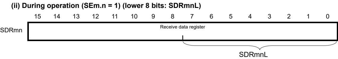
Figure 12-59. Example of Contents of Registers for Slave Reception of 3-Wire Serial I/O (CSI00, CSI01, CSI10) (2/2)
