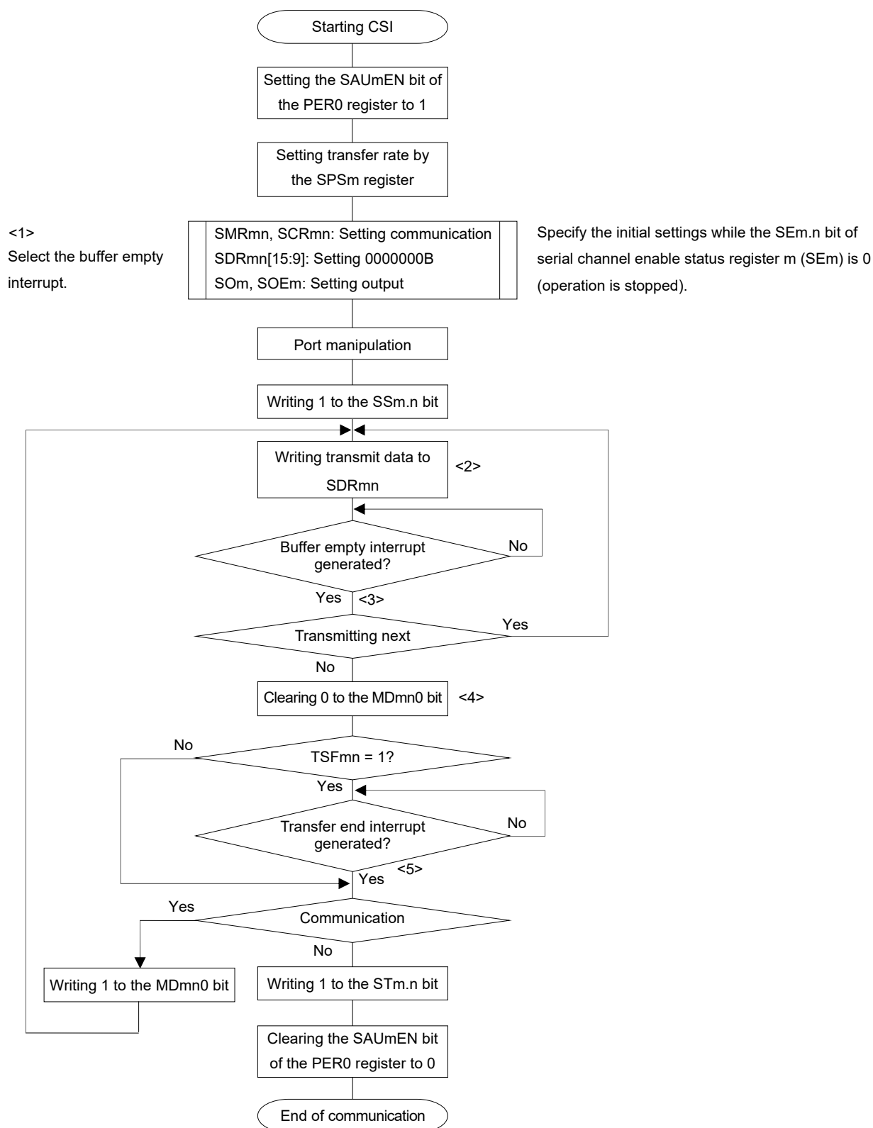
Figure 12-58. Flowchart of Slave Transmission (in Continuous Transmission Mode)
