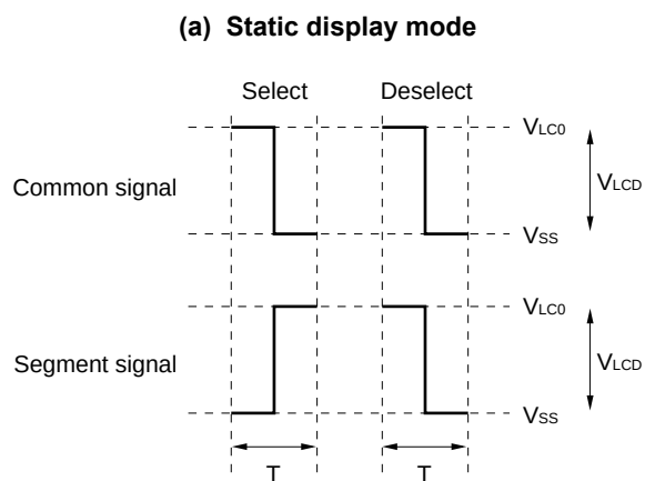
Figure 16-17. Voltages and Phases of Common and Segment Signals
