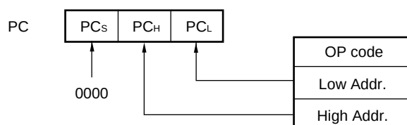
Figure 3-28. Example of CALL !addr16/BR !addr16
