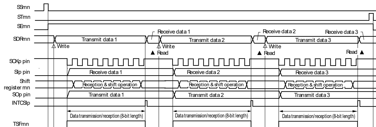
Figure 12-69. Timing Chart of Slave Transmission/Reception (in Single-Transmission/Reception Mode) (Type 1: DAPmn = 0, CKPmn = 0)
