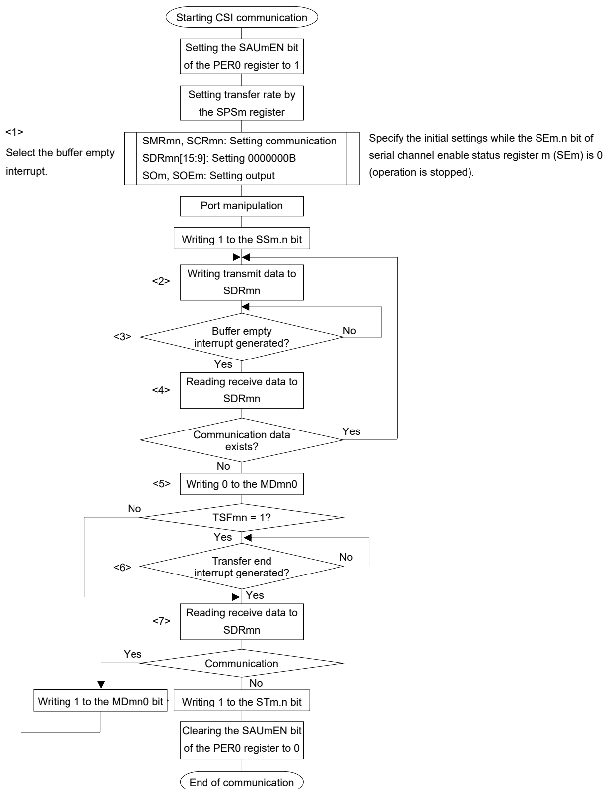
Figure 12-72. Flowchart of Slave Transmission/Reception (in Continuous Transmission/Reception Mode)
