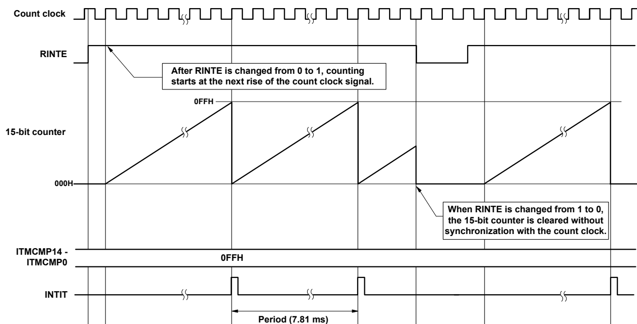
Figure 8-5. Interval Timer Operation Timing (ITMCMP14 to ITMCMP0 = 0FFH, count clock: f_{SUB} = 32.768 kHz)
