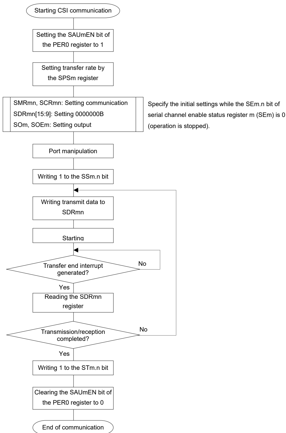
Figure 12-70. Flowchart of Slave Transmission/Reception (in Single- Transmission/Reception Mode)
