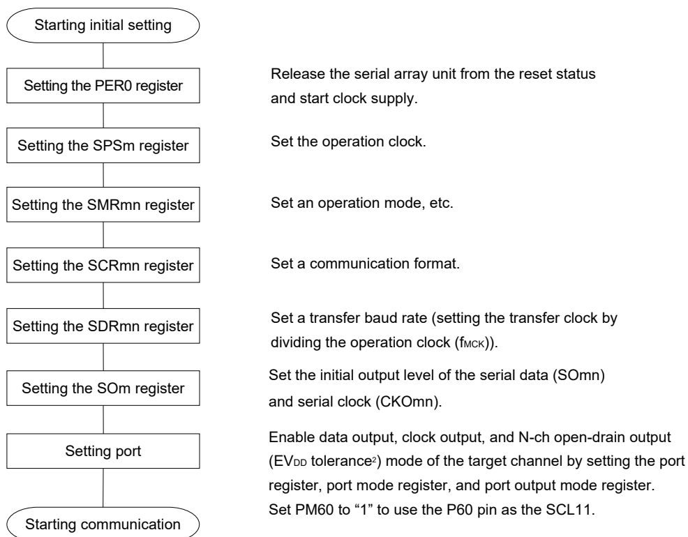
Figure 12-92. Initial Setting Procedure for Address Field Transmission
