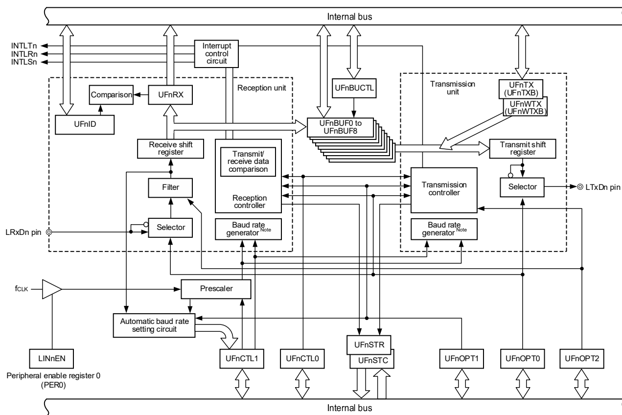
Figure 13-1. Block Diagram of Asynchronous Serial Interface LIN-UART
