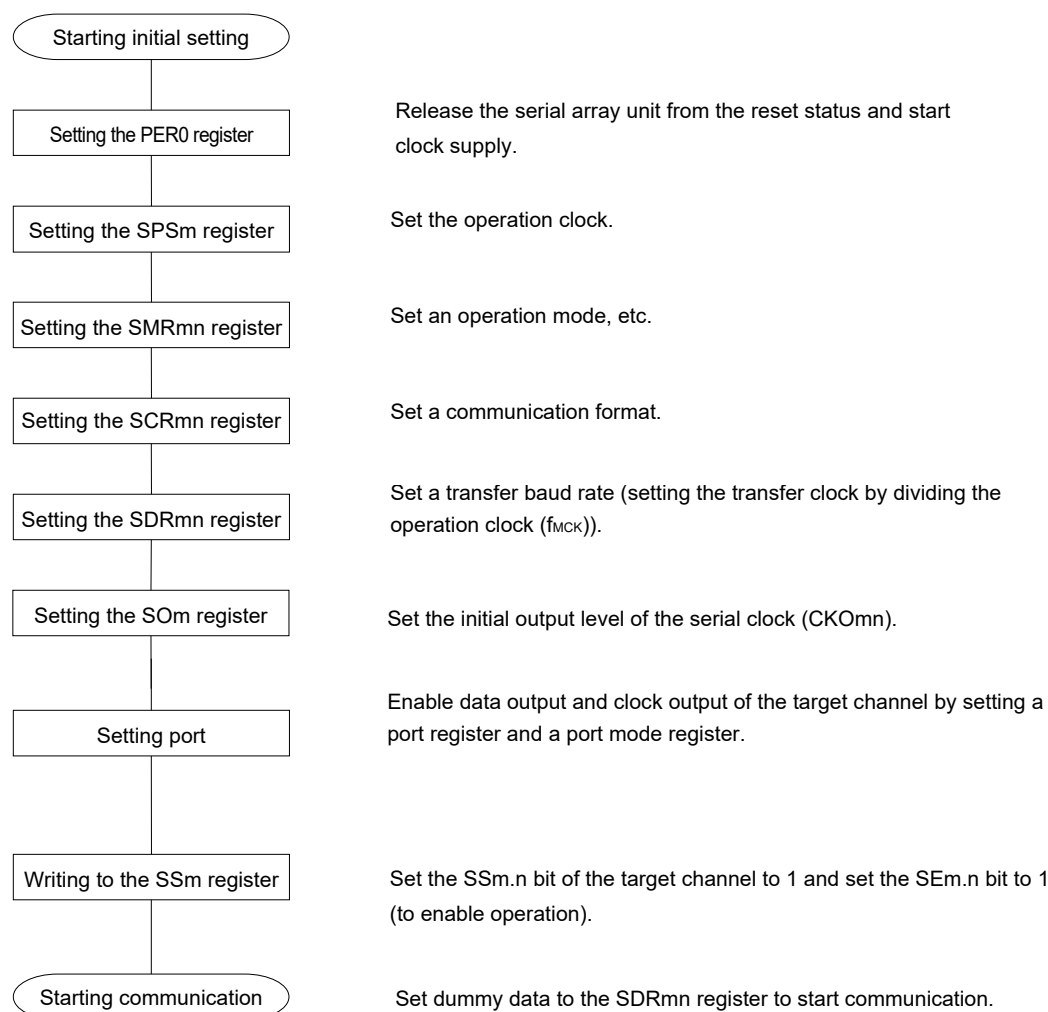
Figure 12-36. Initial Setting Procedure for Master Reception
