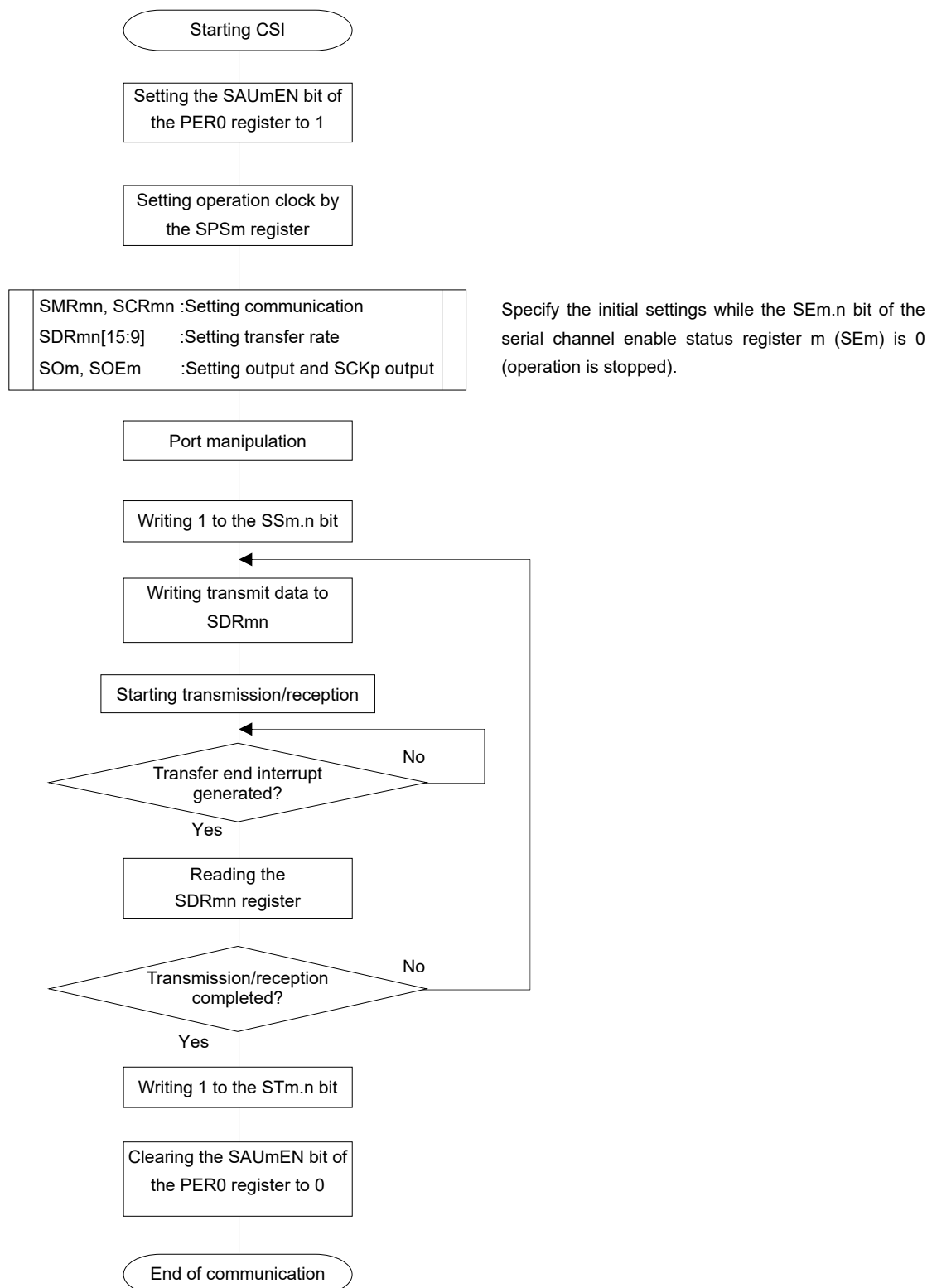
Figure 12-48. Flowchart of Master Transmission/Reception (in Single- Transmission/Reception Mode)
