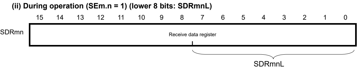
Figure 12-35. Example of Contents of Registers for Master Reception of 3-Wire Serial I/O (CSI00, CSI01, CSI10) (2/2)
