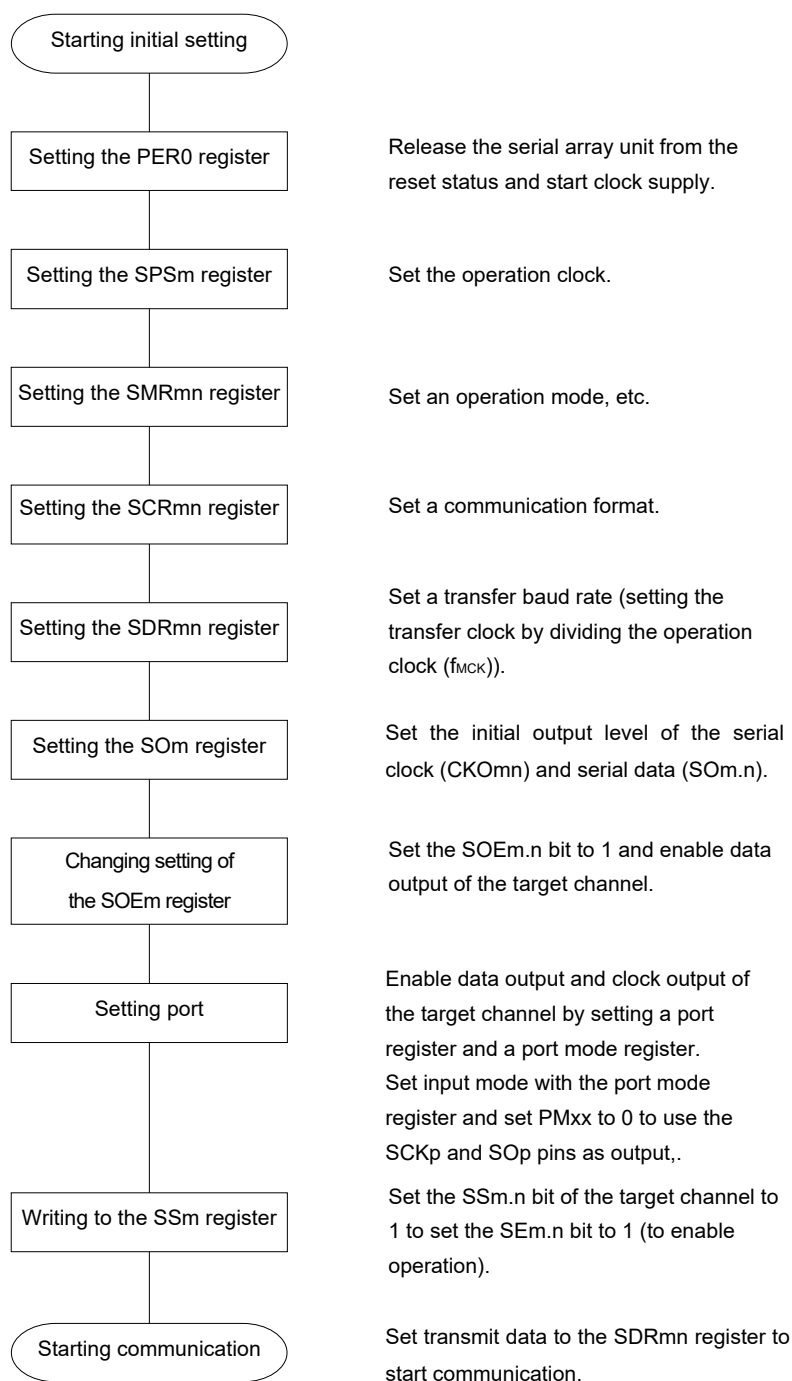
Figure 12-28. Initial Setting Procedure for Master Transmission
