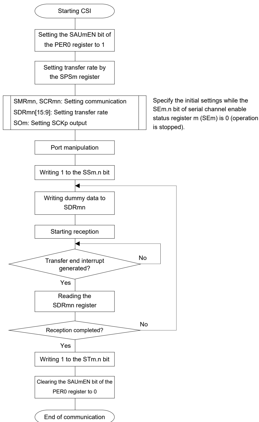
Figure 12-40. Flowchart of Master Reception (in Single-Reception Mode)
