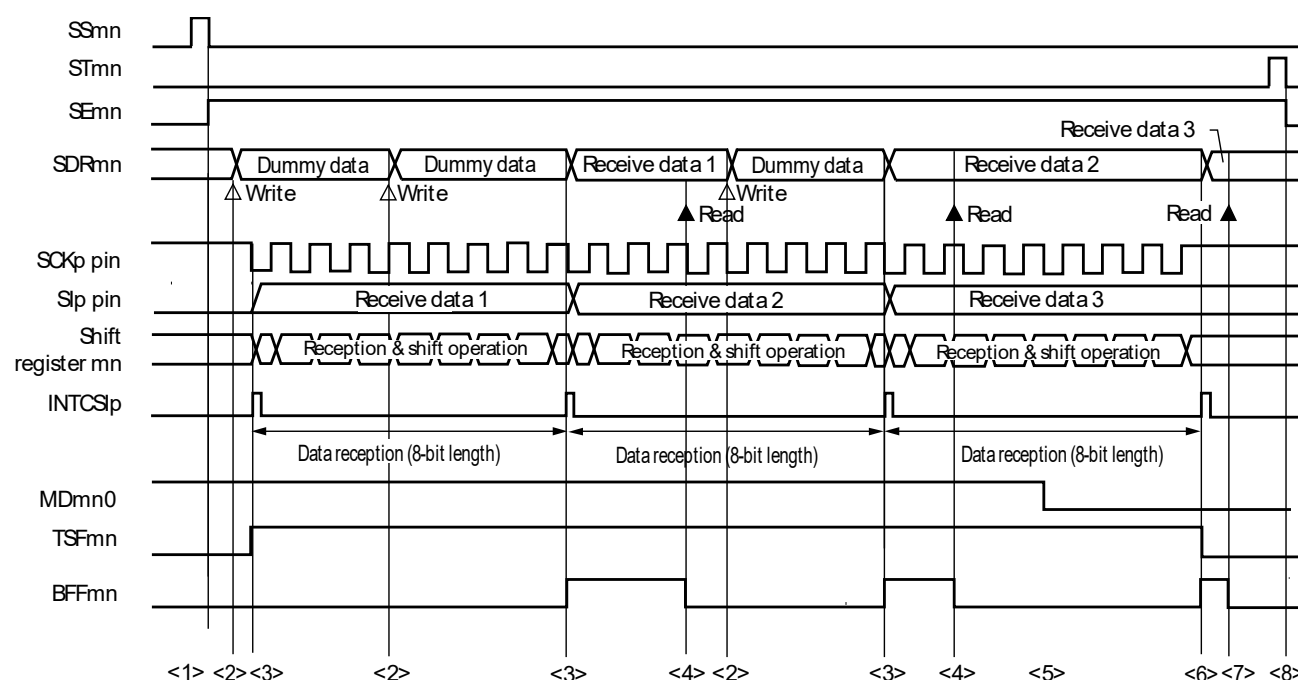
Figure 12-41. Timing Chart of Master Reception (in Continuous Reception Mode) (Type 1: DAPmn = 0, CKPmn = 0)
