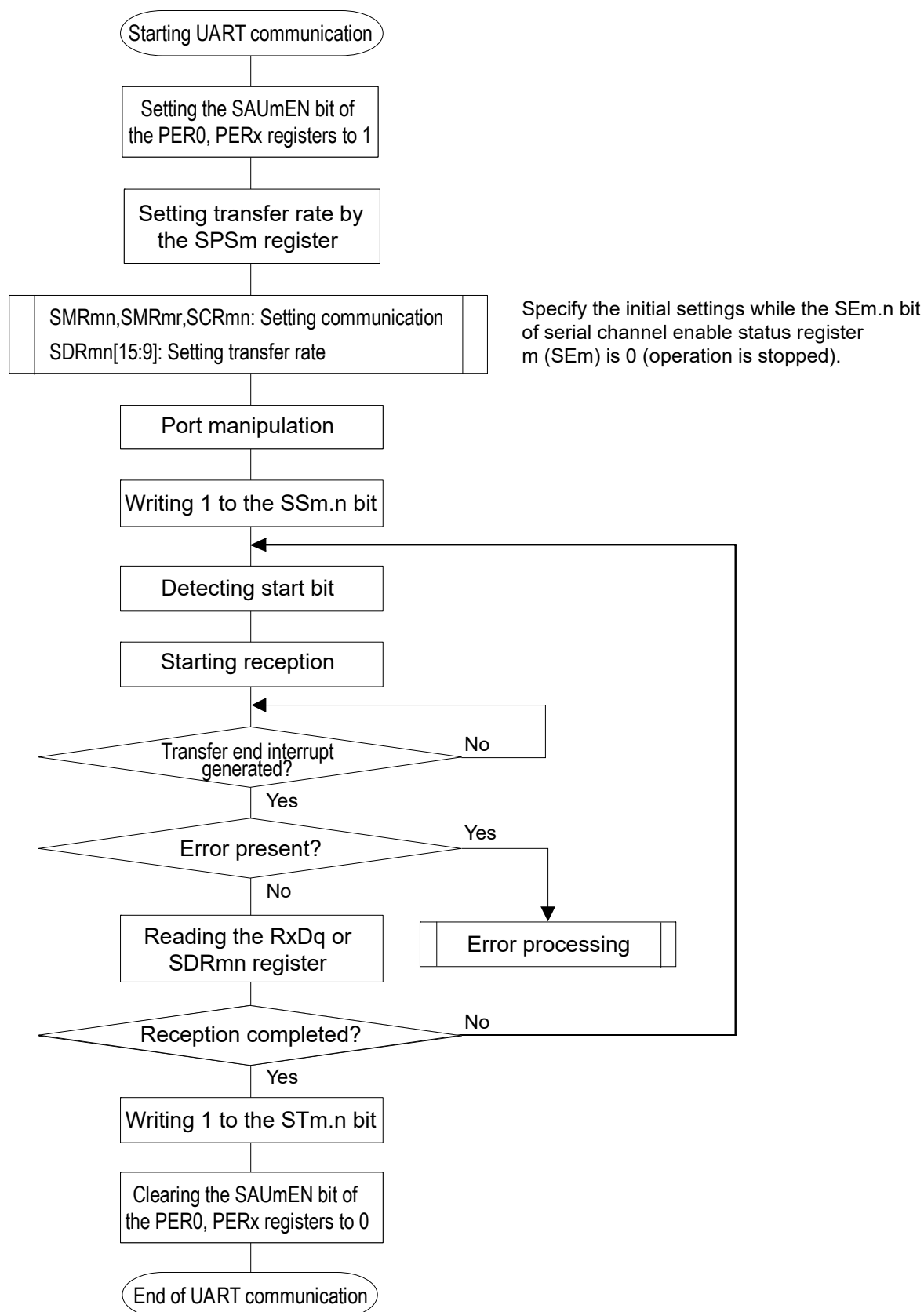
Figure 12-87. Flowchart of UART Reception
