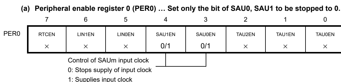
Figure 12-25. Peripheral Enable Registers 0 (PER0) Setting When Stopping the Operation by Units
