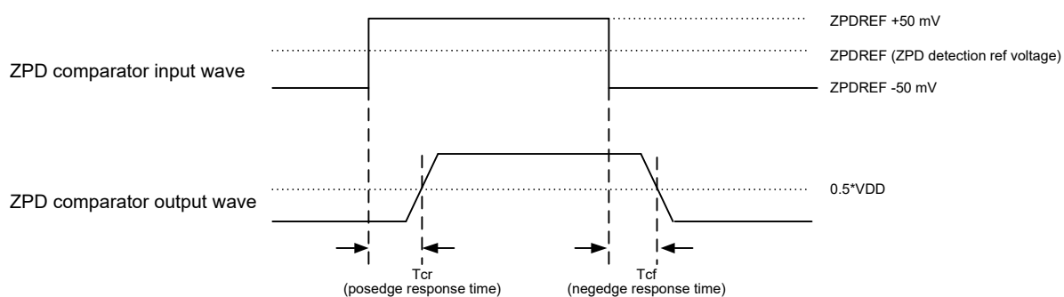
Figure 33-15. ZPD timing
