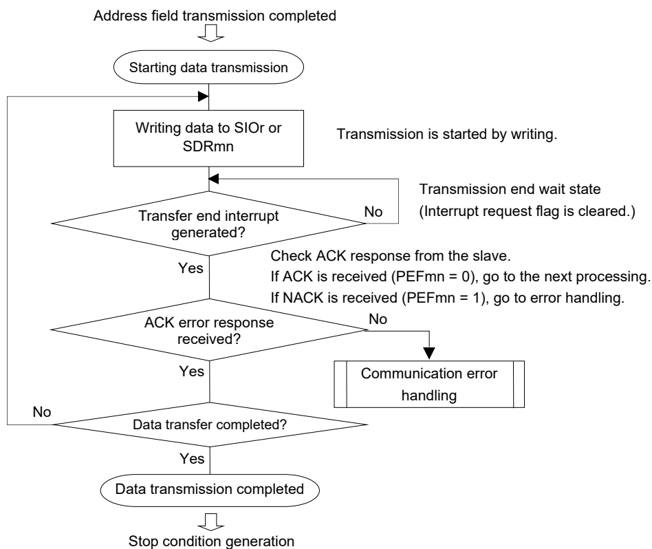
Figure 12-97. Flowchart of Data Transmission
