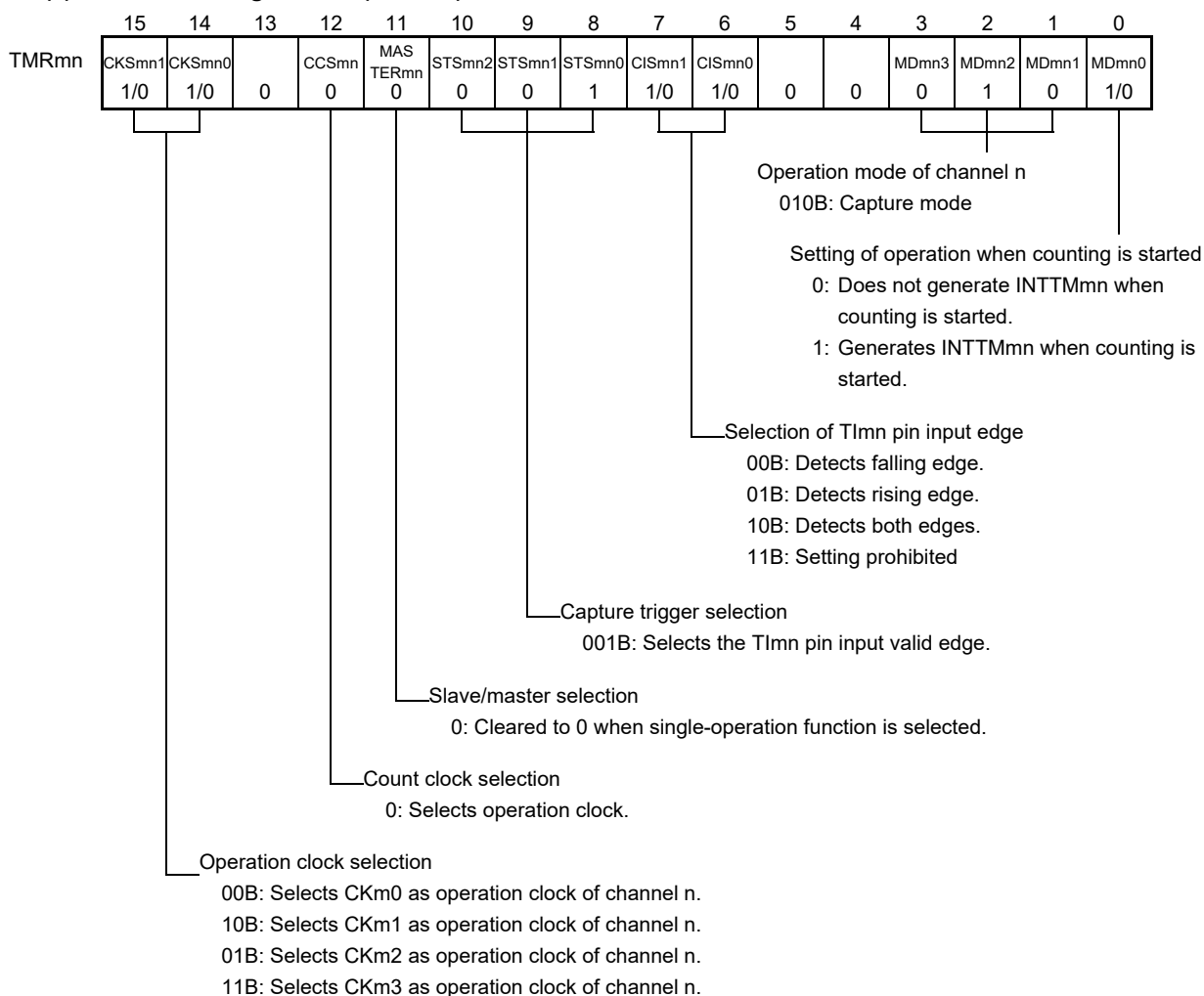
Figure 6-65. Example of Set Contents of Registers to Measure Input Pulse Interval (1/2)
