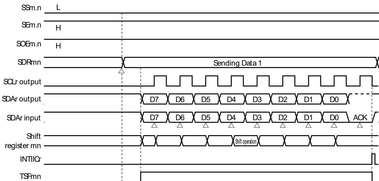
Figure 12-96. Timing Chart of Data Transmission
