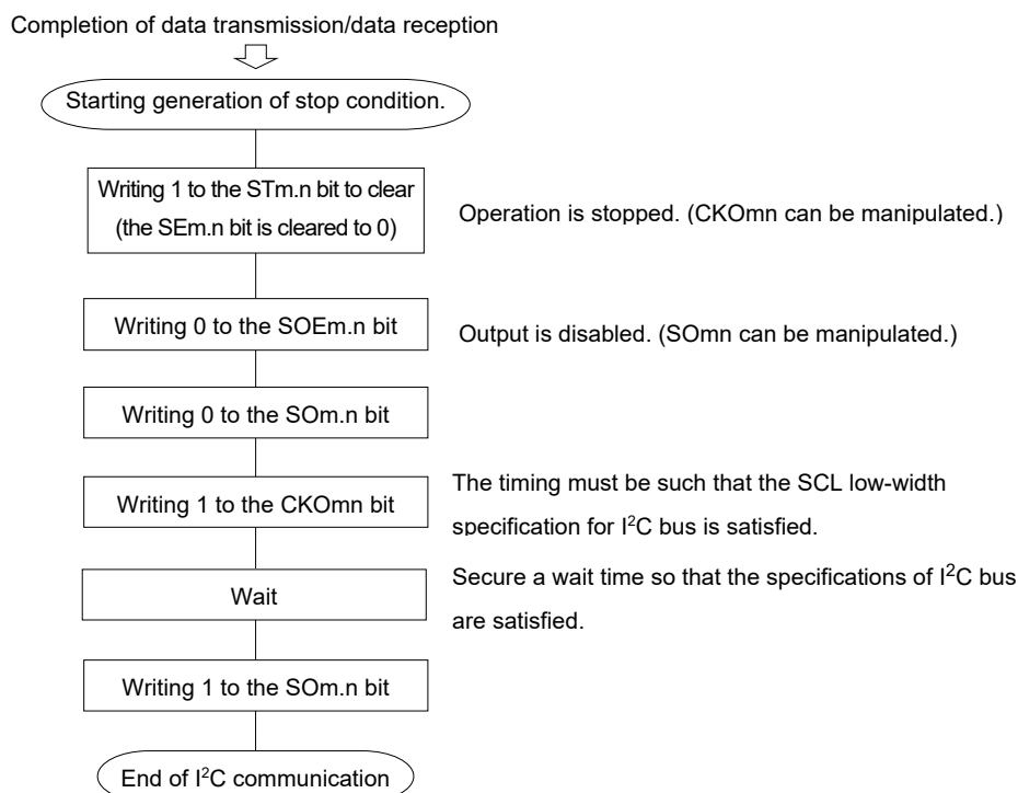
Figure 12-102. Flowchart of Stop Condition Generation
