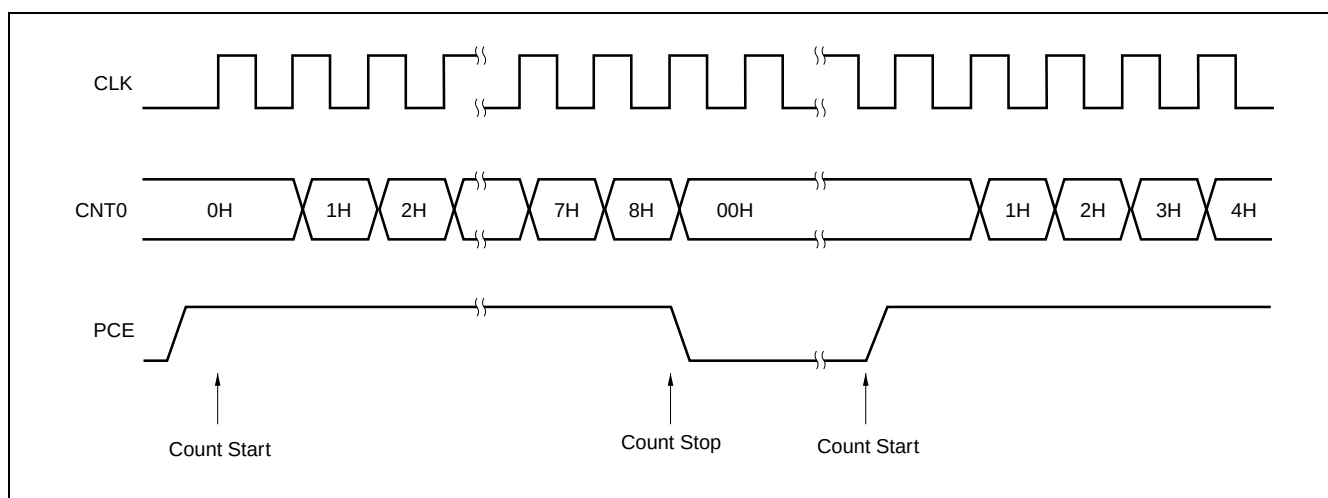
Figure 15-11. Restart Timing after Count Stop (Count Start—Count Stop—Count Start)
