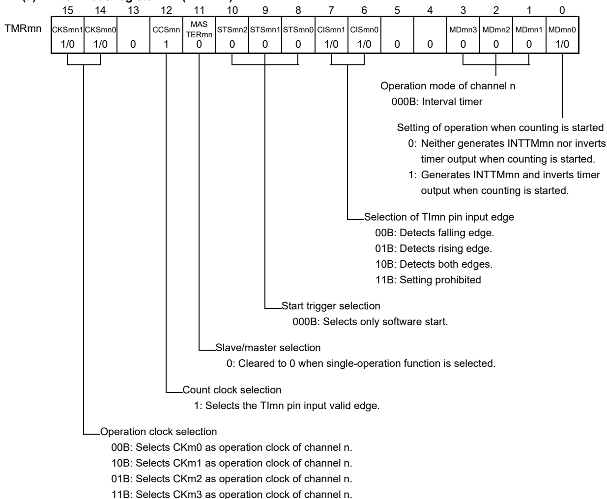
Figure 6-61. Example of Set Contents of Registers When Frequency Divider Is Used (1/2)
