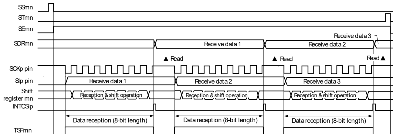
Figure 12-63. Timing Chart of Slave Reception (in Single-Reception Mode) (Type 1: DAPmn = 0, CKPmn = 0)
