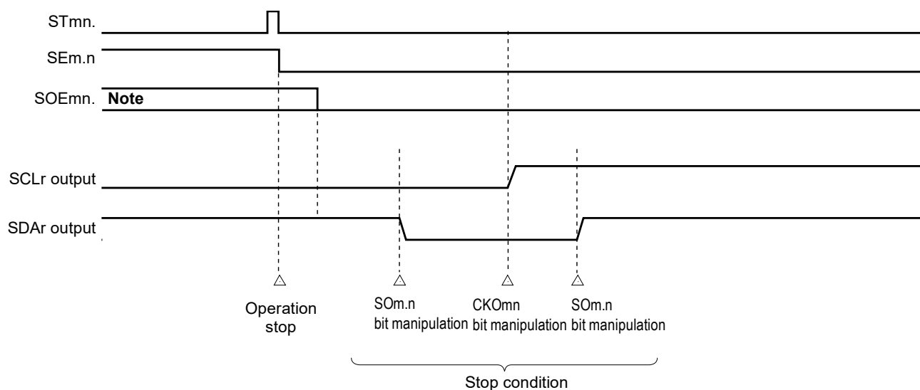
Figure 12-101. Timing Chart of Stop Condition Generation
