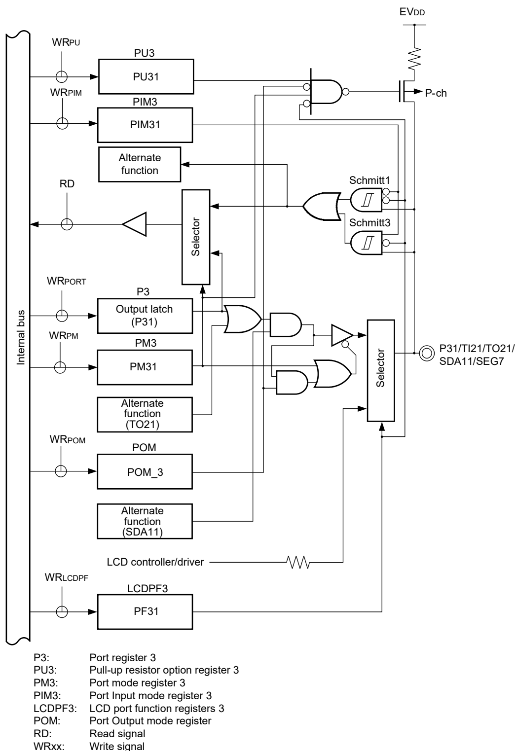
Figure 4-14. Block Diagram of P31
