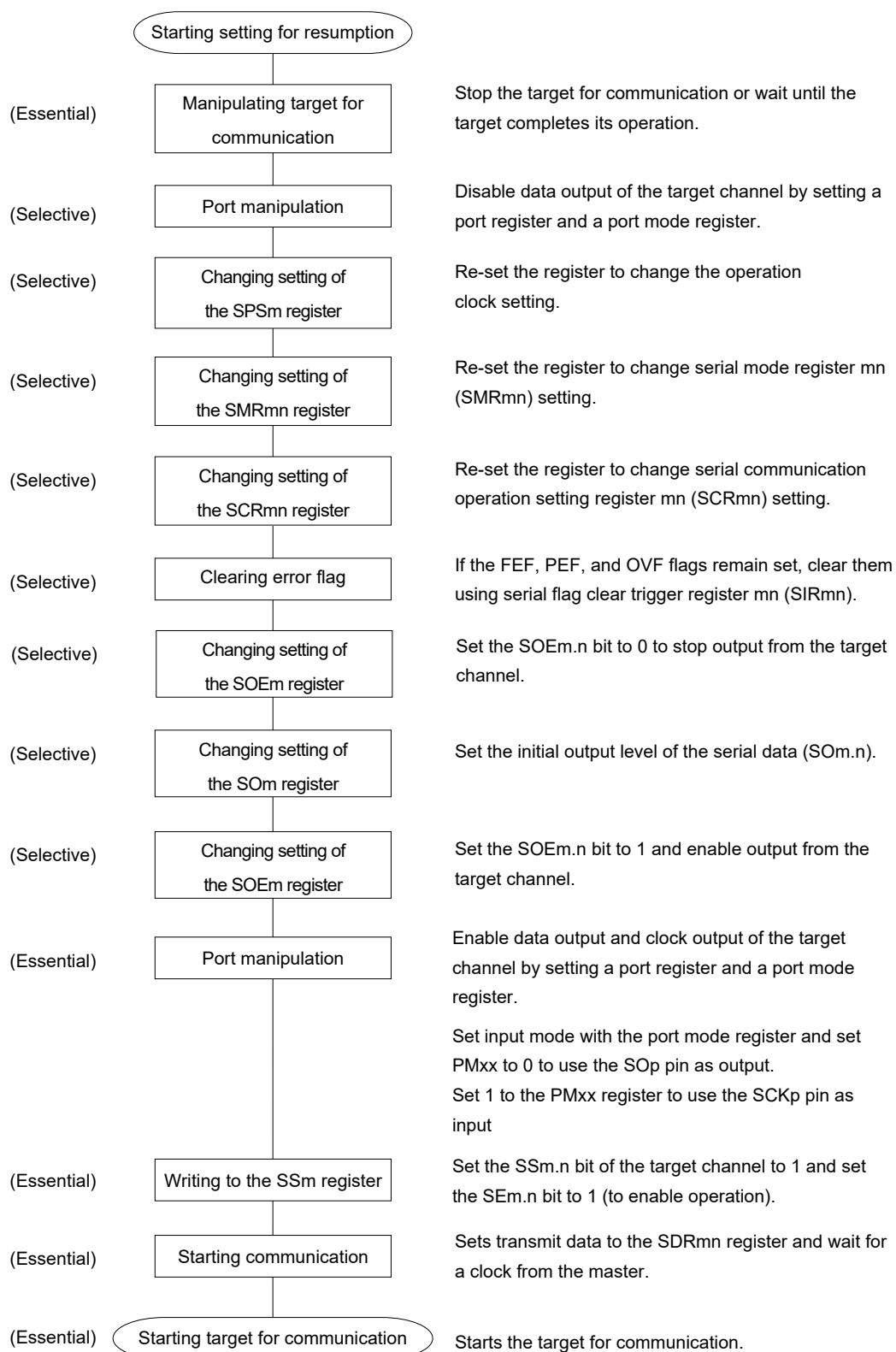
Figure 12-54. Procedure for Resuming Slave Transmission
