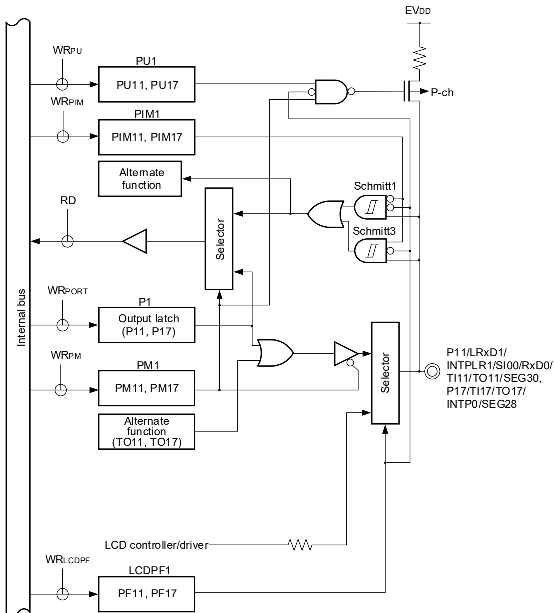
Figure 4-8. Block Diagram of P11, P17
