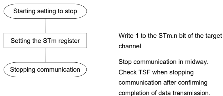
Figure 12-61. Procedure for Stopping Slave Reception
