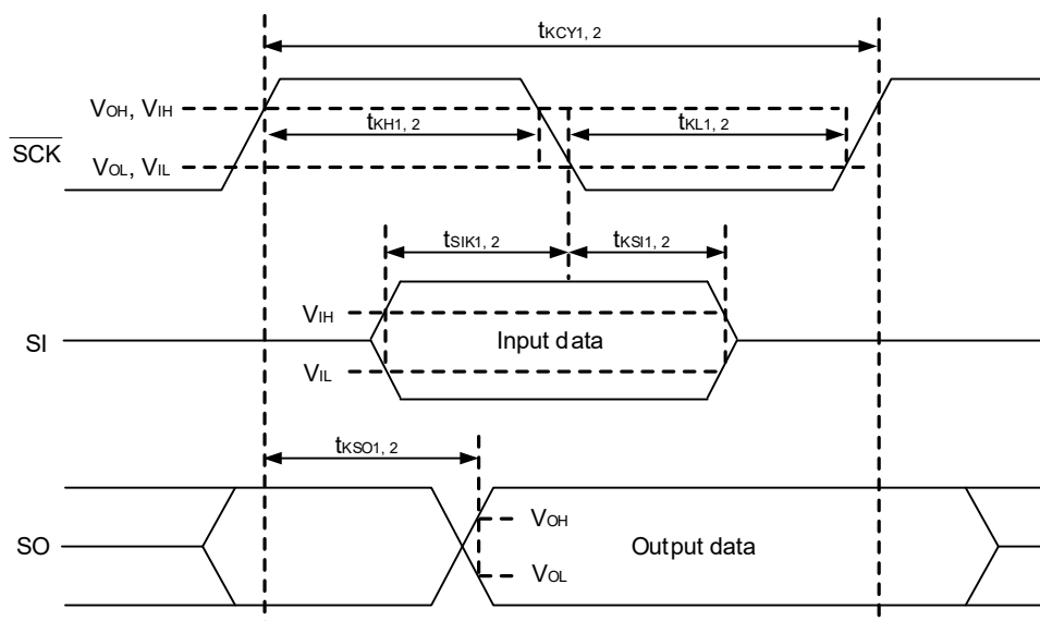
<R> Figure 34-8. CSI mode serial transfer timing (When DAPmn = 0 and CKPmn = 1, or DAPmn = 1 and CKPmn = 0.)
