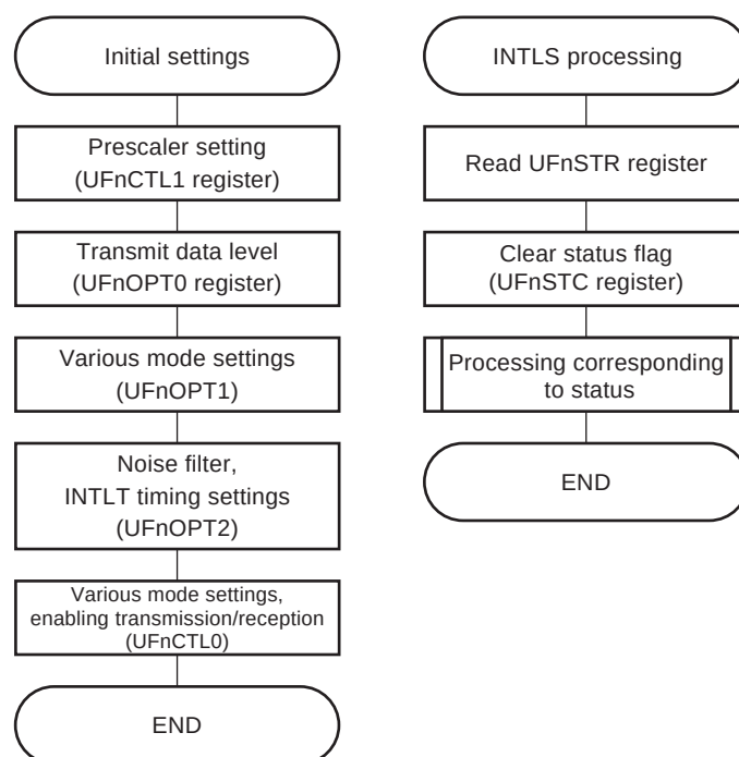
Figure 13-52. Basic Processing Flow Example of LIN Communication Automatic Baud Rate Mode (1/2)
