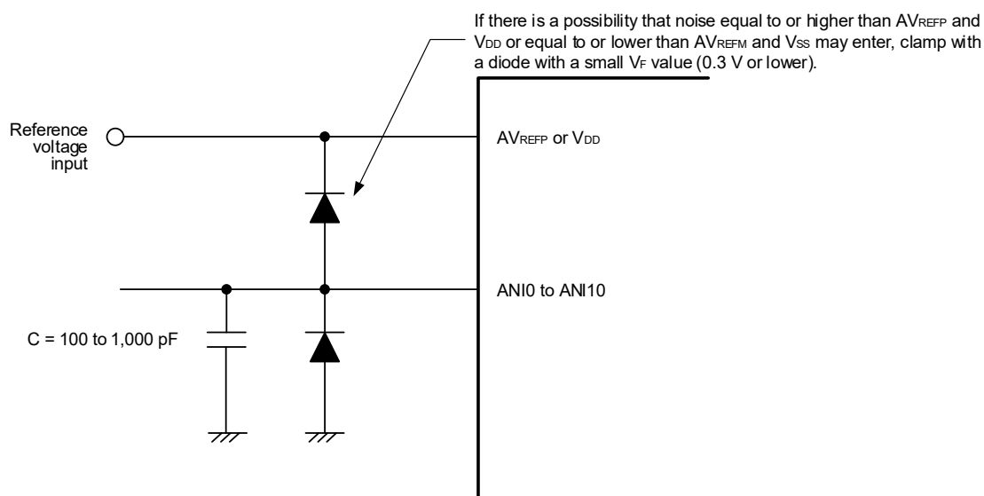
Figure 11-44. Analog Input Pin Connection
