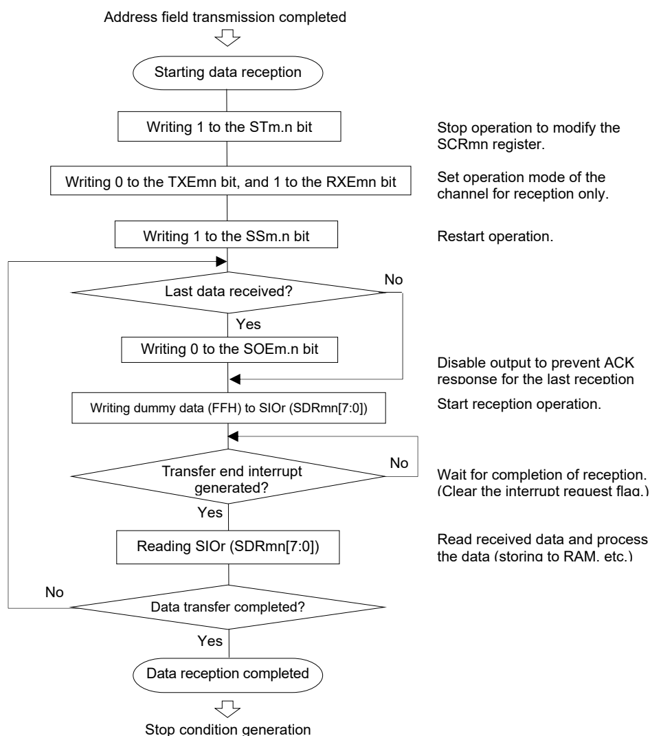
Figure 12-100. Flowchart of Data Reception
