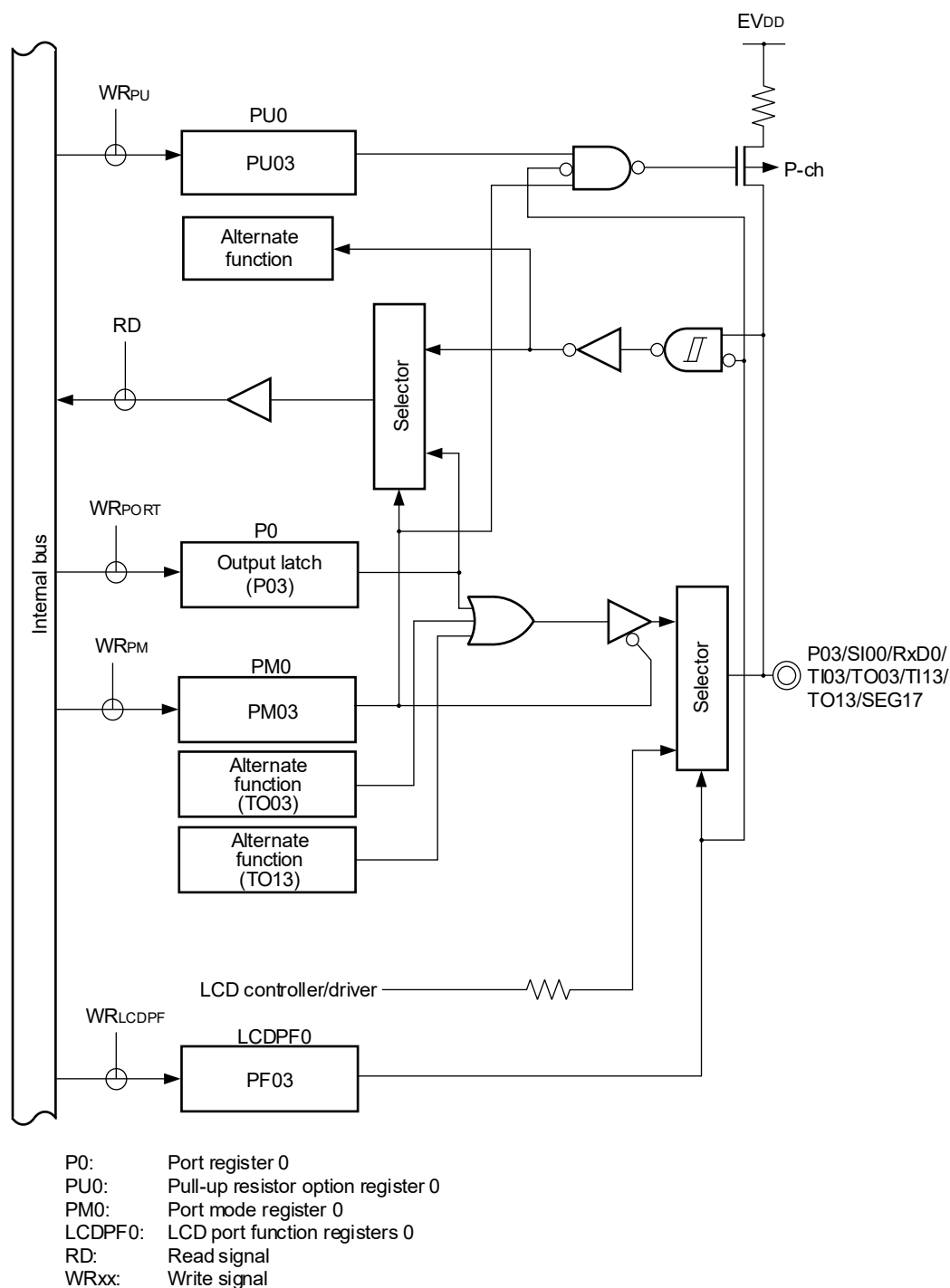
Figure 4-4. Block Diagram of P03
