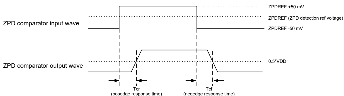
Figure 34-15. ZPD timing
