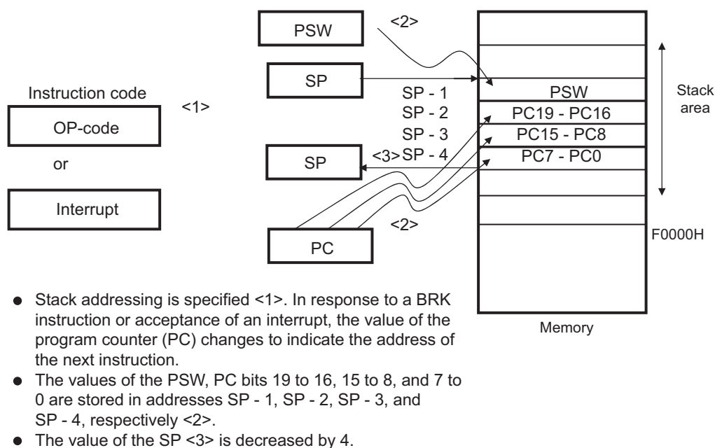
Figure 3-52. Example of Interrupt, BRK
