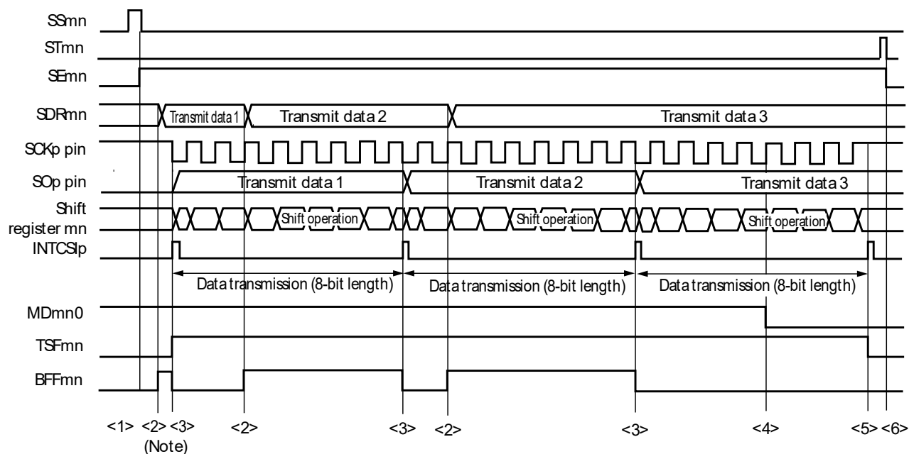
Figure 12-33. Timing Chart of Master Transmission (in Continuous Transmission Mode) (Type 1: DAPmn = 0, CKPmn = 0)
