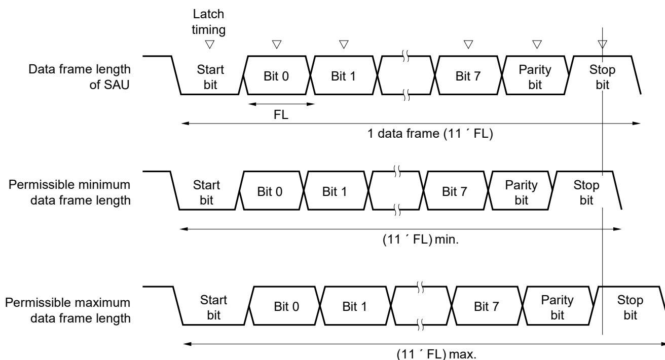
Figure 12-88. Permissible Baud Rate Range for Reception (1 Data Frame Length = 11 Bits)
