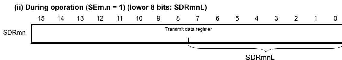
Figure 12-51. Example of Contents of Registers for Slave Transmission of 3-Wire Serial I/O (CSI00, CSI01, CSI10) (2/2)
