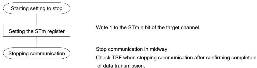
Figure 12-37. Procedure for Stopping Master Reception
