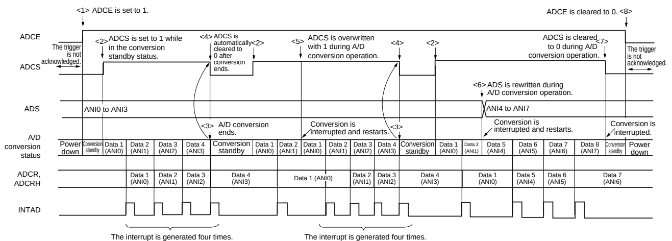
Figure 11-22. Example of Software Trigger Mode (Scan Mode, One-Shot Conversion Mode) Operation Timing
