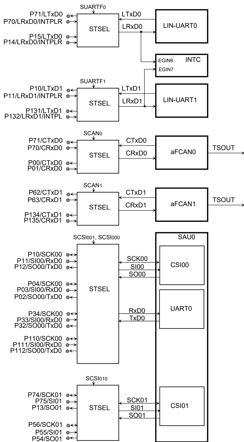
Figure 4-67. Serial unit, SG, and PCL connection (128-pin products) (1/2)
