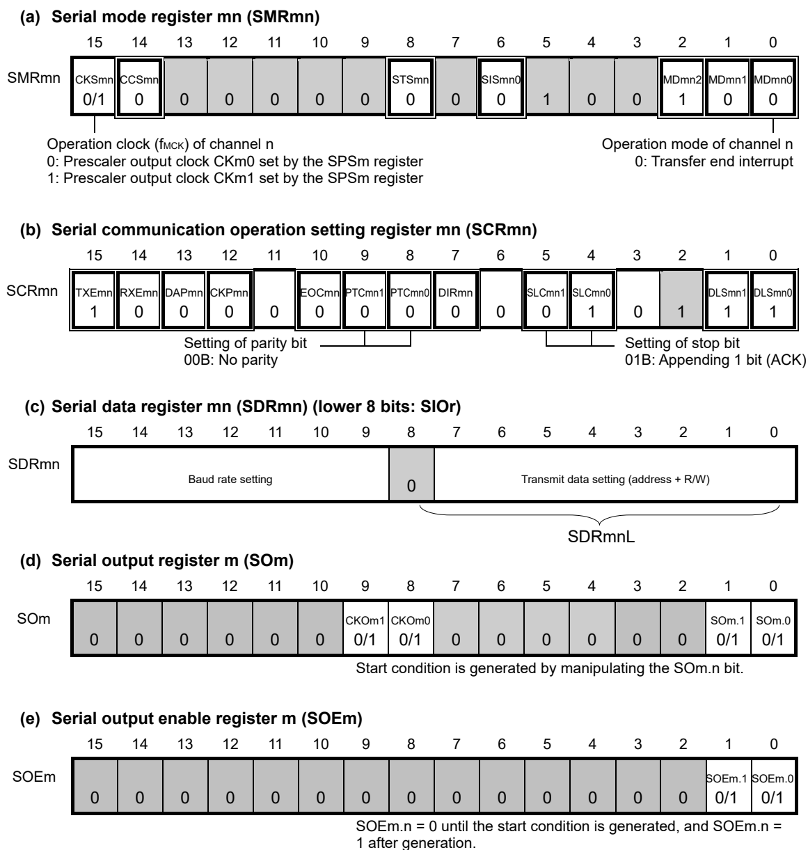
Figure 12-91. Example of Contents of Registers for Address Field Transmission of Simplified I 2 C (IIC11) (1/2)
