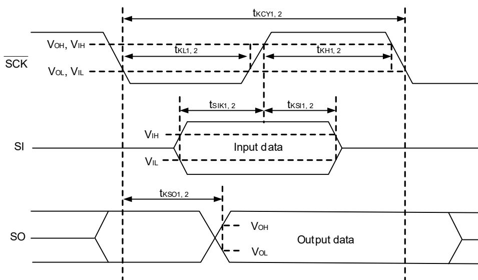
<R> Figure 34-8. CSI mode serial transfer timing (When DAPmn = 0 and CKPmn = 1, or DAPmn = 1 and CKPmn = 0.)
