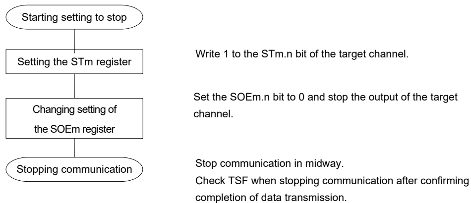
Figure 12-45. Procedure for Stopping Master Transmission/Reception
