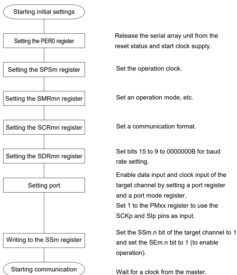
Figure 12-60. Initial Setting Procedure for Slave Reception
