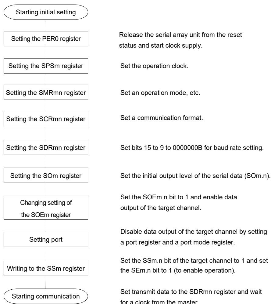
Figure 12-66. Initial Setting Procedure for Slave Transmission/Reception
