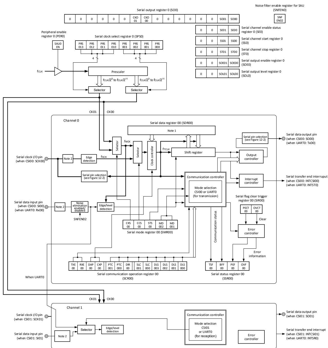
Figure 12-1. Block Diagram of Serial Array Unit 0
