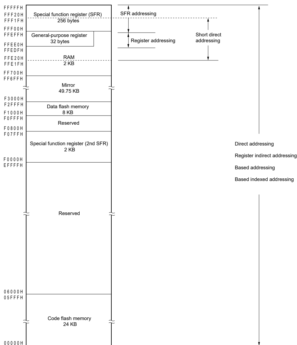
Figure 3-11. Correspondence Between Data Memory and Addressing (R5F10CGB)
