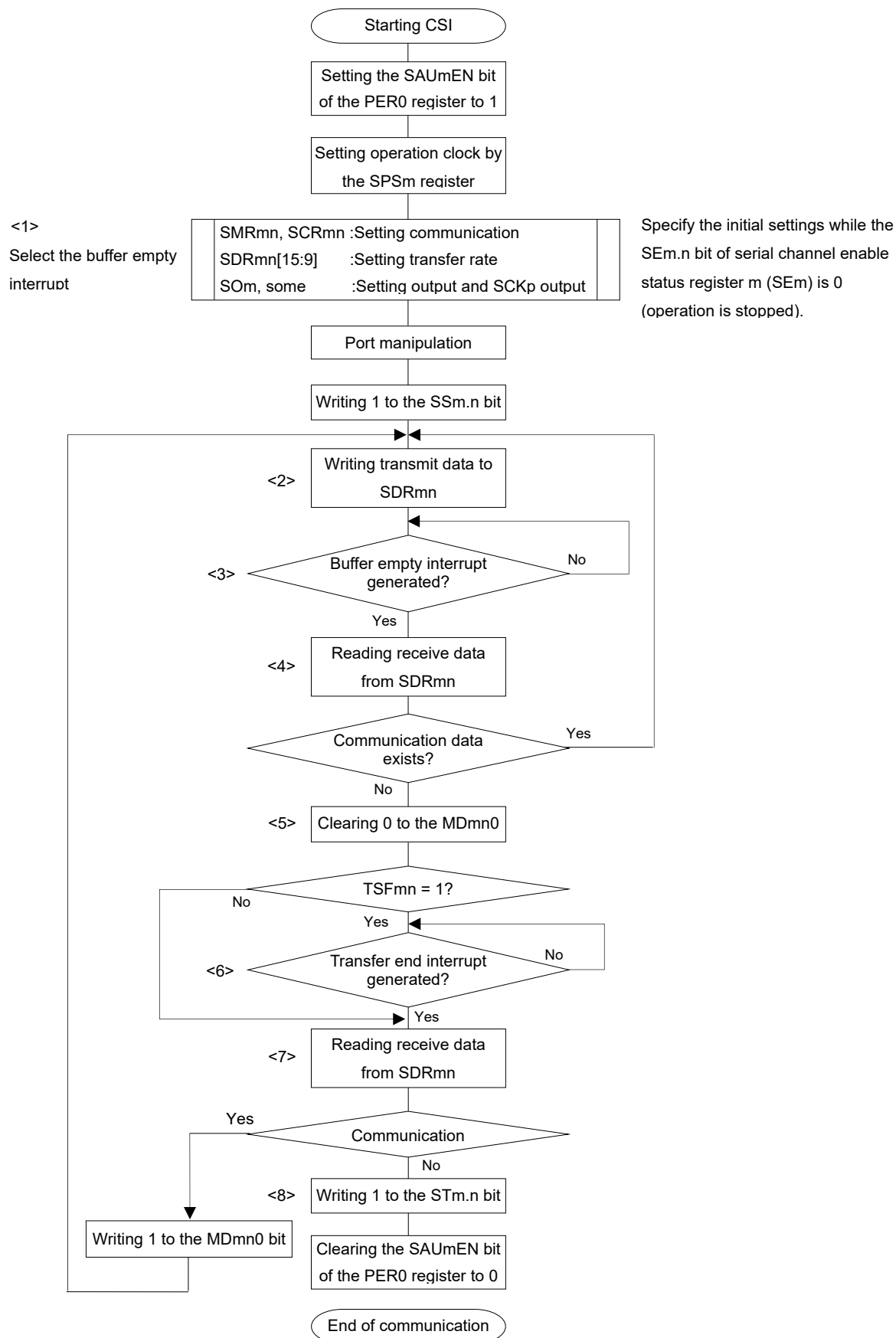
Figure 12-50. Flowchart of Master Transmission/Reception (in Continuous Transmission/Reception Mode)
