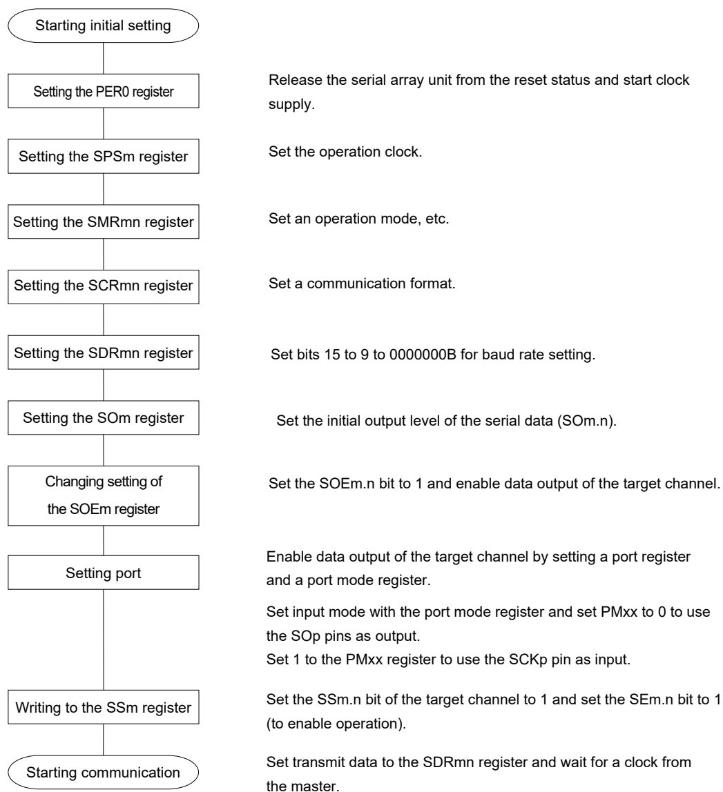
Figure 12-52. Initial Setting Procedure for Slave Transmission
