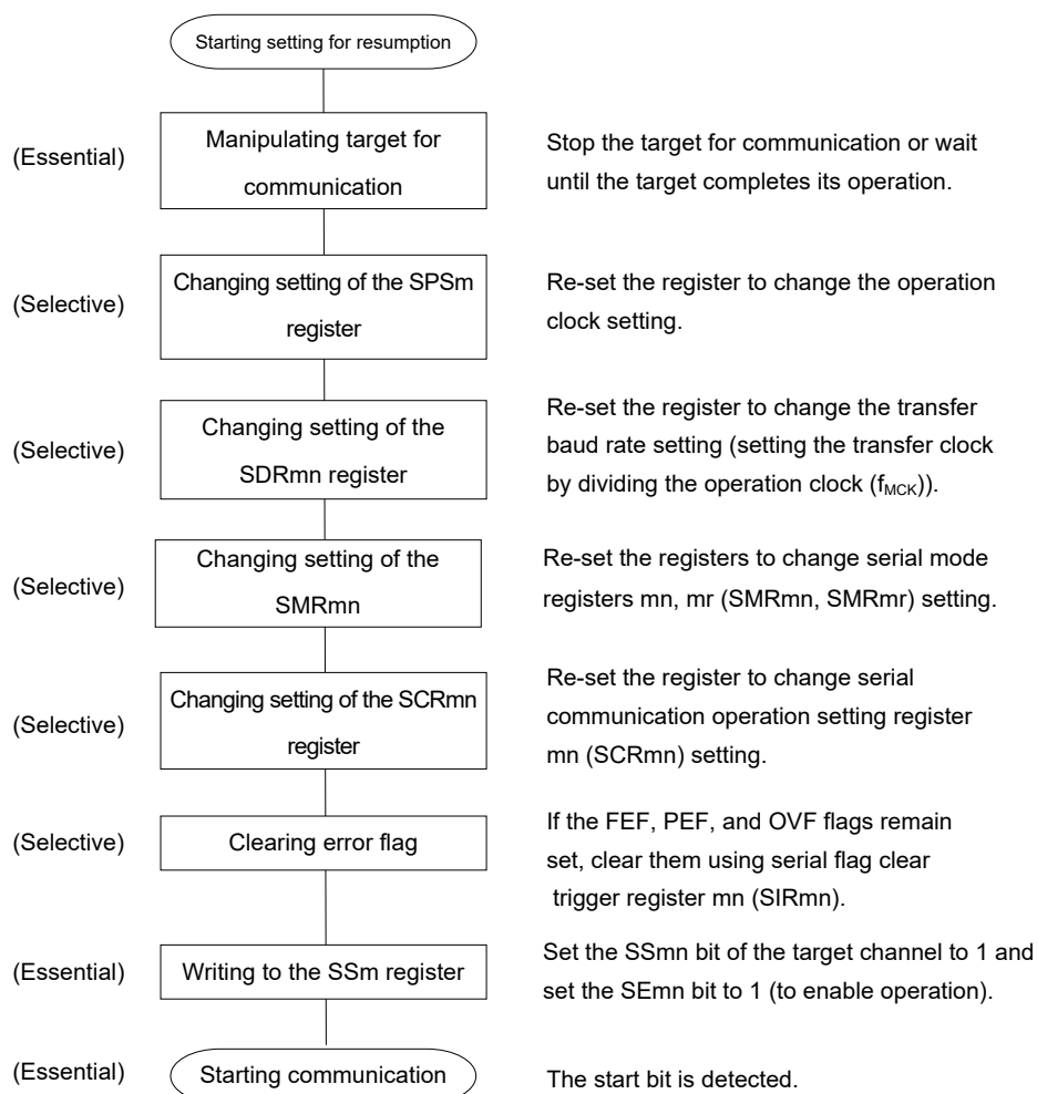
Figure 12-85. Procedure for Resuming UART Reception
