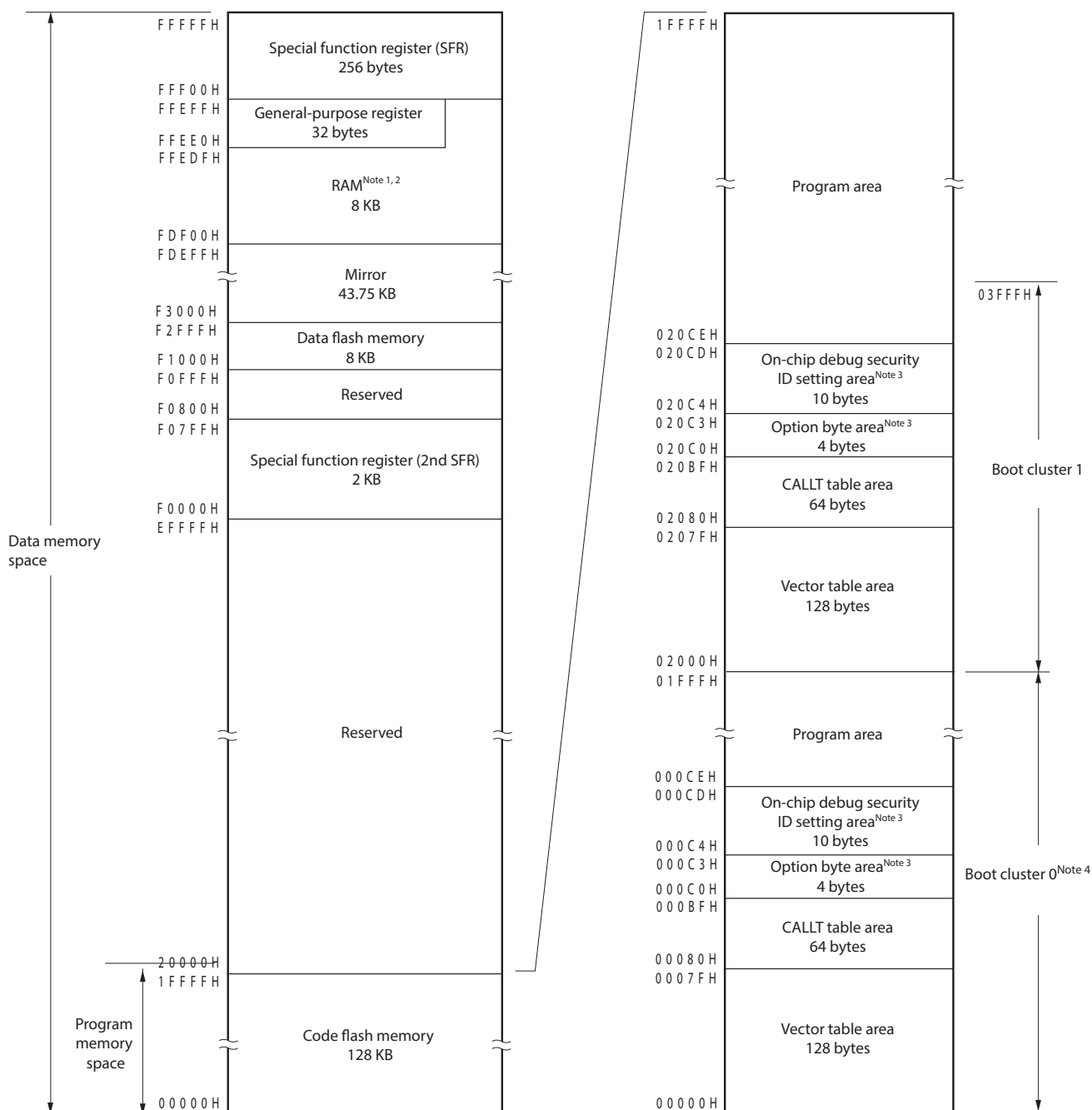
Figure 3-6. Memory Map (R5F10DMG, R5F10DPG)
