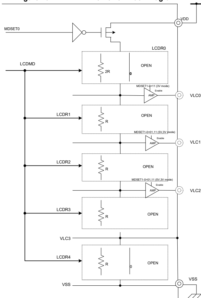
Figure 16-27. LCD Drive Power Block Diagram
