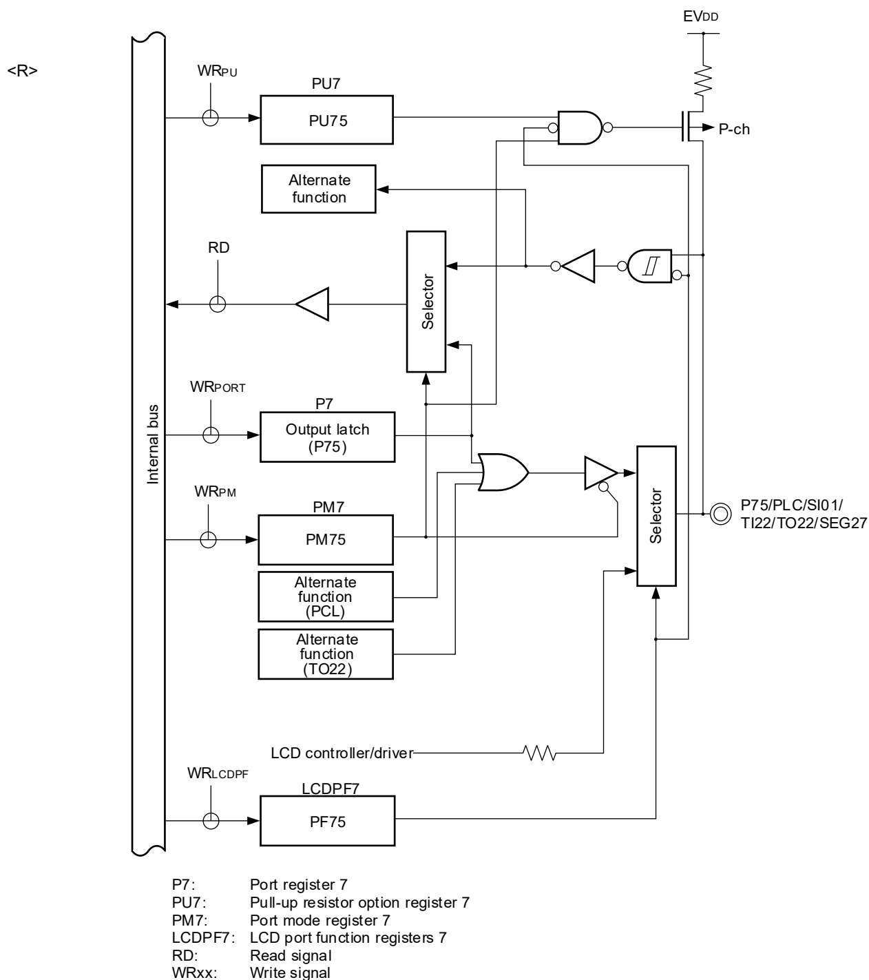
Figure 4-35. Block Diagram of P75
