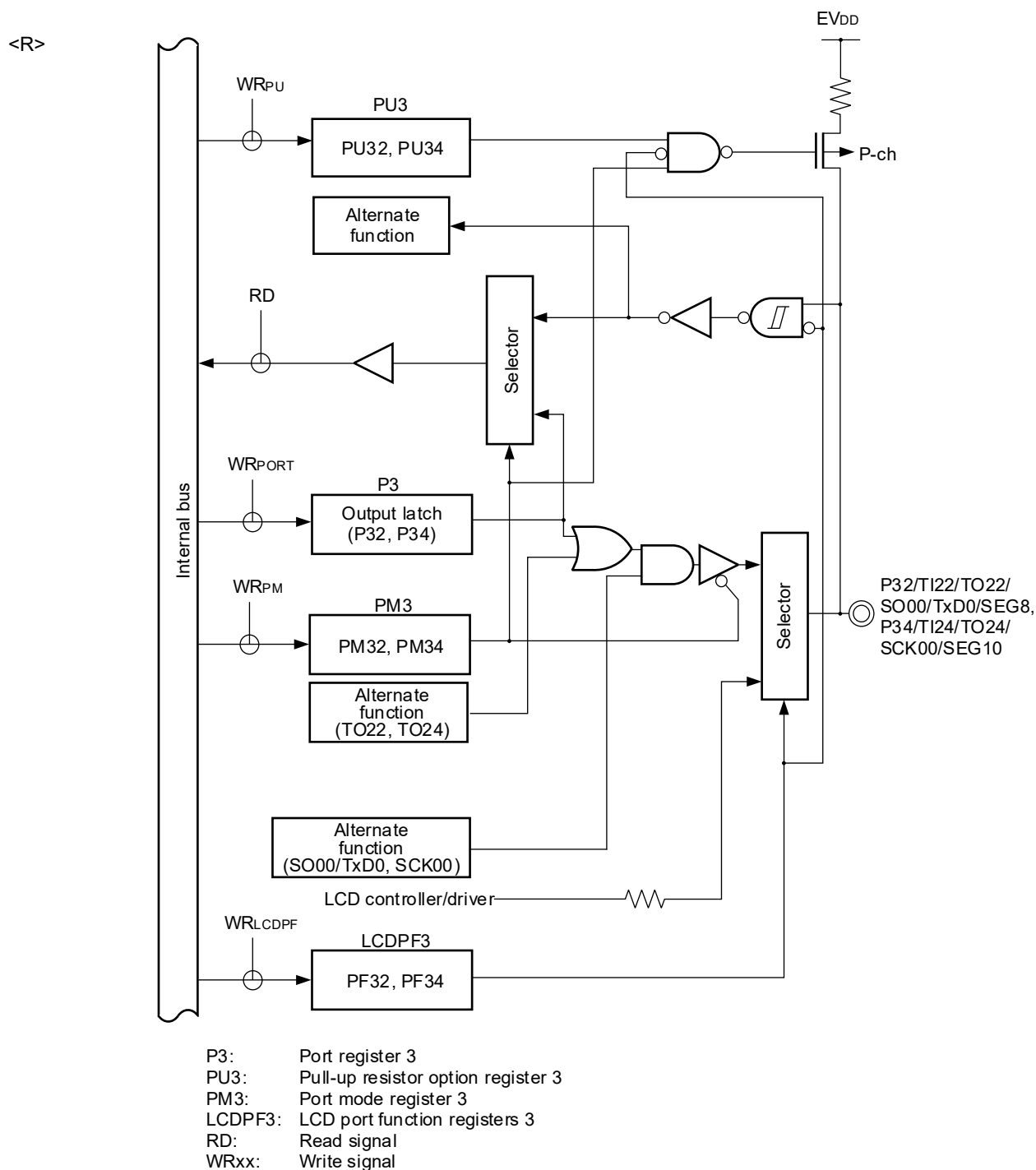
Figure 4-15. Block Diagram of P32, P34
