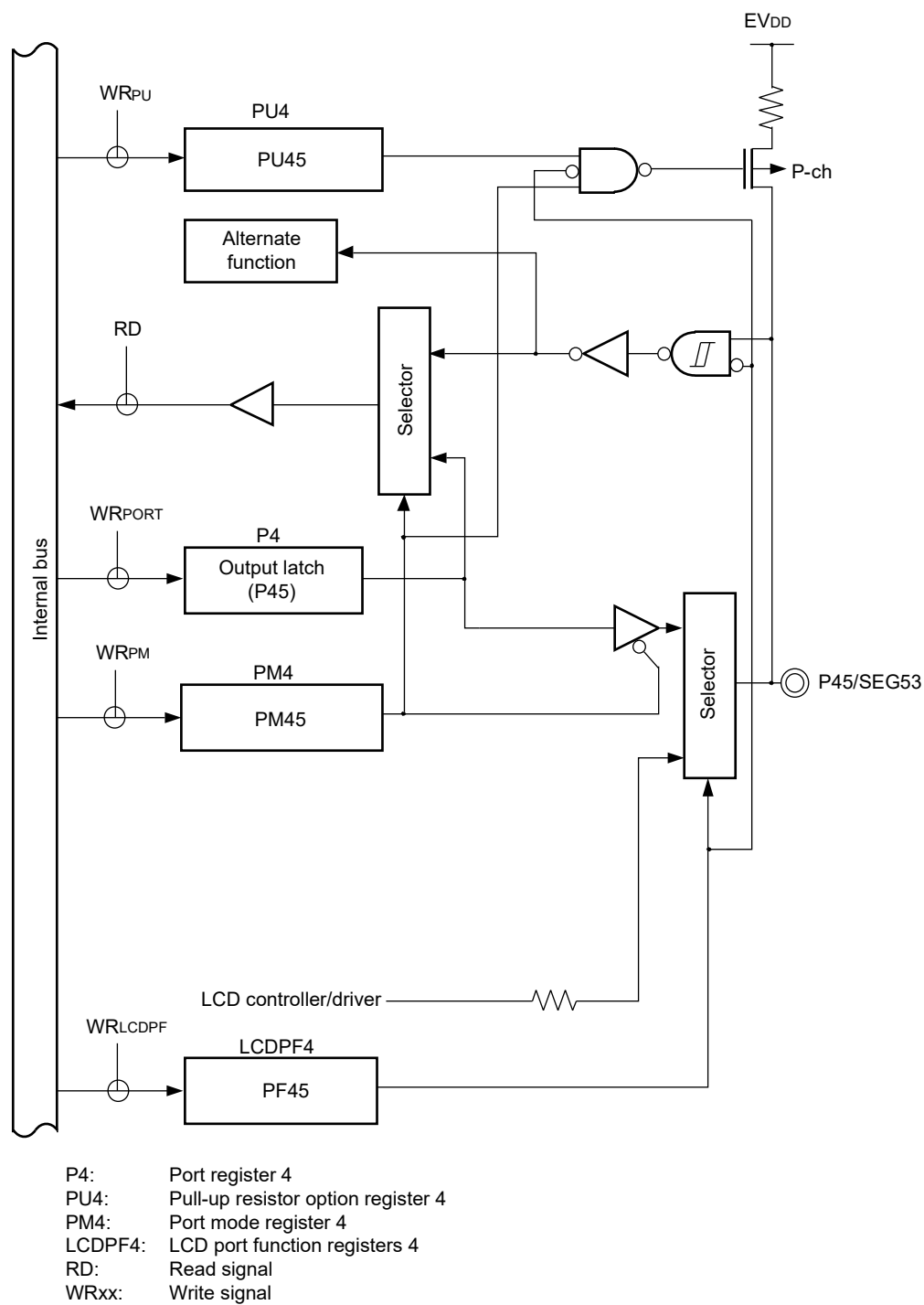
Figure 4-19. Block Diagram of P45
