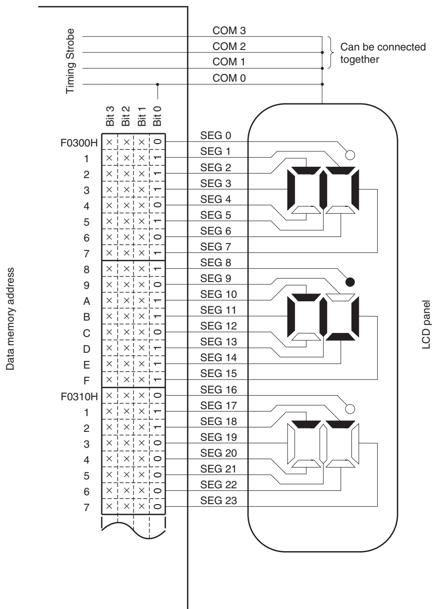
Figure 16-19. Example of Connecting Static LCD Panel
