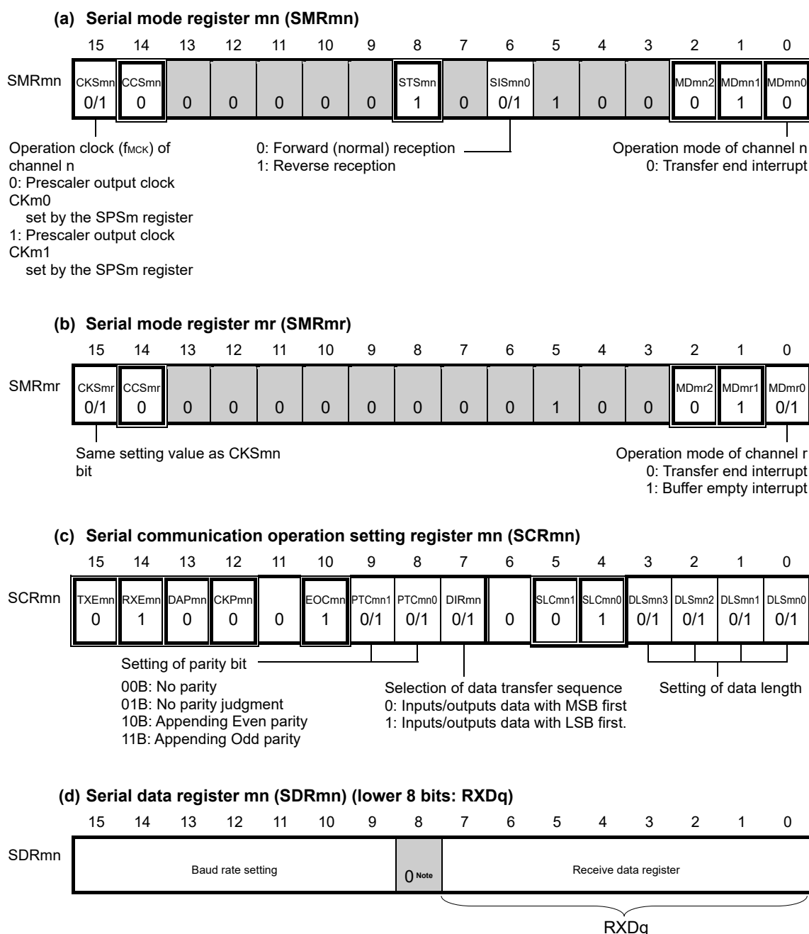
Figure 12-82. Example of Contents of Registers for UART Reception of UART (UART0) (1/2)
