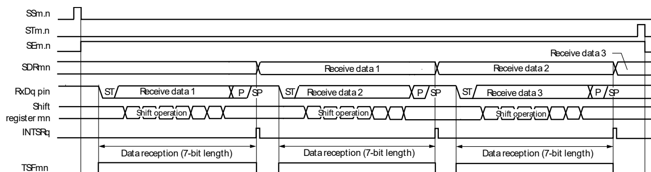
Figure 12-86. Timing Chart of UART Reception
