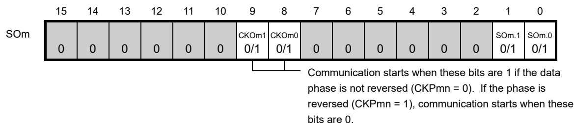
Figure 12-27. Example of Contents of Registers for Master Transmission of 3-Wire Serial I/O (CSI00, CSI01, CSI10) (1/2)
