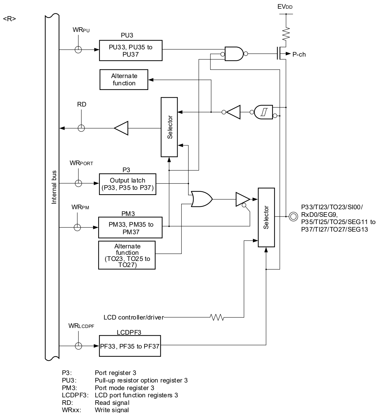
Figure 4-16. Block Diagram of P33, P35 to P37
