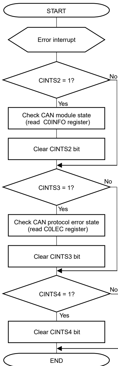
Figure 14-86. Error Handling
