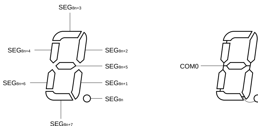
Figure 16-18. Static LCD Display Pattern and Electrode Connections
