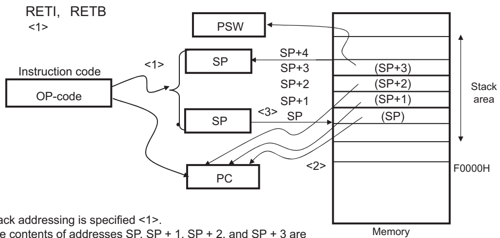
Figure 3-53. Example of RETI, RETB
