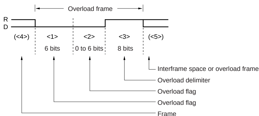
Figure 14-16. Overload Frame
