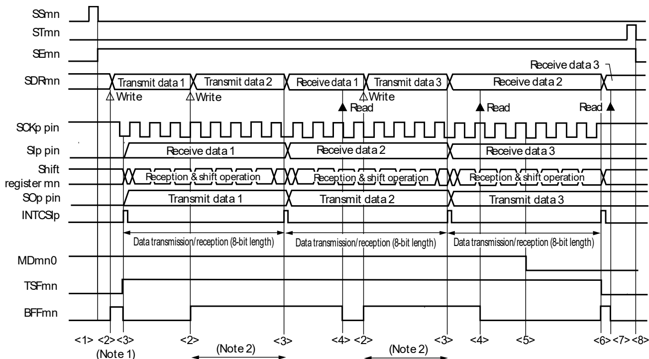
Figure 12-71. Timing Chart of Slave Transmission/Reception (in Continuous Transmission/Reception Mode) (Type 1: DAPmn = 0, CKPmn = 0)
