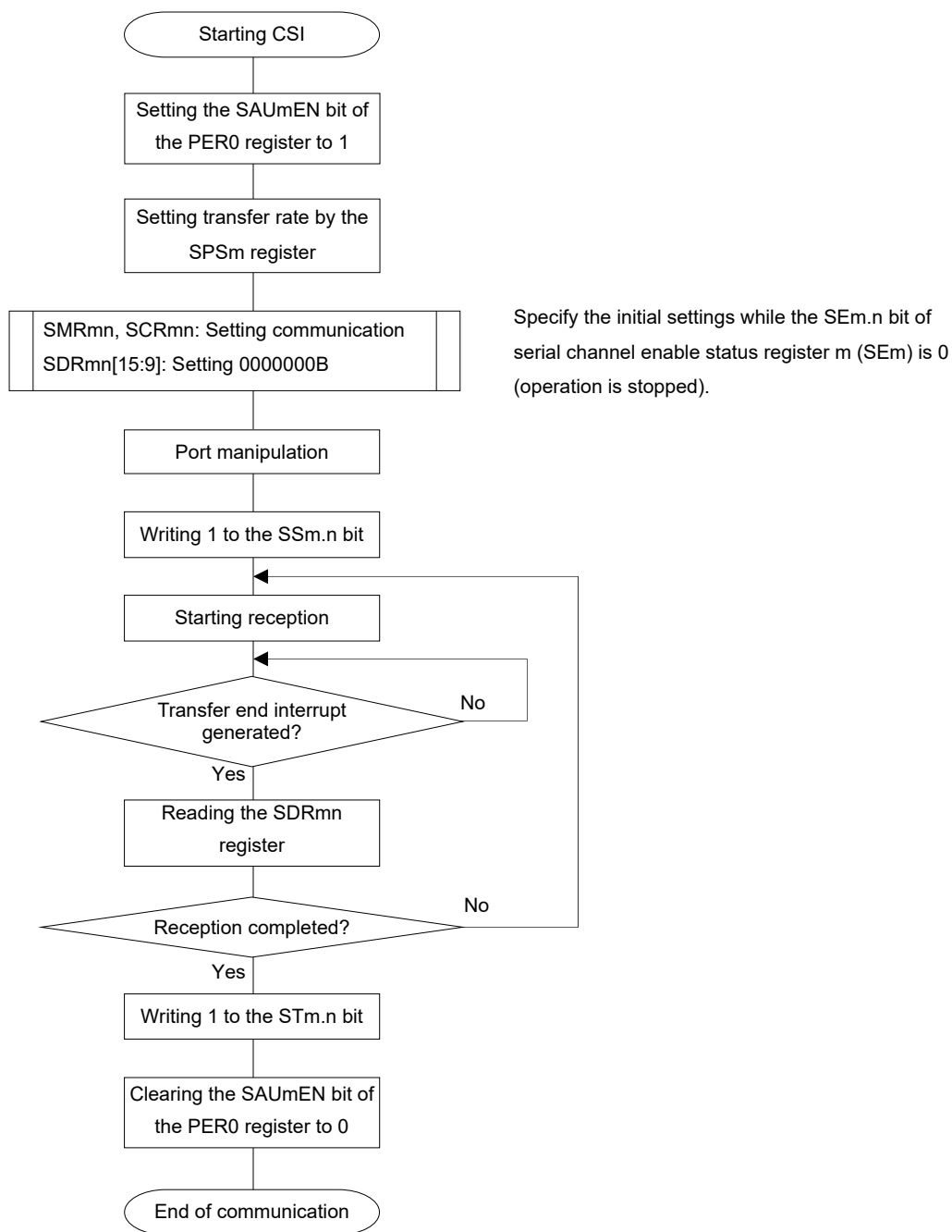
Figure 12-64. Flowchart of Slave Reception (in Single-Reception Mode)
