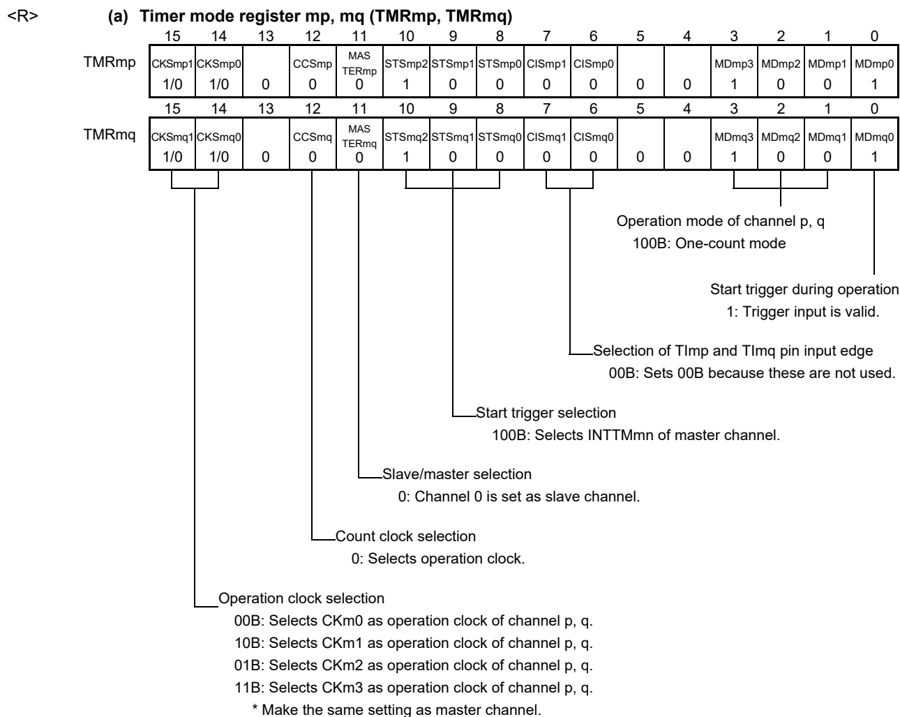
Figure 6-84. Example of Set Contents of Registers When Multiple PWM Output Function (Slave Channel) Is Used (Output Two Types of PWMs) (1/2)
