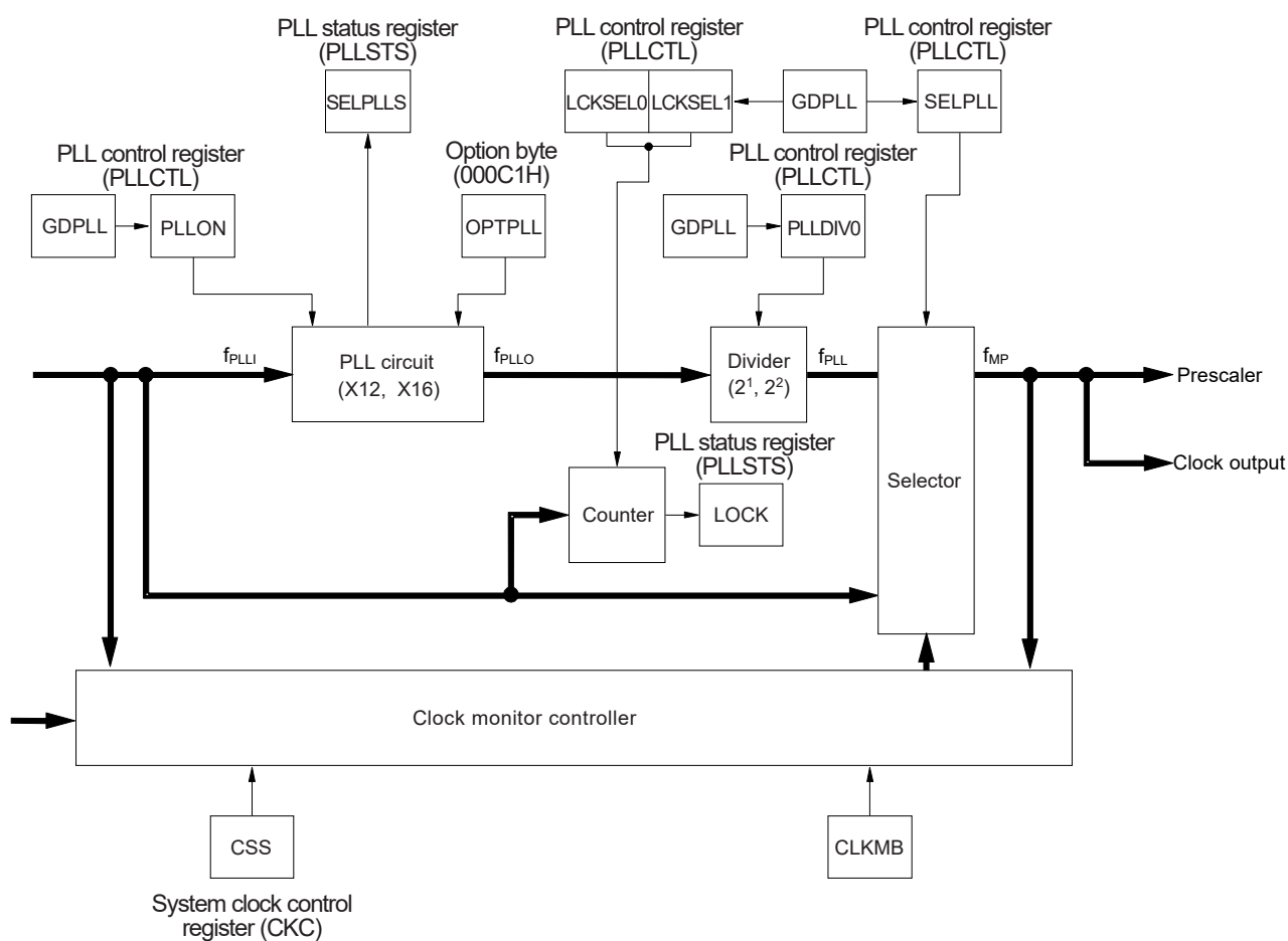
Figure 5-2. Block Diagram of PLL Circuit
