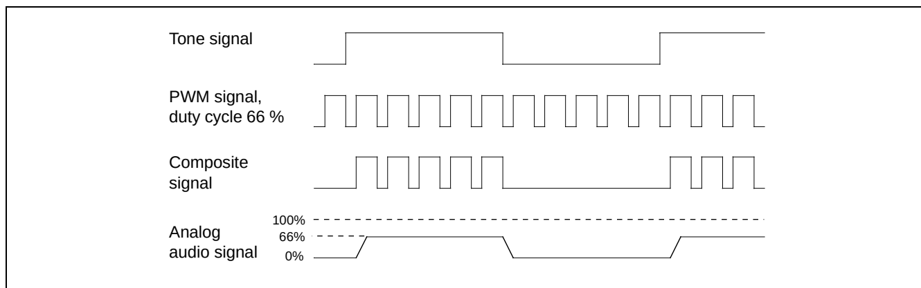
Figure 18-2. Generation of the Composite Output Signal
