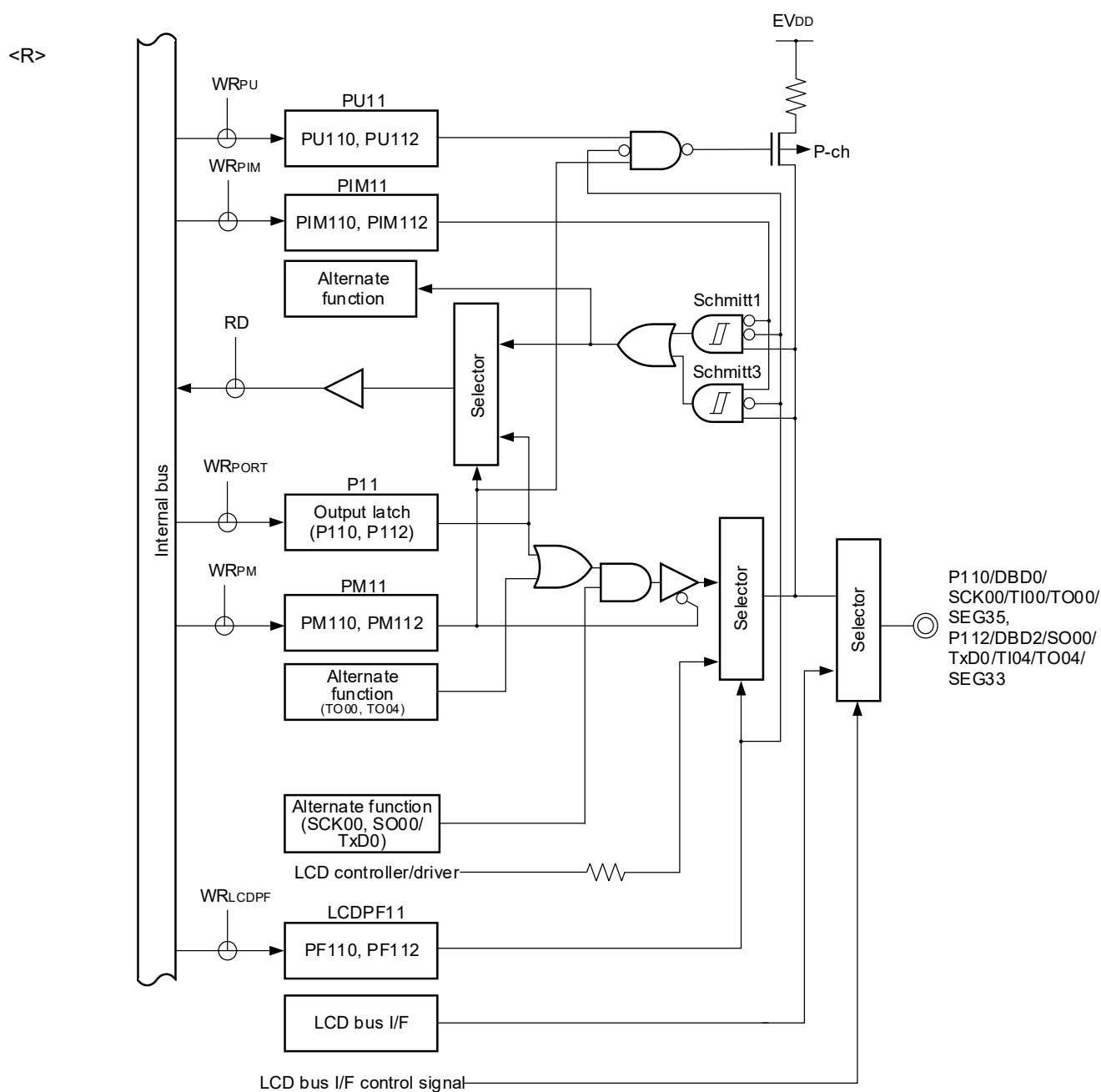
Figure 4-43. Block Diagram of P110 and P112
