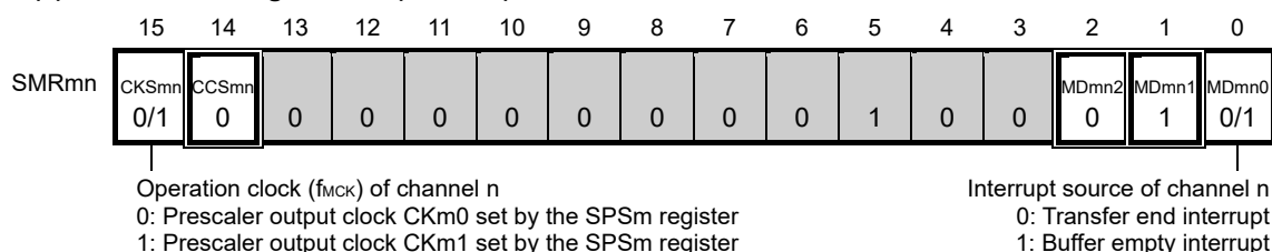
Figure 12-74. Example of Contents of Registers for UART Transmission of UART (UART0) (1/2)
