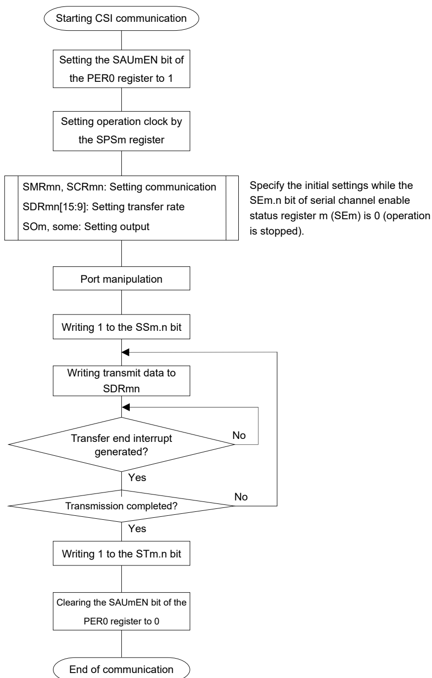
Figure 12-32. Flowchart of Master Transmission (in Single-Transmission Mode)
