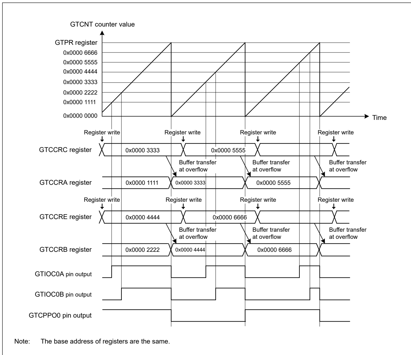
Figure 21.39 Example of saw-wave PWM mode 1 operation with up-counting, buffer operation, high output at GTCCR/GTCCRB compare match, low output at cycle end, and GTIOR.PSYE = 1
