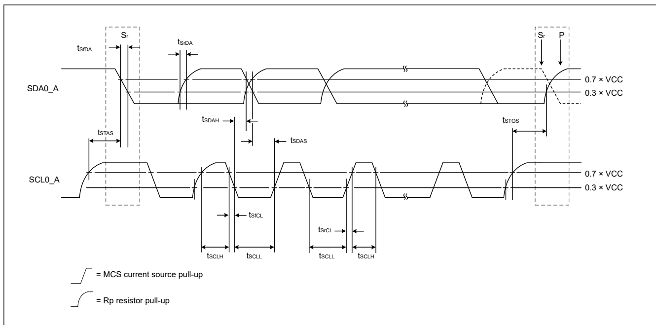
Figure 46.48 I²C bus interface input/output timing (Hs-mode)
