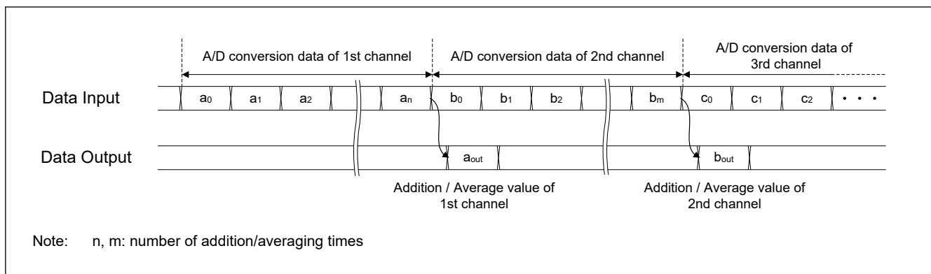
Figure 36.37 Example operation of A/D-converted value addition/averaging function (SAR mode or Oversampling mode)
