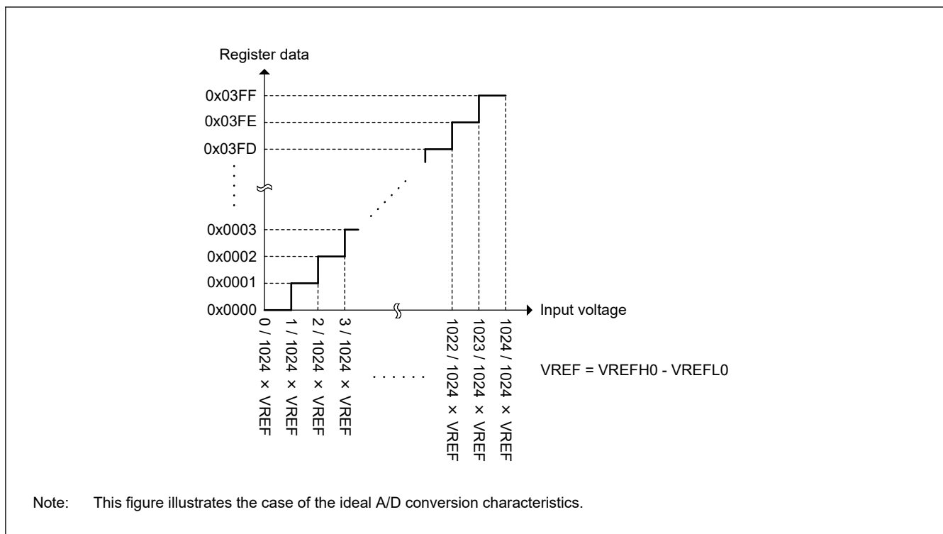
Figure 36.47 Data range of A/D conversion result (10-bit data length, Unsigned data, Single-ended input)
