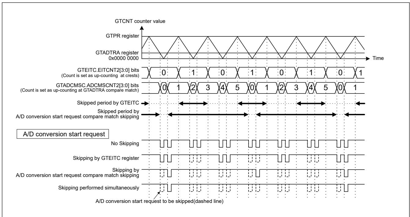
Figure 21.158 Example of A/D Conversion Start Request Compare Match Skipping Function Operation (Extended Interrupt Skipping: EIVTC2[1:0] = 01b, EADTAL[2:0] = 01b, A/D Conversion Start Request Compare Match Skipping: ADCMSC2[1:0] = 01b, ADCMSAL[2:0] = 010b)
