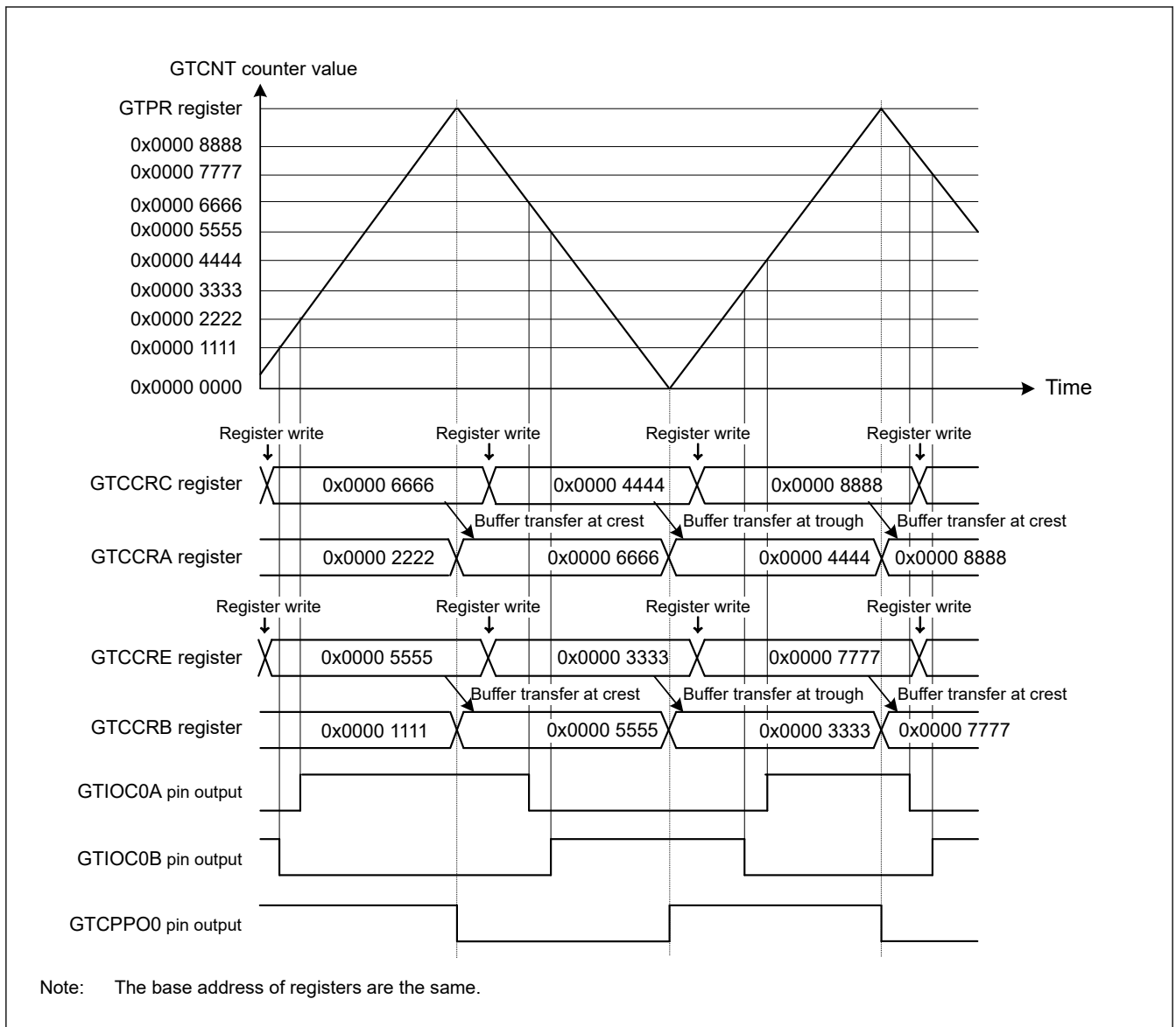
Figure 21.45 Example of triangle-wave PWM mode 2 operation with buffer operation, low output from the GTIOA pin and high output from the GTIOB pin at count start, output toggled at GTCCRA/ GTCCRB compare match, output retained at cycle end, and GTIOR.PSYE = 1
