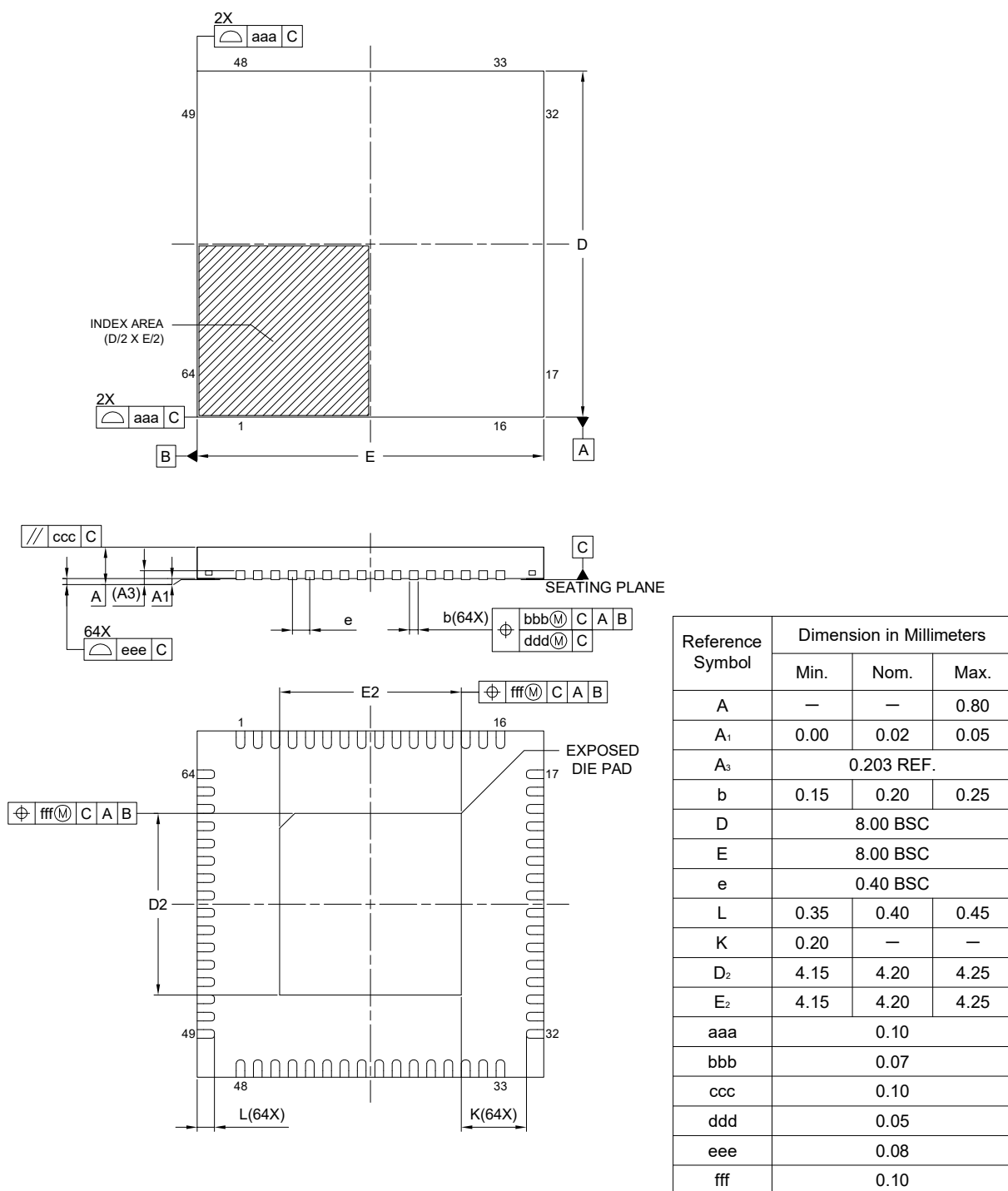
Figure A2.3 QFN 64-pin
