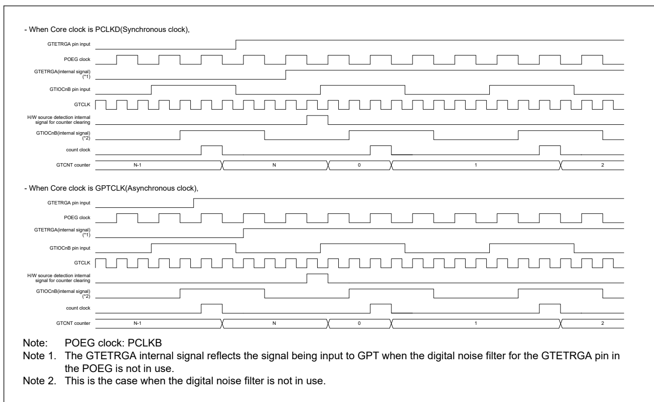
Figure 21.101 Examples of the Timing of Operations for Counter Clearing in Response to a Rising Edge of the Input on the GTETRG Pin (During Counting Triggered by Hardware Source)
