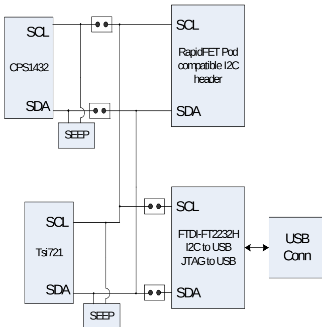
Figure 13: I2C Block Diagram
