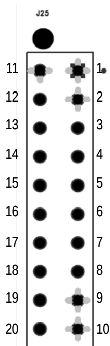
Figure 24: J25 - ATX Power Connector Pinout
