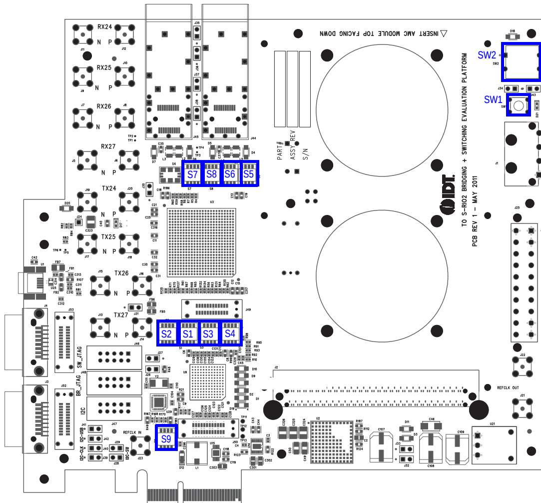
Figure 14: Switch Locations
