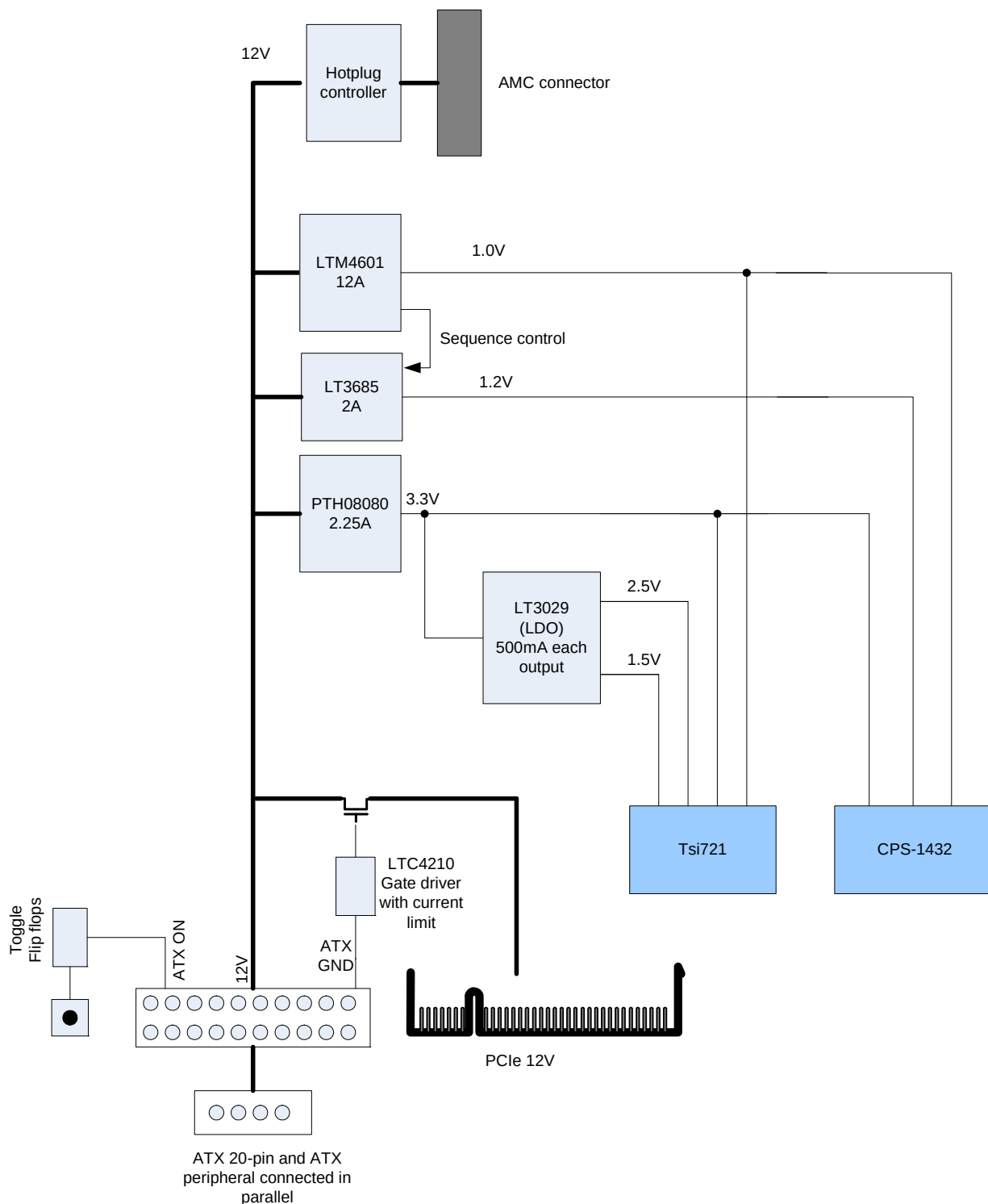
Figure 10: Voltage Regulators
