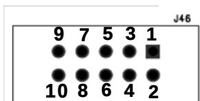
Figure 26: J46, J48 - JTAG Header
