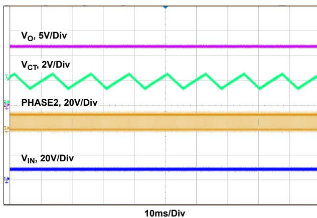
Figure 30. Dither V_{IN} , V_O , V_{CT} (CLKOUT/DITHER pin voltage), V_{IN} = 10V , V_O = 12V , I_{OUT} = 5A
