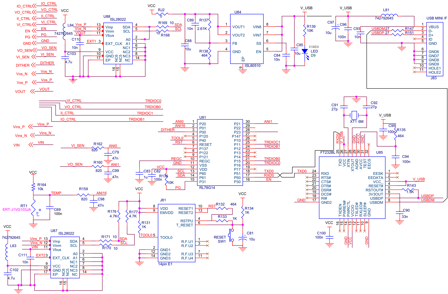
Figure 21. RL78G14 Schematic
