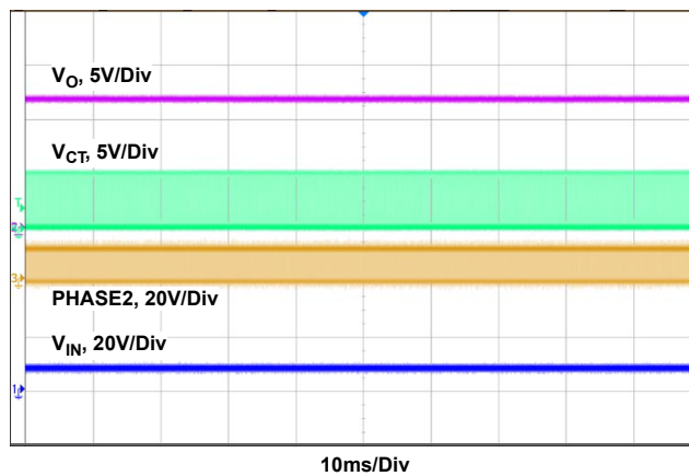
Figure 31. Normal V_{IN} , V_O , V_{CT} (CLKOUT/DITHER pin voltage), V_{IN} = 10V , V_O = 12V , I_{OUT} = 5A
