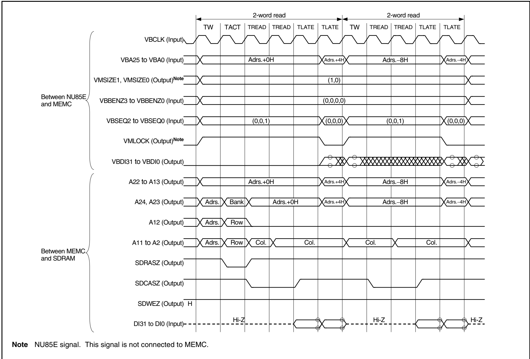
Figure 2-29. Refill Timing Example from SDRAM to Data Cache (Critical First Refill (2R-2R))
