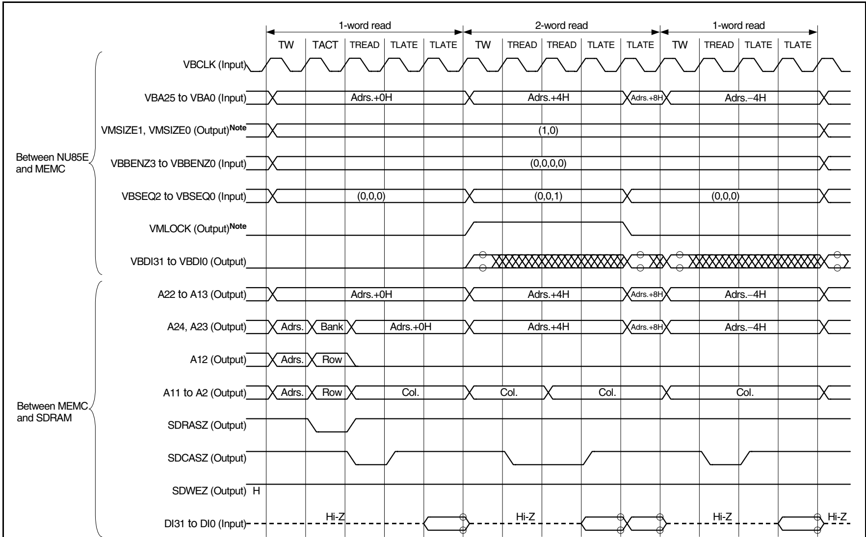
Figure 2-30. Refill Timing Example from SDRAM to Data Cache (Critical First Refill (1R-2R-1R))
