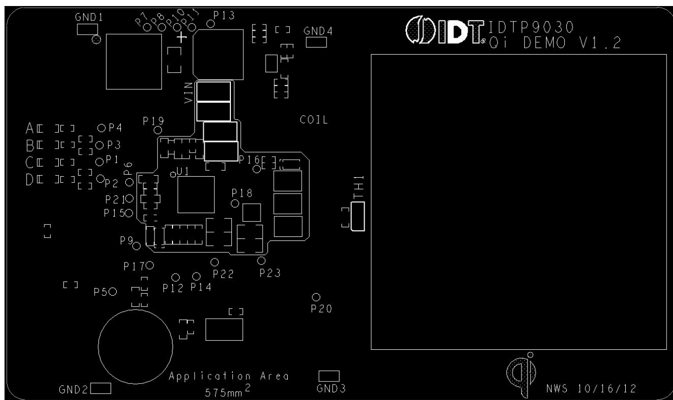
Figure 14. Top Silkscreen
