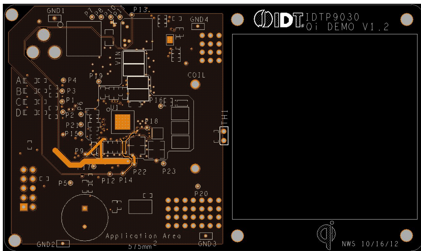
Figure 18. Mid 1 Layer
