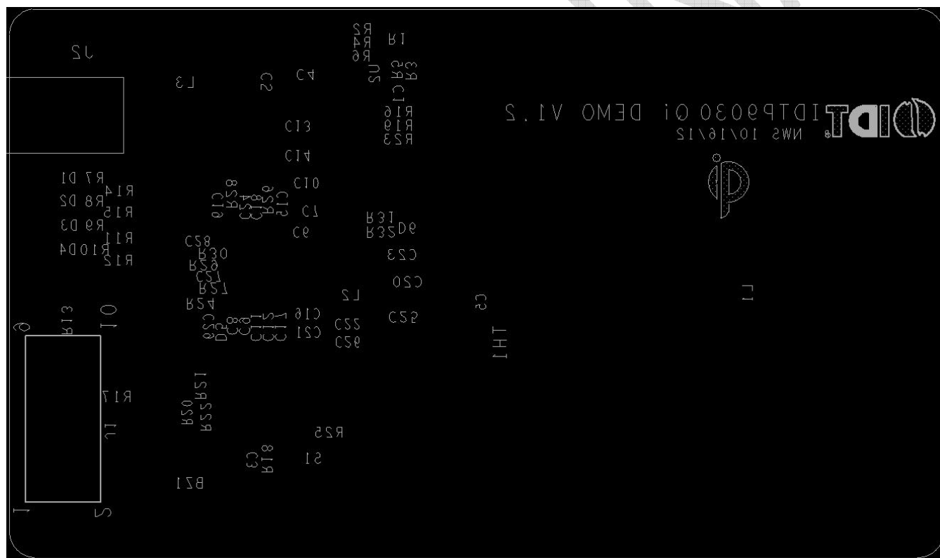
Figure 15. Bottom Silkscreen.
