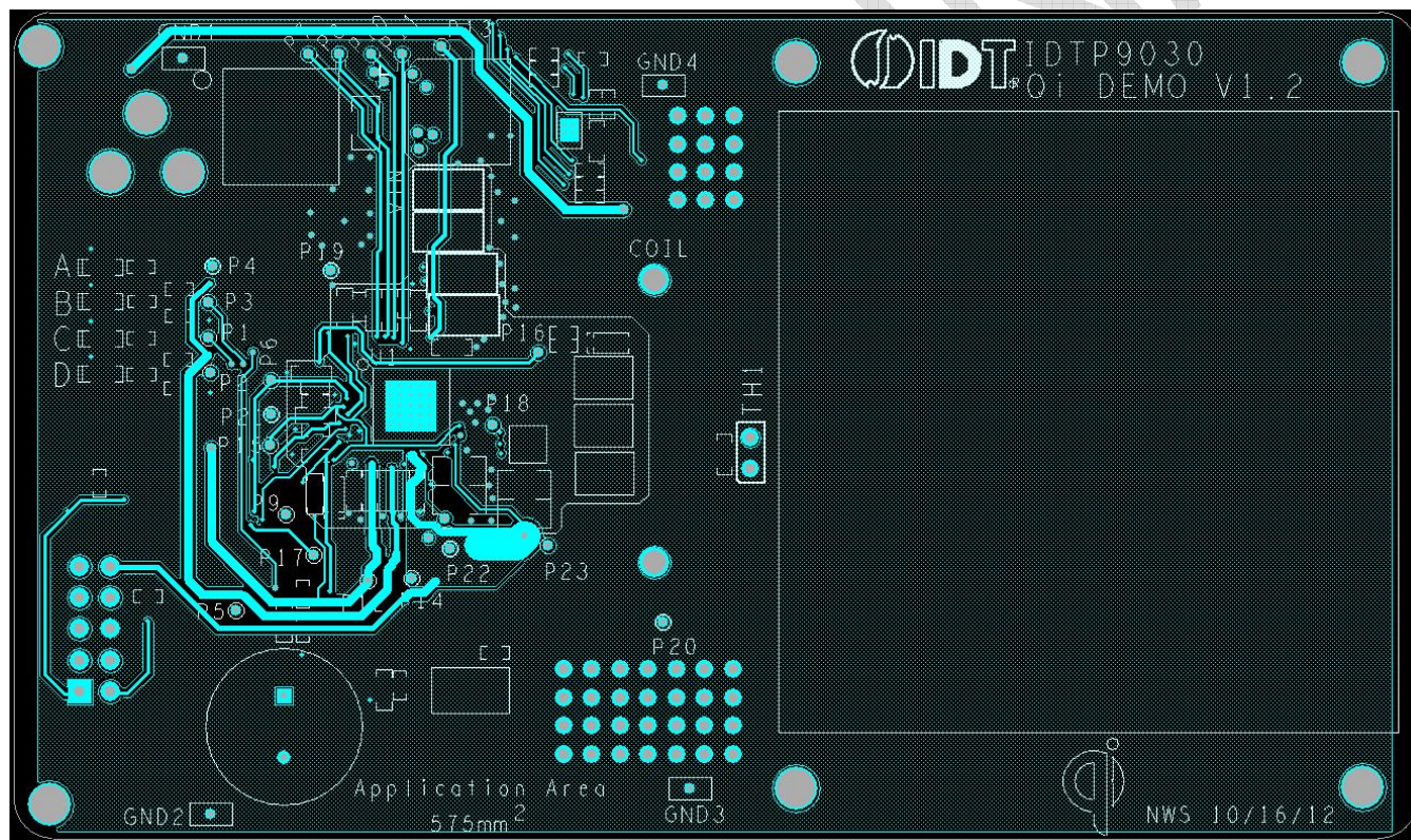
Figure 19. Mid 2 Layer
