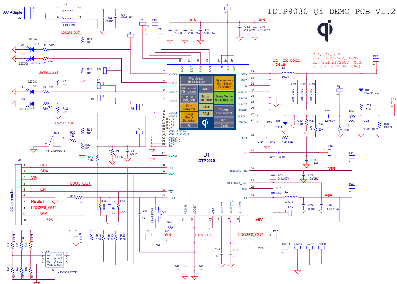
Figure 13. IDTP9030 Eval Kit Board Schematic
