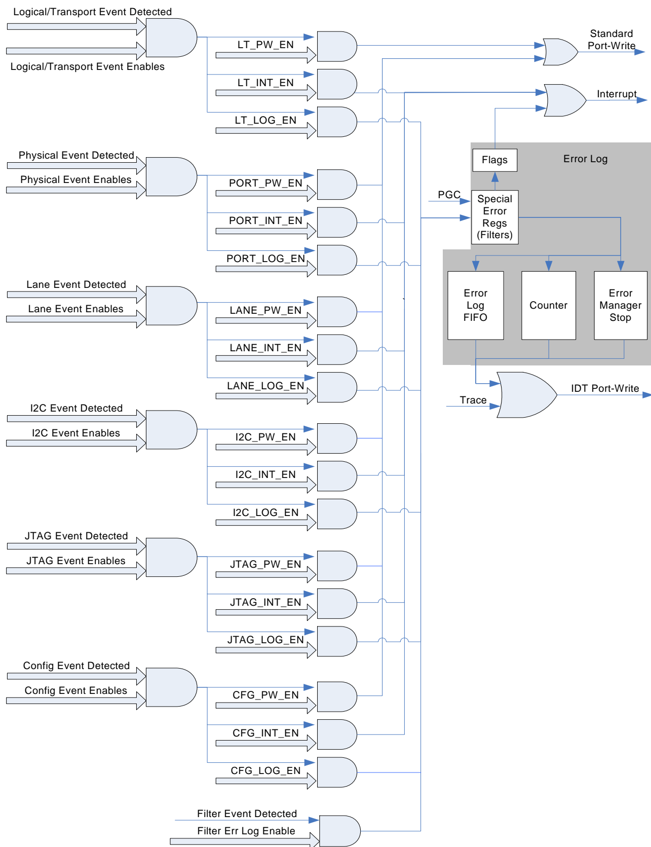
Figure 17: Event Management Overview (Revision A/B)
