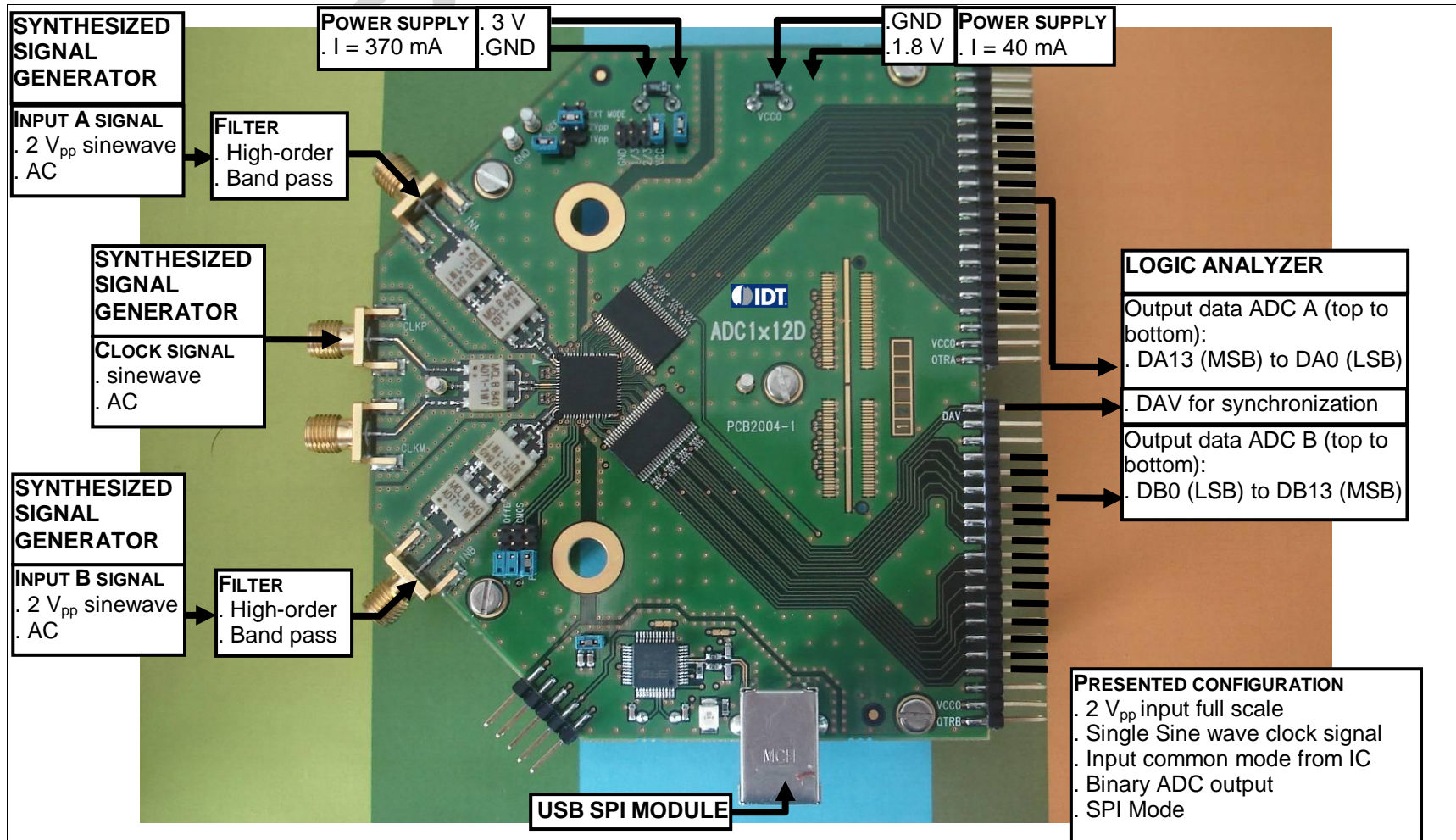
Fig 1. ADC1412D series typical configuration set-up (e.g. demoboard F1/DB)
