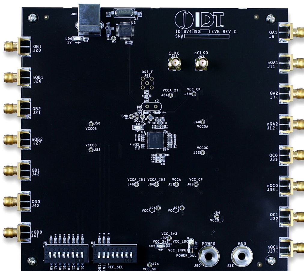
Figure 1. 8V49NS0412 Evaluation Board Diagram
