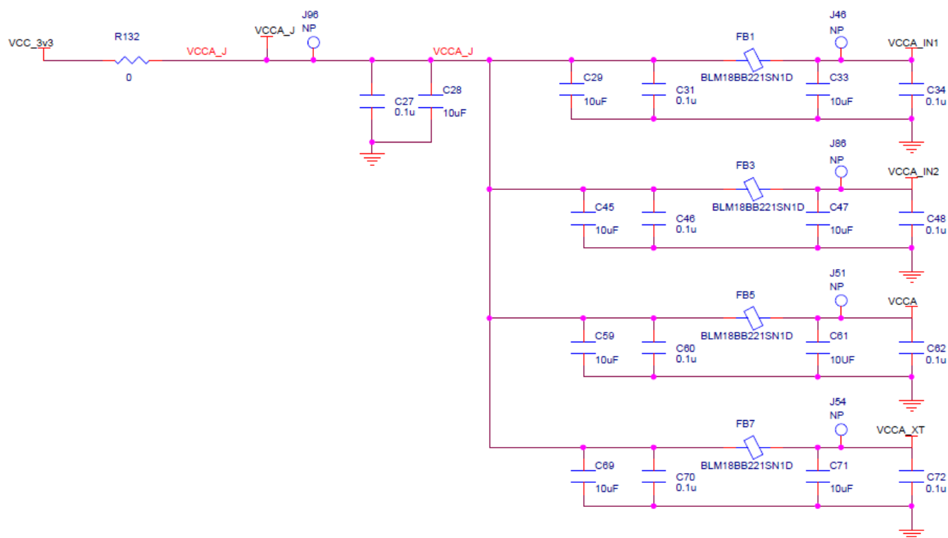
Figure 9. VCC Filtering
