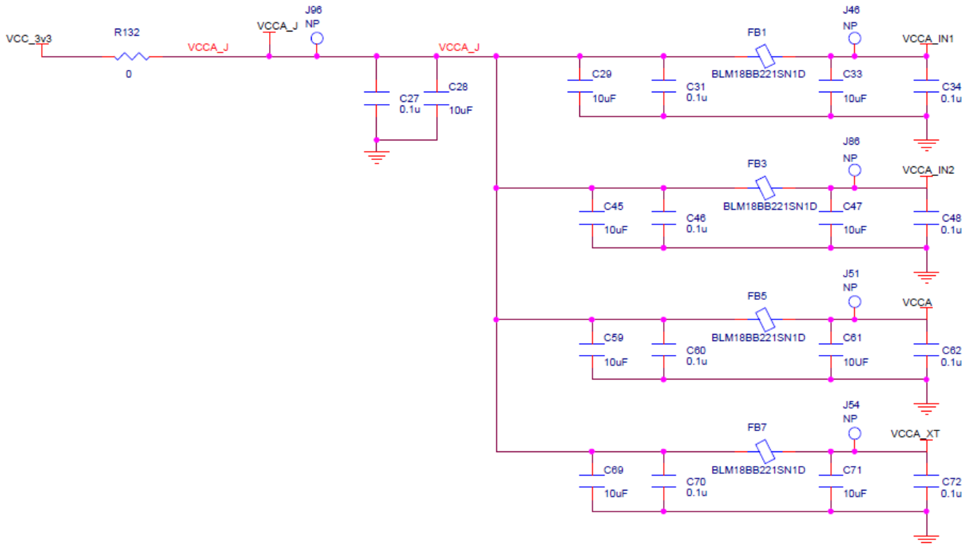
Figure 8. VCC Filtering
