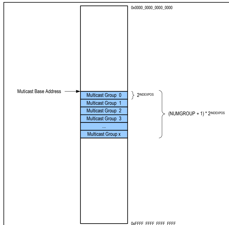
Figure 14.1 Multicast Group Address Ranges
