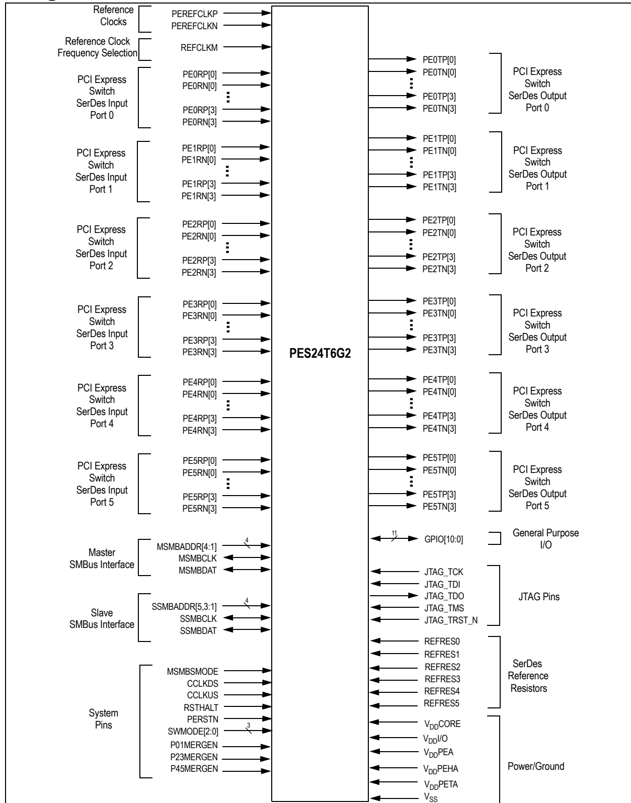
Figure 1.2 PES24T6G2 Logic Diagram
