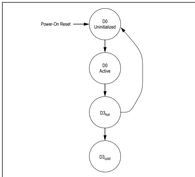
Figure 6.1 PES24T6G2 Power Management State Transition Diagram
