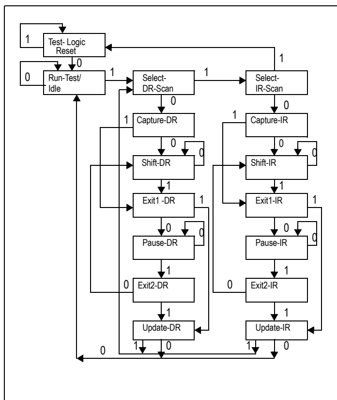
Figure 9.2 State Diagram of PES24T6G2's TAP Controller
