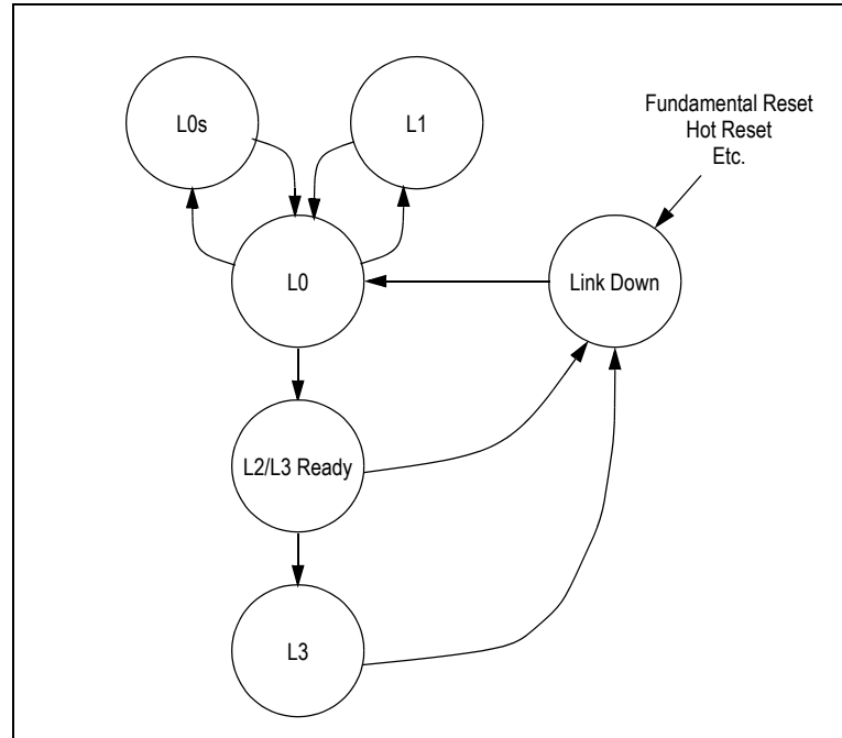
Figure 3.3 PES24T6G2 ASPM Link State Transitions
