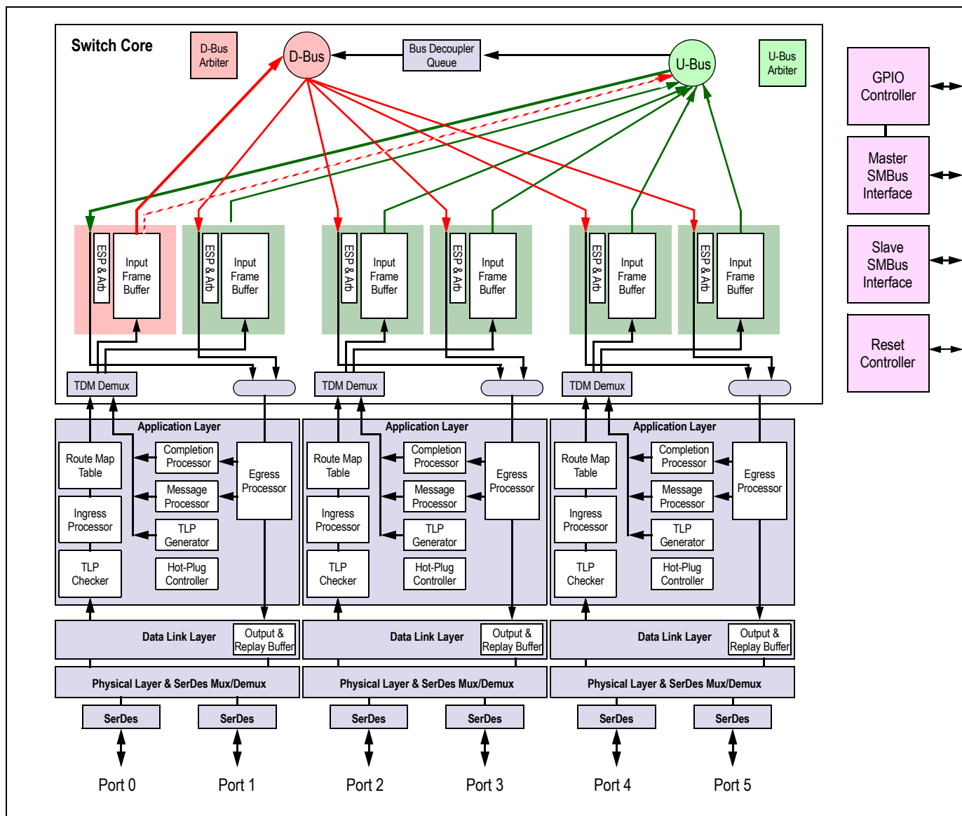
Figure 1.1 PES24T6G2 Architectural Block Diagram
